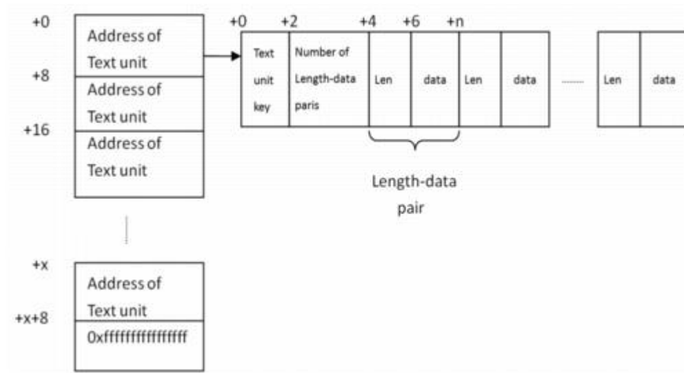
Figure 1-1 Text Unit Pointer Lists and text Units
