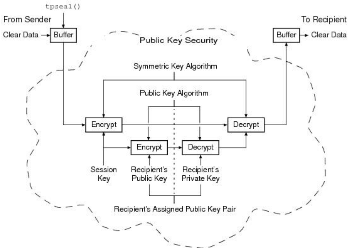
Figure 1-10 ATMI PKCS-7 End-to-End Encryption
