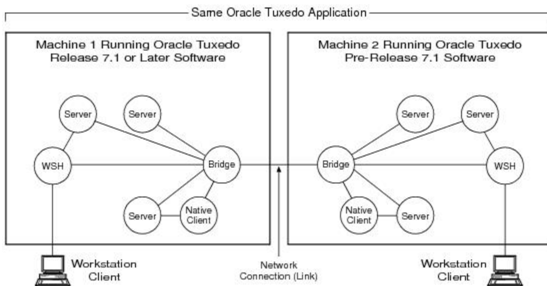
Figure 1-13 Intra-Domain Interoperability
