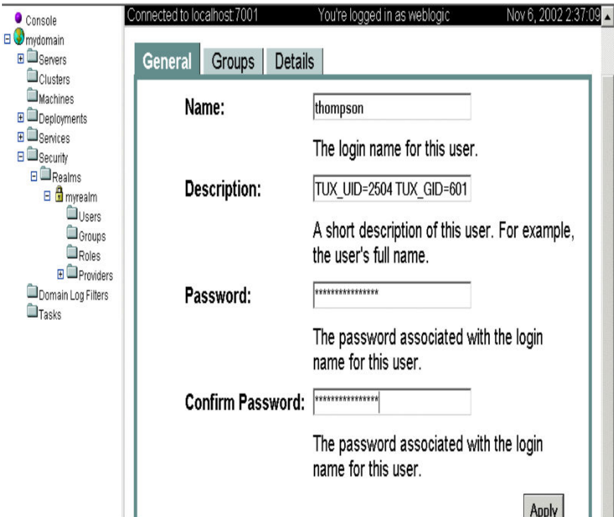
Figure 4-2 WebLogic Administration Console Create Users
