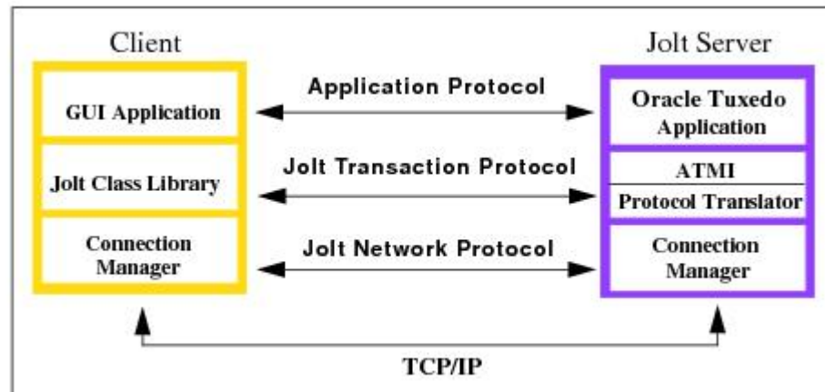
Figure 4-1 Jolt Client/Server Relationship
