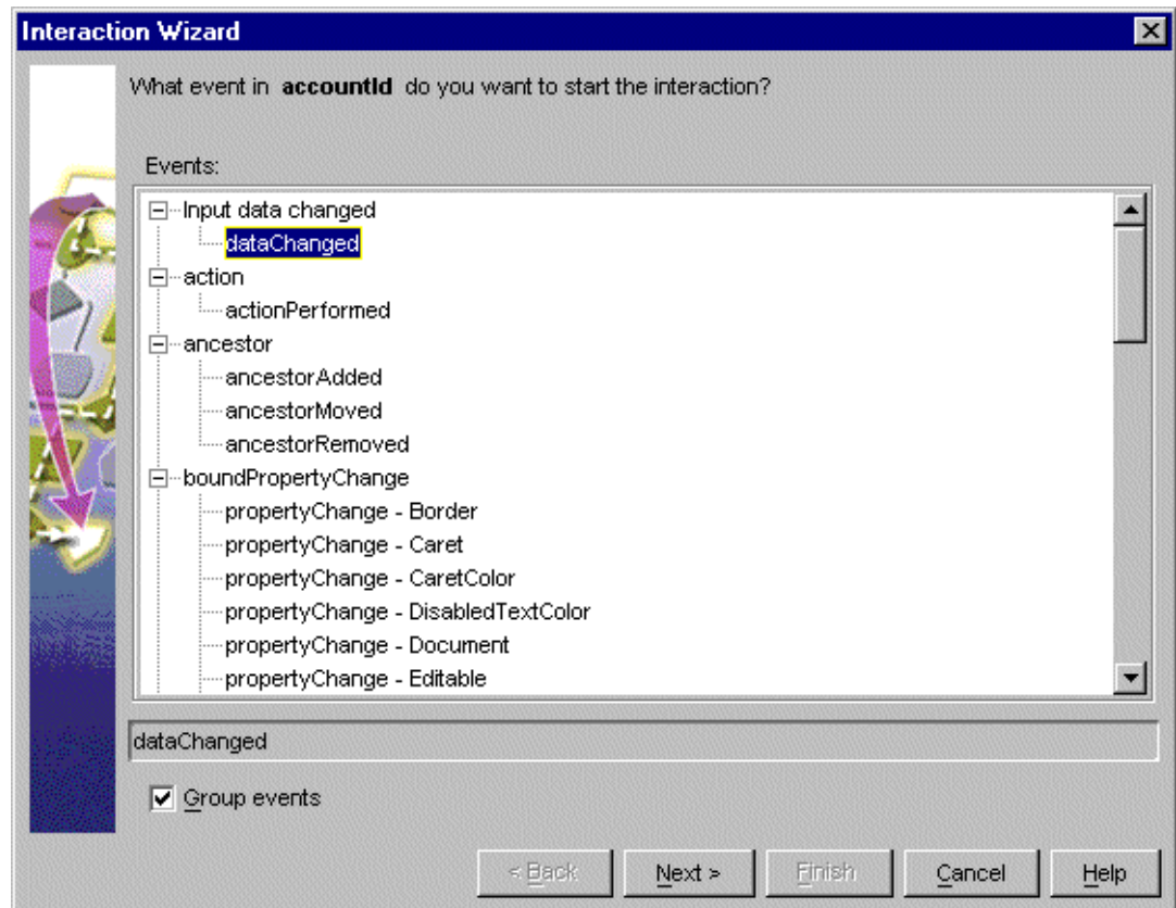
Figure 5-18 Select dataChanged Event
