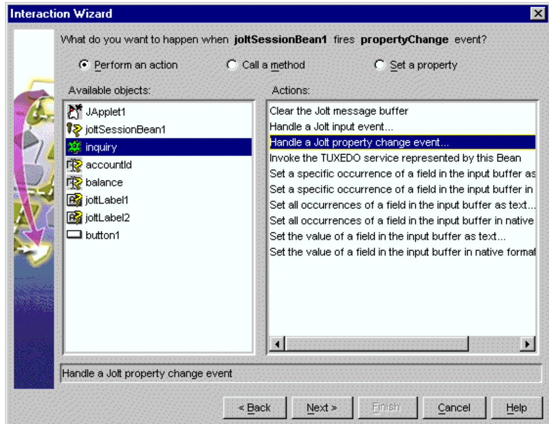
Figure 5-19 Select inquiry Object and Handle a Jolt input event Action
