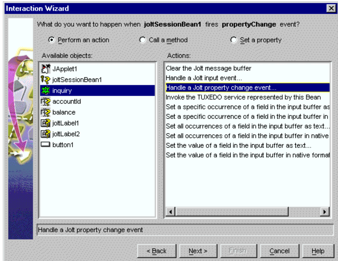
Figure 5-22 Select inquiry Object and Invoke the TUXEDO Service... Action
