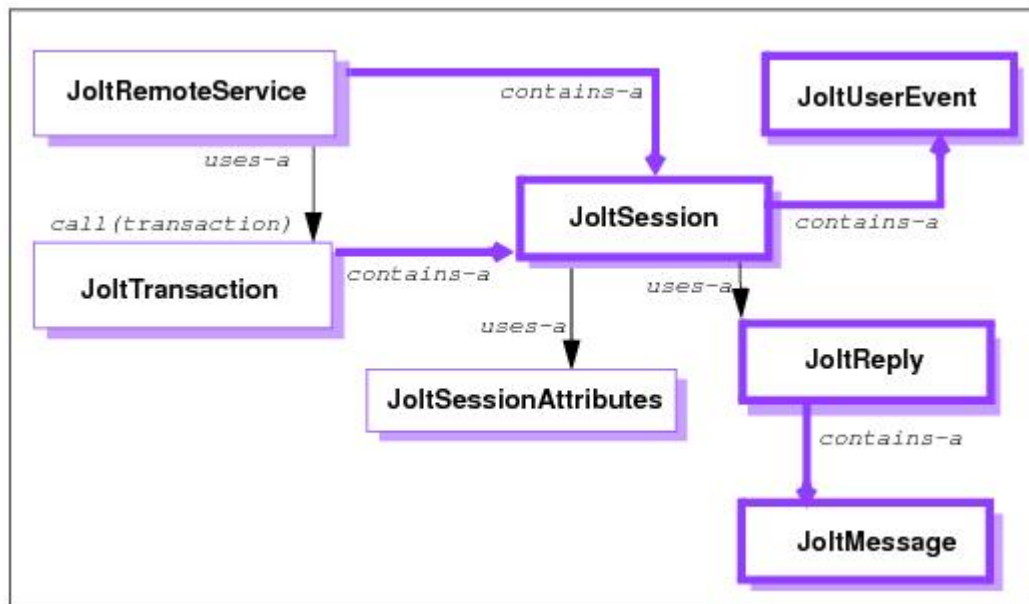
Figure 4-2 Jolt Object Relationships
