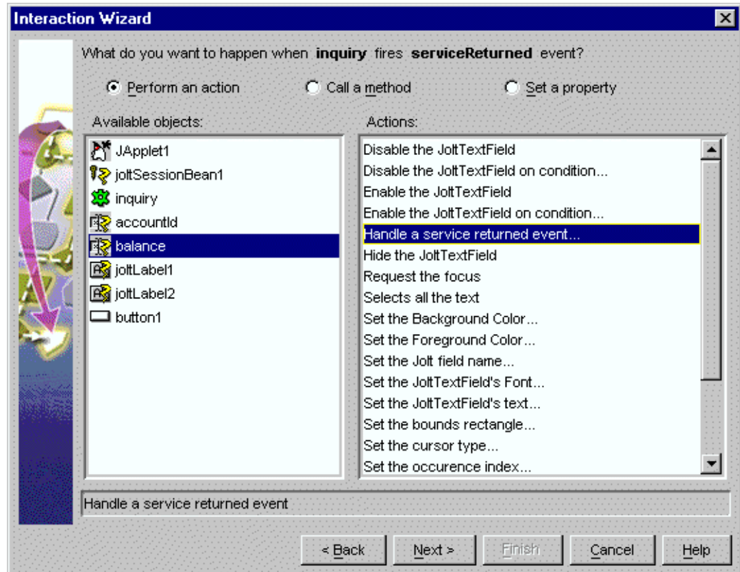
Figure 5-24 Select balance Object and Handle a service returned event Action
