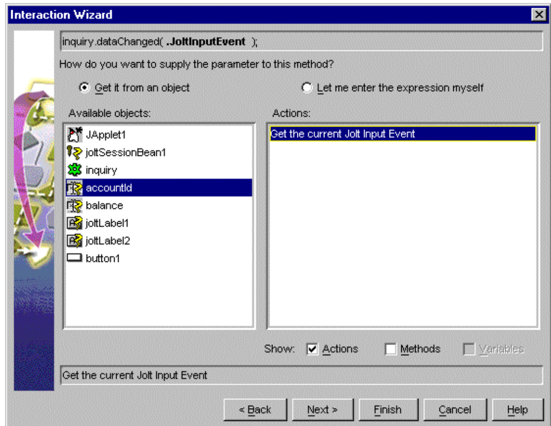
Figure 5-20 Select accountId Object and Get the current Jolt Input Event Action
