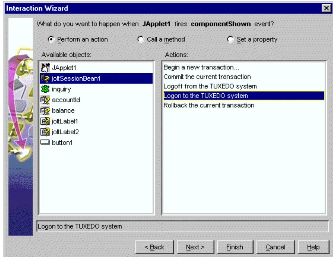
Figure 5-13 Select Logon to the Tuxedo System Action
