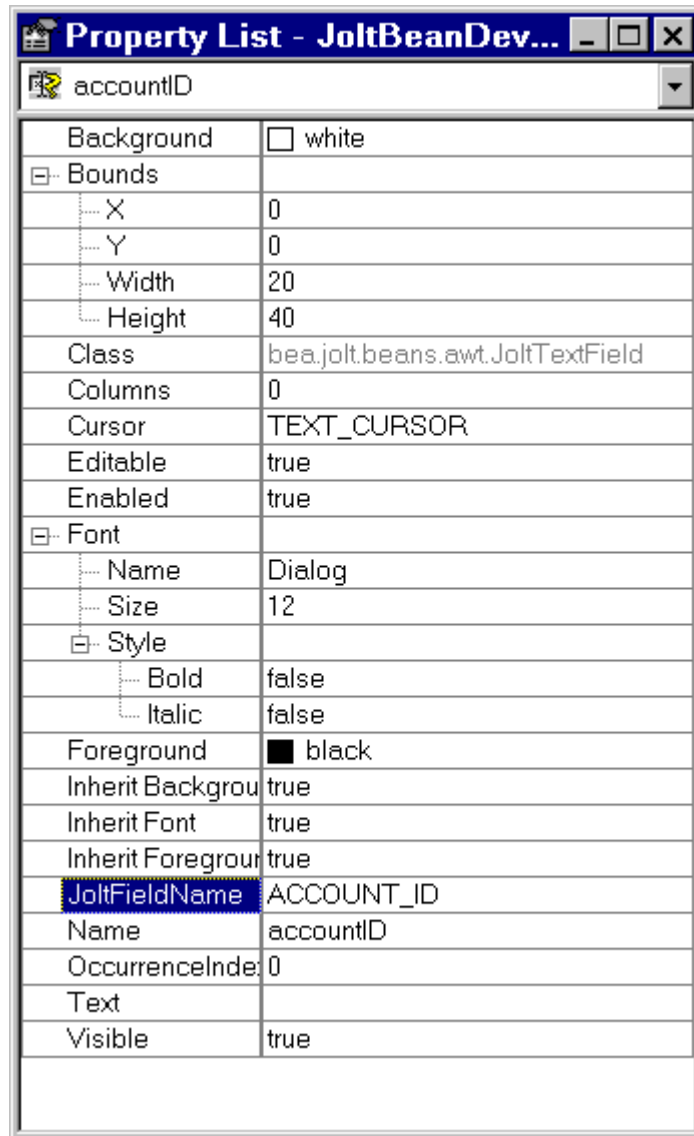
Figure 5-8 Revised JoltFieldName in the JoltTextField Property List
