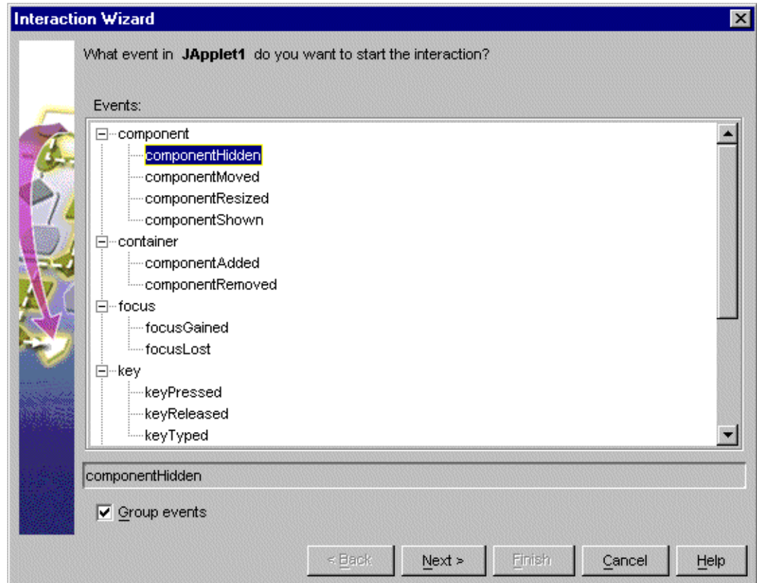
Figure 5-26 Select componentHidden Event
