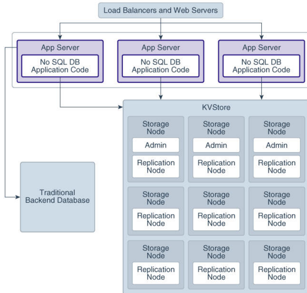
Figure 1-1 Typical Architecture for Oracle NoSQL Database Store
