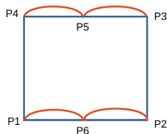
Figure 11-3 Approximating a Search within a GeoJson Box
