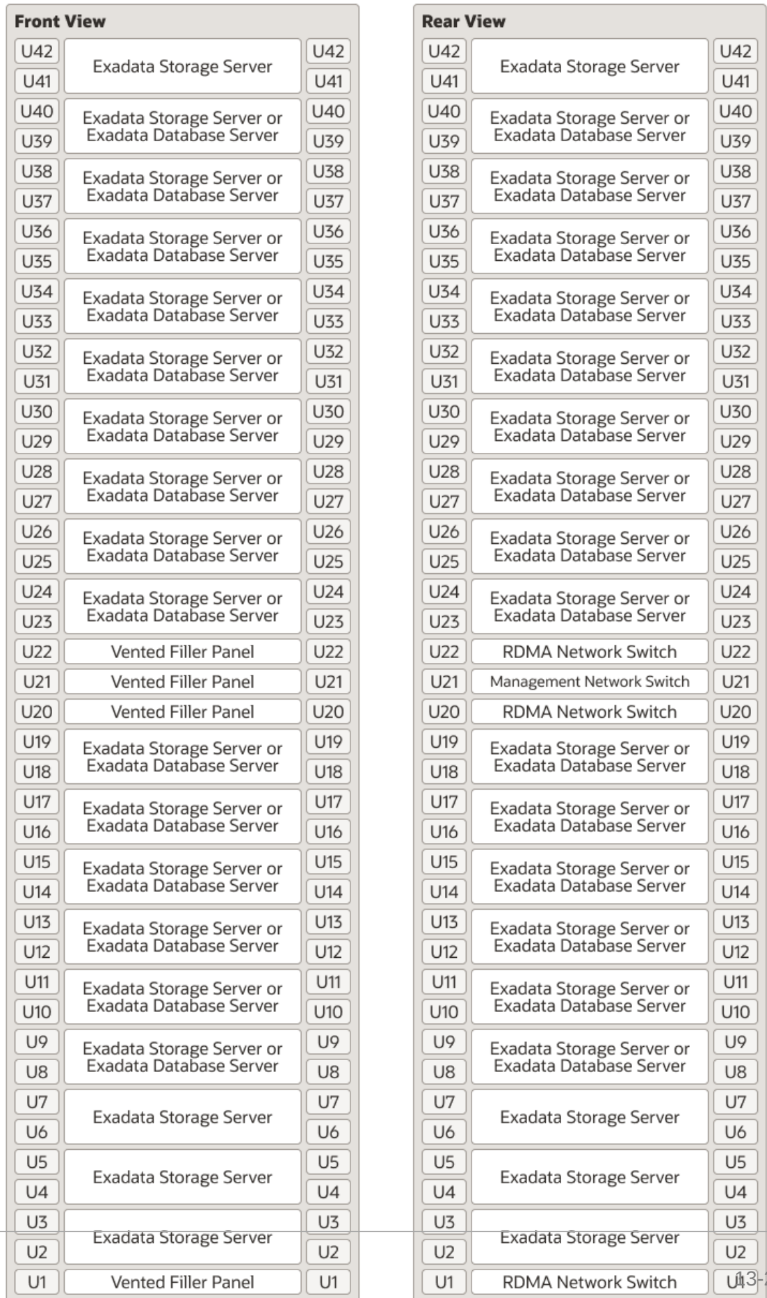
Figure 13-1 Rack Layout for Oracle Exadata Database Machine X10M
