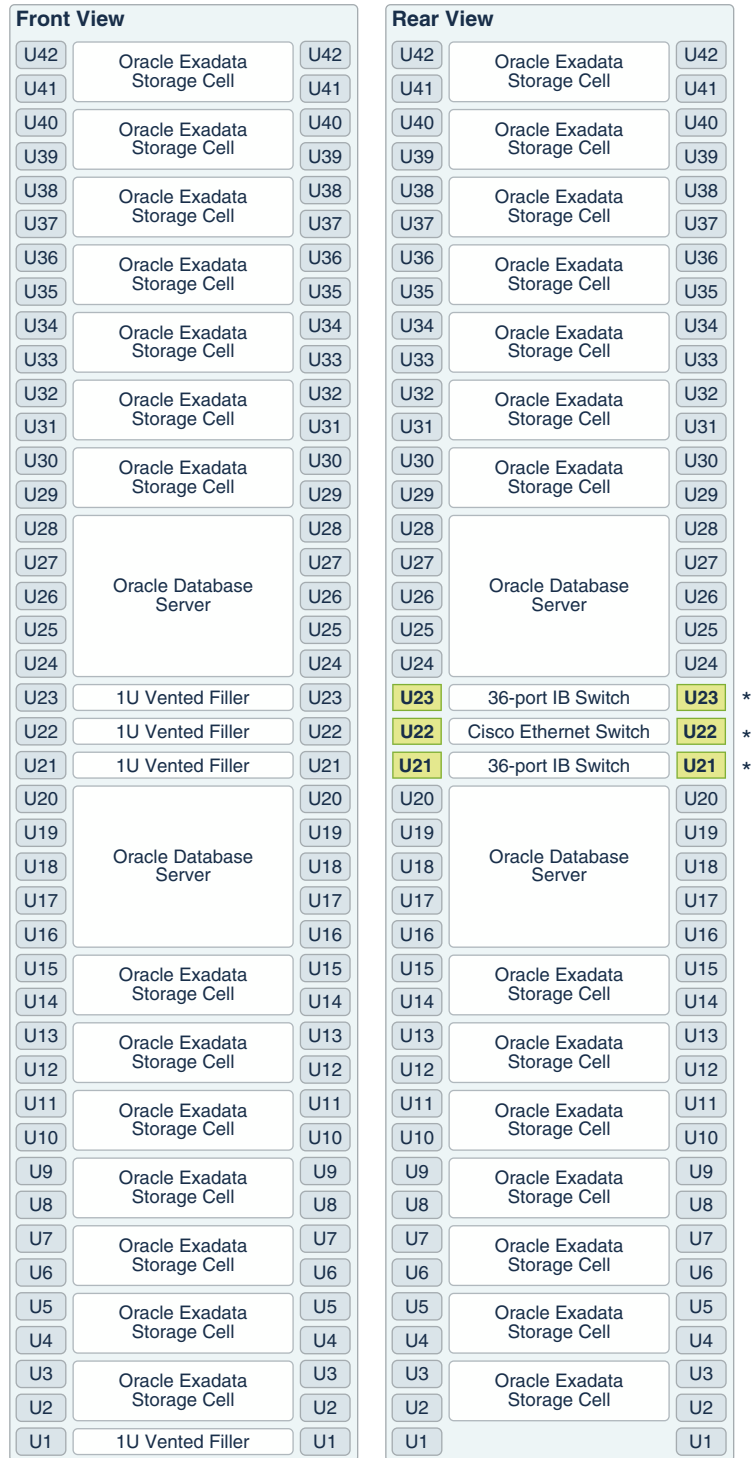
Figure 16-2 Rack Layout of Oracle Exadata Database Machine X8-8 and X7-8
