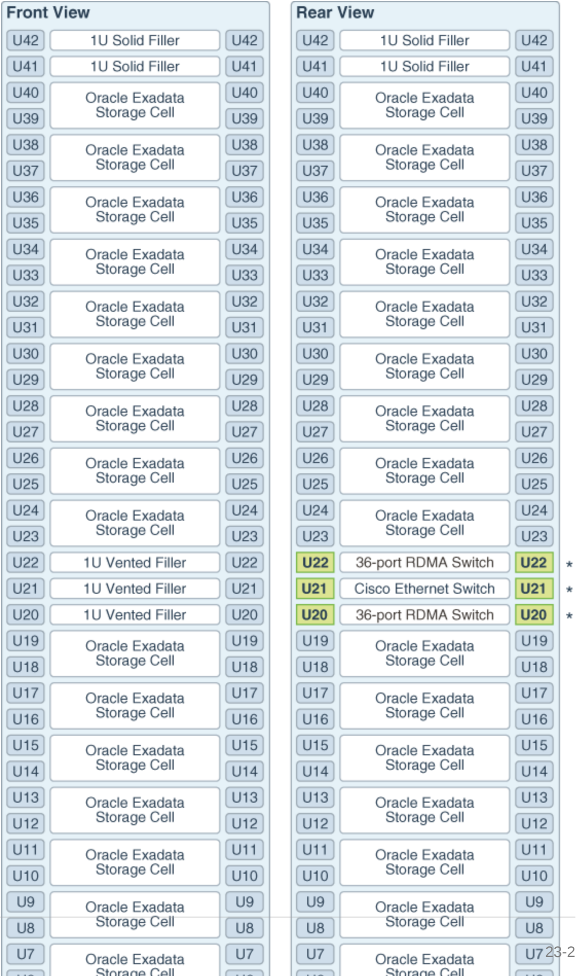
Figure 23-1 Rack Layout of Oracle Exadata Storage Expansion Full Rack X5 to X8M
