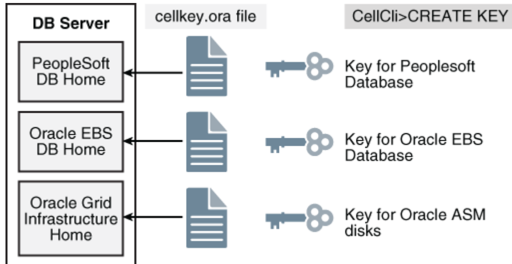
Figure 4-2 Security Keys and cellkey.ora Files
