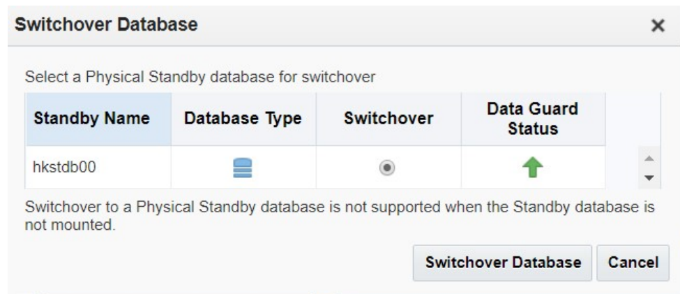
Figure 28-8 Switchover Database
