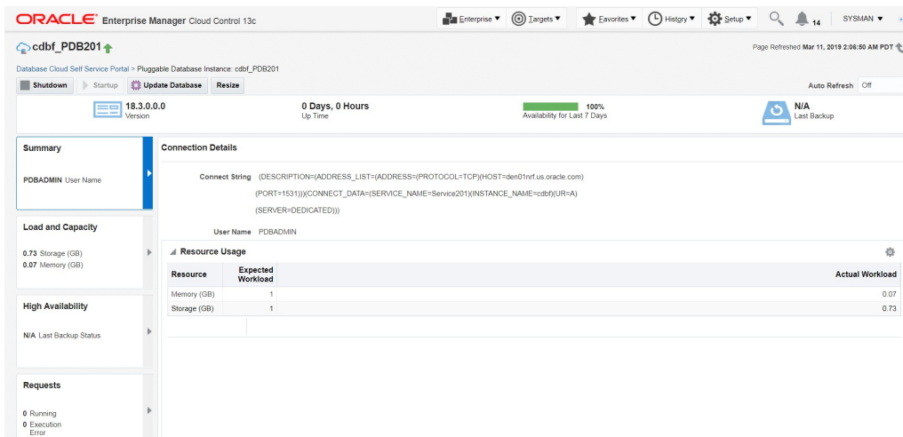
Figure 39-1 PDB Resize
