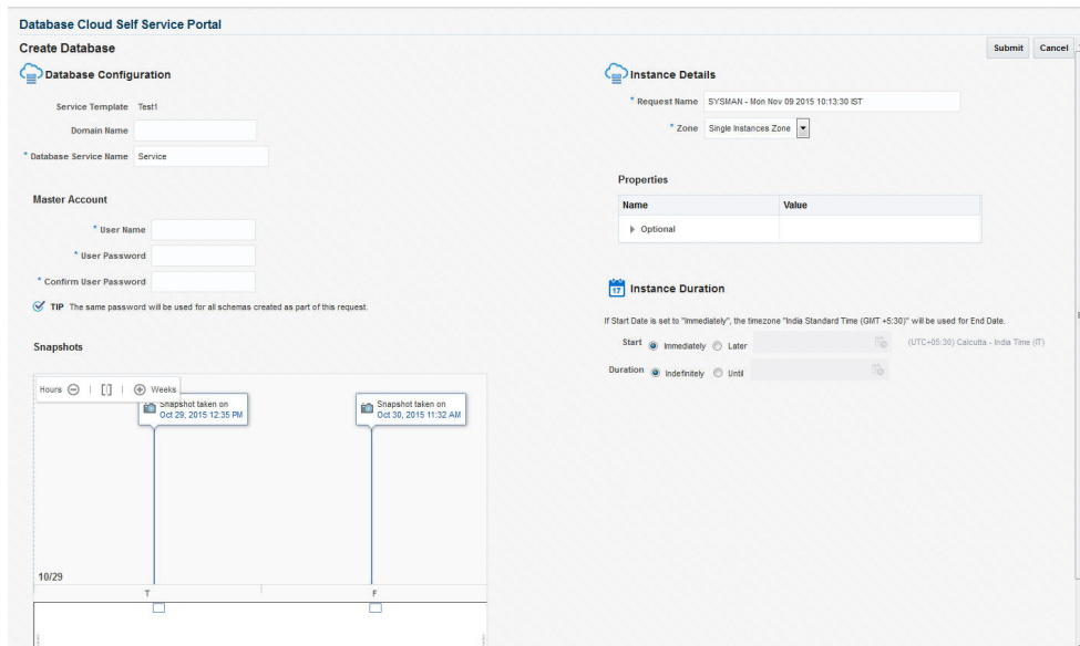
Figure 28-2 Create Database
