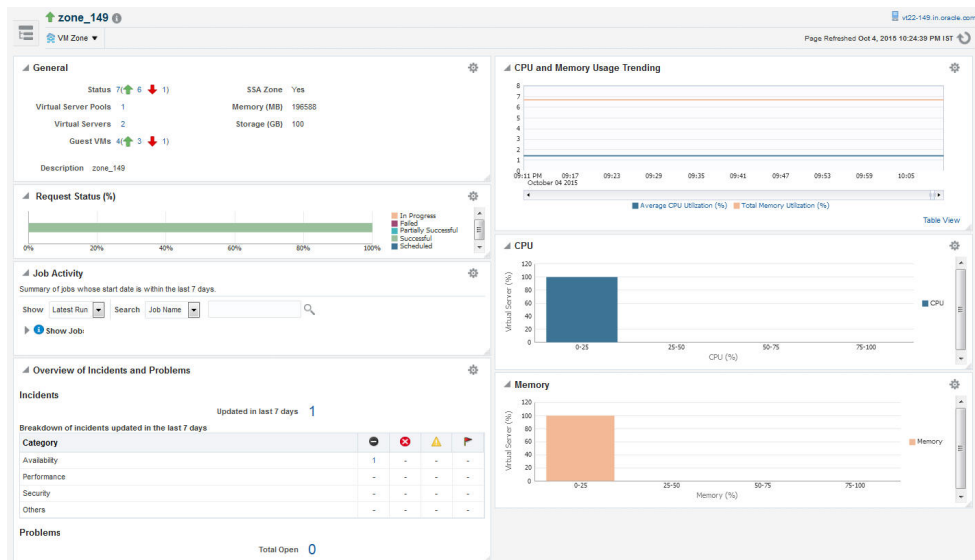
Figure 10-3 Zone Home
