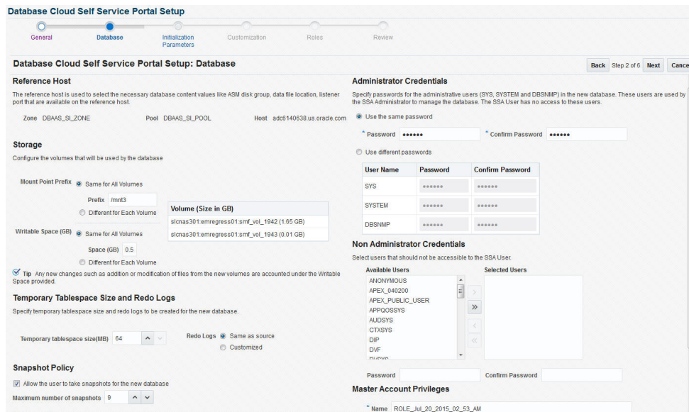
Figure 24-2 Create Service Template: Database (Snap Clone)
