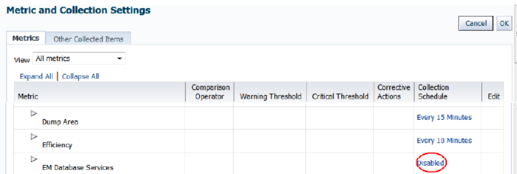
Figure 39-5 Enabling Metric Collection for Database Services
