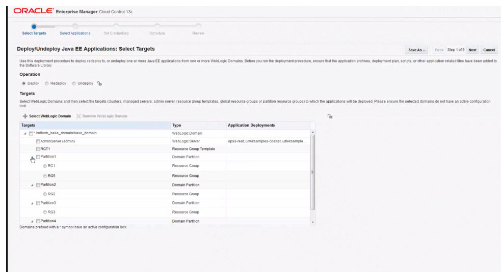
Figure 11-1 Deploy / Undeploy Java EE Applications: Select Target
