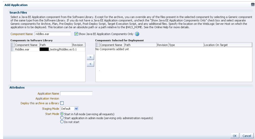
Figure 11-2 Deploy / Undeploy Java EE Applications: Add Applications
