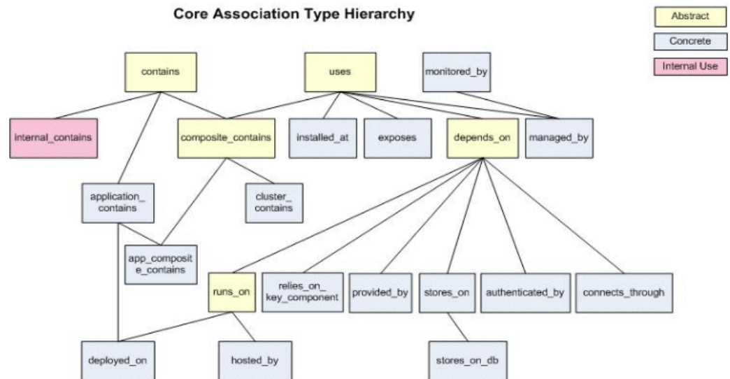
Figure 5-1 Core Association Type Hierarchy
