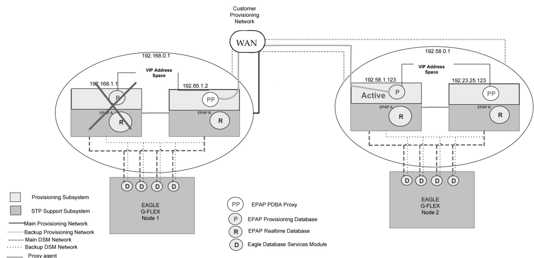
Figure 2-5 Failure of Active PDBA
