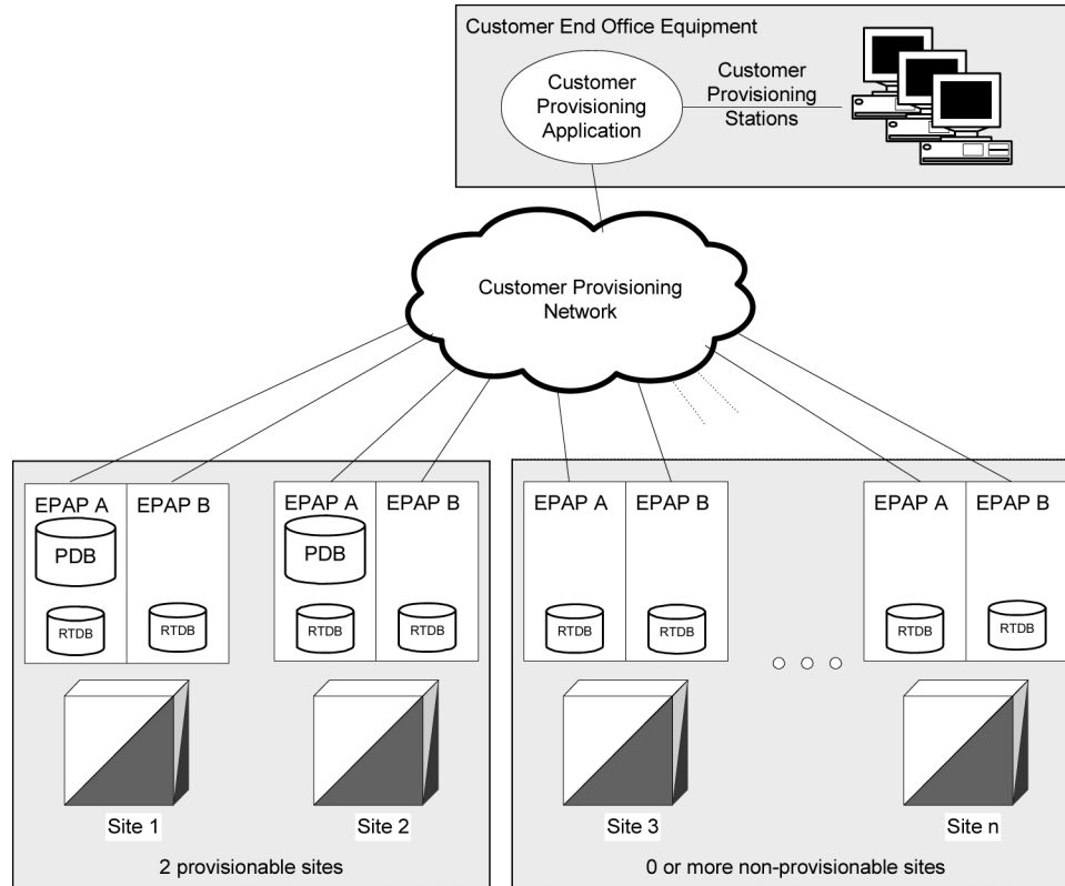
Figure 2-4 Support for Provisioning Multiple EPAPs
