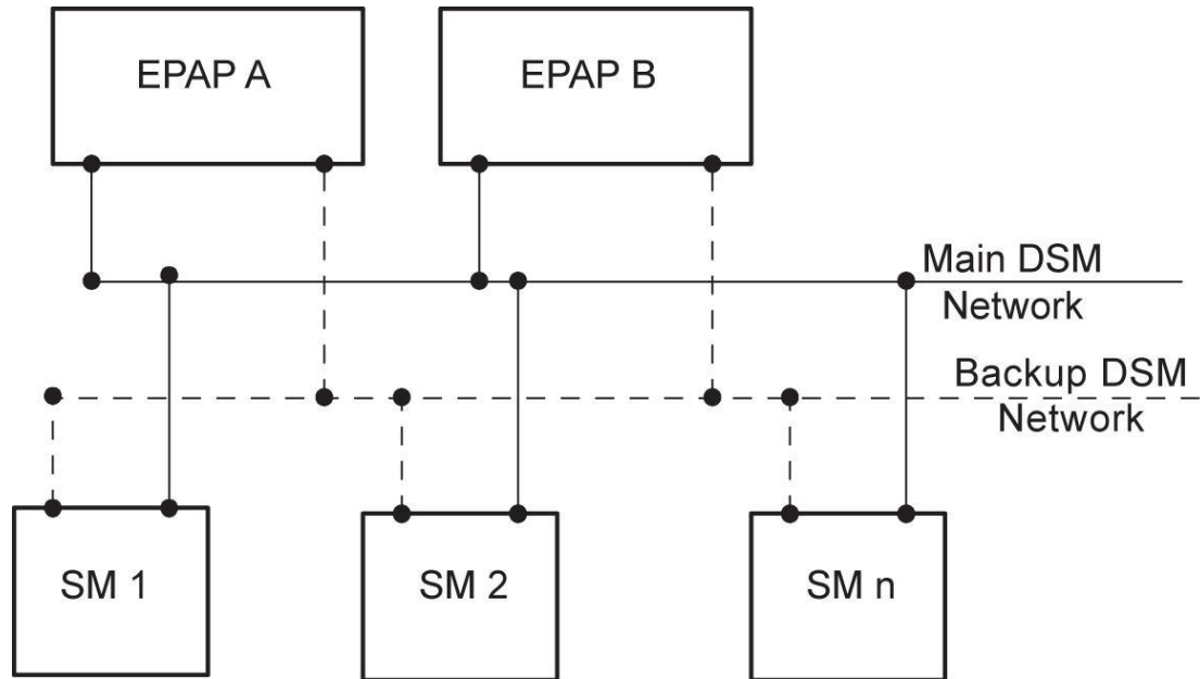
Figure 2-6 DSM Provisioning Network Architecture
