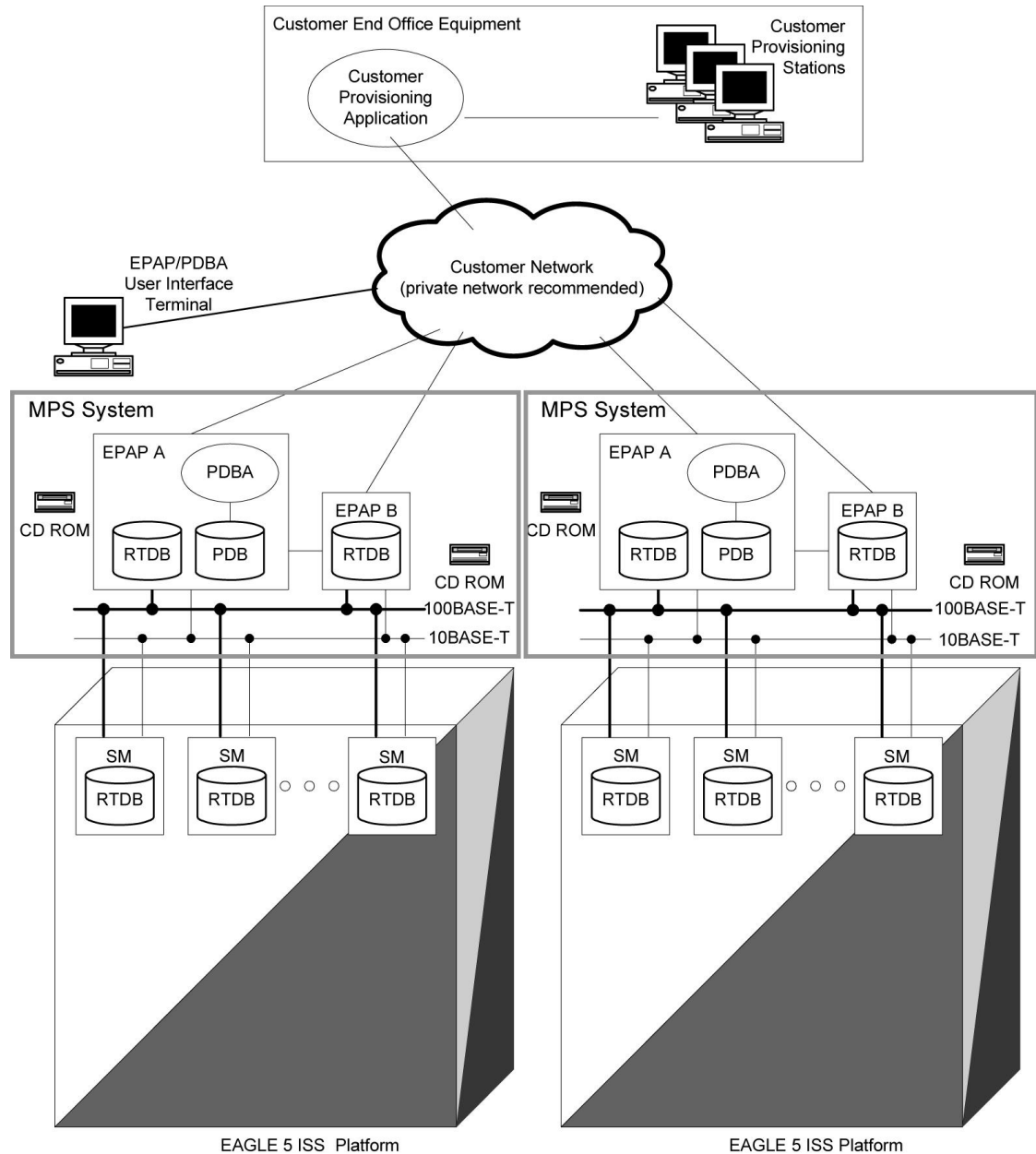
Figure 2-1 Mated EAGLE Platform Example
