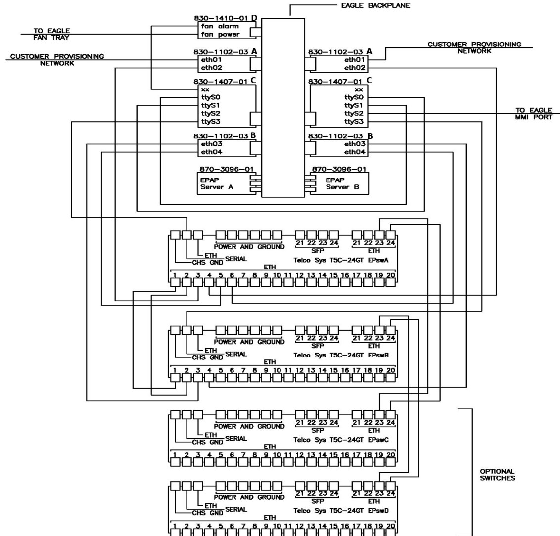
Figure A-1 EPAP Network Connections
