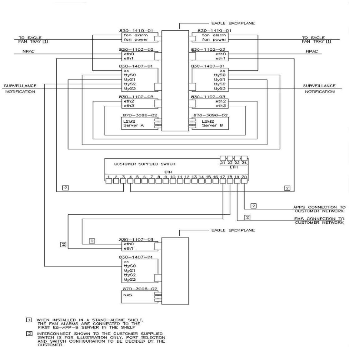
Figure A-6 LSMS and NAS Segmented Connections
