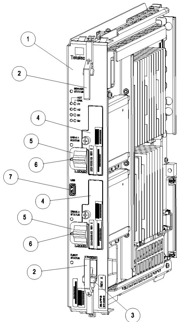
Figure 3-2 E5-APP-B Card
