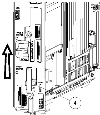
Figure 4-5 E5-APP-B Card Eject Hardware Switch, UNLOCKED
