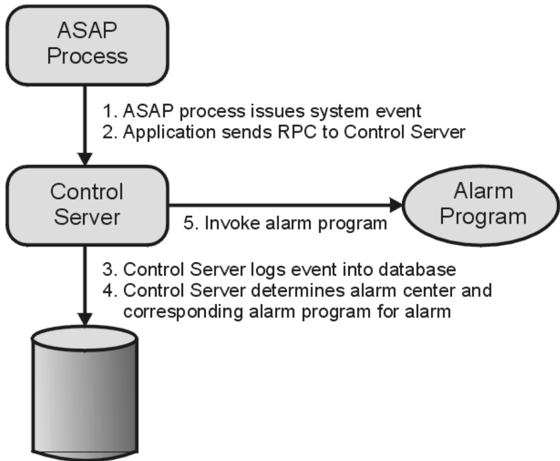
Figure 3-1 Alarm Process
