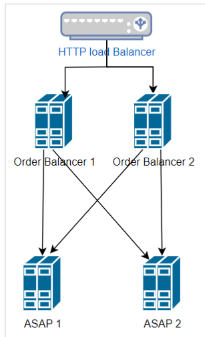
Figure 3-1 High Availability with HTTP Load Balancer
