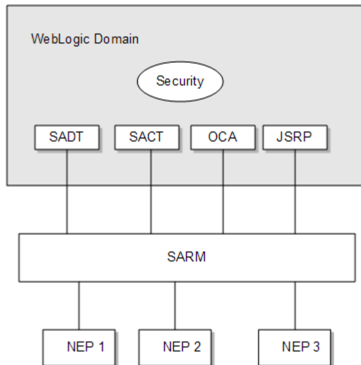
Figure 2-1 WebLogic Domain Within ASAP
