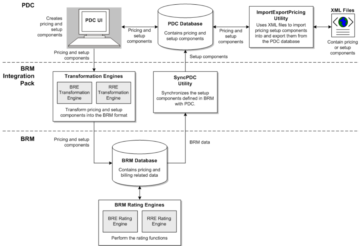
Figure 8-10 PDC and BRM Integration Architecture
