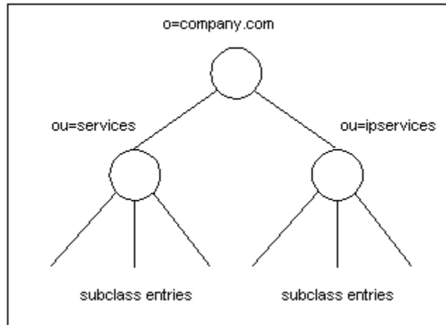
Figure 3-3 Directory Tree
