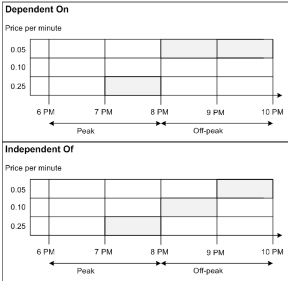
Figure 16-3 Quantity-Based Pricing Split by Time Periods
