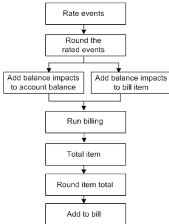
Figure 28-1 BRM Balance Impact Rounding
