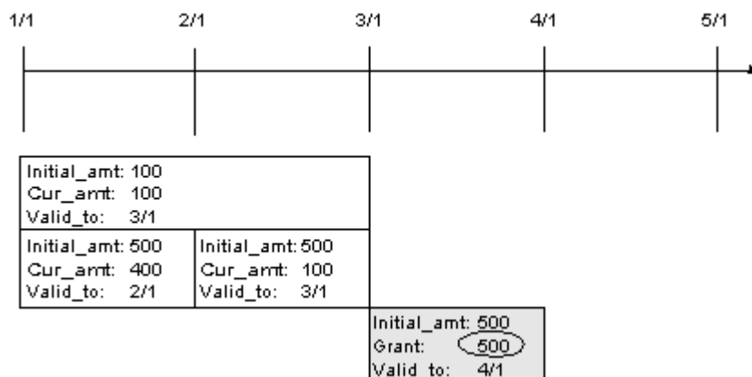
Figure 27-8 March Minutes Grant
