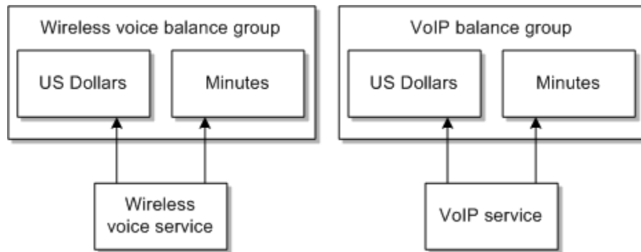
Figure 22-2 Two Balance Groups for Two Services
