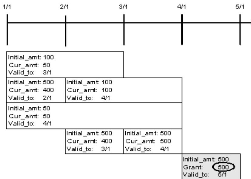
Figure 27-13 April Minutes Grant
