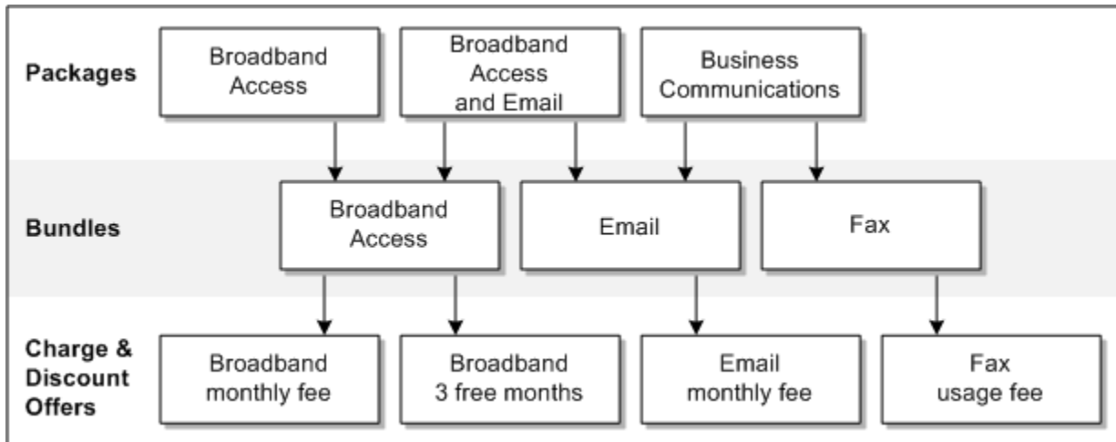
Figure 13-1 Bundles Are Always Associated with a Single Service
