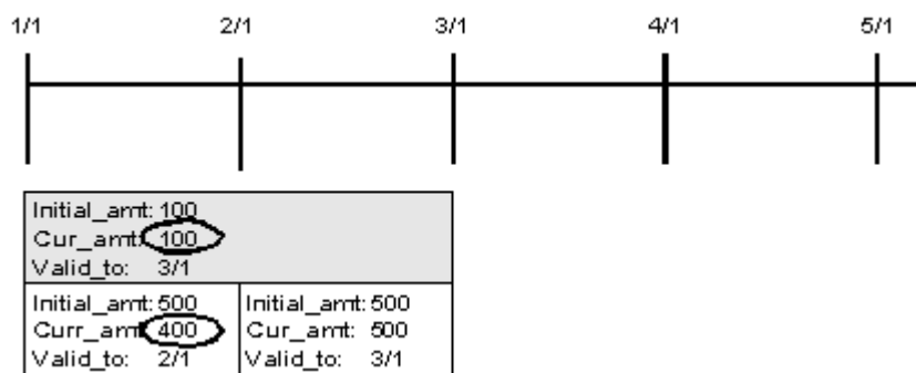
Figure 27-6 January Minutes Rollover
