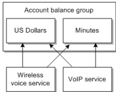
Figure 22-1 Default Balance Group for Two Services
