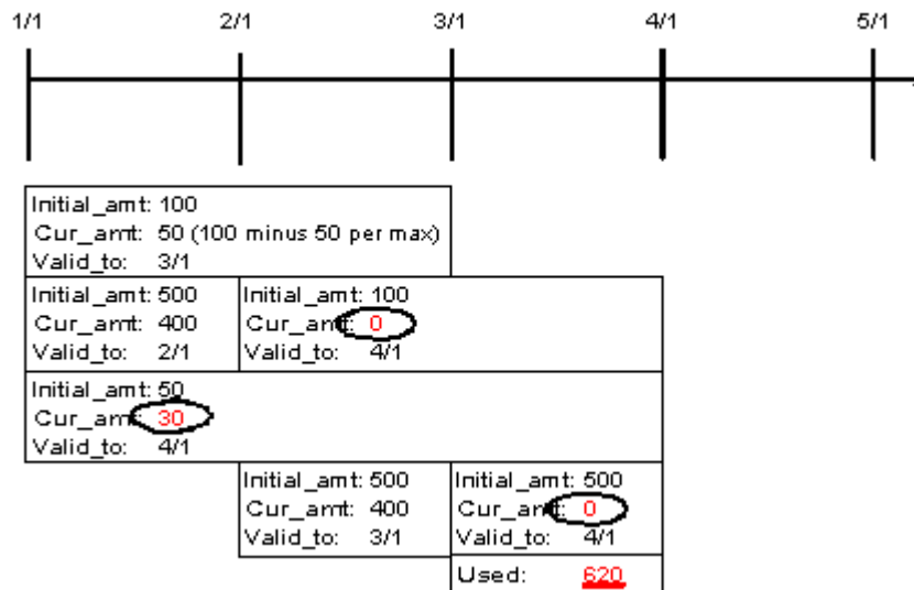
Figure 27-12 March Minutes Usage
