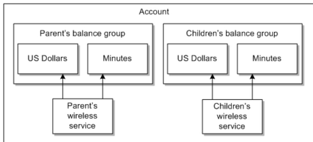
Figure 22-3 Separate Balance Groups By Purchasing Separate Packages
