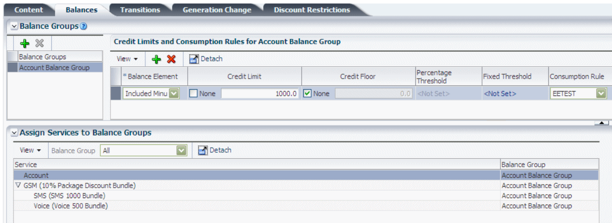
Figure 23-2 Consumption Rules for Balance Groups
