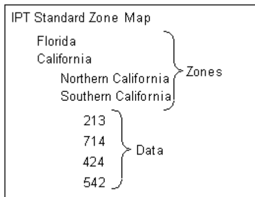
Figure 33-2 Zone Map with Nested Zones
