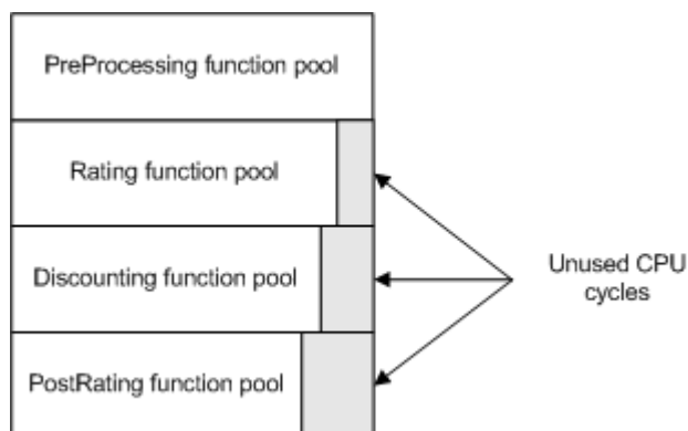
Figure 72-2 Unused CPU Cycles Example 2
