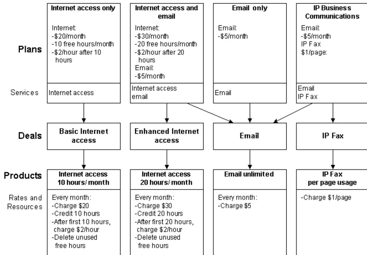
Figure 11-11 Sample Price List
