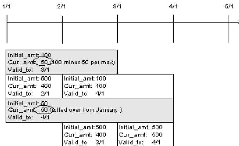
Figure 15-7 Remaining January Free Minutes Rollover
