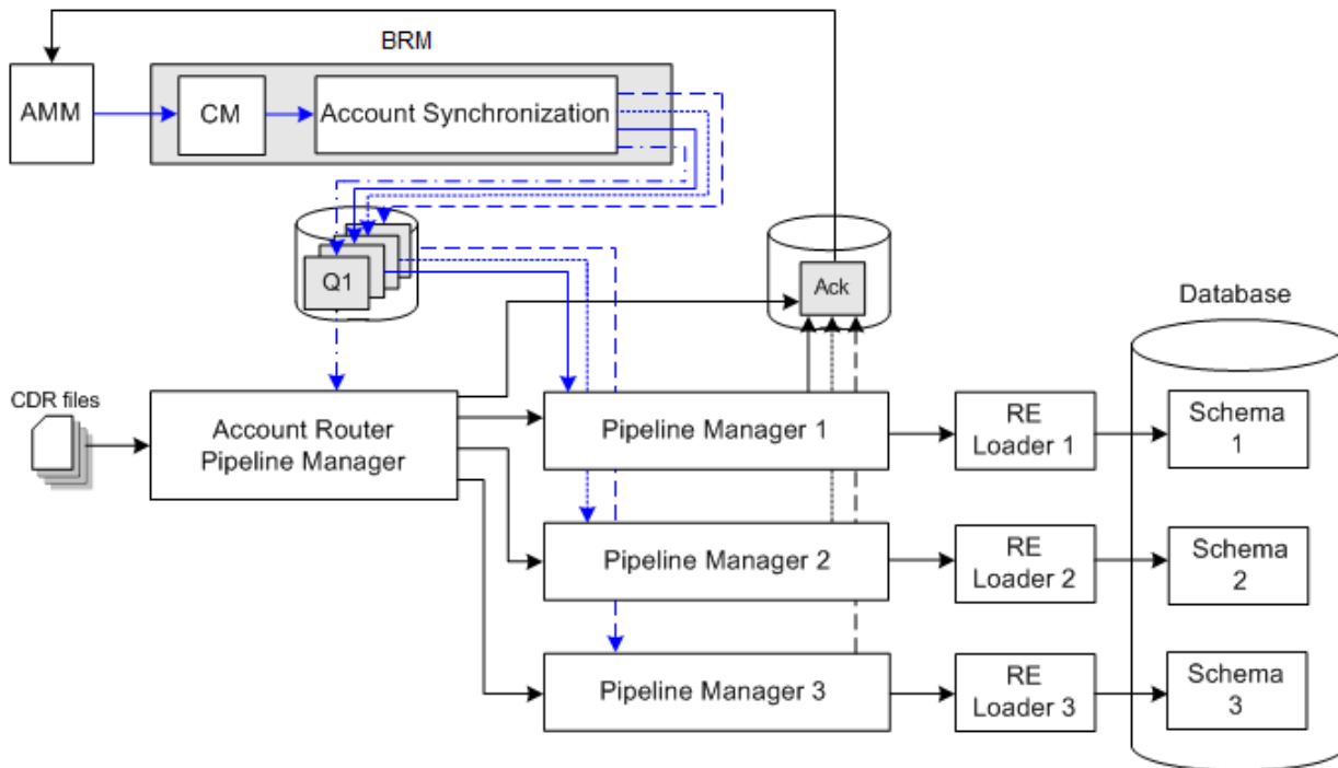
Figure 73-1 AMM Pipeline EDR Management
