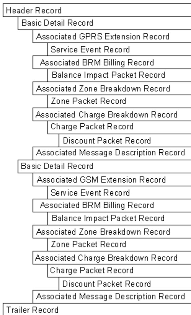
Figure 17-3 BRM EDR Container Organization
