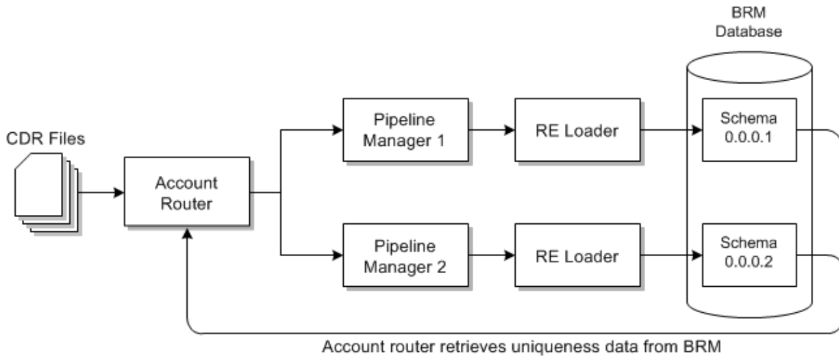
Figure 69-1 FCT_AccountRouter CDR Management
