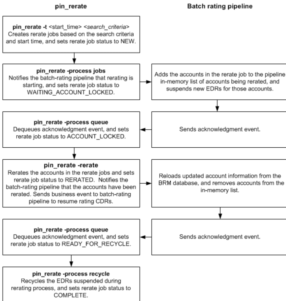
Figure 64-2 Concurrent Rerating Process Flow
