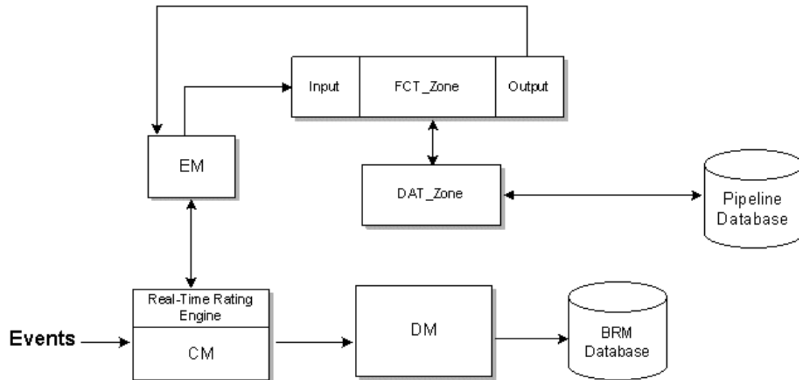
Figure 33-3 Data Flow for Real-Time Pipeline Zoning
