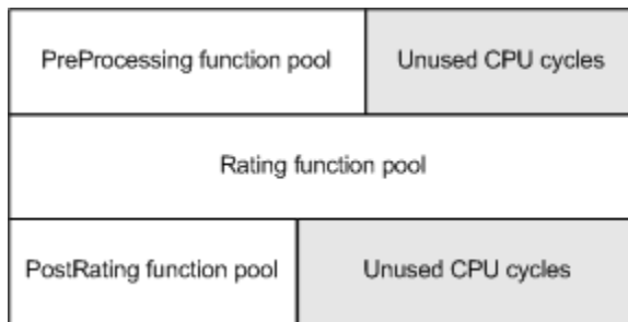
Figure 72-1 Unused CPU Cycles Example 1
