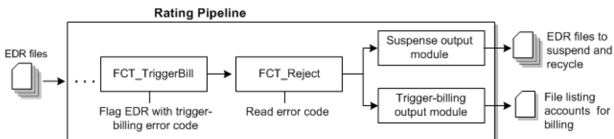
Figure 40-4 EDR Path for Triggered Billing
