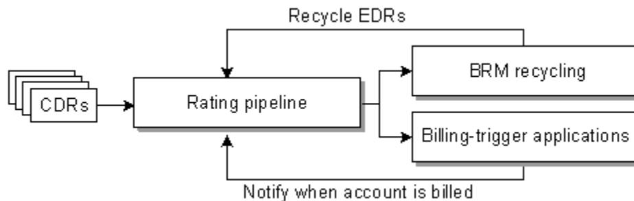
Figure 40-3 Pipeline Manager, Recycling and Billing Applications Relationship
