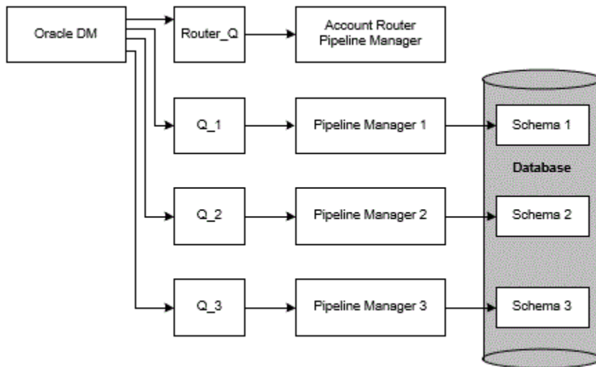
Figure 73-5 Sample Synchronization Architecture
