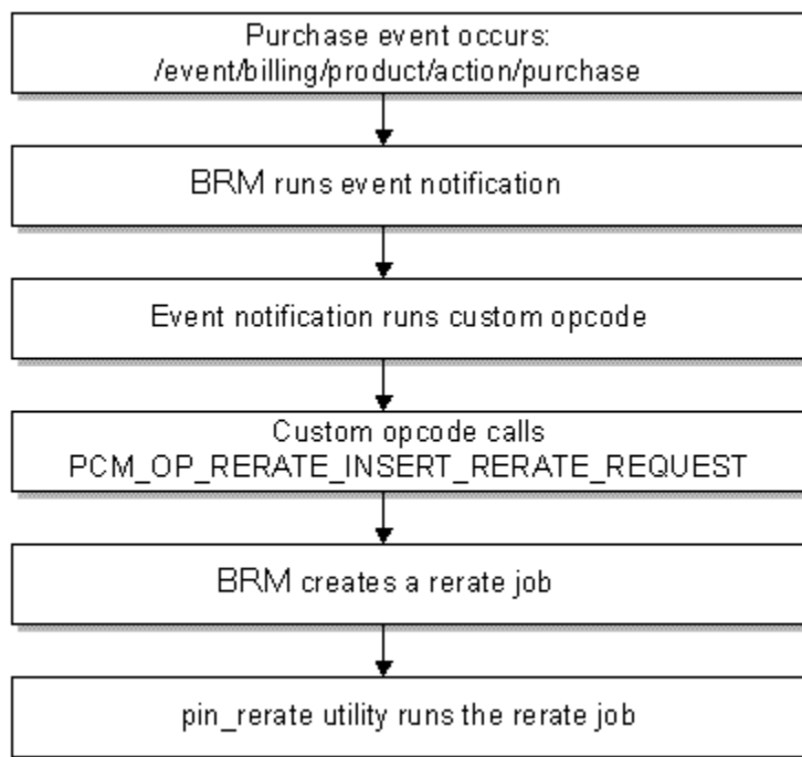
Figure 65-2 Trigger-Dependent Rerating Process
