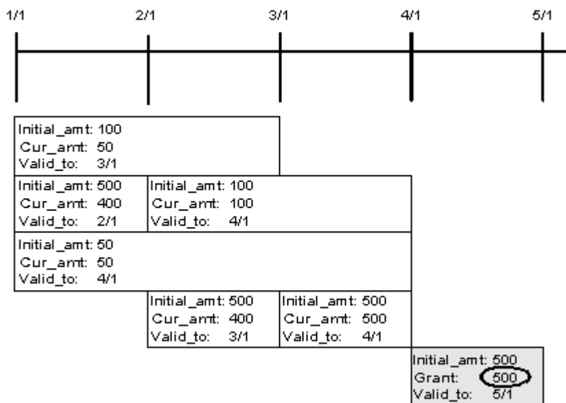
Figure 15-10 April Free Minutes Grant
