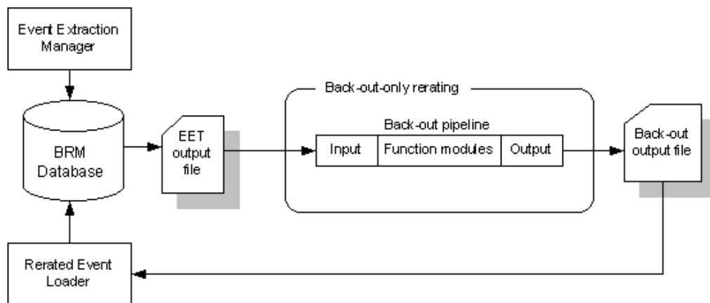
Figure 61-3 Back-Out-Only Rerating Process
