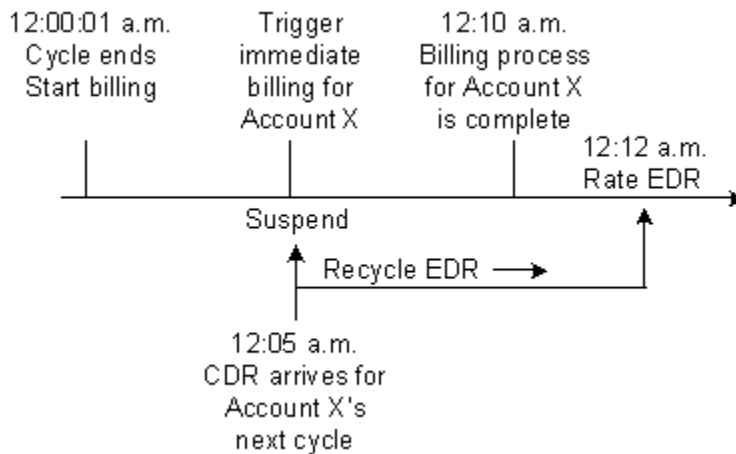
Figure 40-2 Pipeline-Triggered Billing
