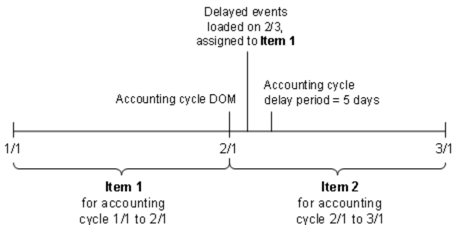
Figure 17-6 Delayed Events Arriving During Cycle Delay Period
