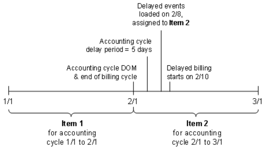
Figure 17-7 Delayed Events Arriving After Cycle Delay Period
