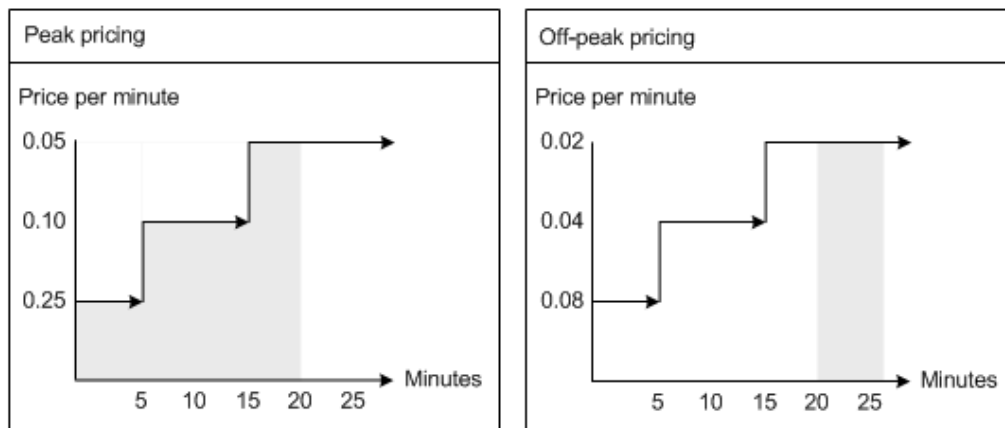
Figure 1-2 Consecutive Splitting
