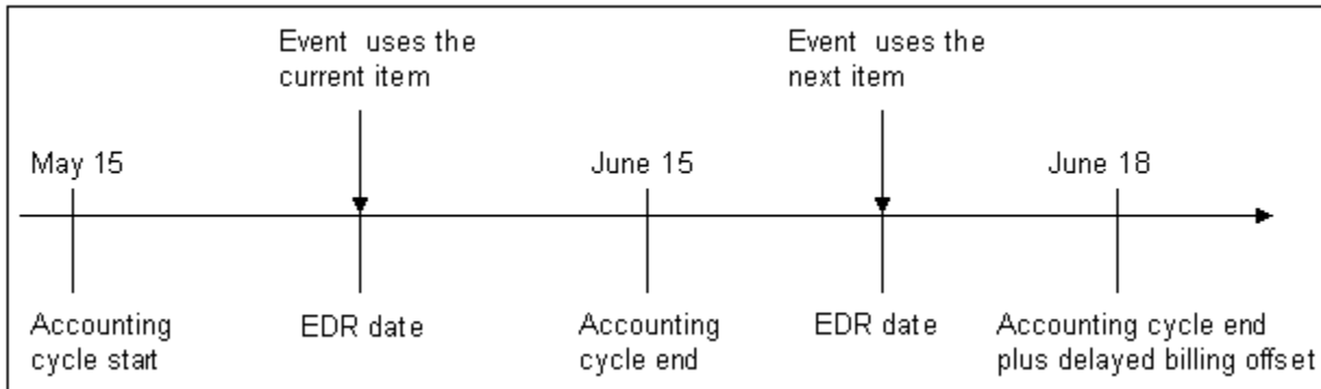
Figure 17-4 Event Assignment
