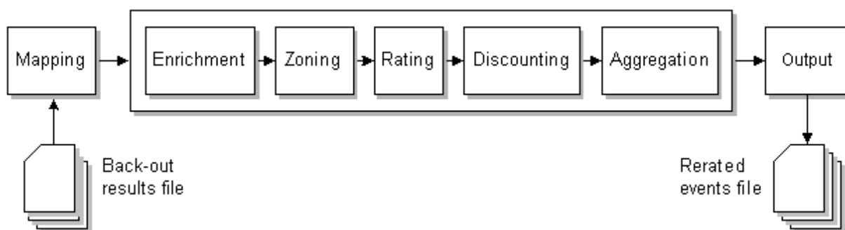
Figure 63-2 Rerating Pipeline
