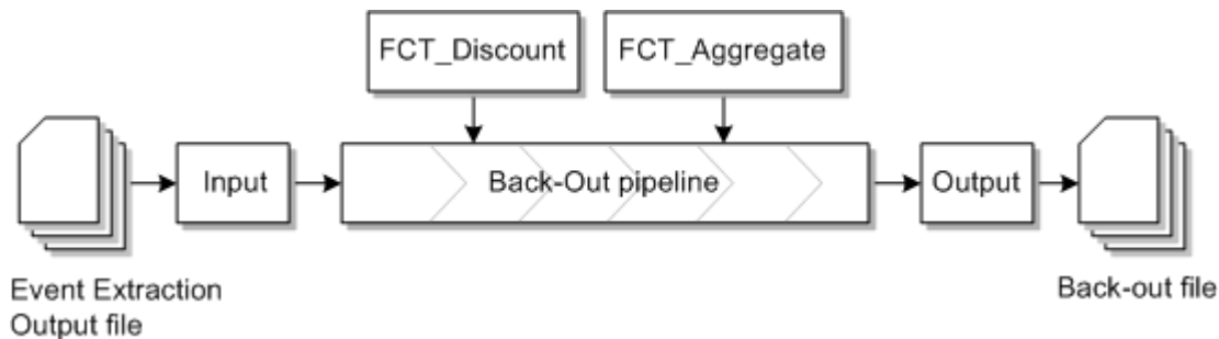
Figure 63-1 Back-Out Pipeline
