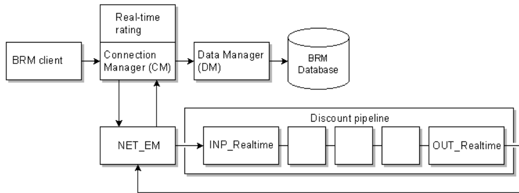
Figure 68-2 Real-Time Discounting
