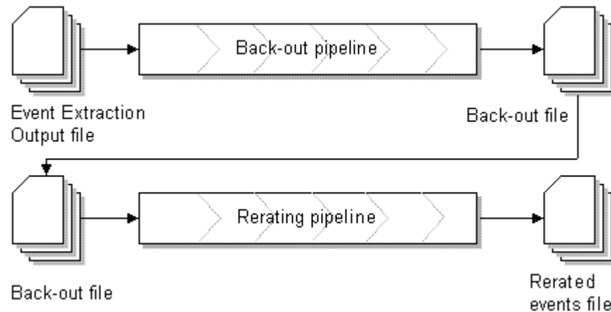
Figure 61-2 Pipeline Manager Rerating Process
