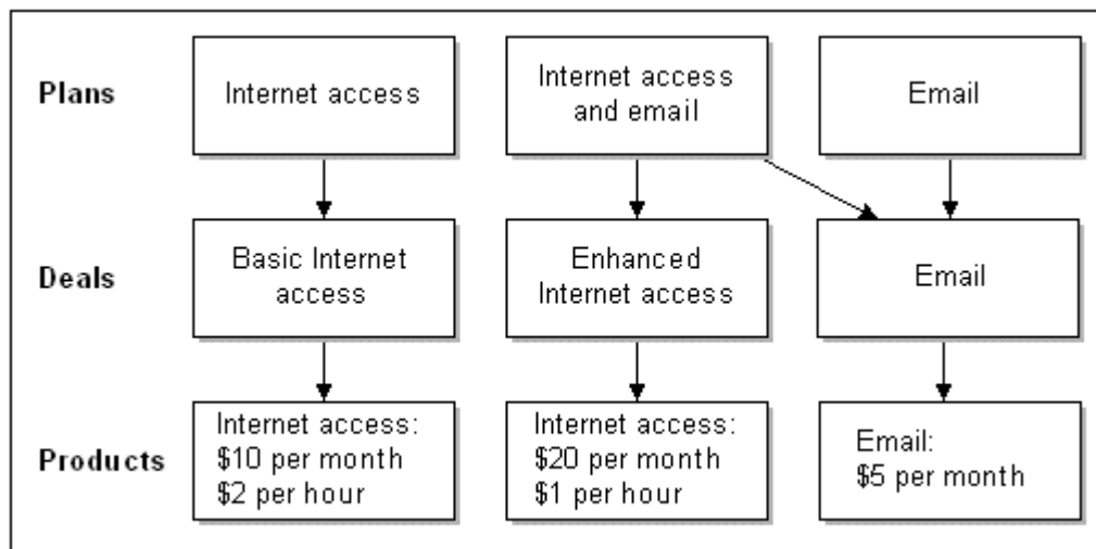
Figure 11-1 Simple Price List
