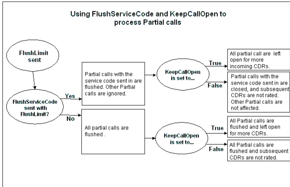
Figure 5-1 FlushServiceCode and KeepCallOpen Semaphore Interaction
