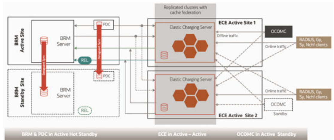
Figure 84-4 Site Deployment with Recommended Options
