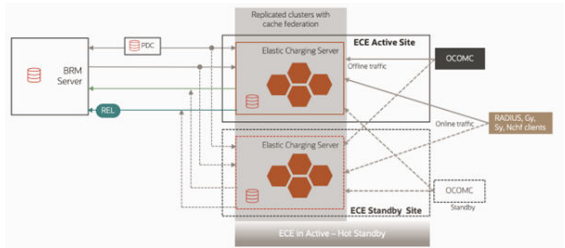
Figure 84-3 Active-Hot Standby Deployment Mode for ECE
