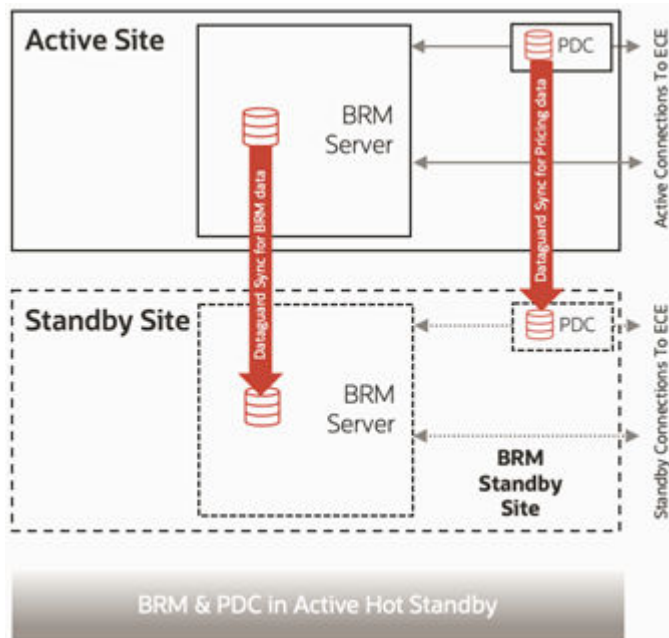
Figure 84-1 Deployment Modes for BRM and PDC
