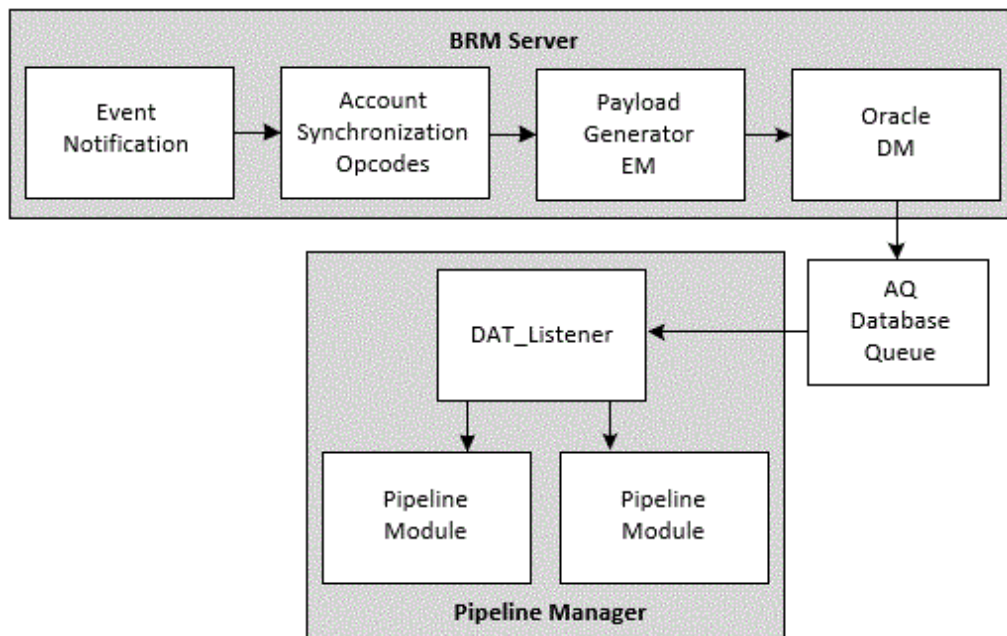
Figure 46-1 Data Flow from BRM to Pipeline Manager
