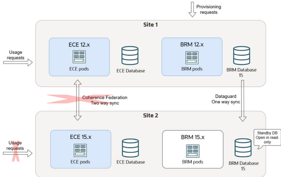
Figure 18-7 Failing Over Site 1 to Site 2
