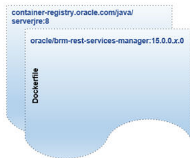
Figure 15-1 Image Stack for BRM REST Services Manager
