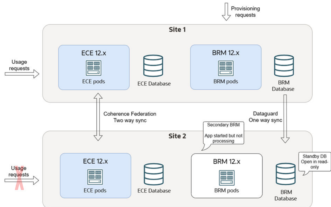
Figure 18-2 Usage Requests for Switching Off Site 2
