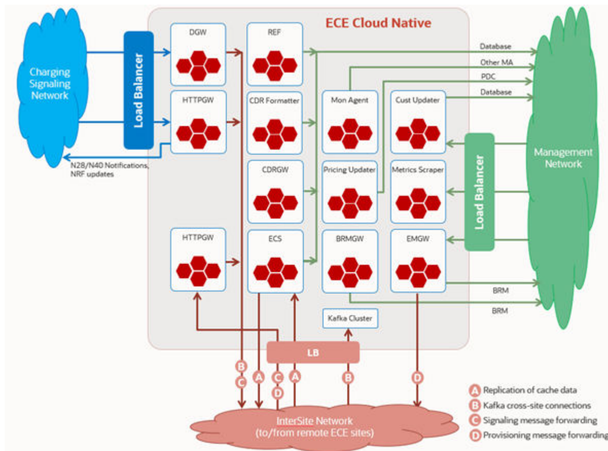
Figure 4-2 ECE Cloud Native Ingress and Egress Flows
