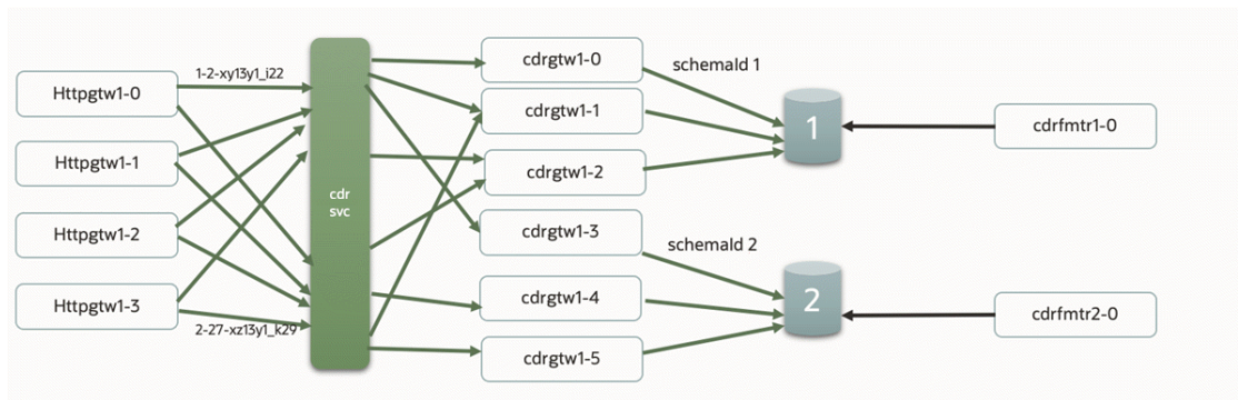
Figure 10-1 Scaled Architecture with an Oracle Database
