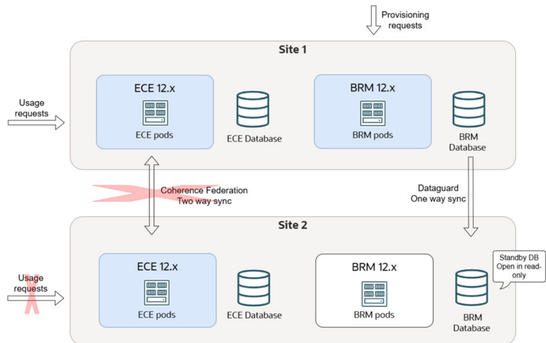
Figure 18-4 Stopped Federation from ECE Site 2 to Site 1
