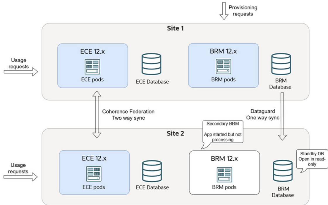
Figure 18-1 Initial State of BRM Cloud Native Active-Active Disaster Recovery System
