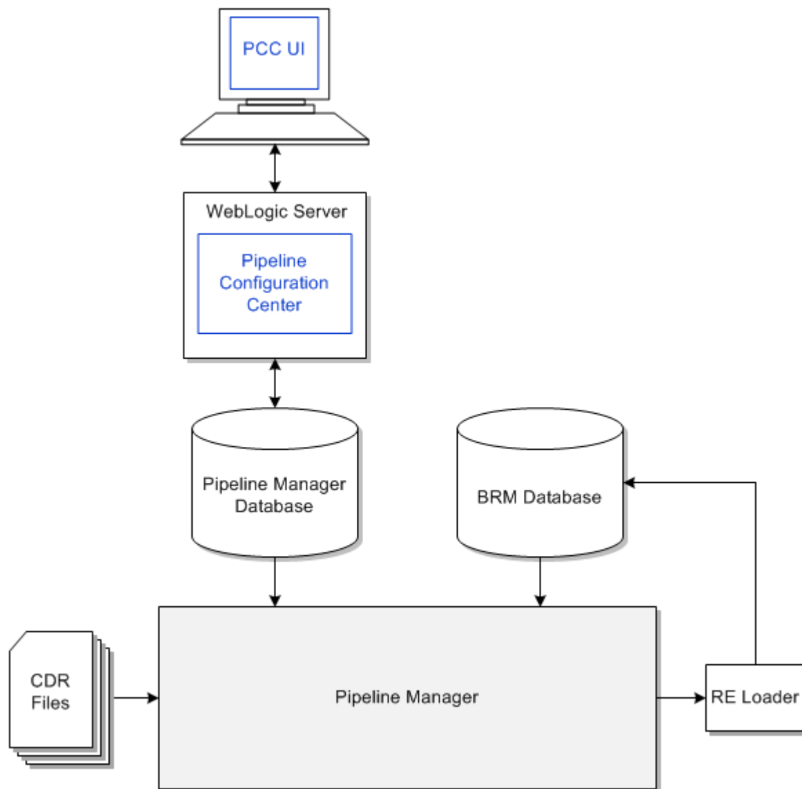
Figure 10-1 PCC and Pipeline Manager Integrated Architecture
