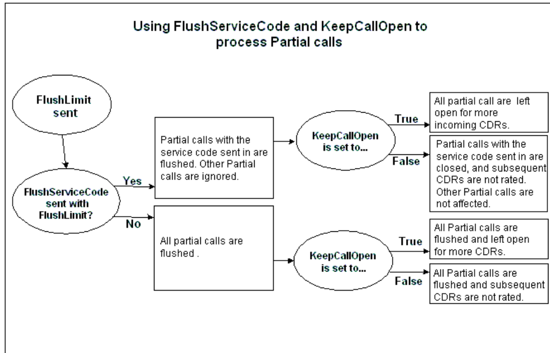
Figure 5-1 FlushServiceCode and KeepCallOpen Semaphore Interaction
