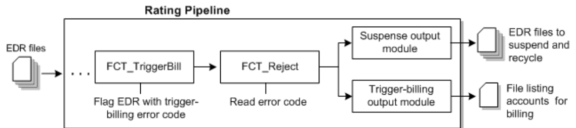
Figure 14-4 EDR Path for Triggered Billing
