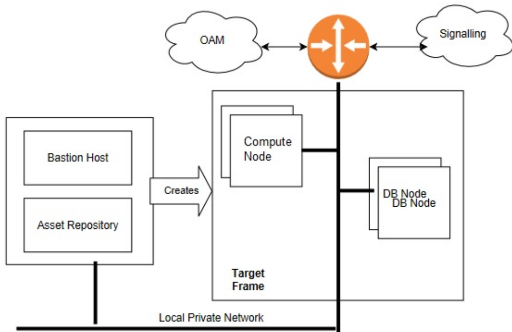
Figure 3-5 OCCNE Installation Overview
