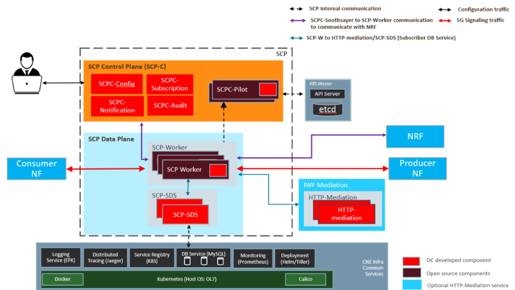
Figure 2-1 Service Communication Proxy Architecture
