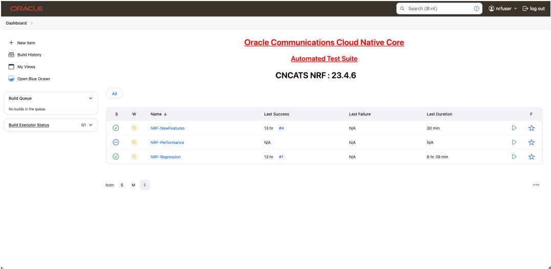
Figure 4-24 NRF Pre-Configured Pipelines
