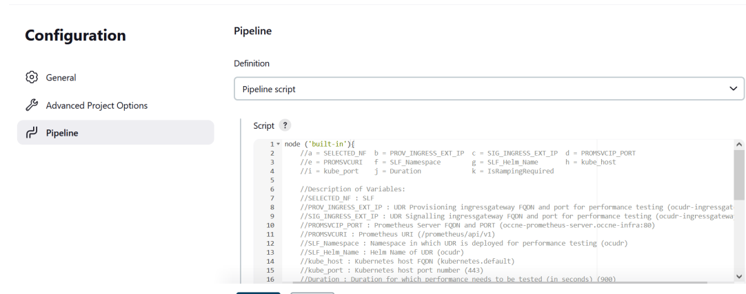
Figure 4-99 SLF-Performance Pipeline Configuration
