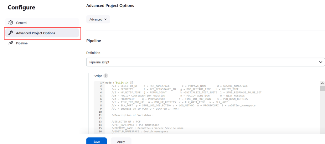
Figure 2-40 Advanced Project Options
