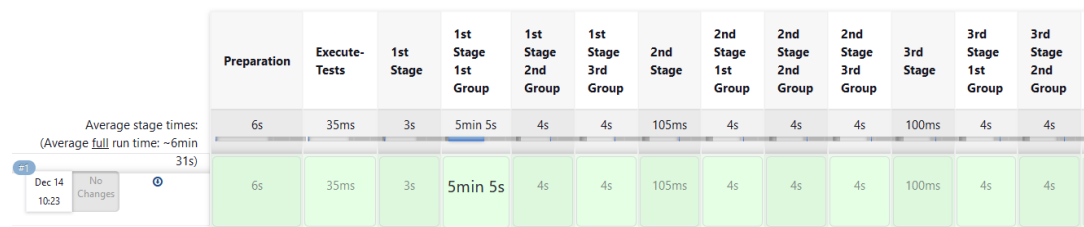
Figure 4-5 BSF New Feature Pipeline
