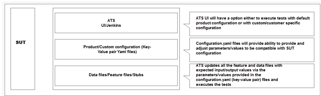
Figure 2-56 SUT Design Summary
