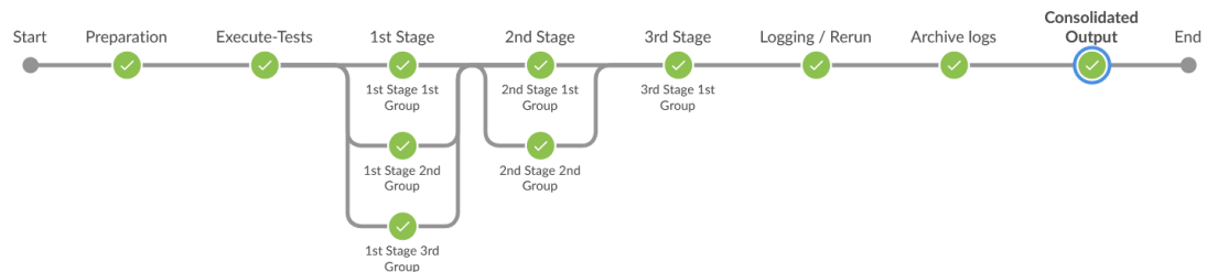
Figure 2-45 Pipeline Blue Ocean View
