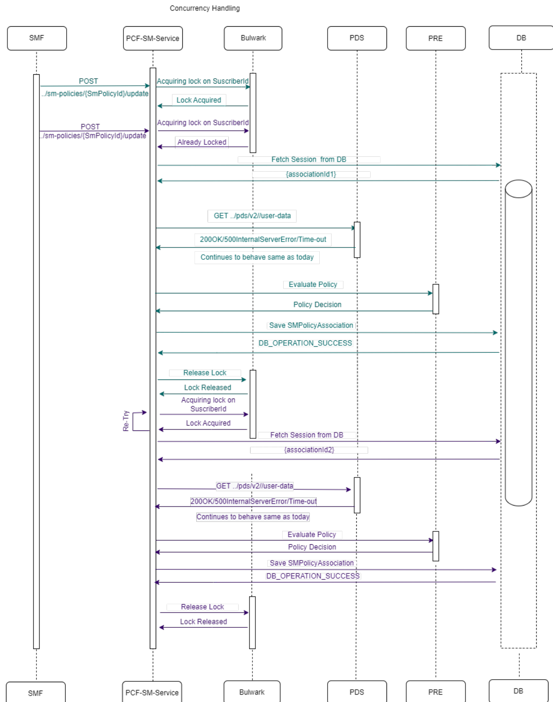
Figure 4-91 Concurrency Enabled for SM-Update and multiple updates for the same subscriber
