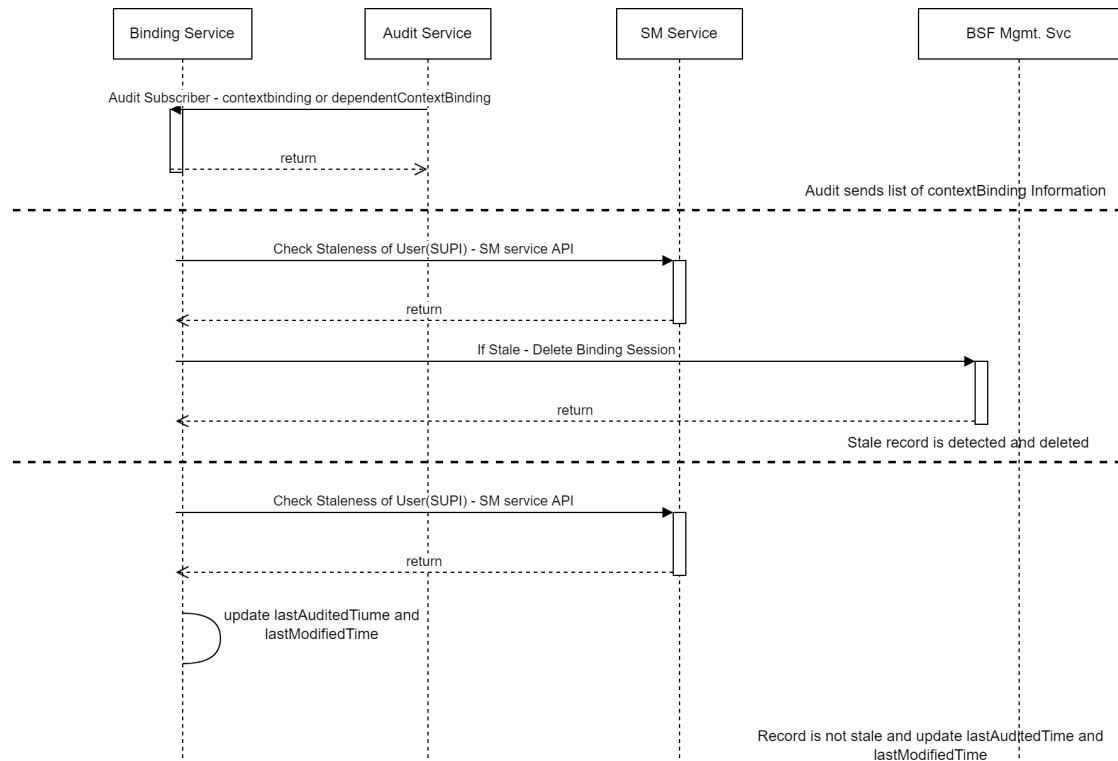
Figure 4-70 Example call flow for Stale Session Detection and Handling in Binding Service
