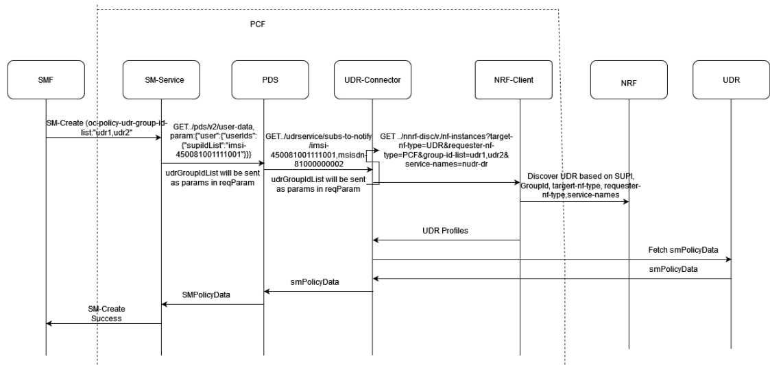
Figure 4-24 SMF sends SM Policy Association Request with oc-policy-udr-group-id
