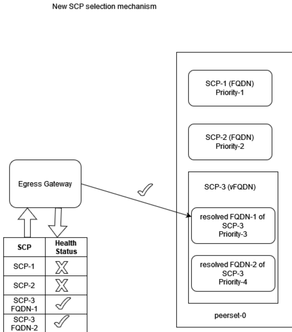
Figure 4-47 New SCP selection mechanism
