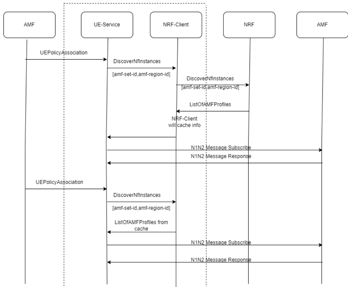
Figure 4-4 AMF Discovery/ Re-Discovery
