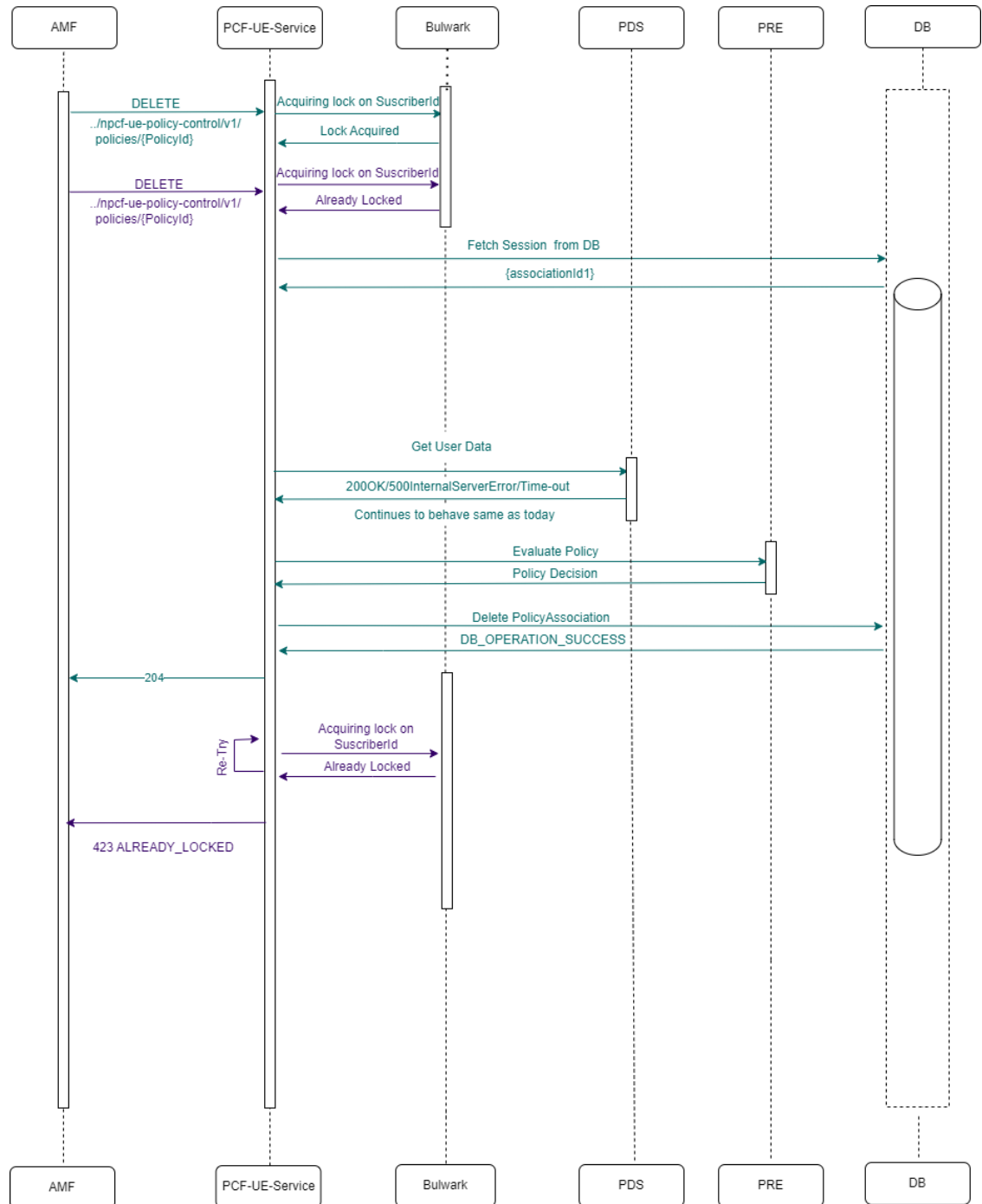
Figure 4-112 Two AM-Delete requests for same Subscriber and retry failure (retry =1)
