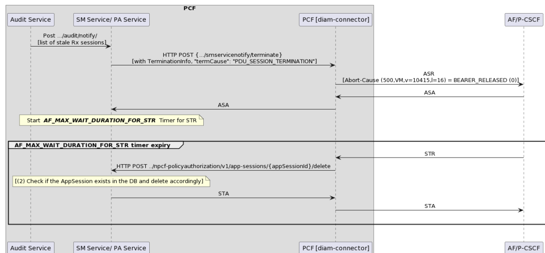
Figure 4-32 Rx session cleanup when Audit service detects a stale session
