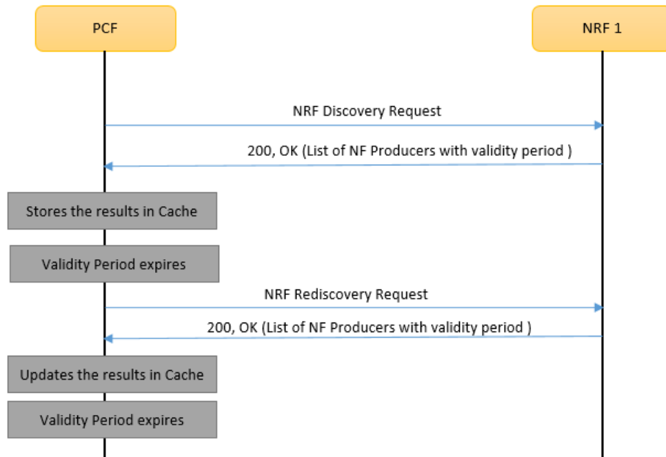
Figure 4-135 Call Flow - NRF Rediscovery
