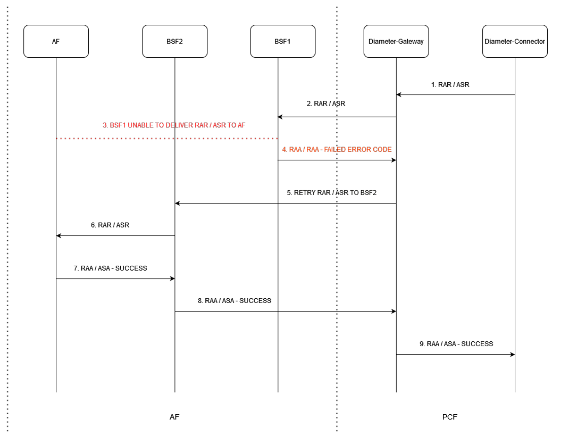
Figure 4-42 Call Flow Rx RAR or Rx ASR one time message retry - Success Case:
