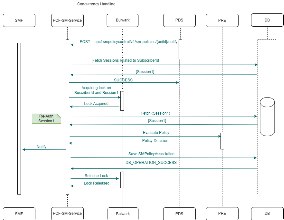
Figure 4-86 Call Flow for SM Update-Notify Request (One Notification and One Session)
