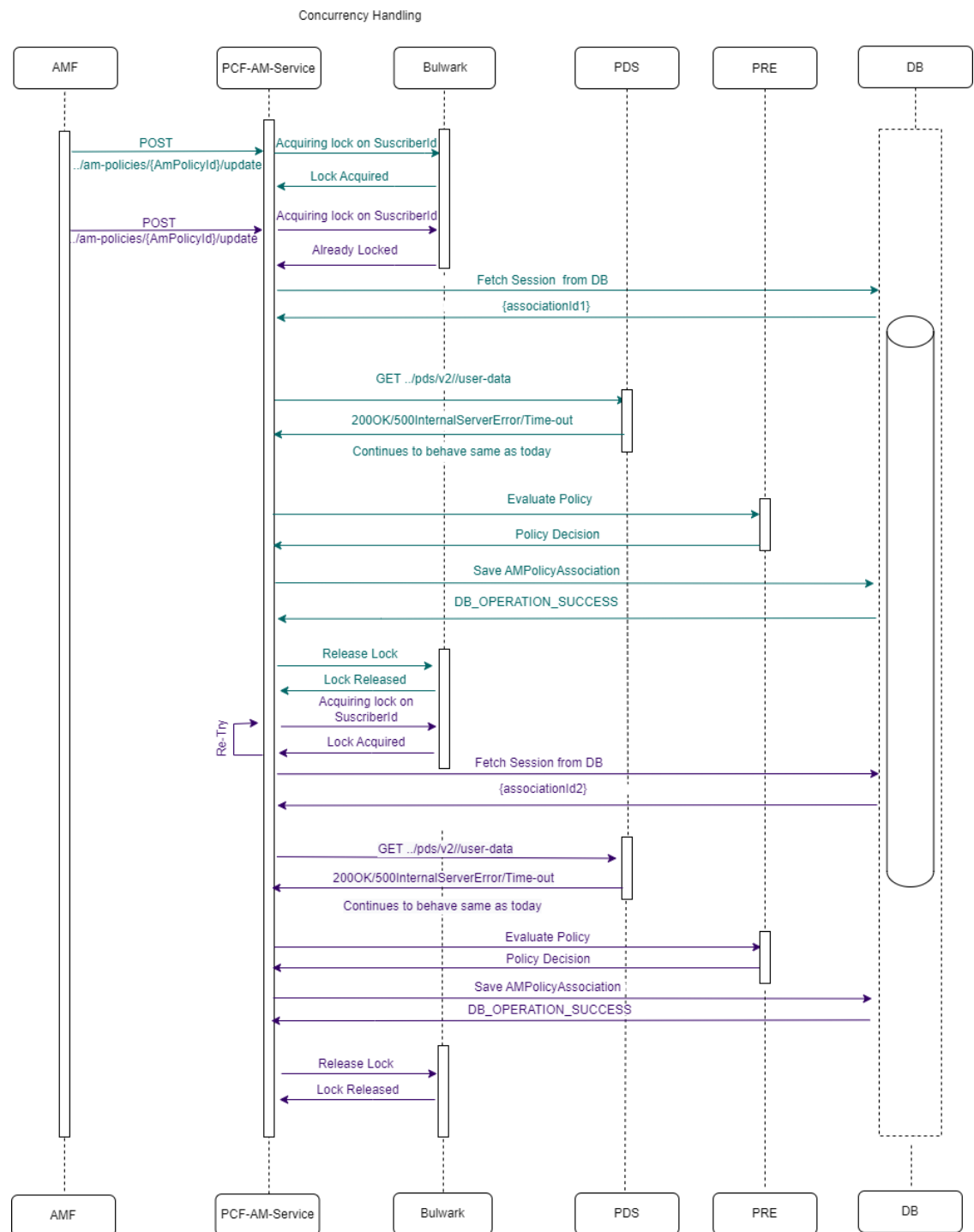
Figure 4-105 Two AM-Update requests for same Subscriber but different Sessions and retry success
