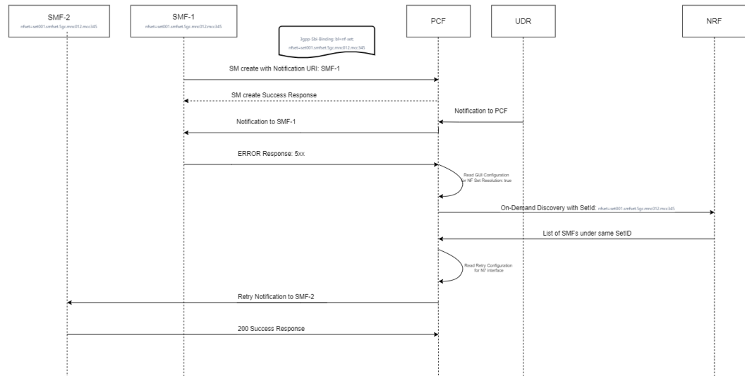
Figure 4-61 On demand NF Discovery is enabled (NF Set Resolution is set to NRF Discovery)
