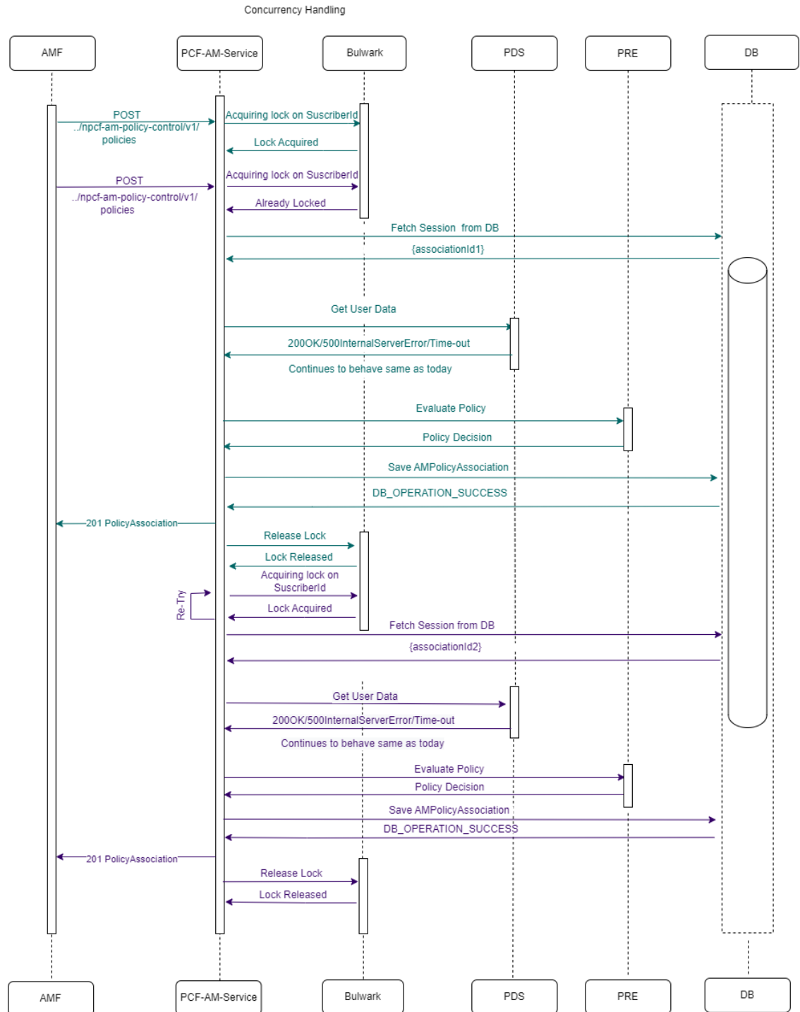
Figure 4-101 Call flow for two AM-Create requests for same subscriber and retry success
