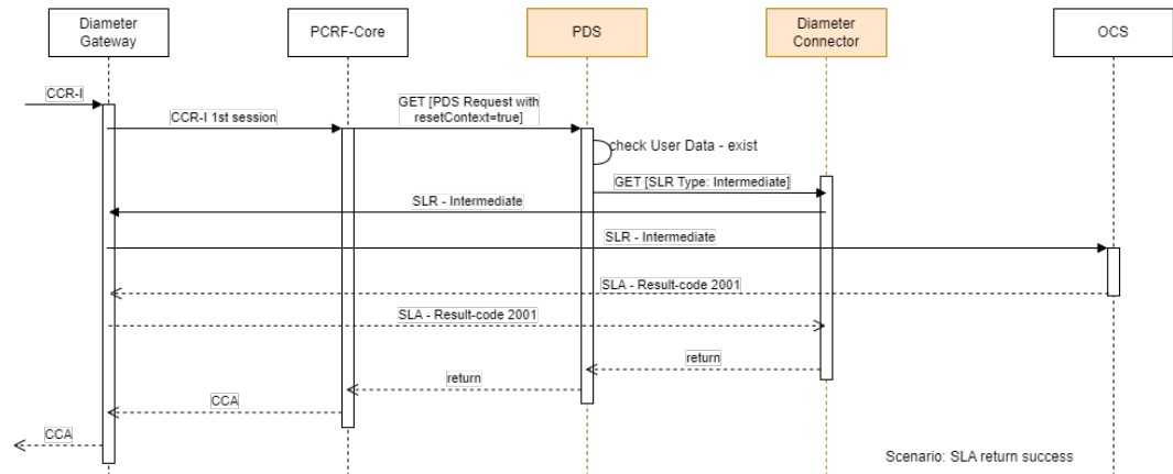
Figure 4-6 SLA Returns Success
