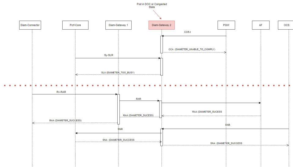
Figure 4-77 Call flow diagram for Diameter Congestion Control
