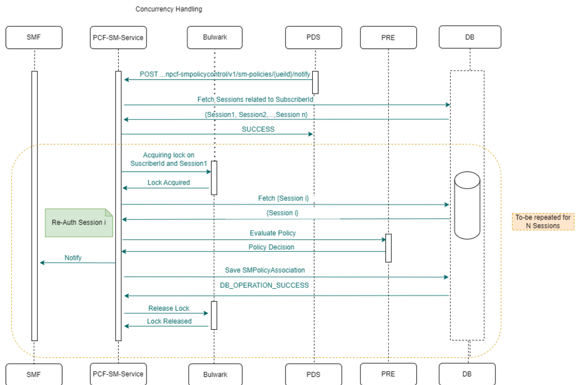
Figure 4-87 Call Flow for SM Update-Notify Request (One Notification and n Sessions)
