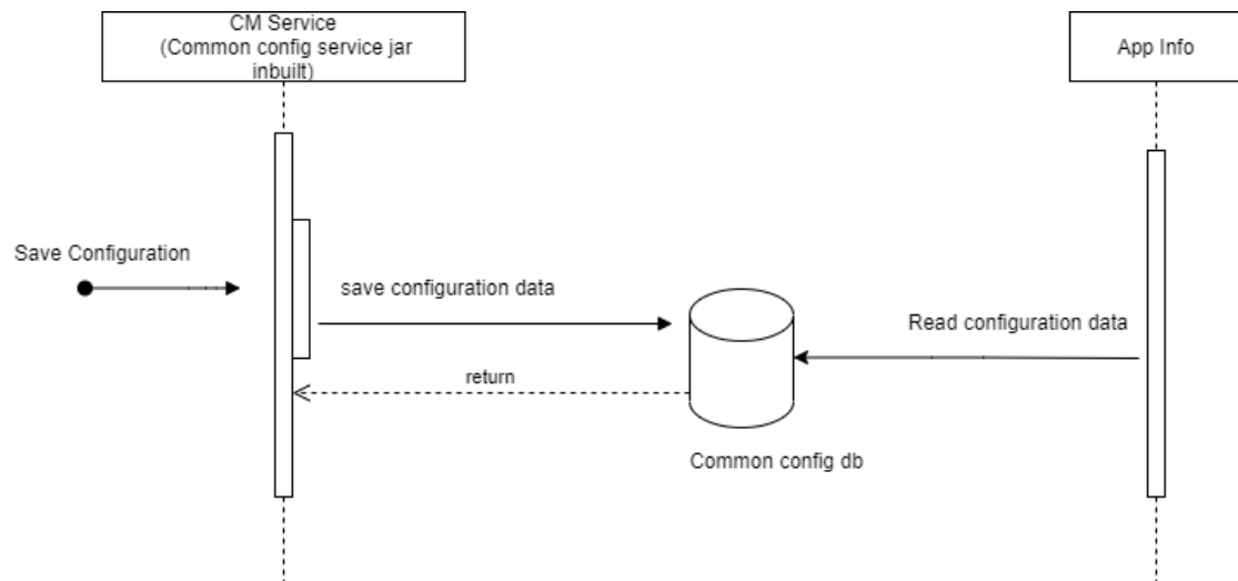
Figure 4-143 Call flow to Save Configuration Data
