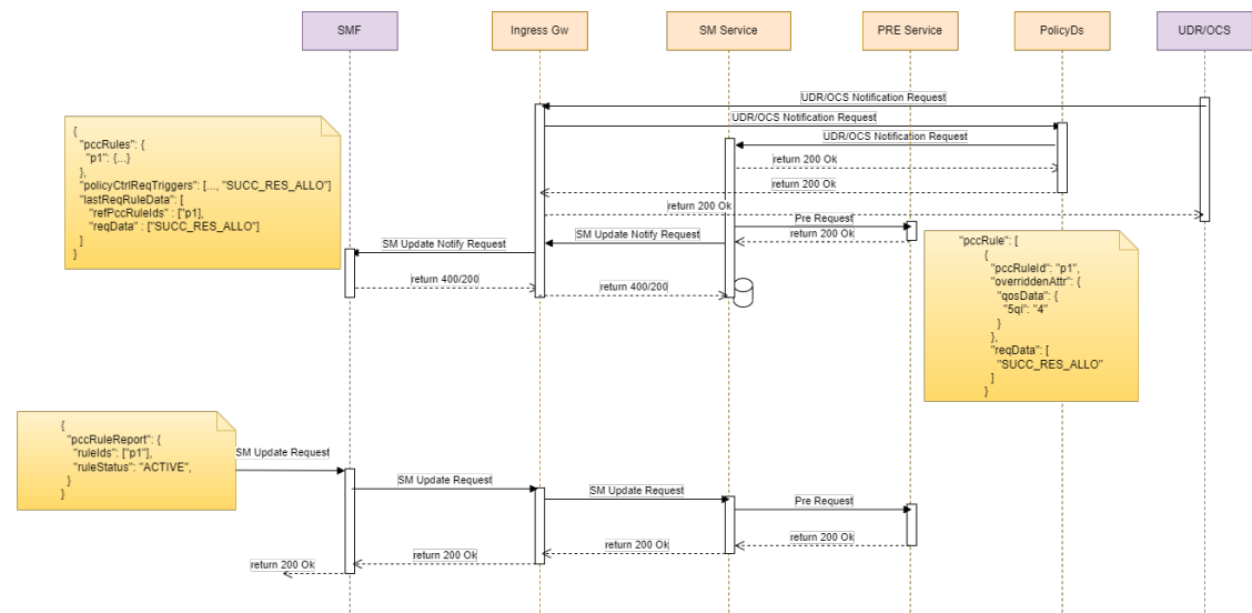
Figure 4-146 PCC Rule in SM-UPDATE-NOTIFY request (Re-authorization)
