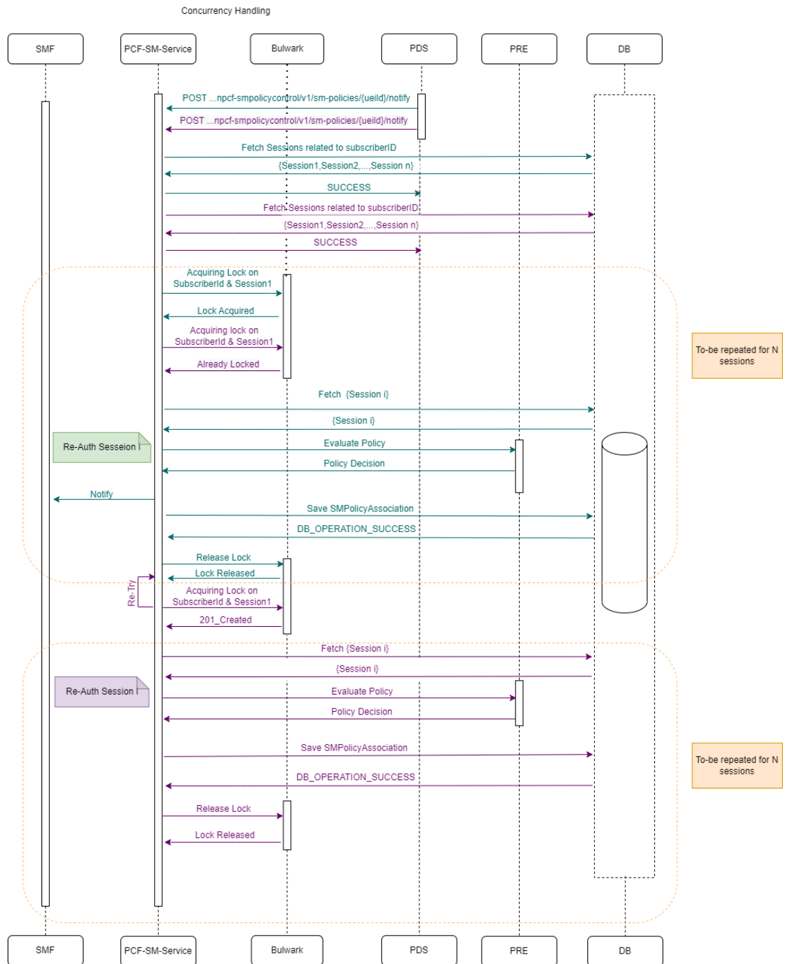
Figure 4-89 Call Flow for SM Update-Notify Request (Two Notifications from Same Subscriber and n Sessions Each)
