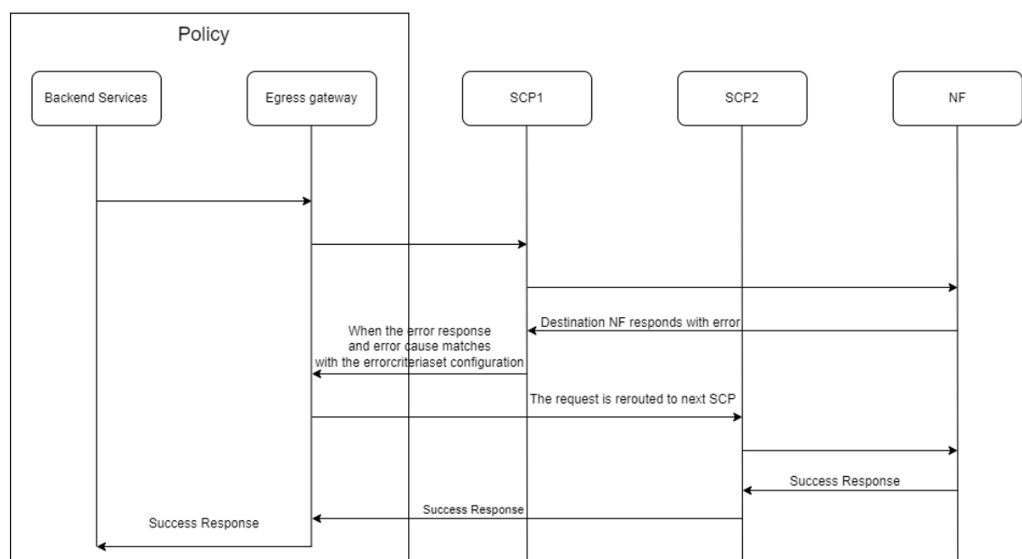
Figure 4-60 Session Retry at Egress Gateway
