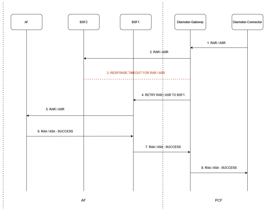
Figure 4-43 Call Flow RX RAR or RX ASR Timeout Retry - Success Case:
