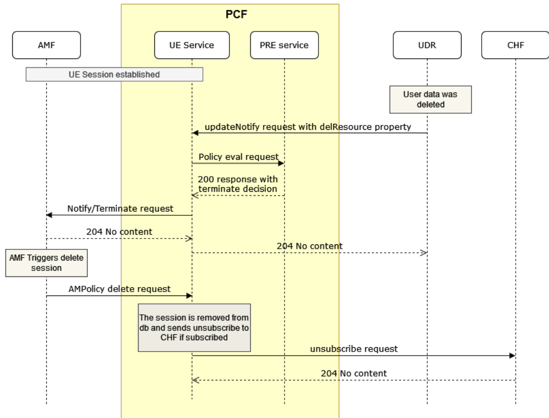
Figure 4-15 Call Flow for UE Terminate for UDR updateNotify with delResources
