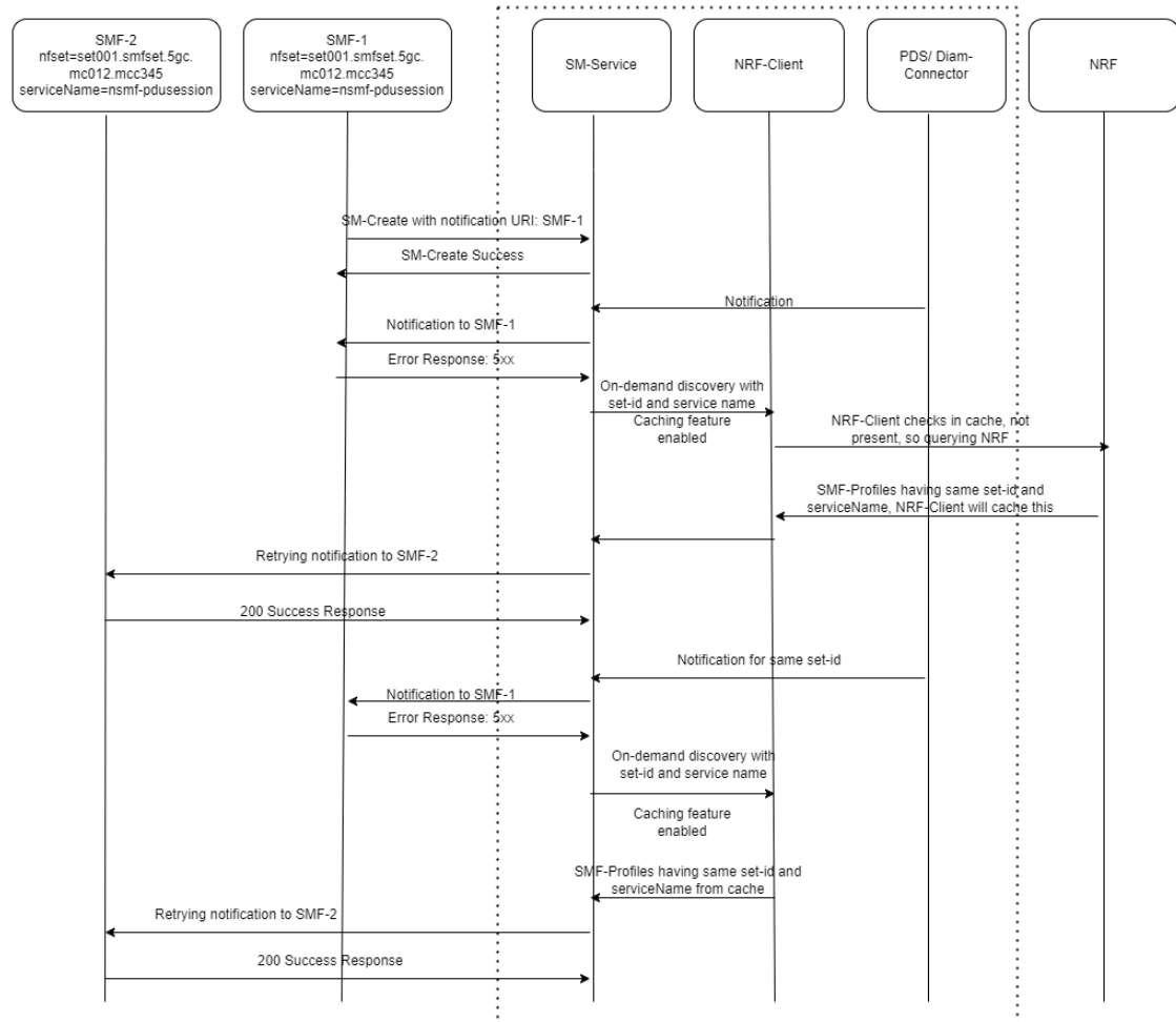
Figure 4-1 SMF Notification for SM Policy (NFSetid based discovery for retry on Notification Request failure)
