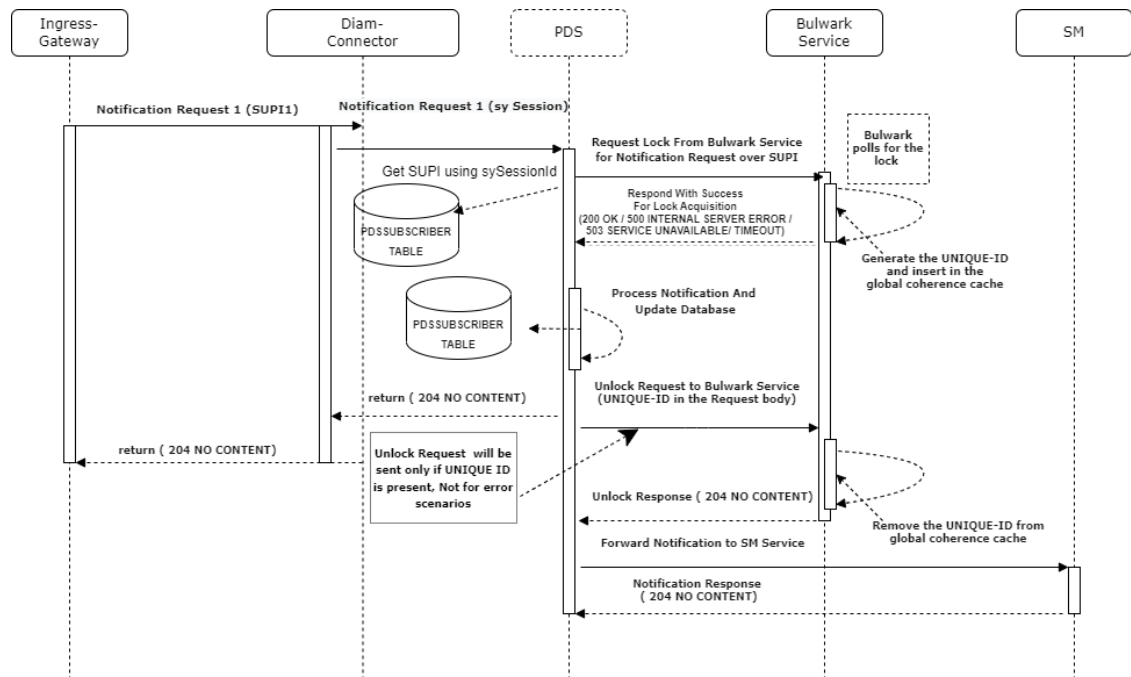
Figure 4-121 Call Flow - Bulwark Lock Request For OCS Notification
