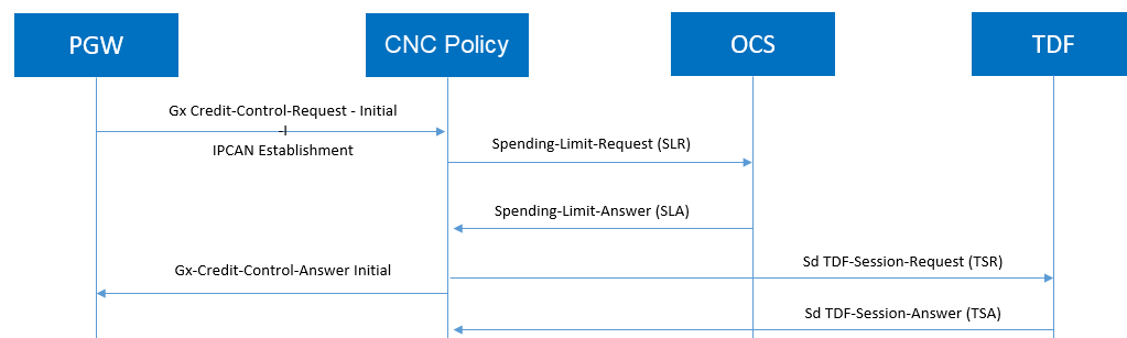
Figure 4-123 Call Flow for TDF Session
