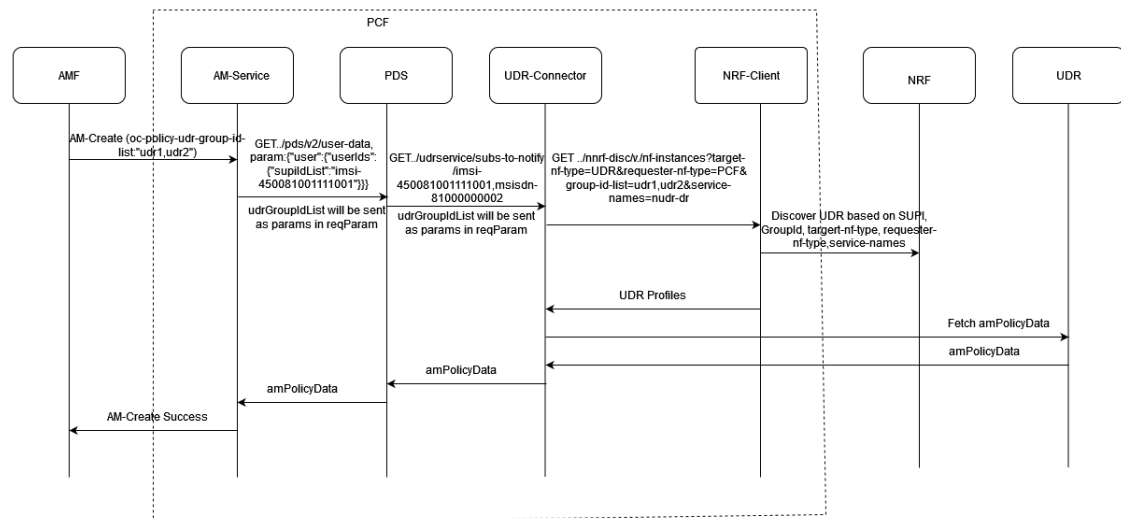
Figure 4-25 AMF sends AM Policy Association Request with oc-policy-udr-group-id
