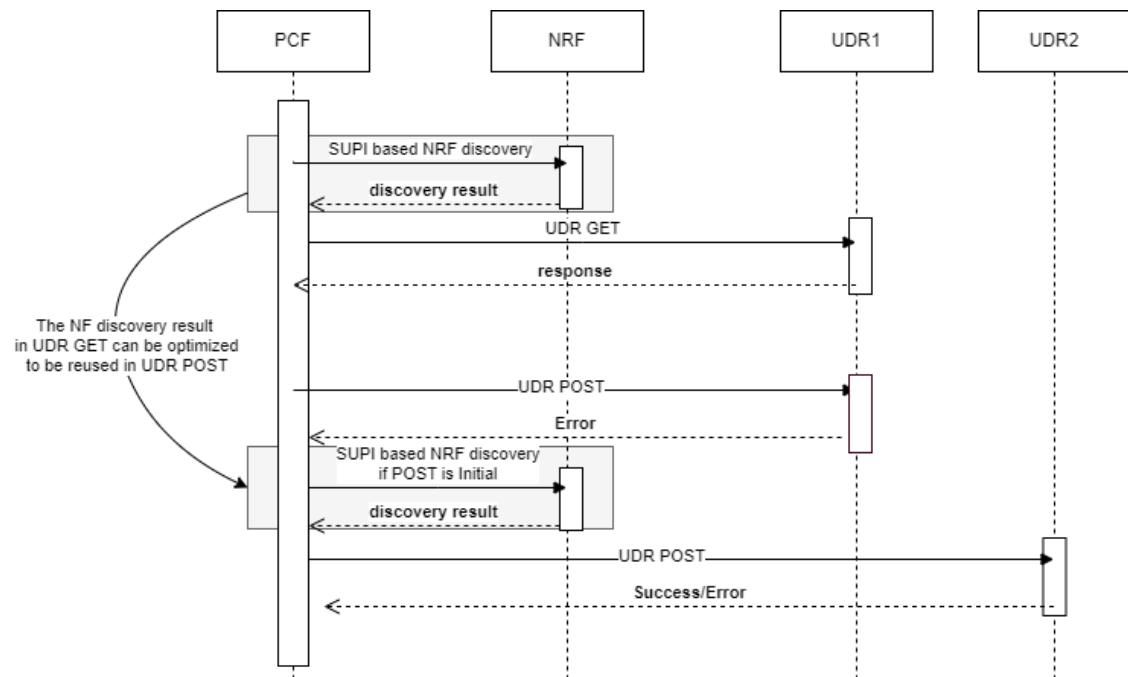
Figure 4-29 UDR GET Discovery Result Reused in UDR POST
