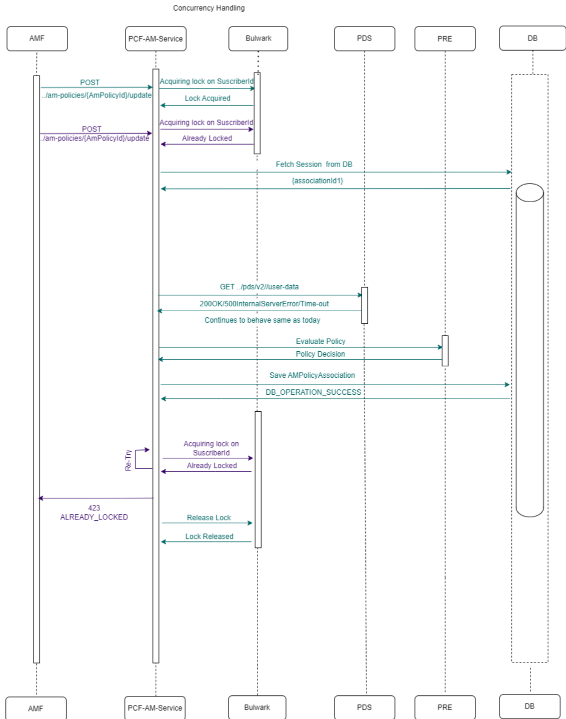
Figure 4-106 Two AM-Update requests for same Subscriber but different Sessions and retry failure (retry =1)
