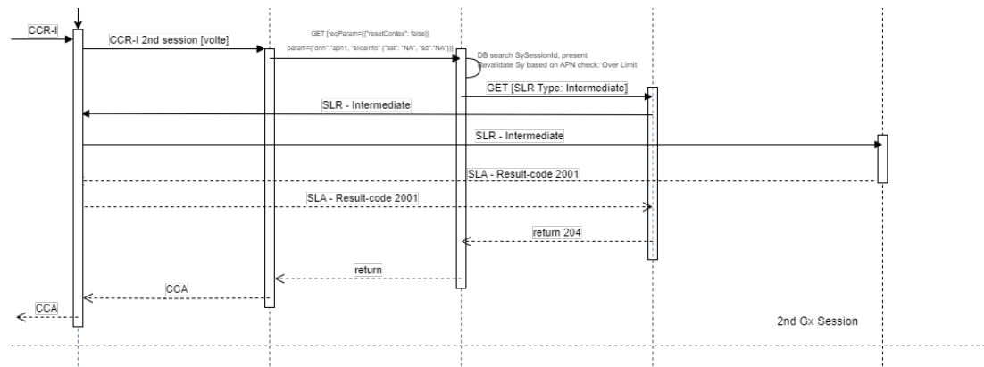
Figure 4-9 Second Gx Session
