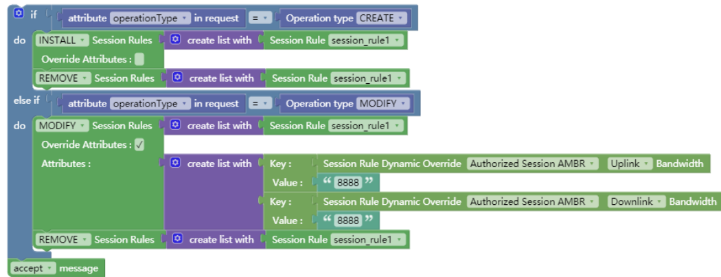
Figure 4-40 Example of Policy with Conflicts in a Session Rule
