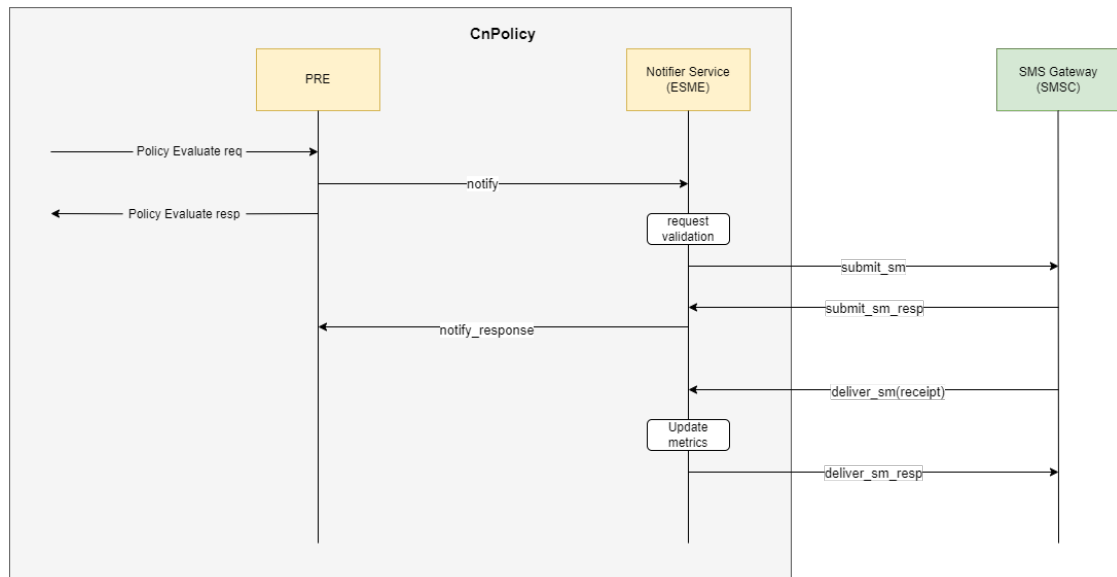
Figure 4-35 Call flow for sending messages using SMPP protocol
