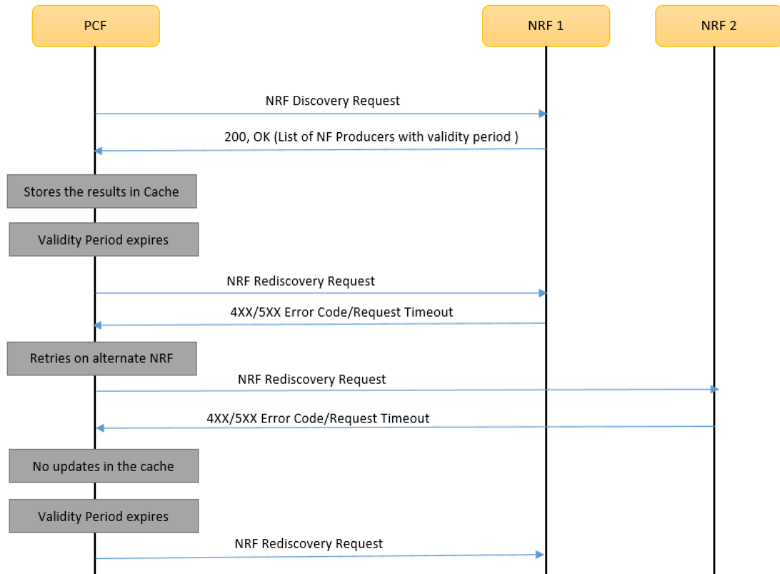
Figure 4-136 Call Flow - NF Discovery Error Scenario
