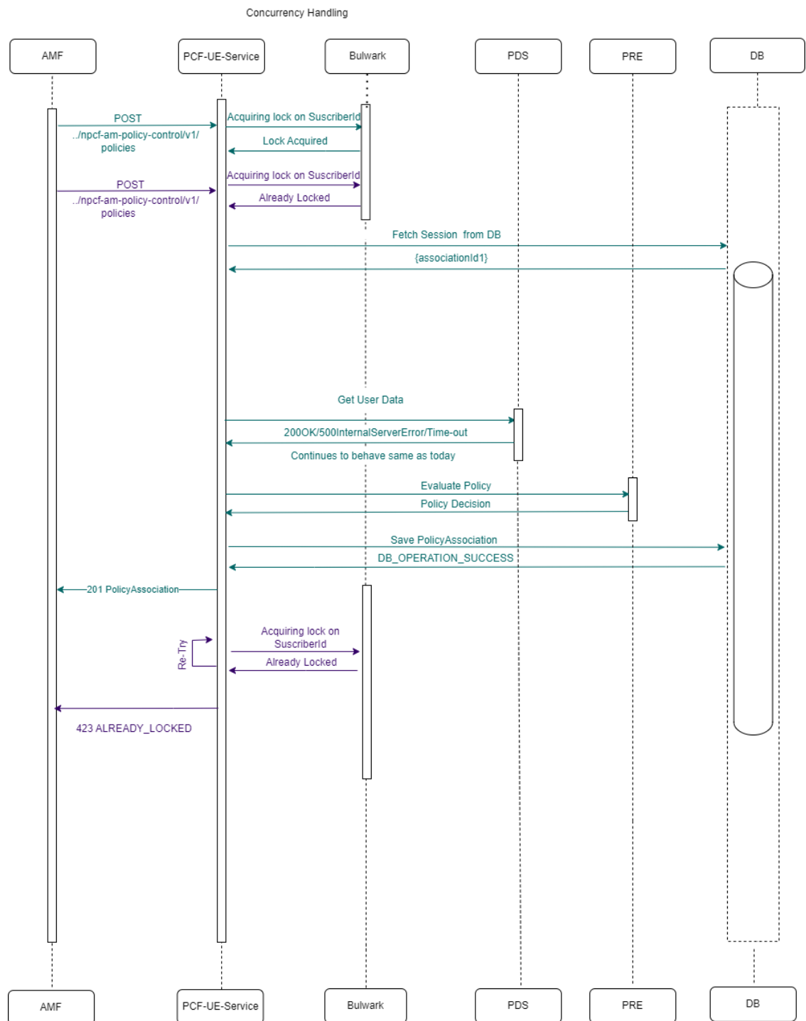
Figure 4-110 Two UE-Create requests for same Subscriber and retry failure (retry =1)
