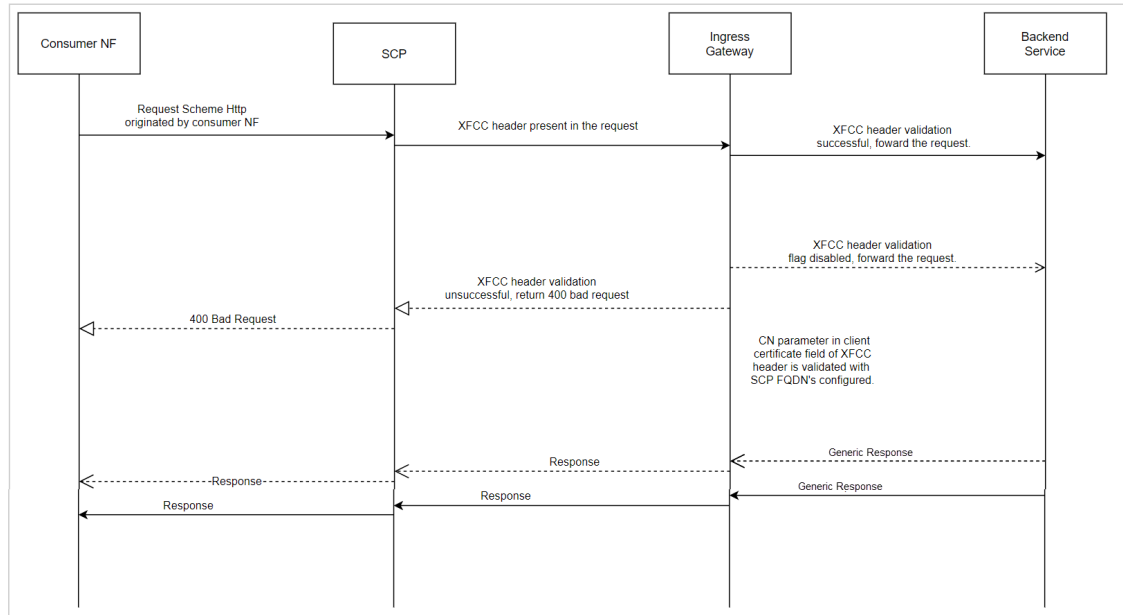
Figure 4-80 Call Flow Validating single XFCC Header
