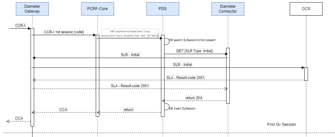
Figure 4-8 First Gx Session
