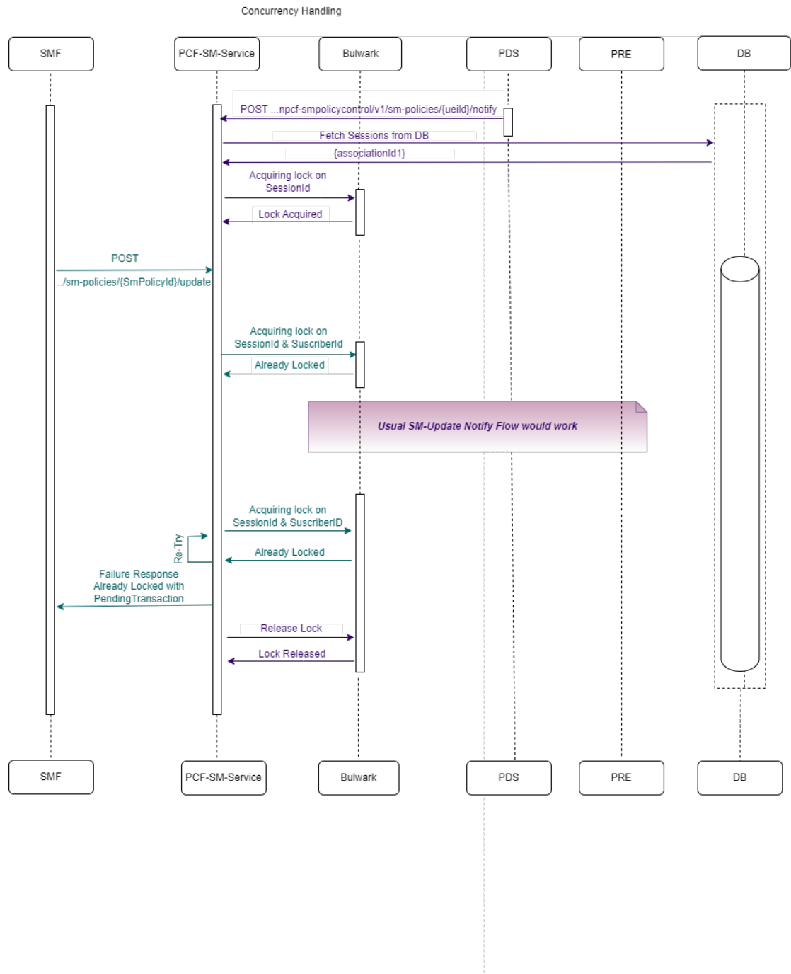
Figure 4-94 Pending transaction and Concurrent SM-Update for same session - Retry failure scenario
