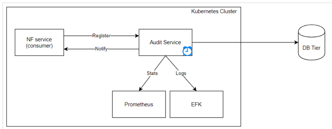
Figure 4-64 High Level Design for Stale Session Handling using Audit Service
