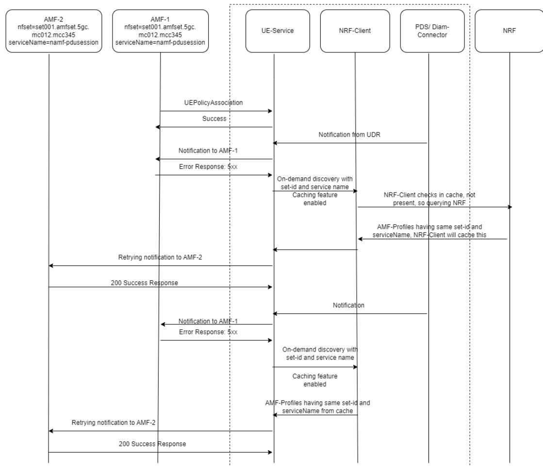
Figure 4-3 AMF Notification for UE Policy (NFSetid based discovery for retry on Notification Request failure)
