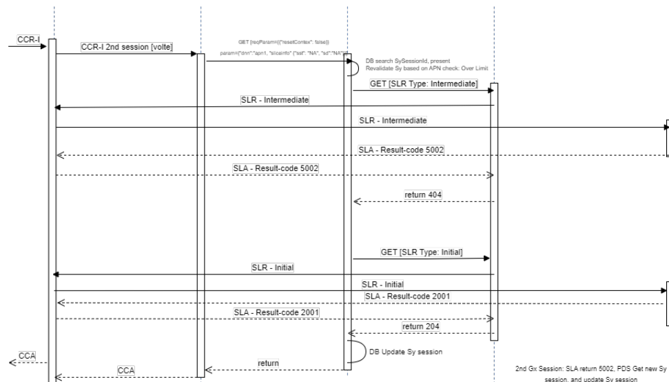
Figure 4-10 Second Gx Session: SLA Returns 5002, Get New Sy Session, PDS Update Sy Session
