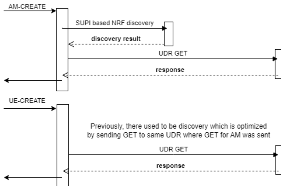
Figure 4-30 Reuse of UDR profile for amPolicyData GET in uePolicySet GET
