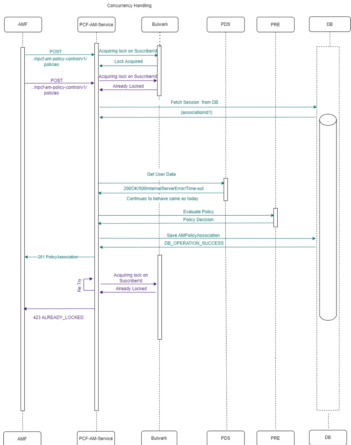
Figure 4-102 Two AM-Create requests for same Subscriber and retry failure (retry =1)
