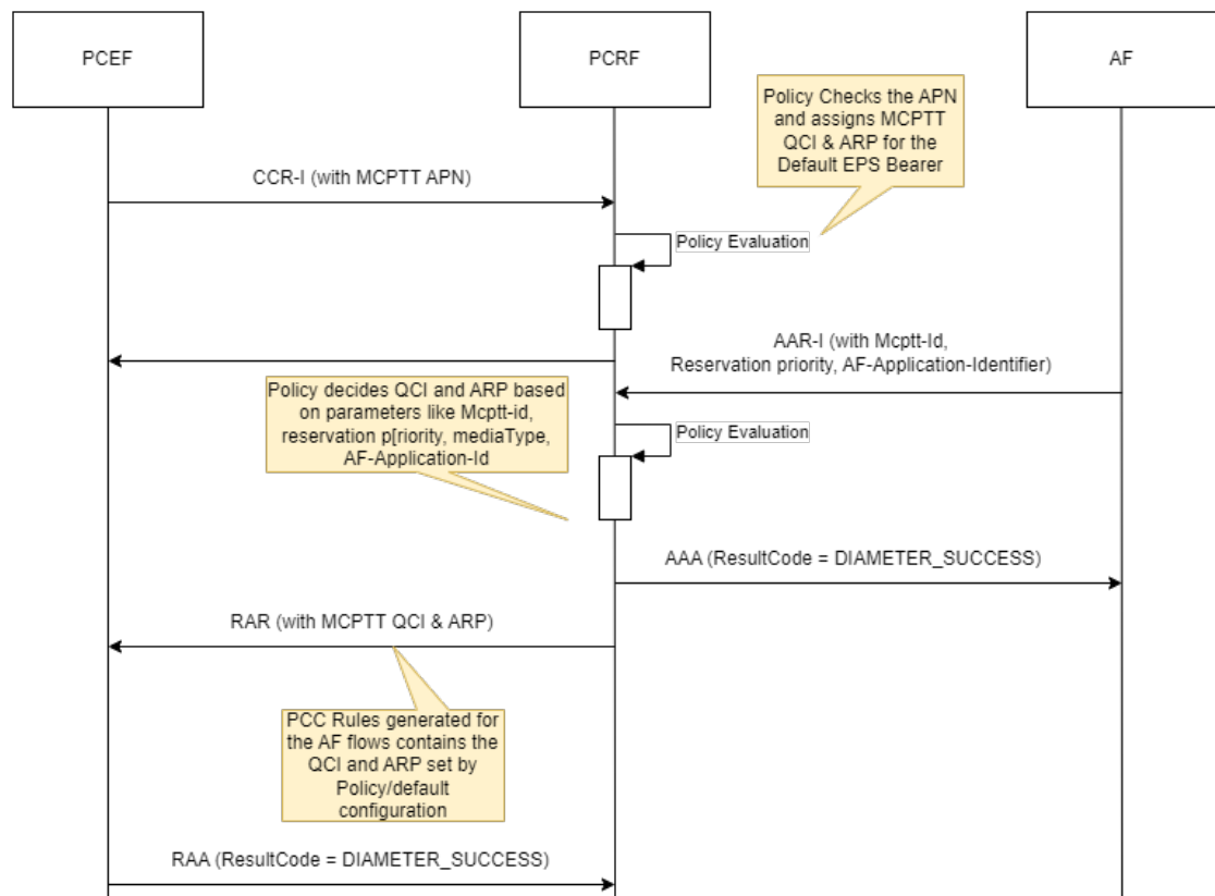
Figure 4-153 MCPTT QCI & ARP settings for MCPTT AF flows
