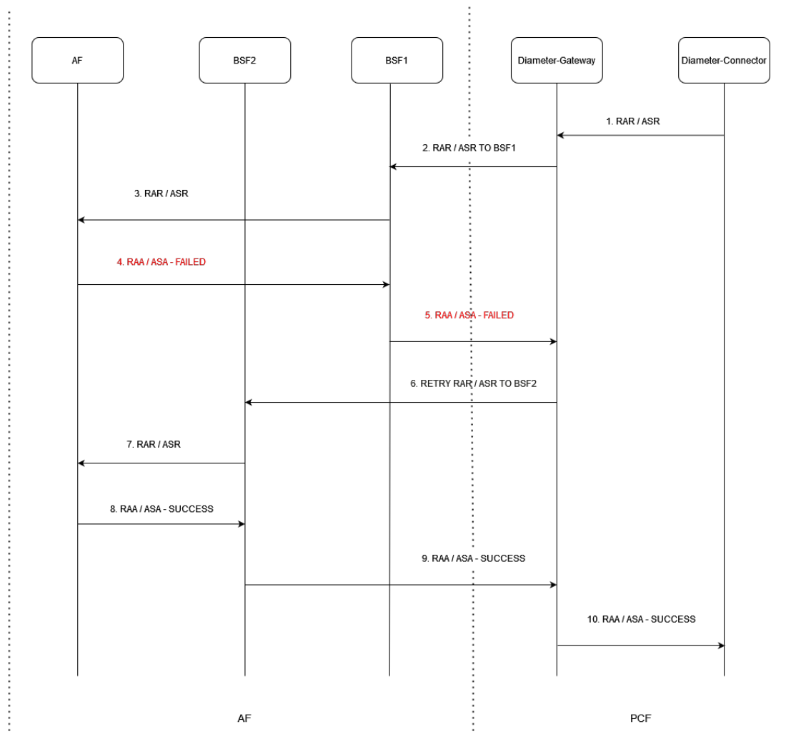
Figure 4-46 RX RAR/RX ASR Retry - Error Originated by Destination Peer (Not Intermediate Peer)
