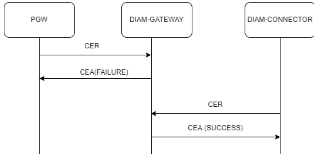
Figure 4-131 Call Flow for Diameter Gateway COMPLETE SHUTDOWN
