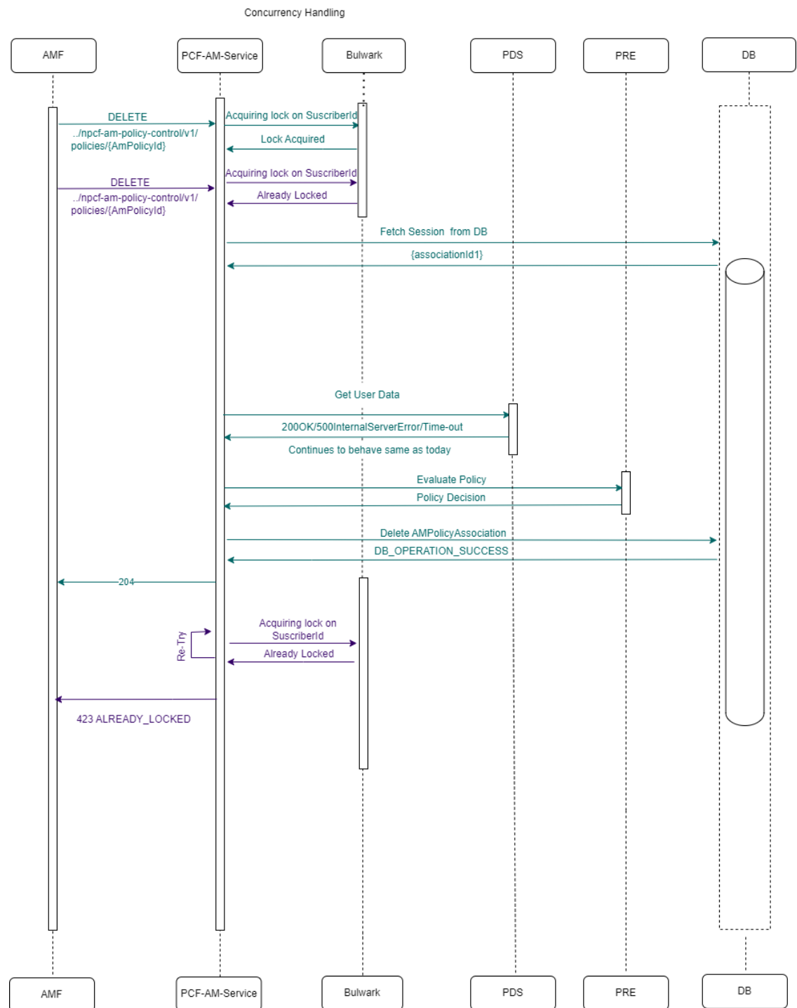
Figure 4-104 Two AM-Delete requests for same Subscriber and retry failure (retry =1)
