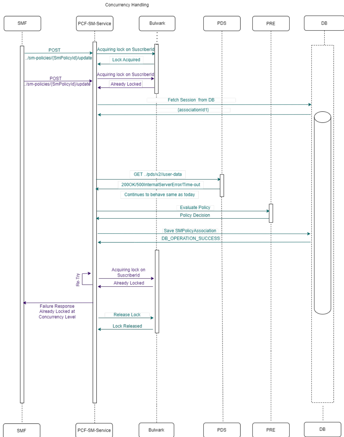
Figure 4-92 Retrial failure when there are multiple updates for same subscriber in different sessions
