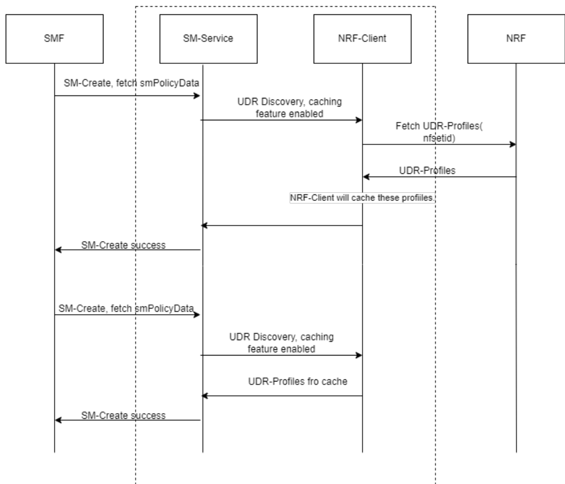
Figure 4-5 Non-SUPI based on-demand discovery caching for User Service
