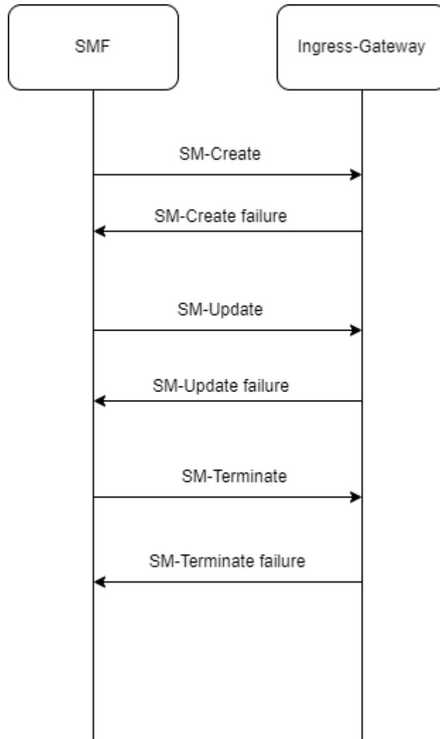
Figure 4-134 Call Flow for Ingress Gateway COMPLETE SHUTDOWN
