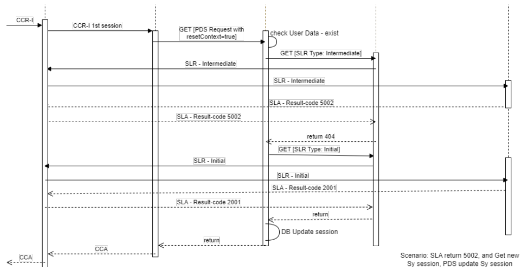
Figure 4-7 SLA Returns 5002, Get New Sy Session, PDS Update Sy Session
