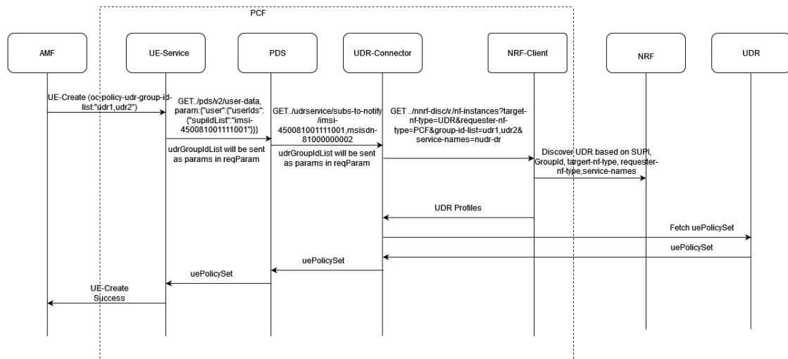
Figure 4-26 AMF sends UE Policy Association Request with oc-policy-udr-group-id
