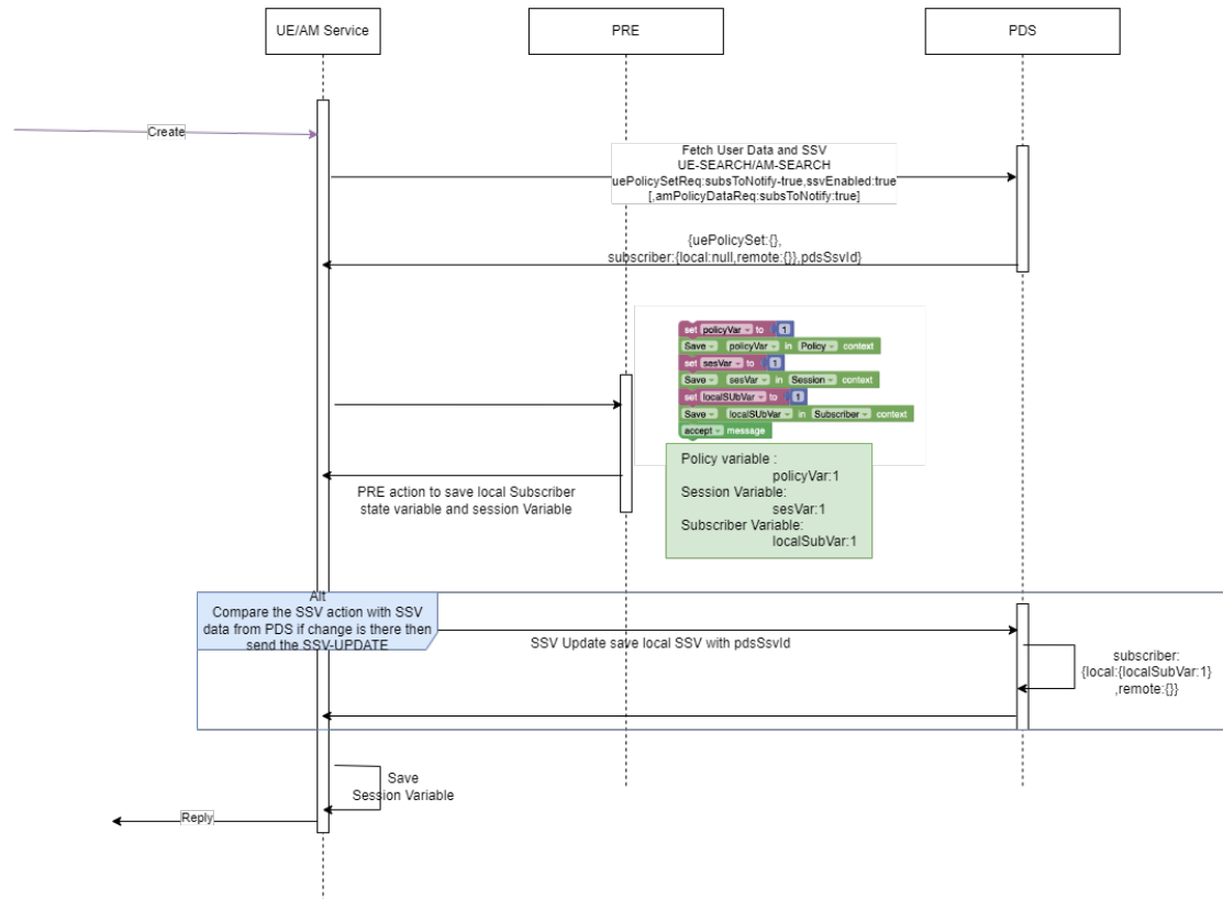
Figure 4-148 State variables in create session call flow
