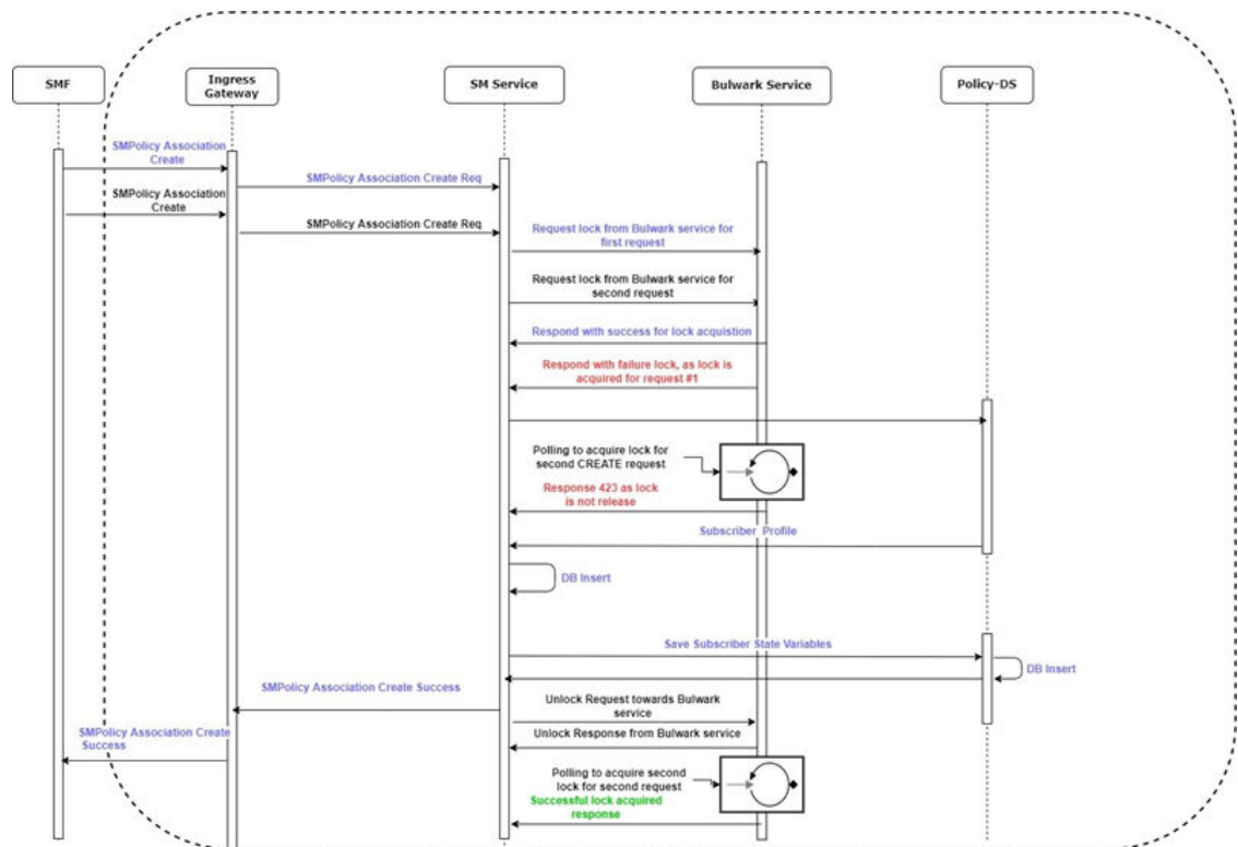
Figure 4-85 Call Flow - Bulwark Lock Request SM Create Procedure
