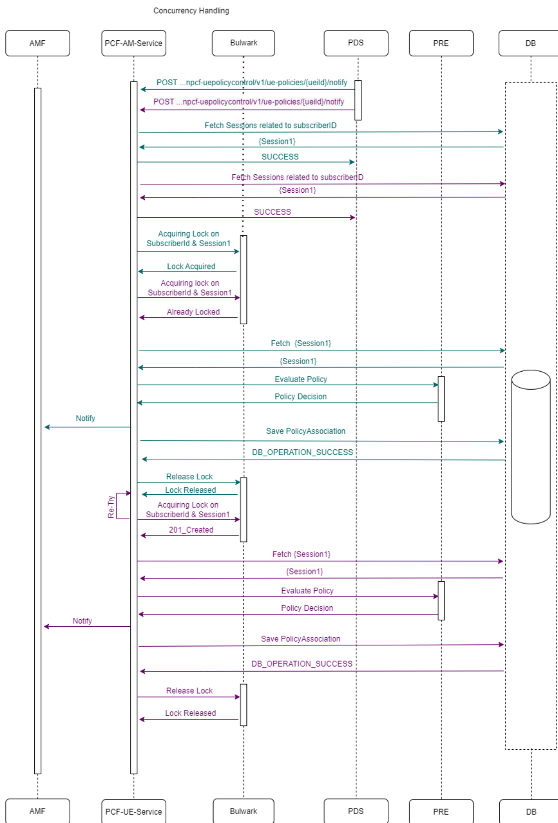
Figure 4-115 Two UENotify requests for same Subscriber each having 1 session
