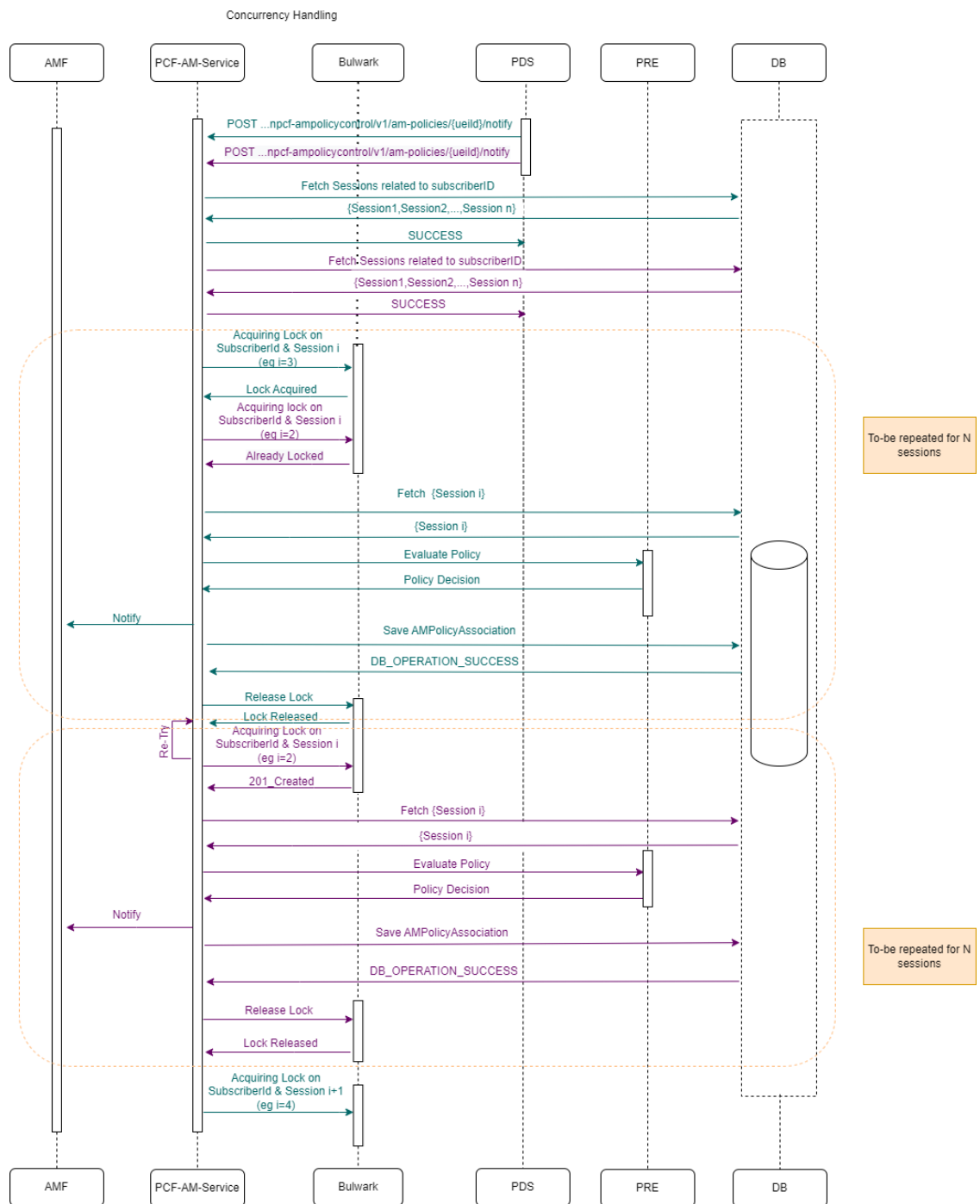
Figure 4-108 Two AM-Notify request for same Subscriber each having n Sessions
