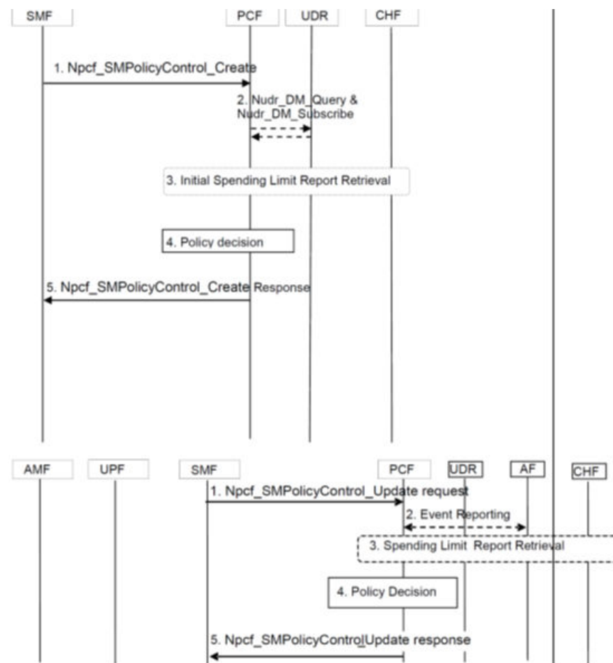
Figure 4-37 PRA Support for SM Service
