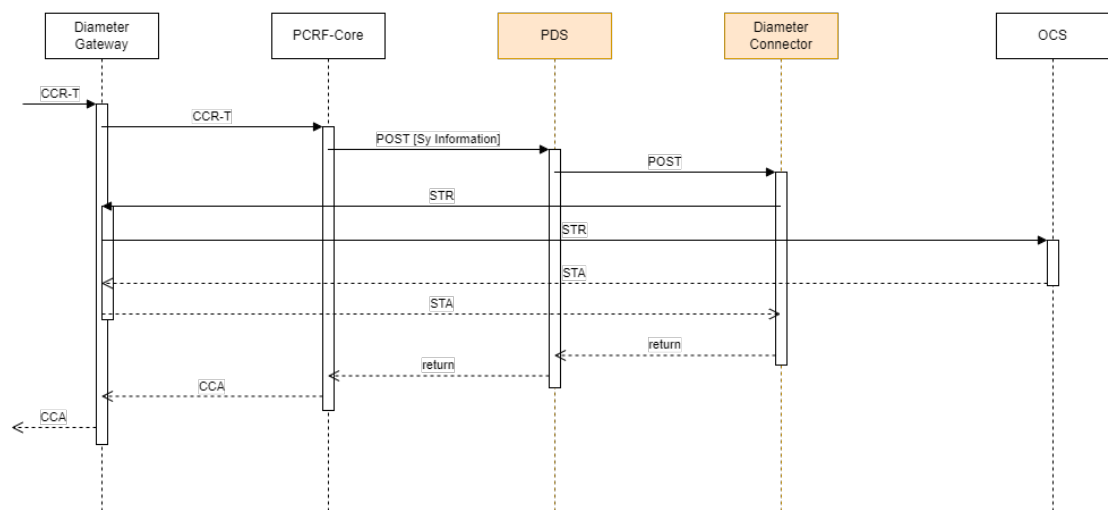
Figure 4-79 Communicating STR messages
