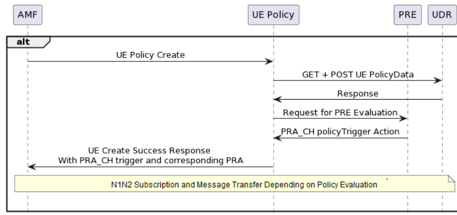
Figure 4-38 UE Policy Association create scenario:
