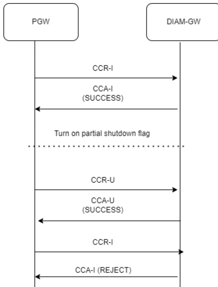
Figure 4-130 Call Flow for Diameter Gateway PARTIAL SHUTDOWN
