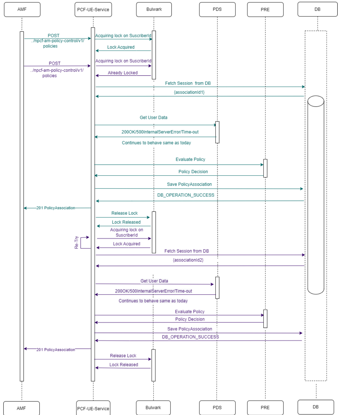
Figure 4-109 Two UE-Create requests for same Subscriber and retry success.
