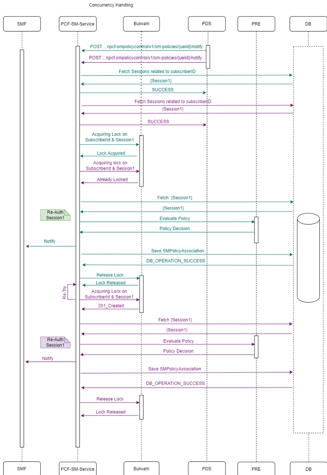
Figure 4-88 Call Flow for SM Update-Notify Request (Two Notifications and 1 Session)
