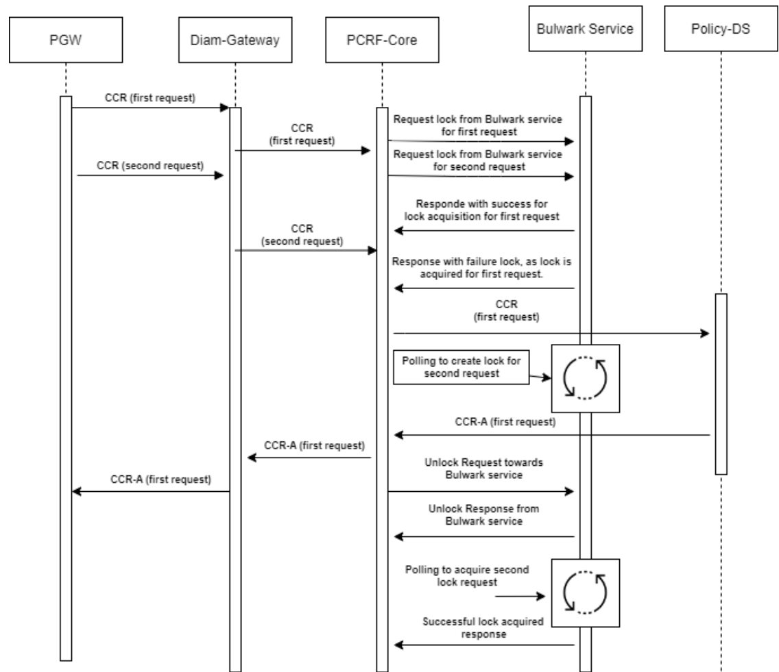
Figure 4-117 CCR-I, CCR-U and CCR-T messages Integration with Bulwark Service
