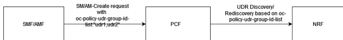
Figure 4-23 UDR Discovery with oc-policy-udr-group-id-list Header to NRF
