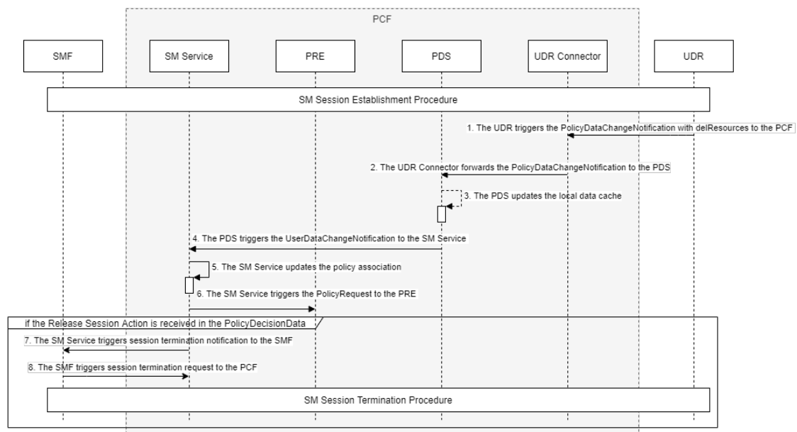
Figure 7-12 Call Flow for UDR Subscriber Resource Deletion
