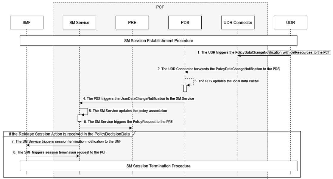
Figure 4-17 Call Flow for SM Terminate for UDR updateNotify with delResources
