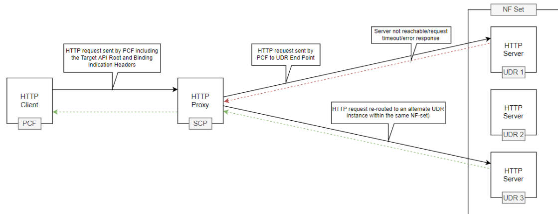
Figure 4-71 Example of NF Set and Binding Header based Indirect Communication
