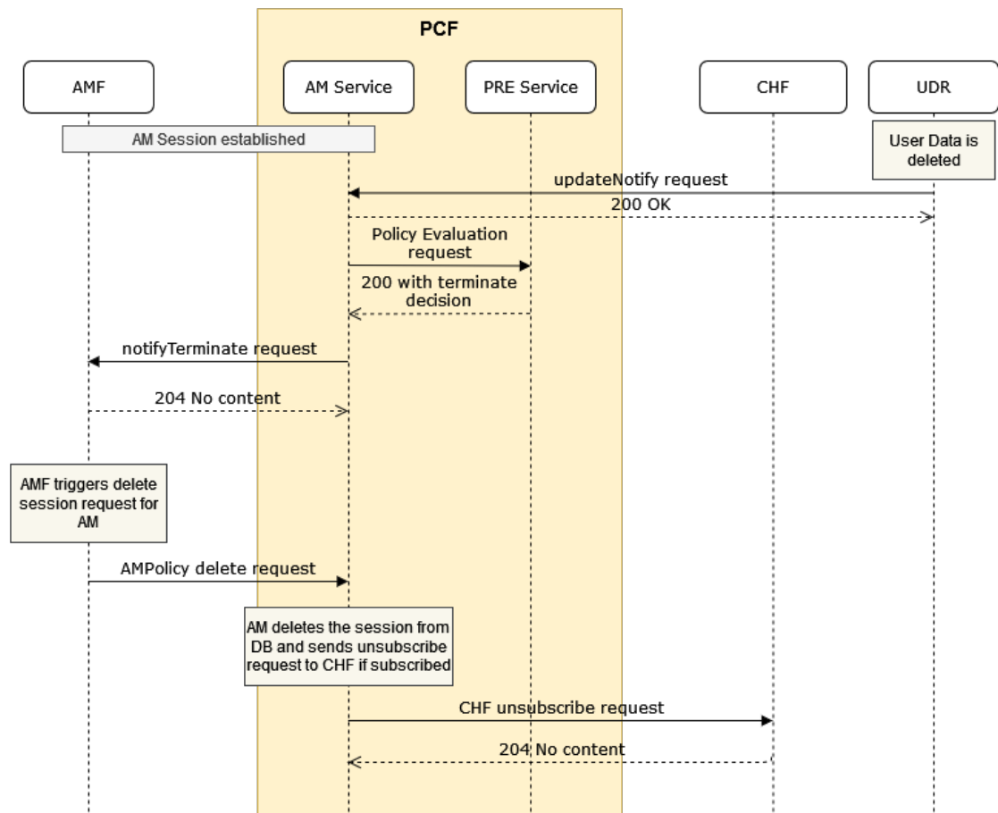
Figure 4-13 Call Flow for AM Terminate for UDR updateNotify with delResources
