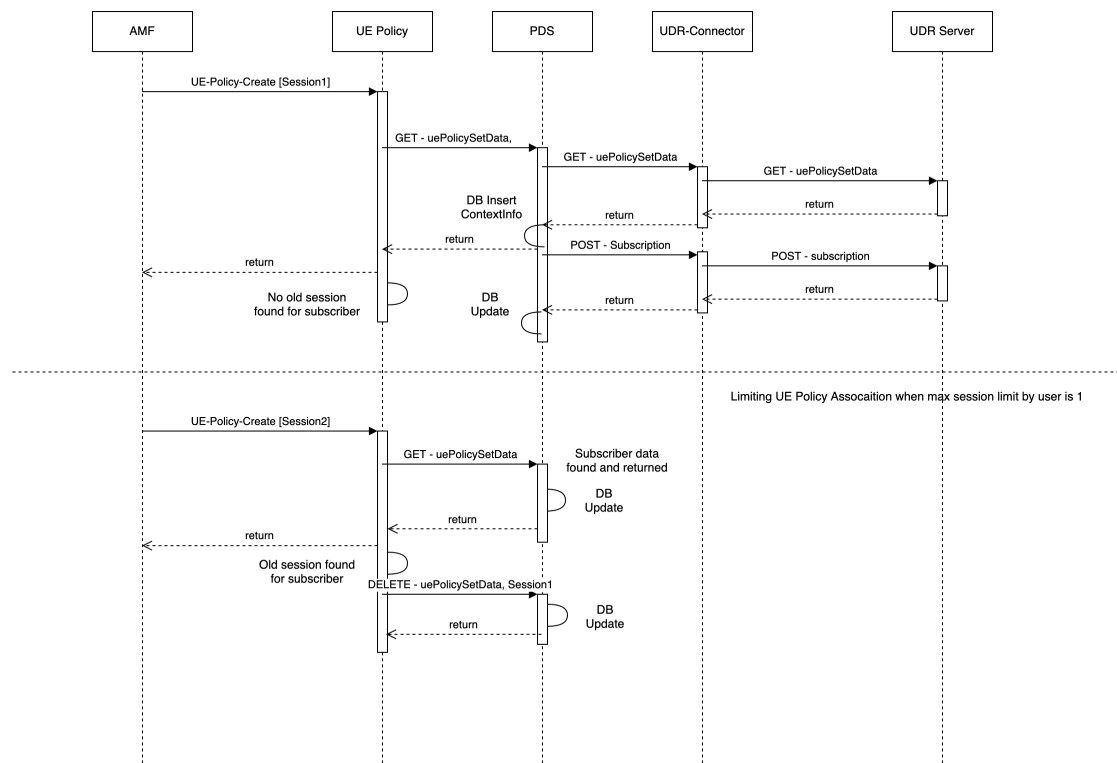
Figure 4-137 Limiting the number of sessions for UE Policy Service
