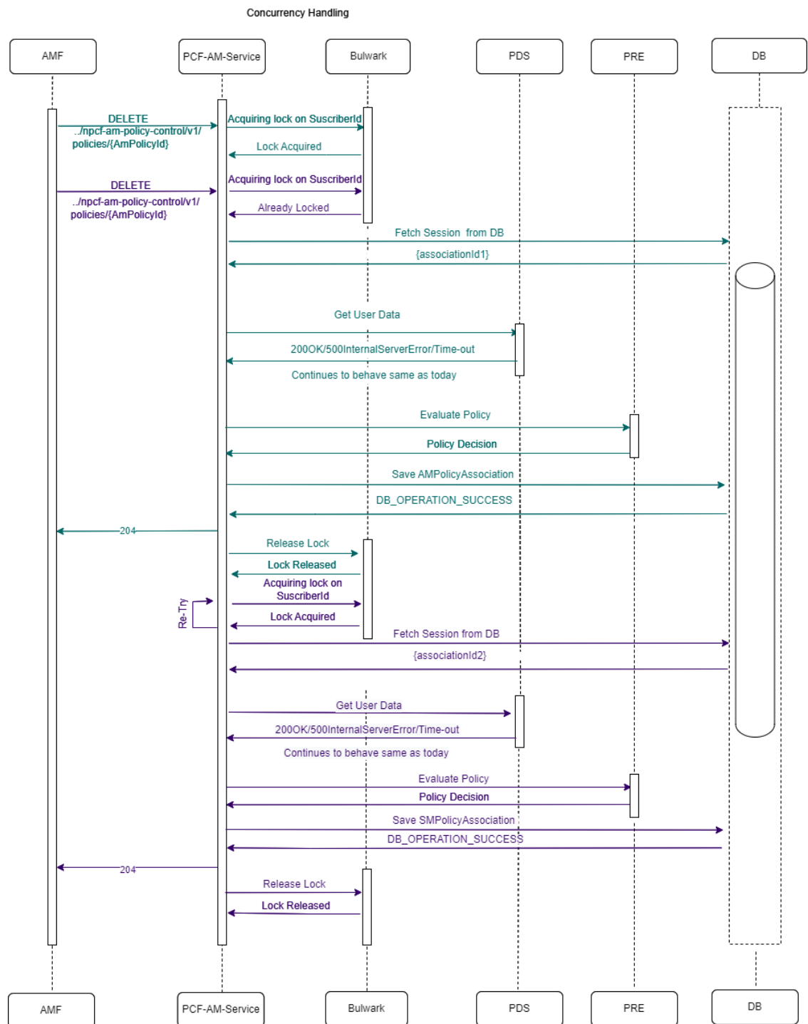
Figure 4-103 Two AM-Delete requests for same Subscriber and retry success
