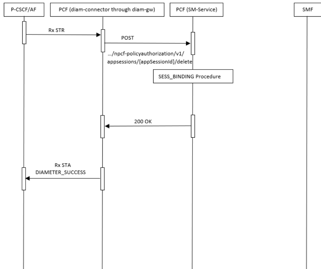
Figure 4-55 Cancellation of subscription to notification of the AF Signaling Transmission in 5G
