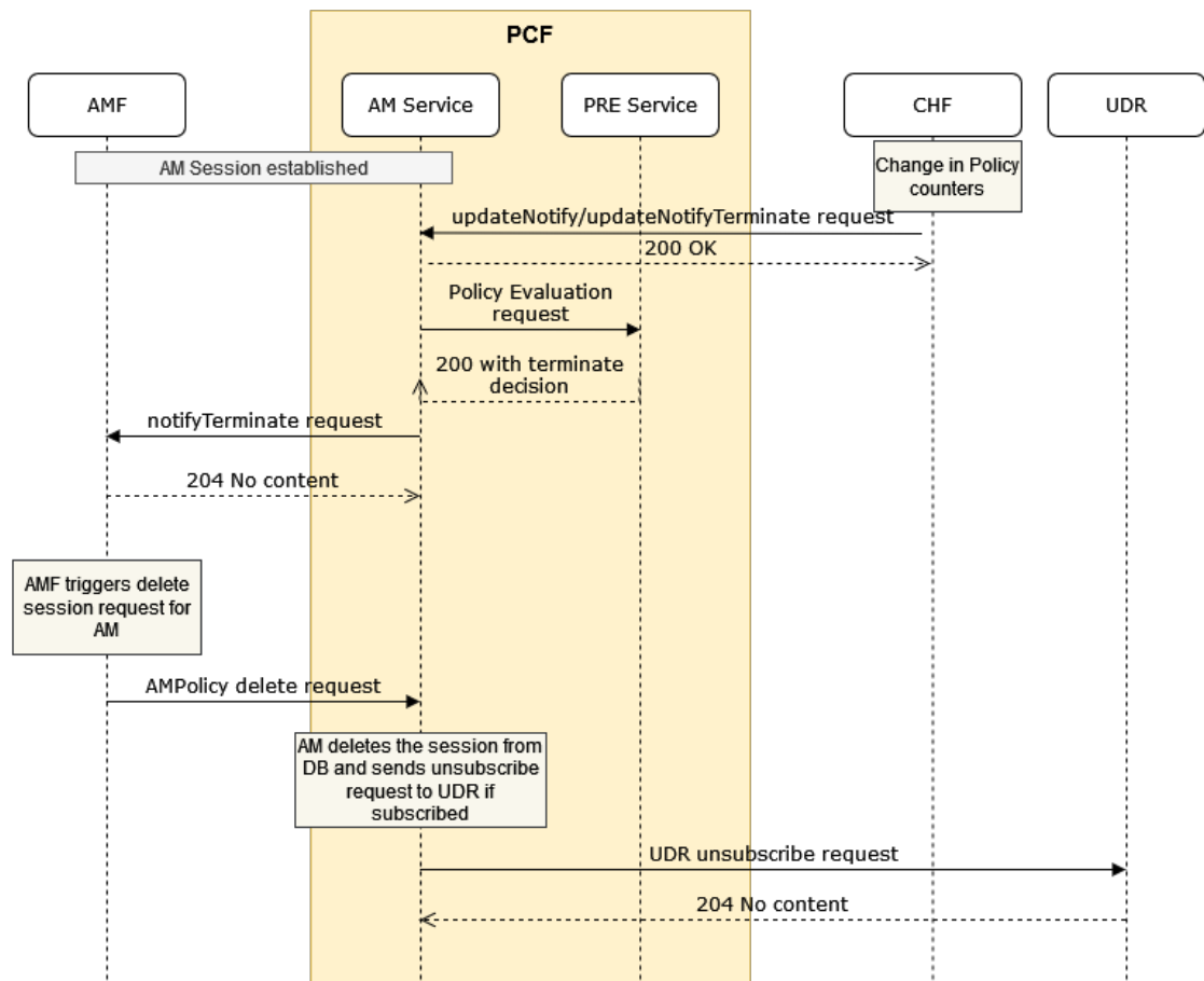
Figure 4-14 Call Flow for AM Terminate for CHF updateNotify or TerminateNotify
