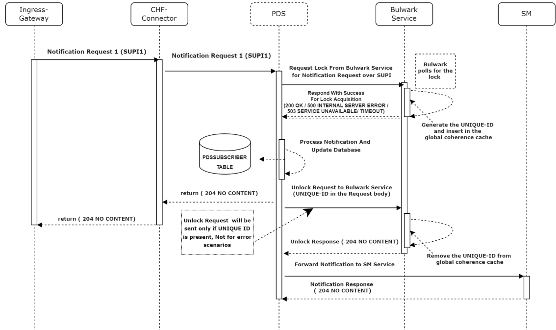
Figure 4-119 Call Flow - Bulwark Lock Request For CHF Notification
