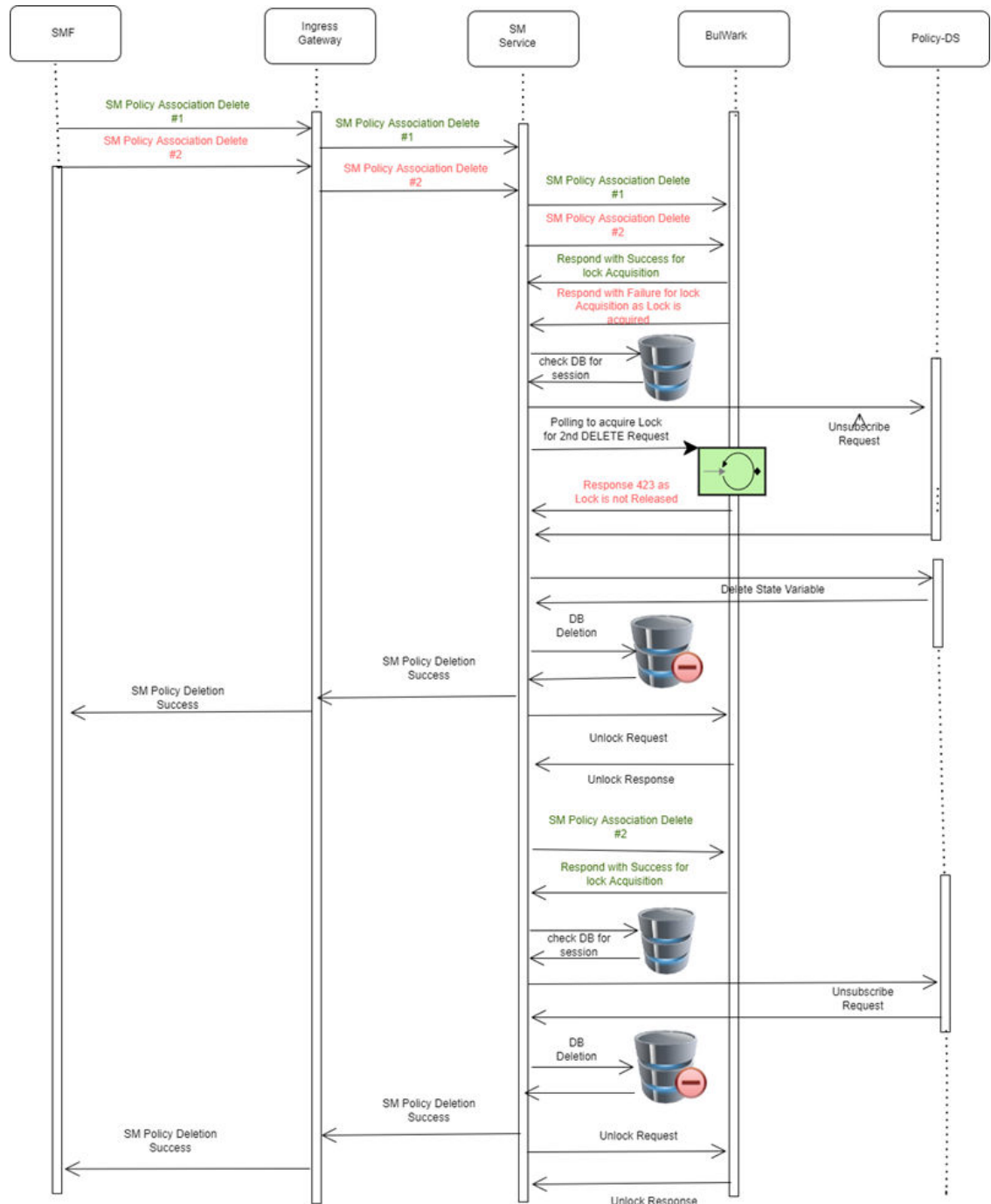
Figure 4-97 Call Flow - Bulwark Lock Request SM Delete Procedure
