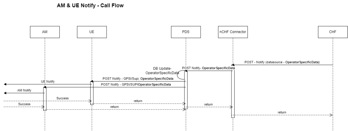
Figure 4-142 Update notification to AM Service and UE Policy Service
