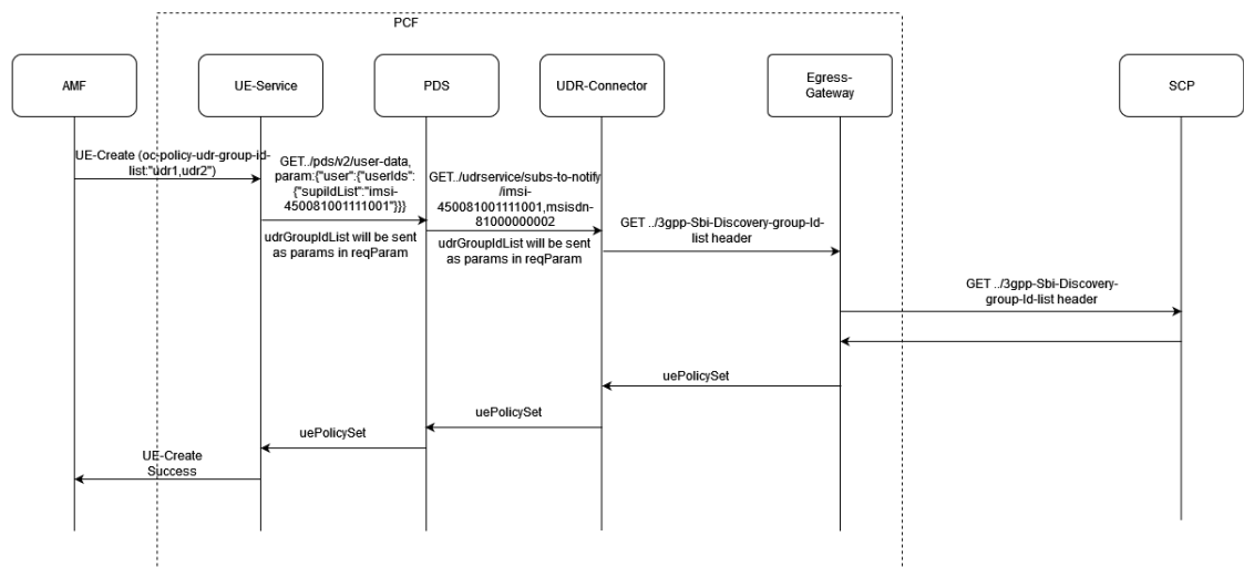
Figure 4-28 Model D, AMF sends UE Policy Association Request with oc-policy-udr-group-id-list
