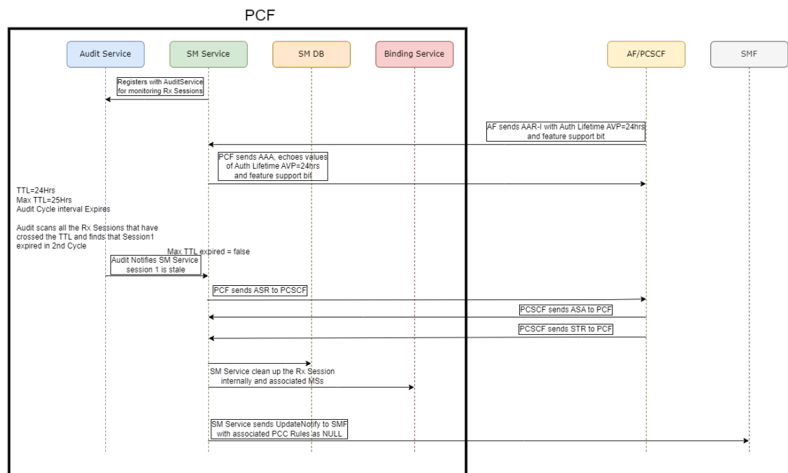
Figure 4-31 Rx Stale Session Detection and Deletion Based on TTL and Authorization-Lifetime
