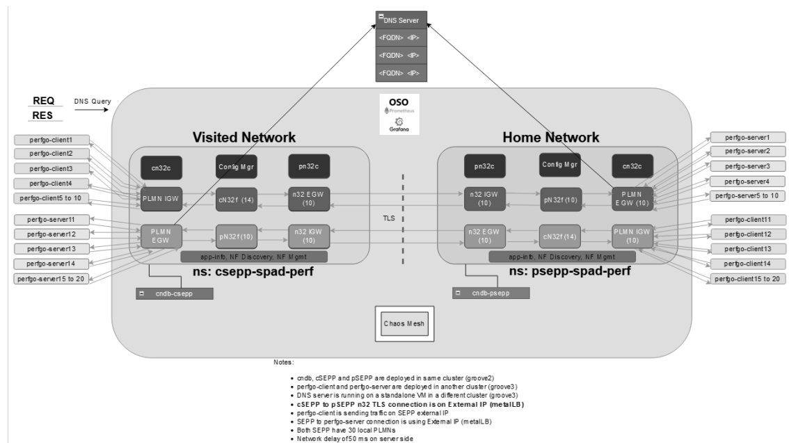
Figure 2-1 Deployment Diagram
