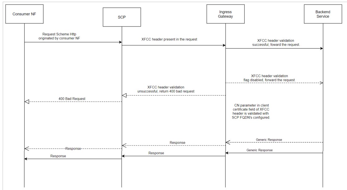
Figure 3-15 Call Flow Validation of Single XFCC Header
