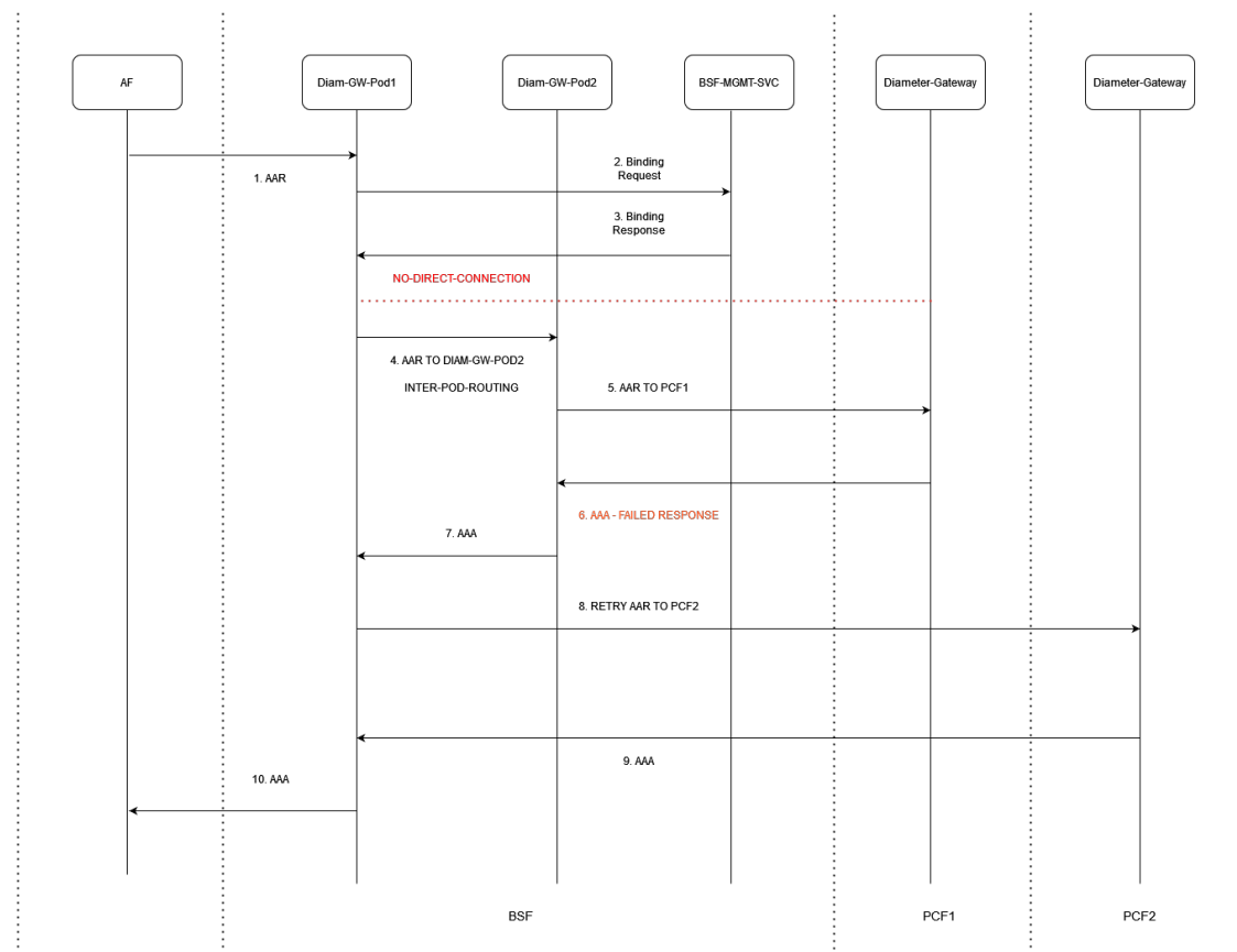
Figure 3-8 Rx AAR Retry Inter-Pod Routing Case - When Binding Found
