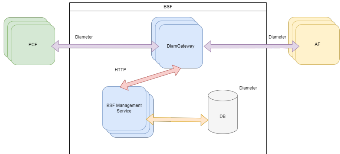
Figure 3-1 Diameter Gateway for BSF
