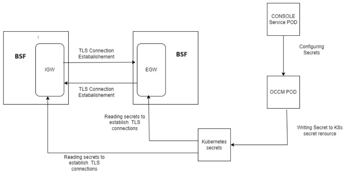
Figure 3-3 BSF Integration with OCCM
