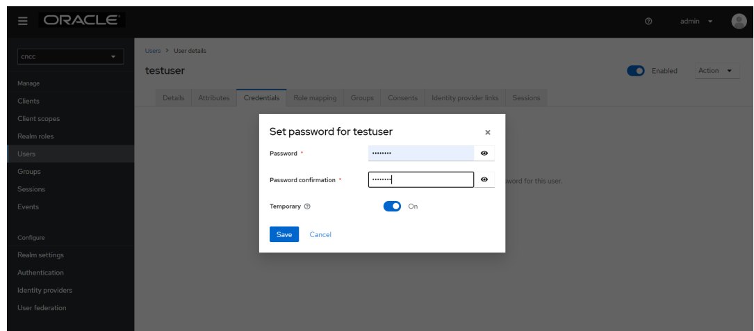
Figure 4-18 Set Password
