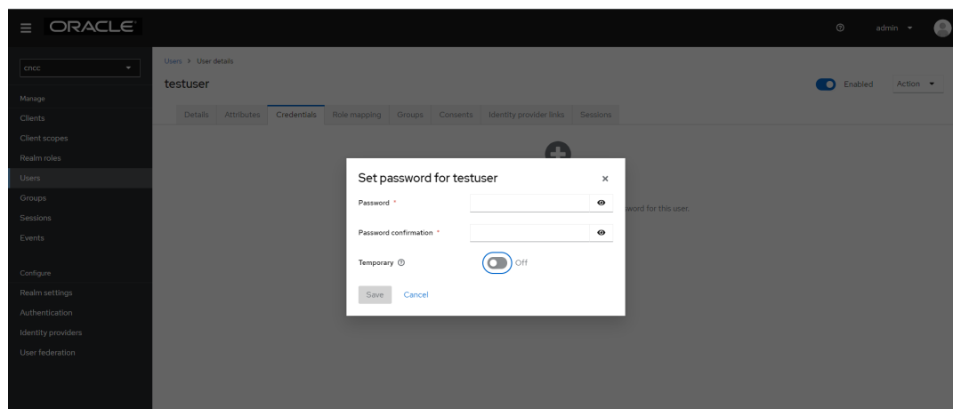
Figure 4-11 Credentials
