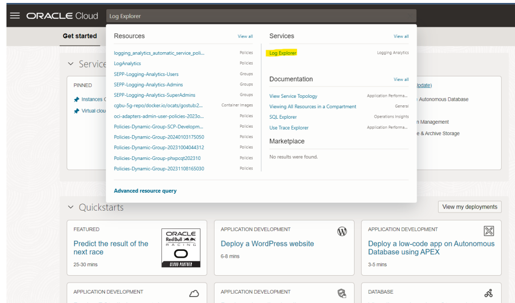
Figure 10-2 Log Explorer
