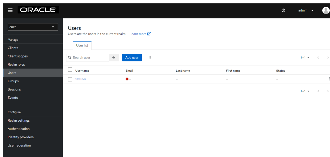
Figure 4-10 Users
