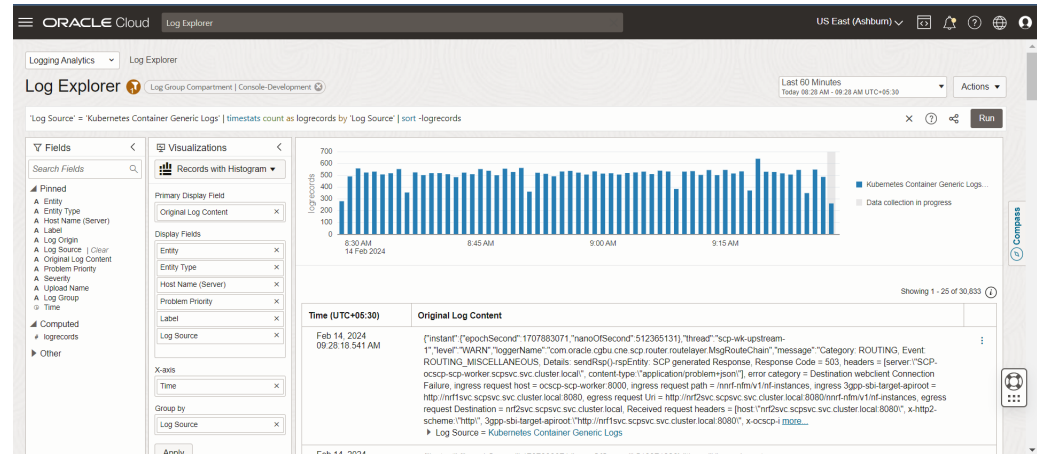
Figure 10-4 View Logs
