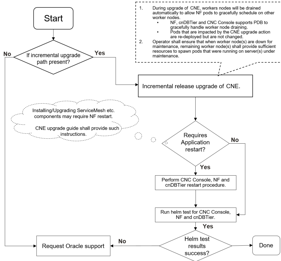
Figure 2-4 CNE Upgrade Procedure
