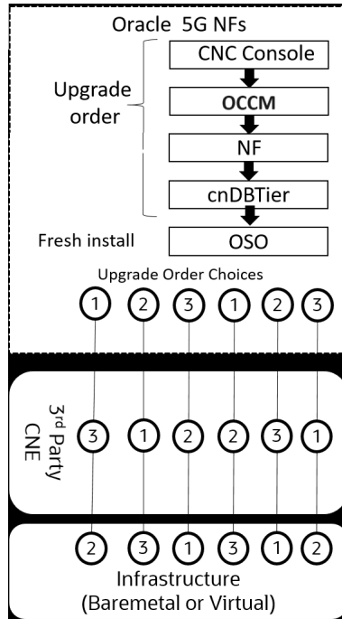
Figure 3-1 CNC Upgrade Order on Non-Oracle CNE
