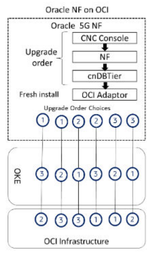
Figure 4-1 CNC Upgrade Order on OCI Environment
