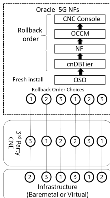
Figure 3-4 Rollback Sequence with Non-Oracle CNE
