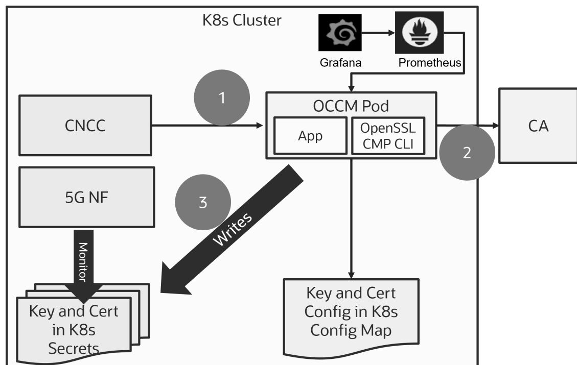
Figure 1-2 OCCM Architecture
