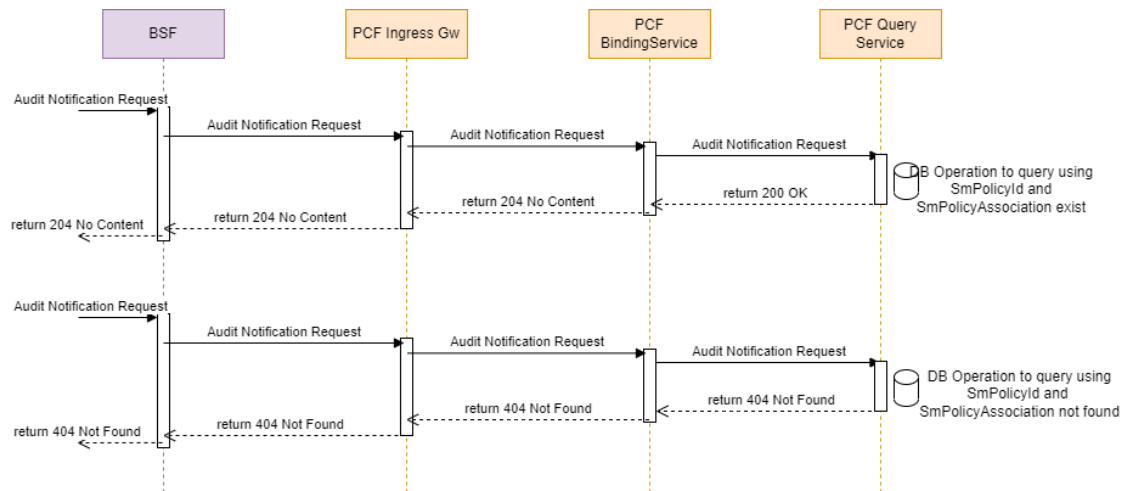
Figure 4-96 BSF and PCF Interaction for Stale Binding Detection
