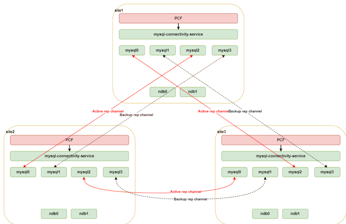
Figure 4-85 Three-Site Georedundancy Deployment
