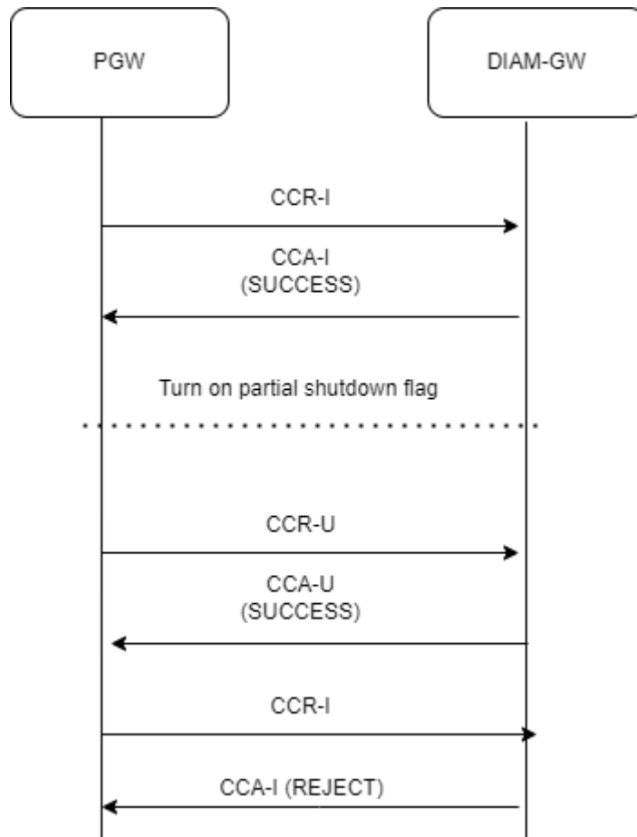
Figure 4-142 Call Flow for Diameter Gateway PARTIAL SHUTDOWN
