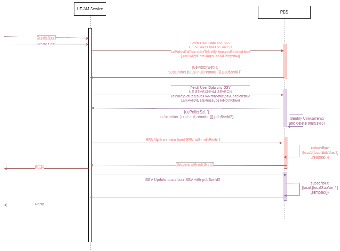
Figure 4-163 State variables in concurrent flows
