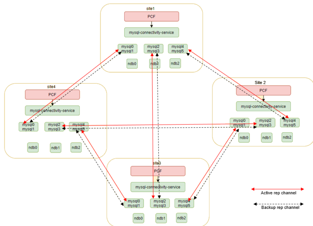
Figure 4-86 Four-Site Georedundancy Deployment
