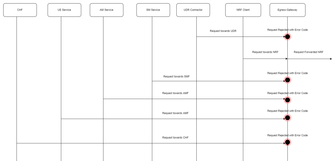
Figure 4-144 Call Flow for Egress Gateway COMPLETE SHUTDOWN
