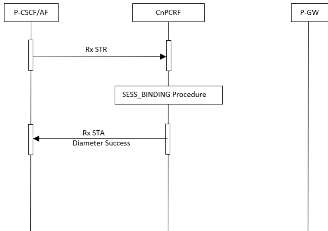
Figure 4-65 Cancellation of subscription to notification of the AF Signaling Transmission in 4G
