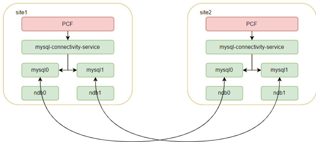
Figure 4-84 Two-Site Georedundancy Deployment
