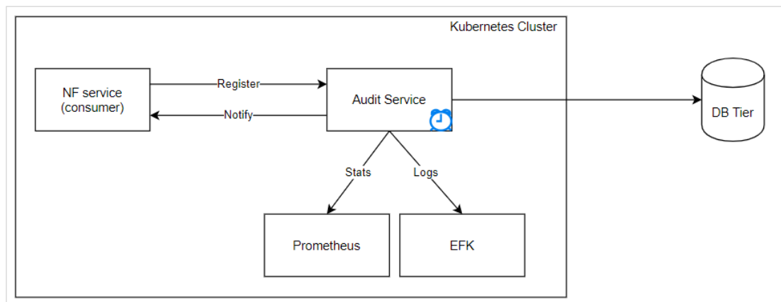
Figure 4-74 High Level Design for Stale Session Handling using Audit Service
