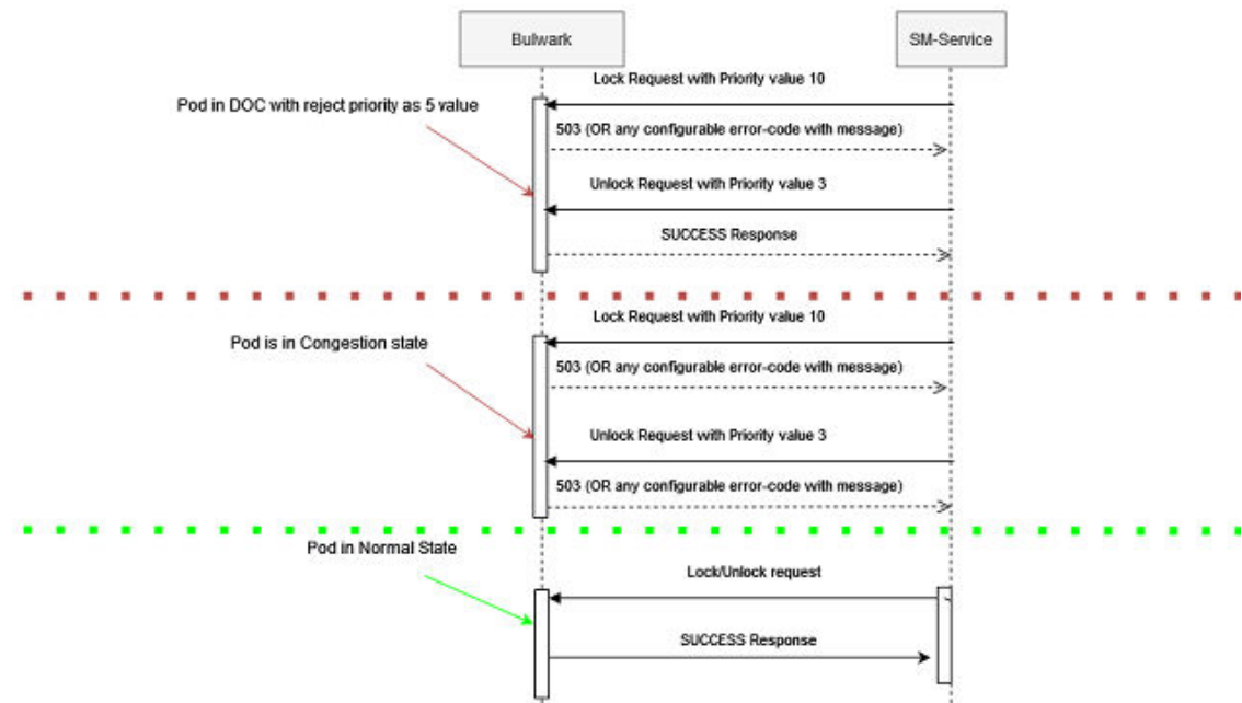
Figure 4-31 Call Flow Diagram for Bulwark Congestion Control
