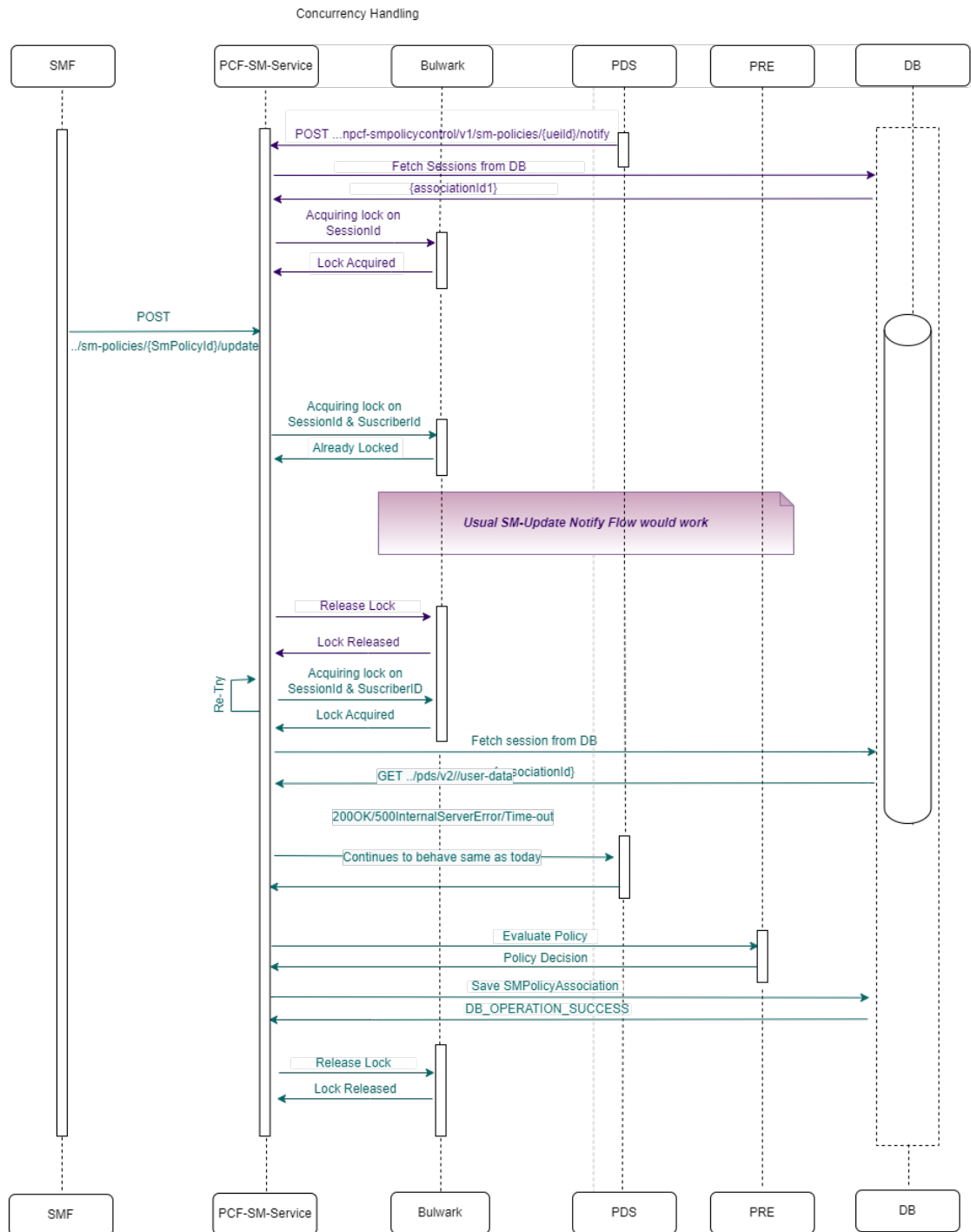
Figure 4-105 Pending transaction and Concurrent SM-Update for same session - Success scenario
