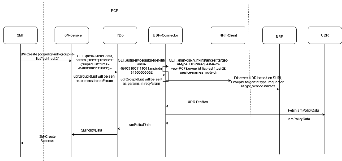
Figure 4-33 SMF sends SM Policy Association Request with oc-policy-udr-group-id
