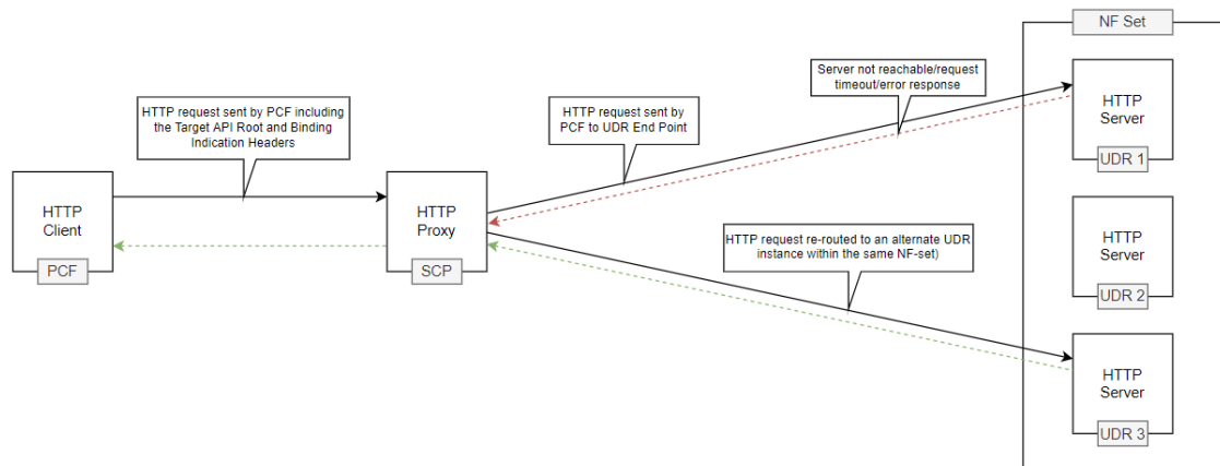
Figure 4-83 Example of NF Set and Binding Header based Indirect Communication
