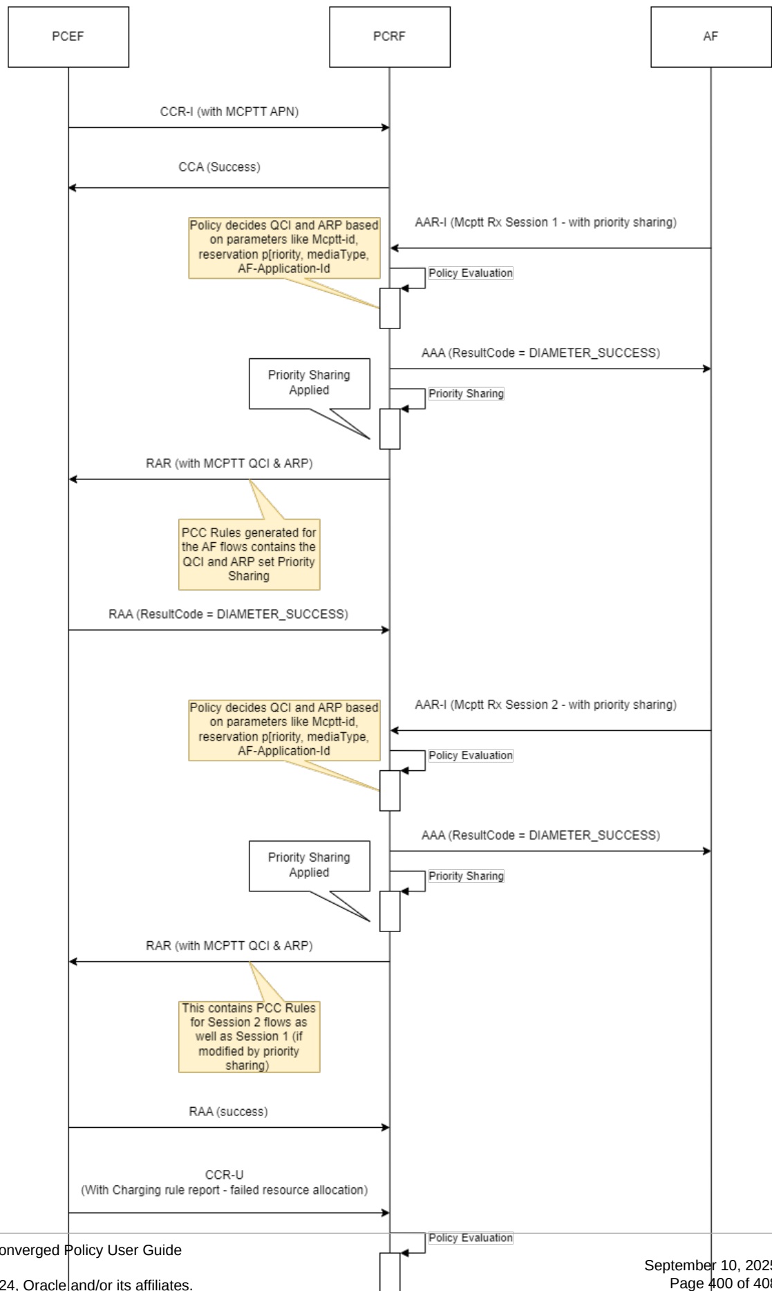
Figure 4-167 Preemption Control - CCRU- CharginRuleReport scenario
