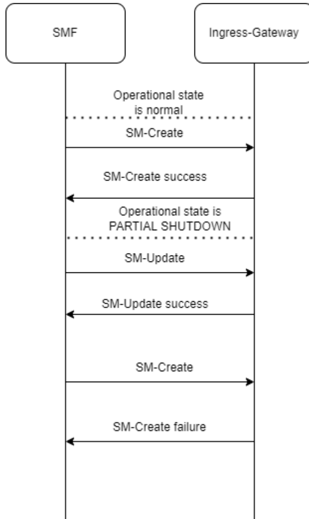
Figure 4-145 Call Flow for Ingress Gateway PARTIAL SHUTDOWN
