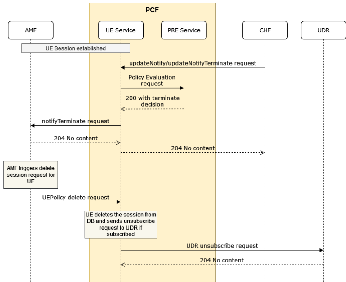
Figure 4-25 Call Flow for UE Terminate for CHF updateNotify or updateNotifyTerminate
