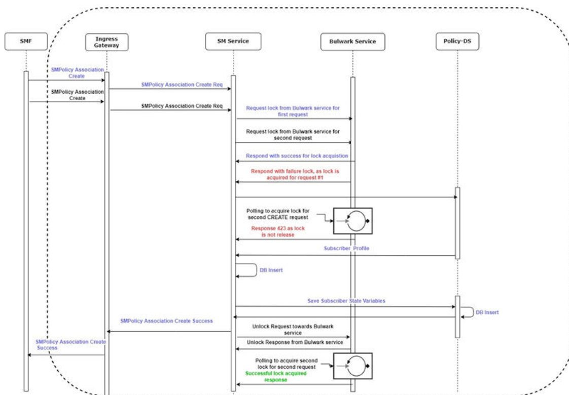
Figure 4-97 Call Flow - Bulwark Lock Request SM Create Procedure
