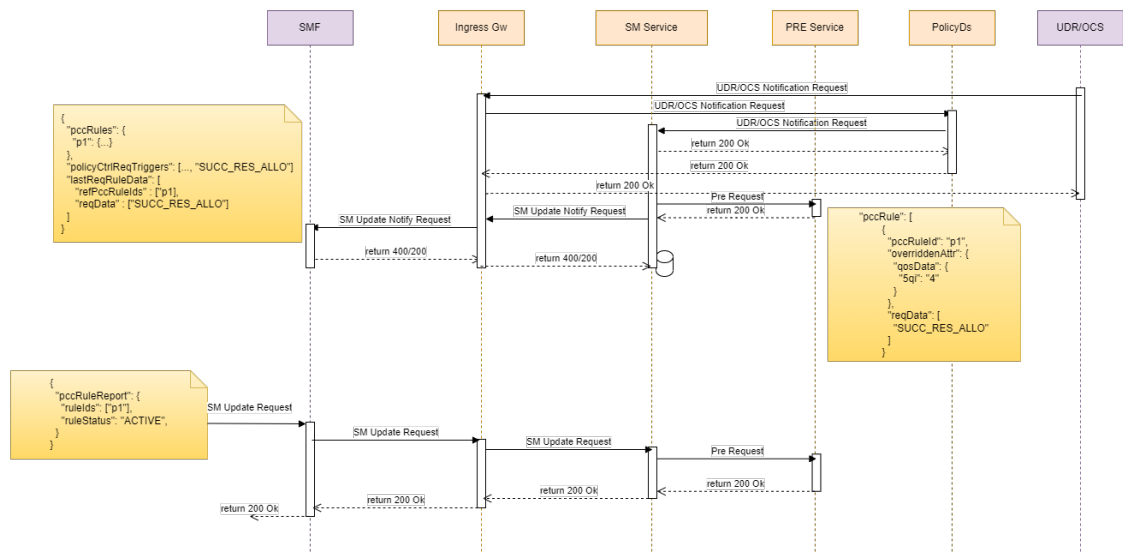
Figure 4-158 PCC Rule in SM-UPDATE-NOTIFY request (Re-authorization)
