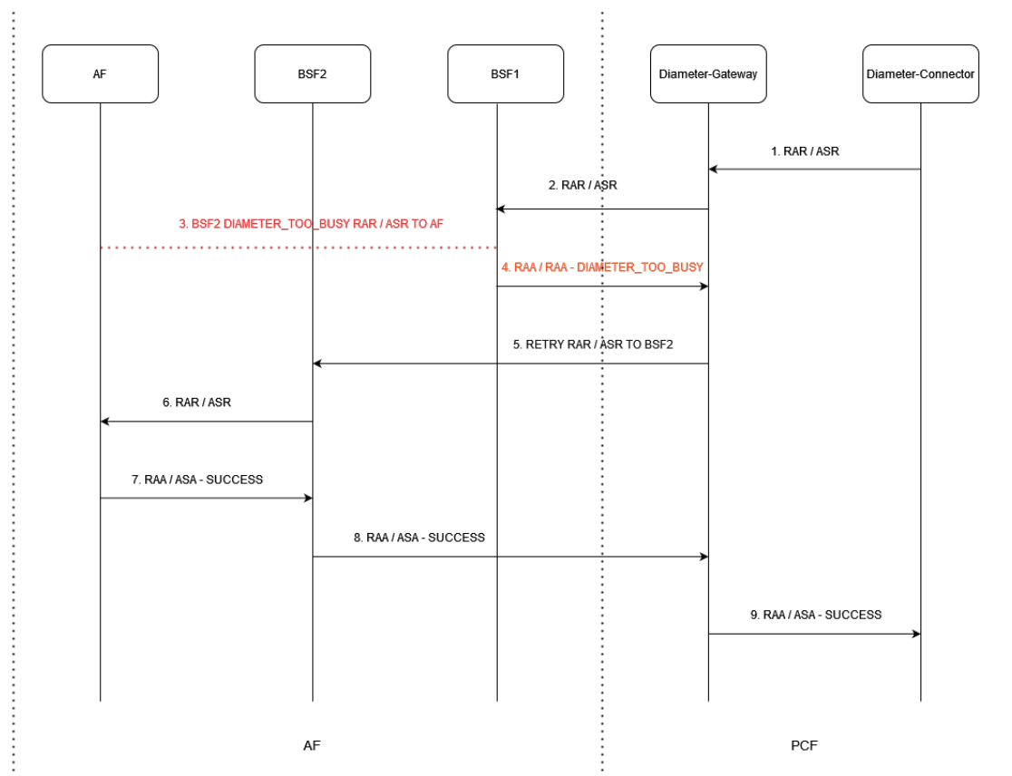
Figure 4-54 RX RAR/RX ASR Retry - Error Originated by Intermediate Peer
