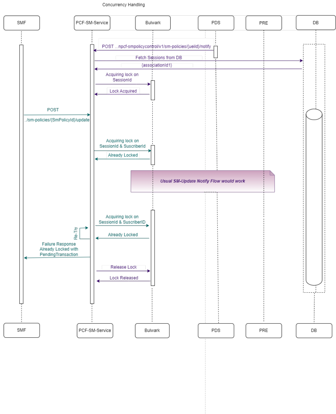
Figure 4-106 Pending transaction and Concurrent SM-Update for same session - Retry failure scenario
