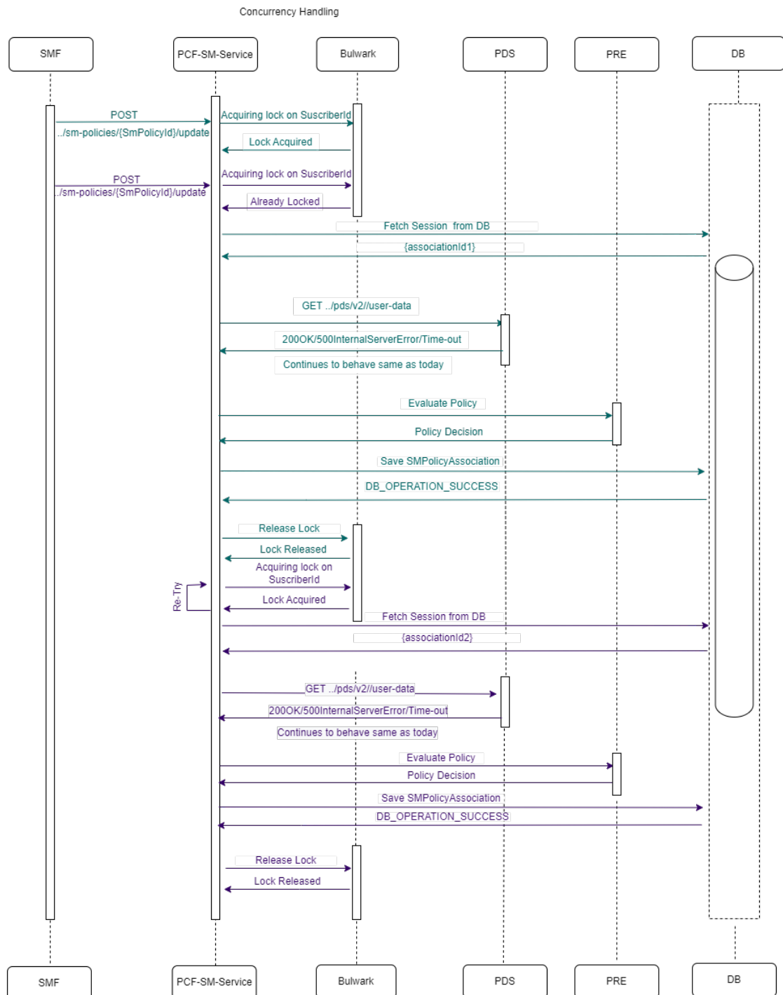
Figure 4-103 Concurrency Enabled for SM-Update and multiple updates for the same subscriber
