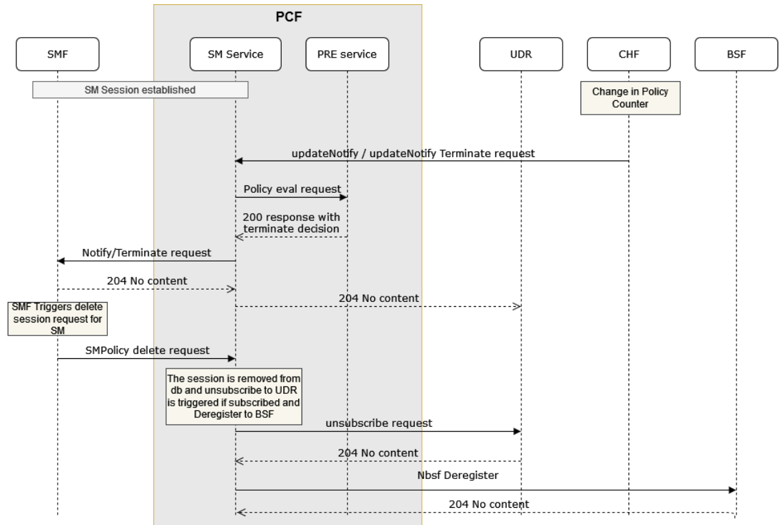
Figure 4-27 Call Flow for AM Terminate for CHF updateNotify or TerminateNotify
