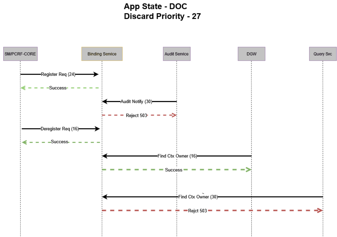
Figure 4-8 Binding Service Pod in DOC State
