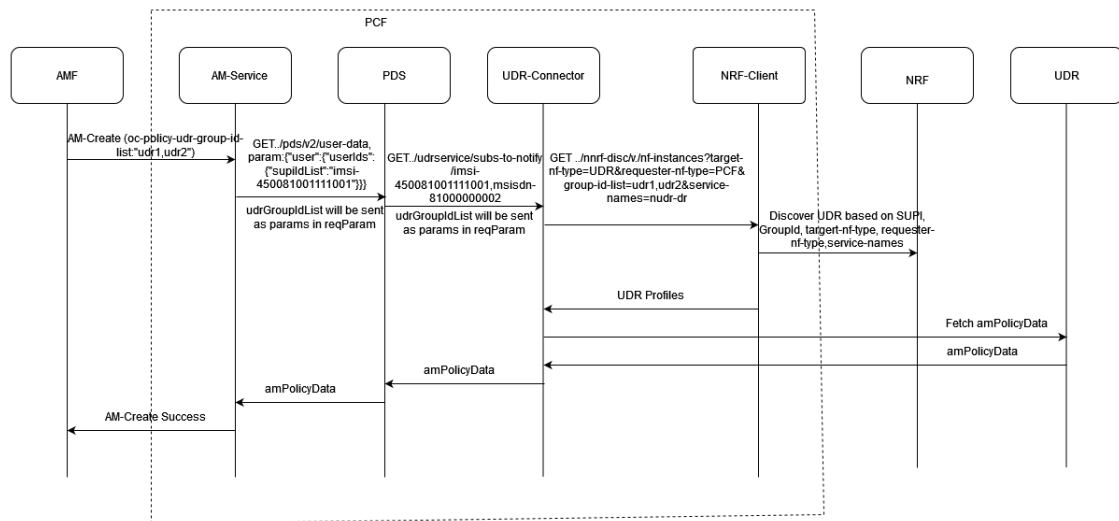
Figure 4-34 AMF sends AM Policy Association Request with oc-policy-udr-group-id
