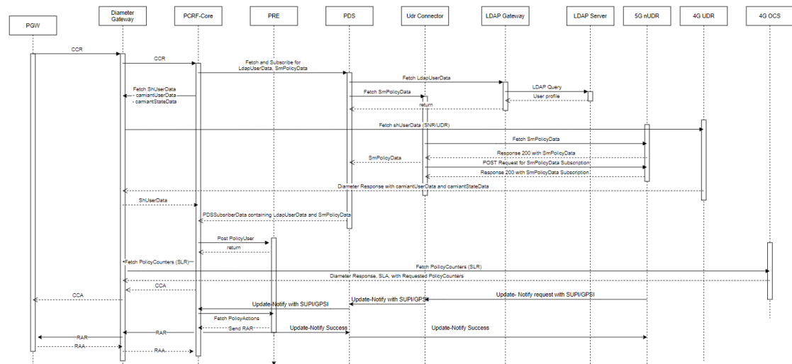
Figure 4-95 Call flow for notification handling from PDS for PCRF-Core
