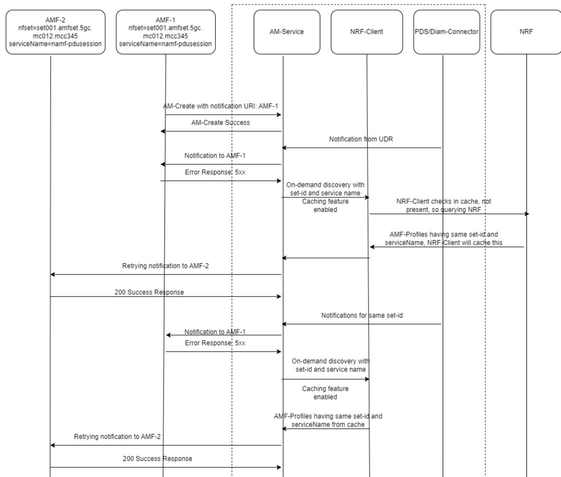
Figure 4-11 AMF Notification for AM Policy (NFSetid based discovery for retry on Notification Request failure)
