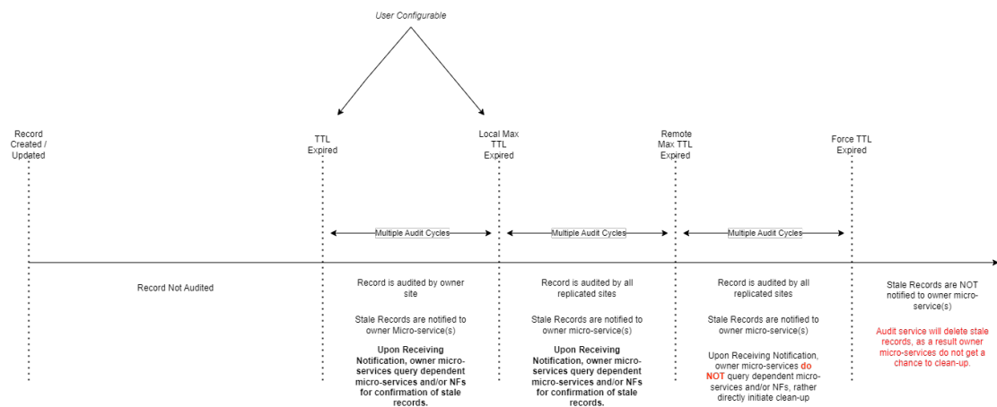
Figure 4-75 Timeline view of Audit Service
