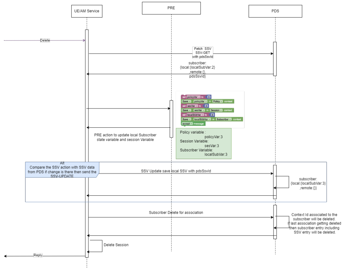
Figure 4-162 State variables in delete session call flow
