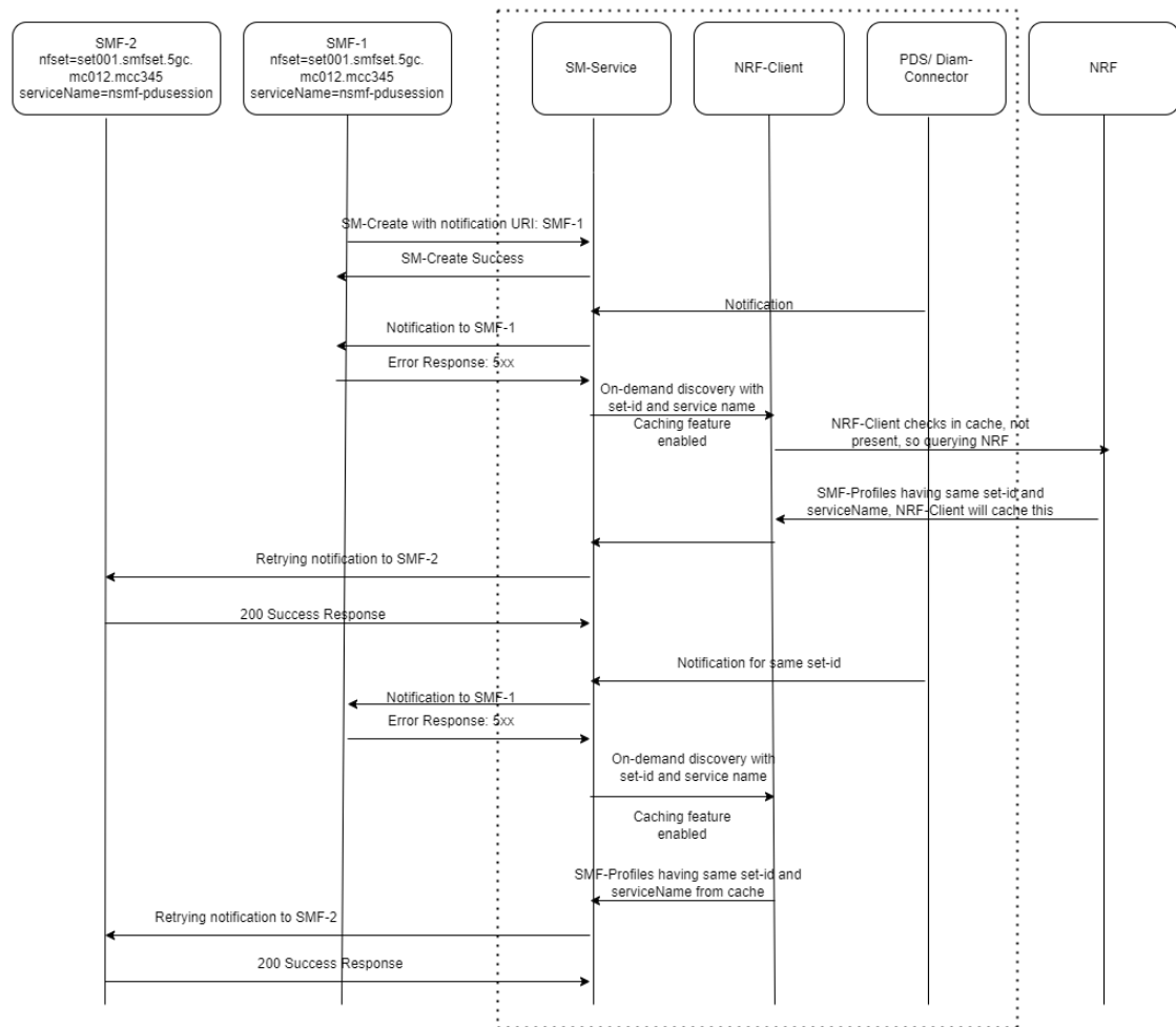
Figure 4-10 SMF Notification for SM Policy (NFSetid based discovery for retry on Notification Request failure)
