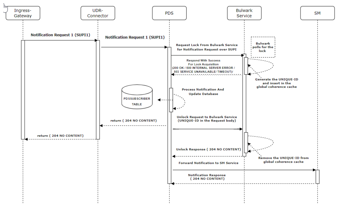
Figure 4-132 Call Flow - Bulwark Lock Request For UDR Notification
