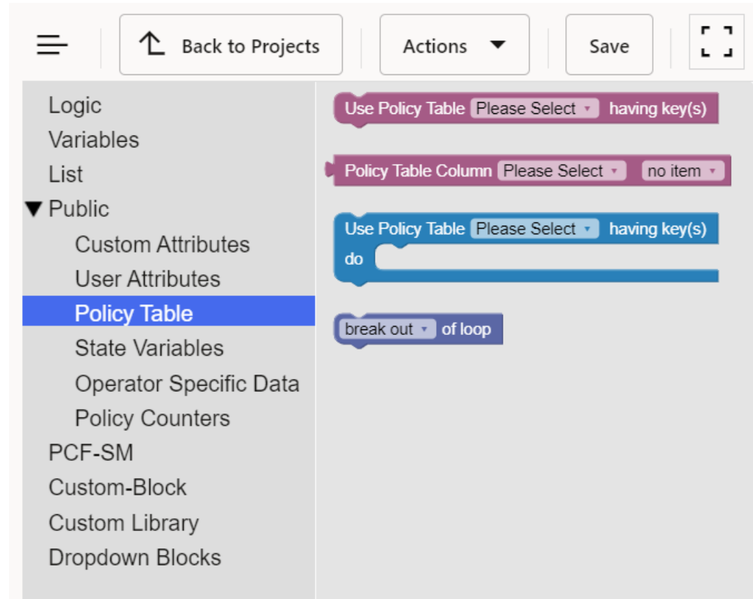
Figure 7-23 Example of Policy Table Blocks for SM Policy
