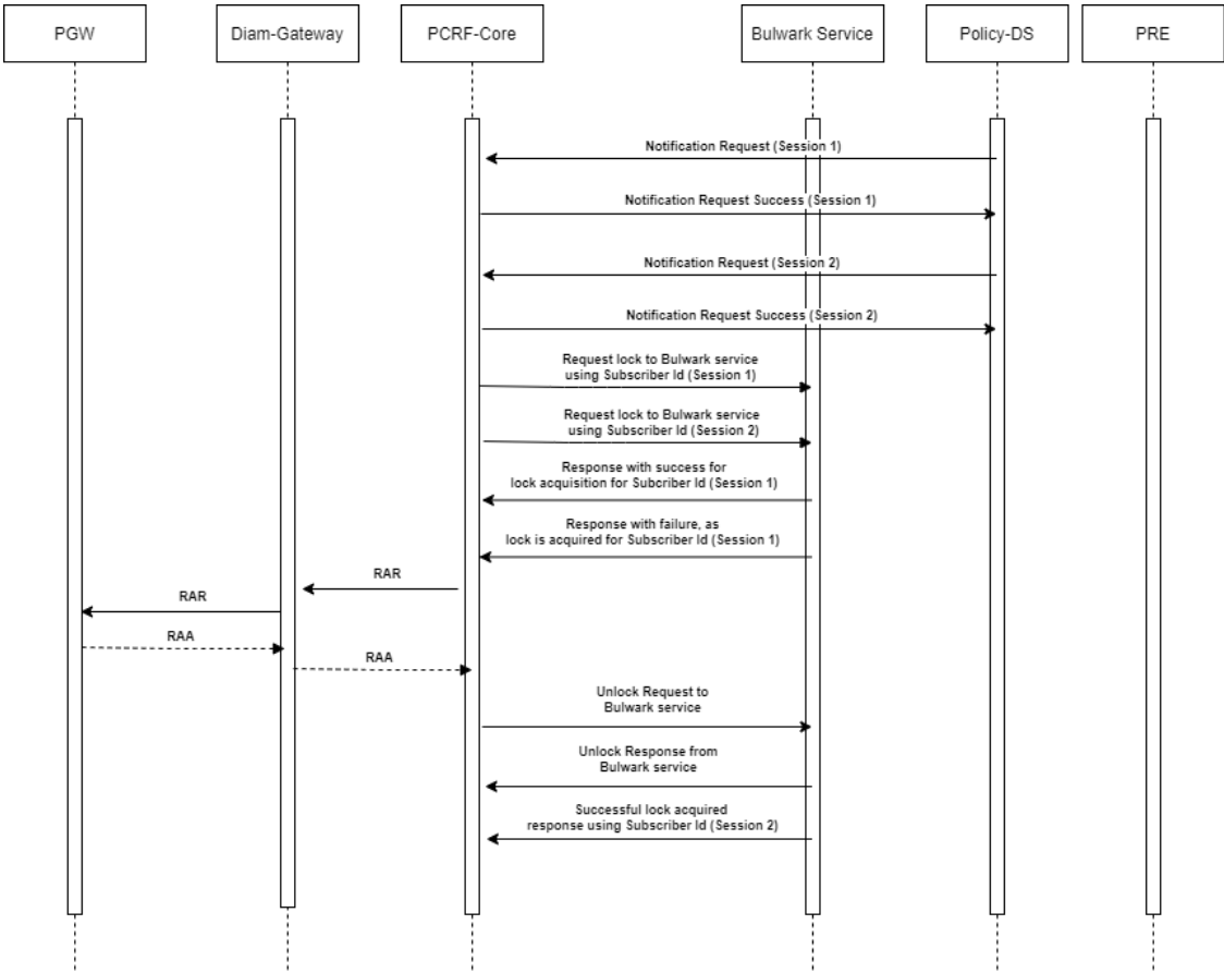
Figure 4-130 Call Flow- PDS notification (RAR) Integration with Bulwark Service
