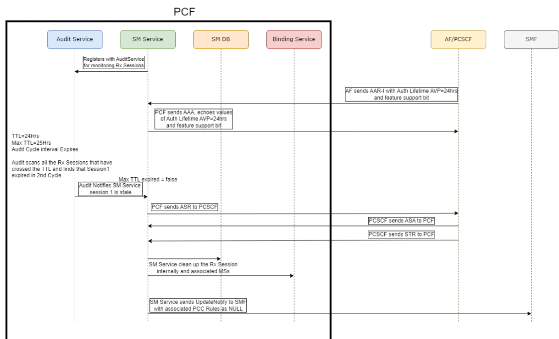
Figure 4-40 Rx Stale Session Detection and Deletion Based on TTL and Authorization-Lifetime
