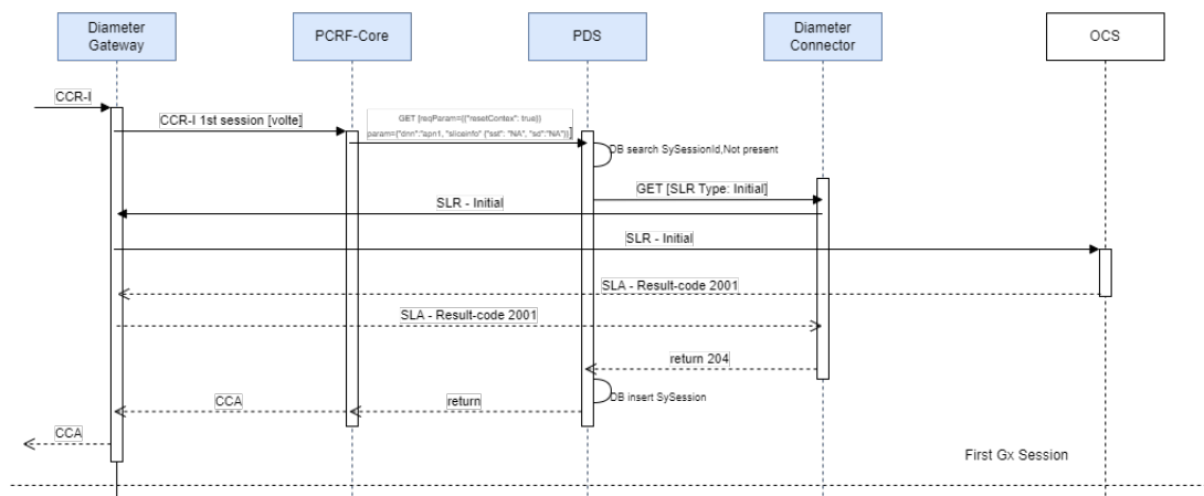
Figure 4-17 First Gx Session
