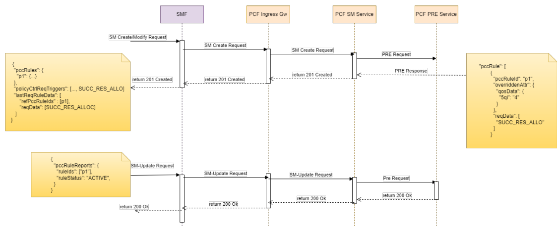
Figure 4-157 PCC Rule for SM Create and SM Update requests
