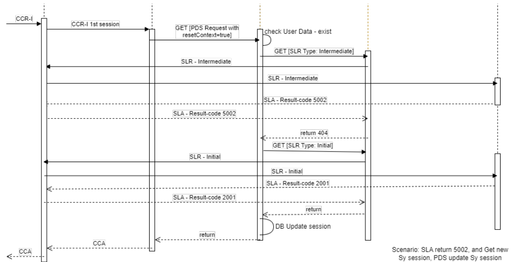
Figure 4-16 SLA Returns 5002, Get New Sy Session, PDS Update Sy Session
