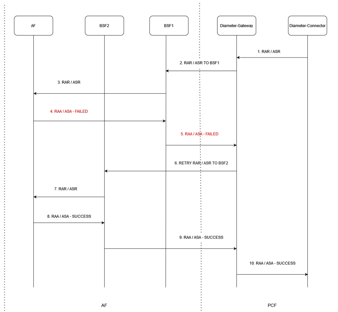
Figure 4-55 RX RAR/RX ASR Retry - Error Originated by Destination Peer (Not Intermediate Peer)
