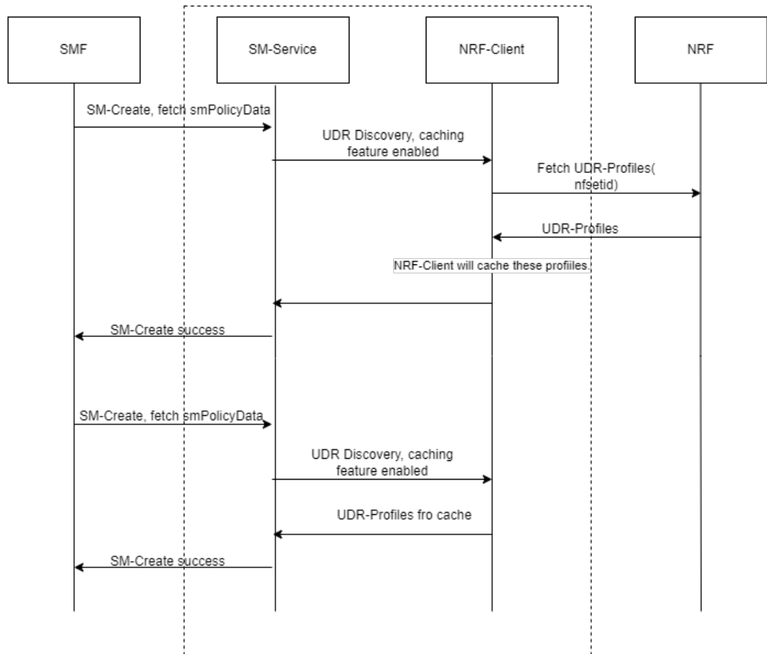
Figure 4-14 Non-SUPI based on-demand discovery caching for User Service
