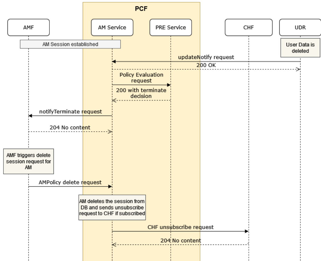
Figure 4-22 Call Flow for AM Terminate for UDR updateNotify with delResources
