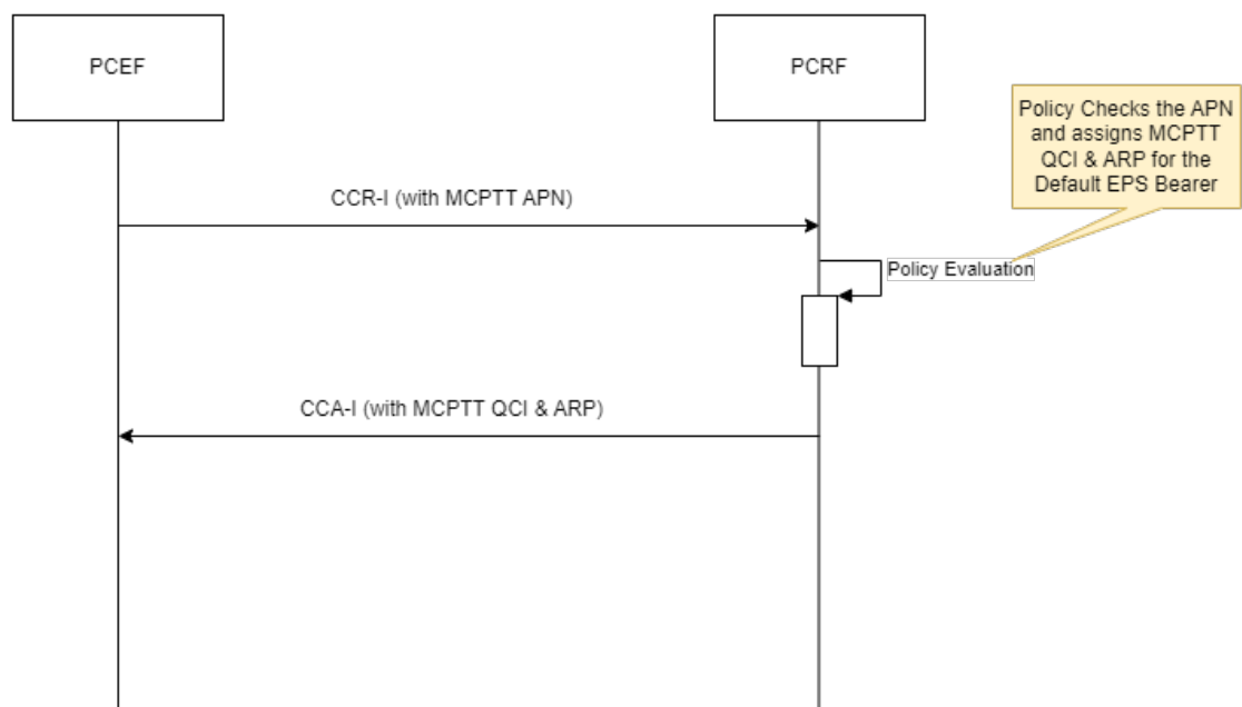
Figure 4-164 MCPTT APN Handling
