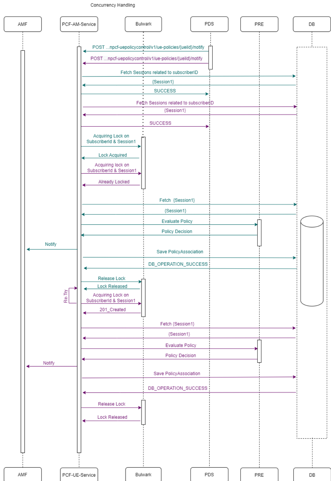
Figure 4-127 Two UENotify requests for same Subscriber each having 1 session
