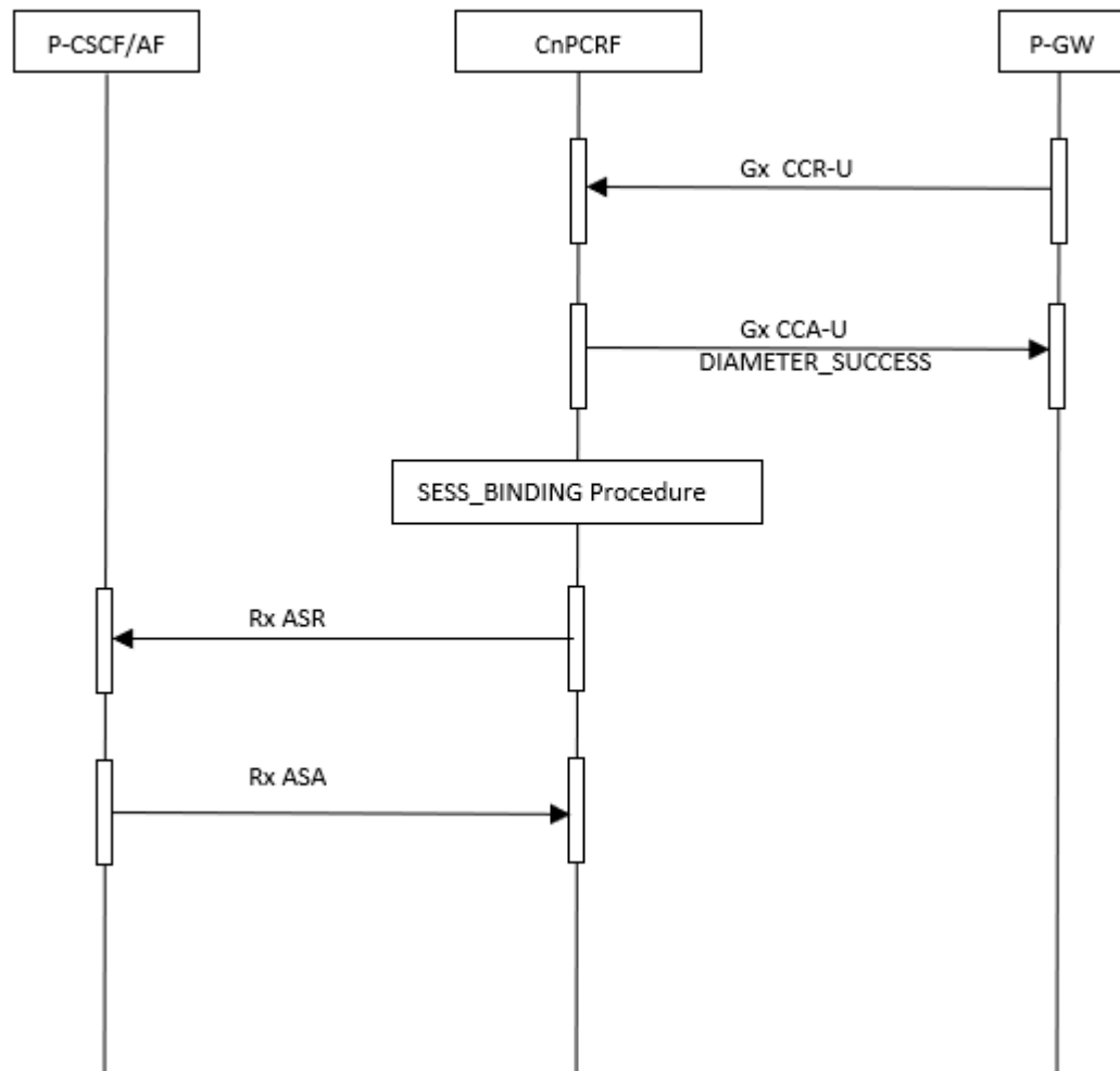
Figure 4-61 Notification of the AF Signaling Transmission in 4G
