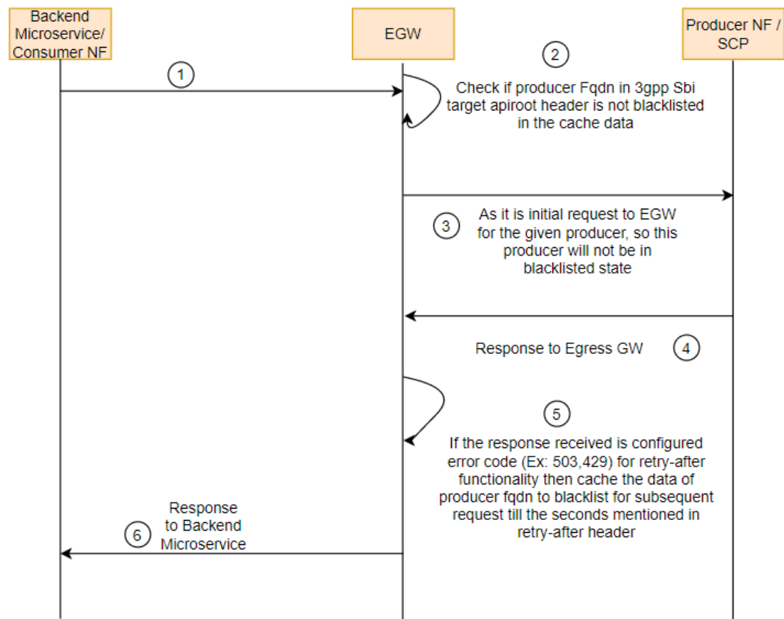
Figure 4-72 Initial Calls for Producer FQDNs
