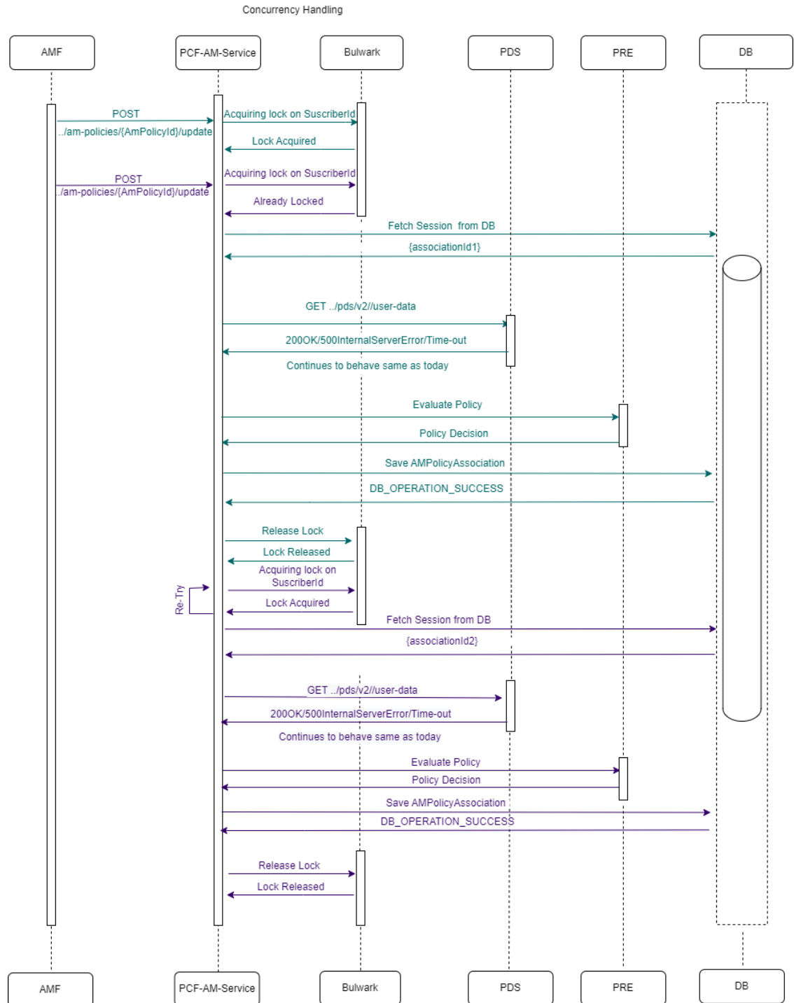
Figure 4-117 Two AM-Update requests for same Subscriber but different Sessions and retry success
