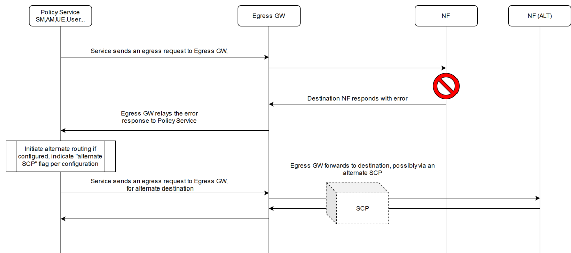
Figure 4-69 Egress Gateway get Error Response
