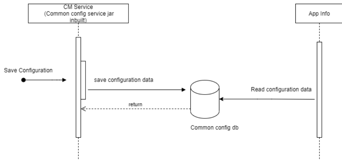
Figure 4-155 Call flow to Save Configuration Data
