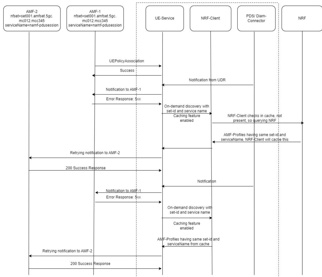
Figure 4-12 AMF Notification for UE Policy (NFSetid based discovery for retry on Notification Request failure)
