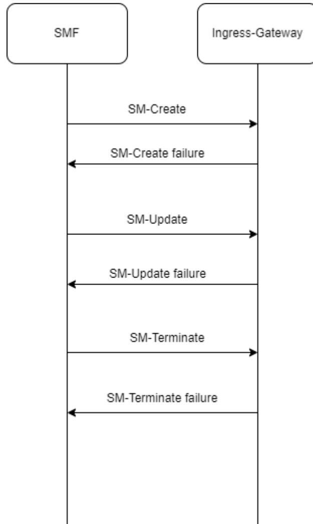
Figure 4-146 Call Flow for Ingress Gateway COMPLETE SHUTDOWN
