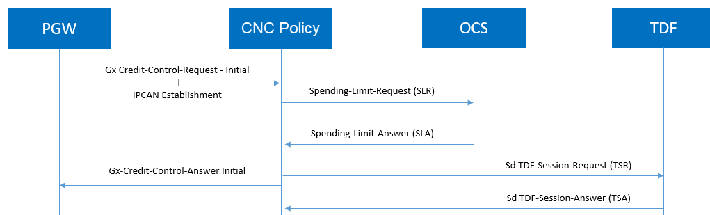
Figure 4-135 Call Flow for TDF Session
