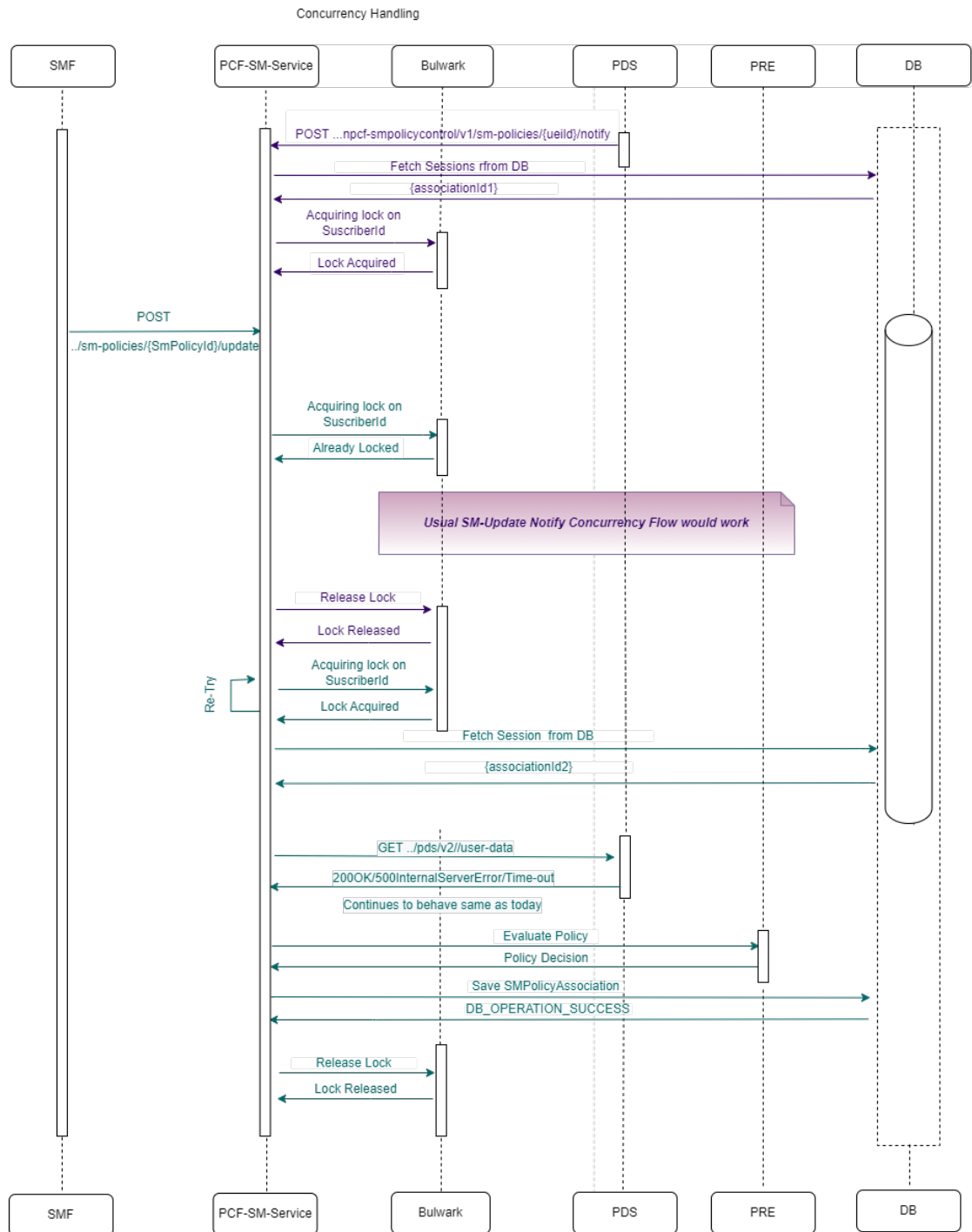
Figure 4-107 Concurrent SM-Update-Notify and Concurrent SM-Update - Success scenario
