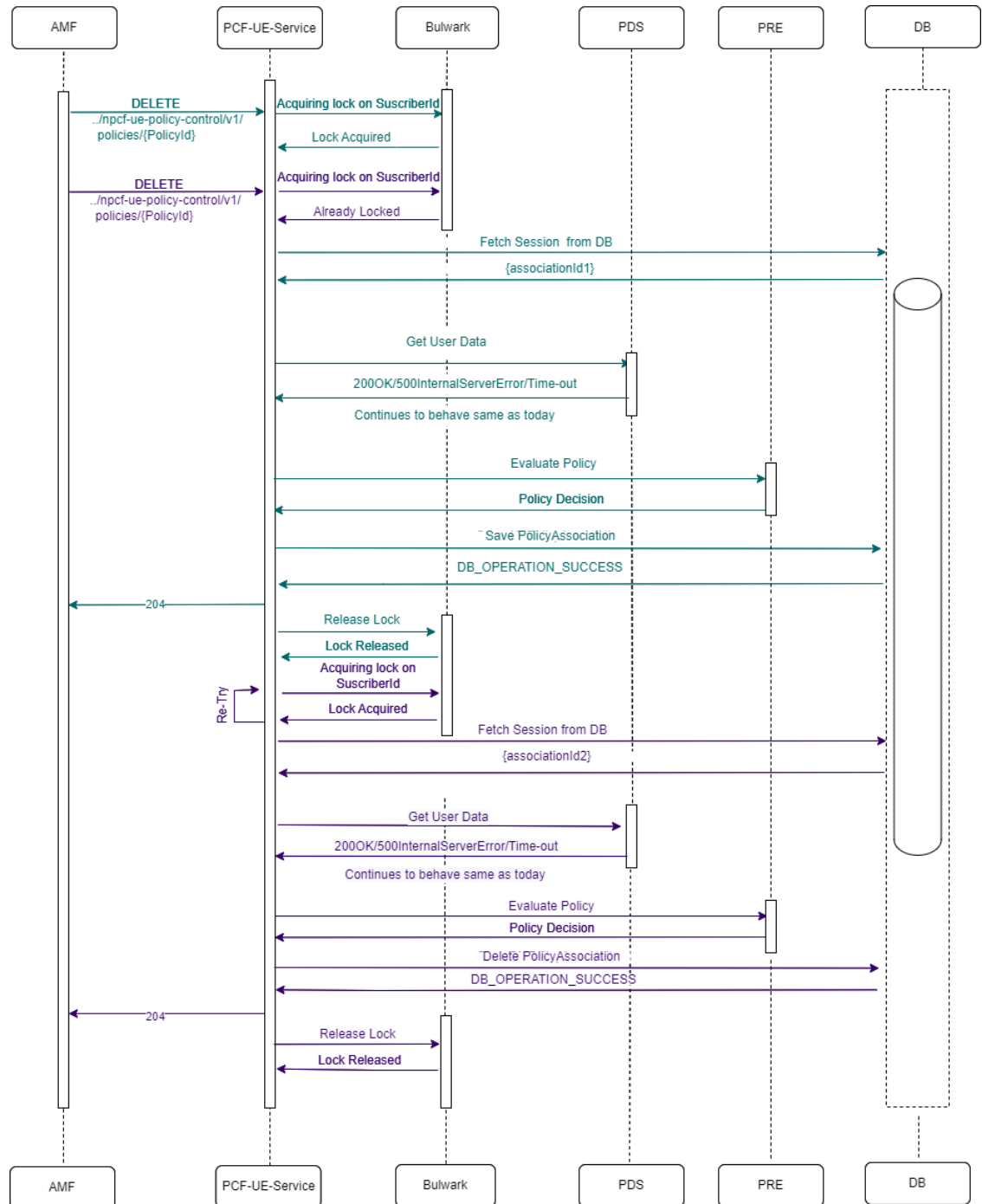
Figure 4-123 Two UE-Delete requests for same Subscriber and retry success.
