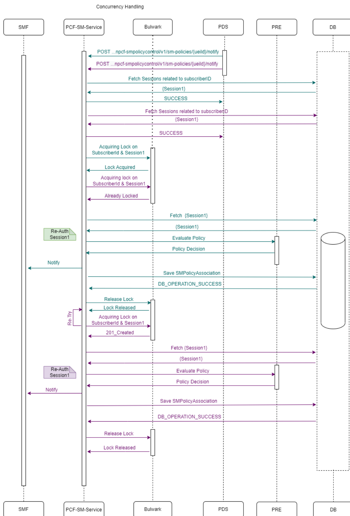
Figure 4-100 Call Flow for SM Update-Notify Request (Two Notifications and 1 Session)
