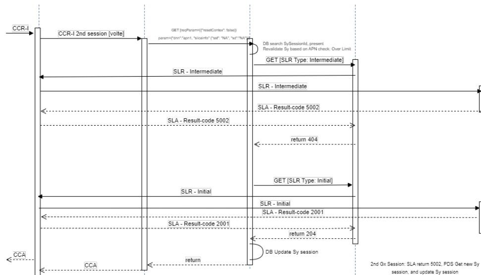
Figure 4-19 Second Gx Session: SLA Returns 5002, Get New Sy Session, PDS Update Sy Session
