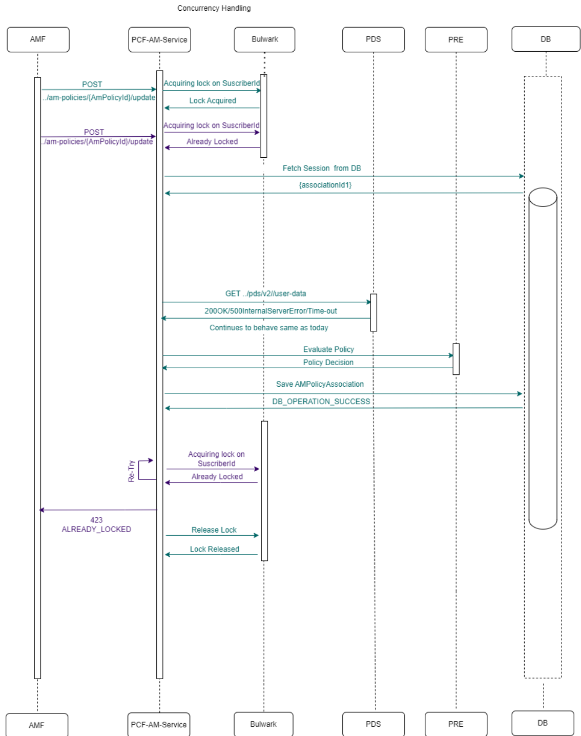
Figure 4-118 Two AM-Update requests for same Subscriber but different Sessions and retry failure (retry =1)
