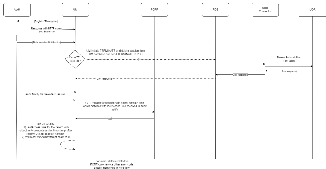
Figure 4-82 Example call flow for Stale Session Detection and Handling in Usage Monitoring Service
