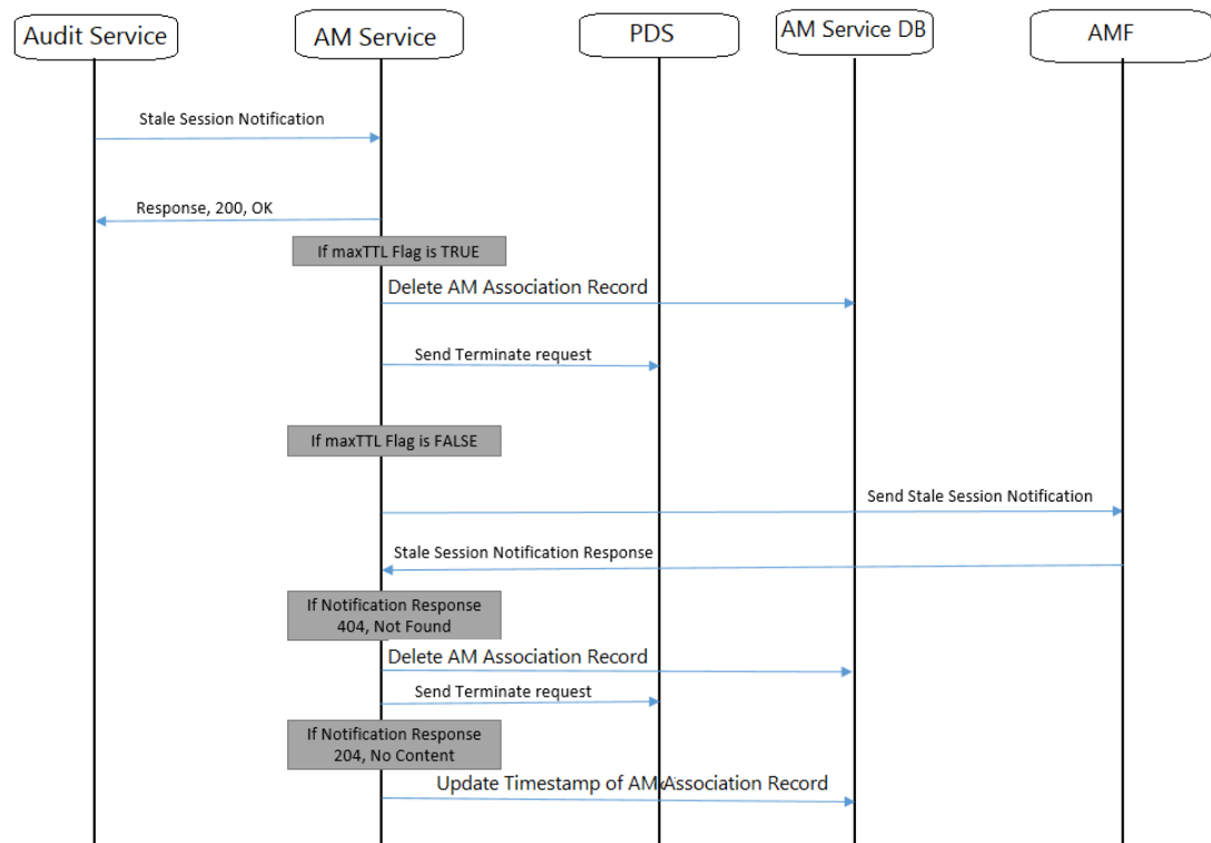
Figure 4-79 Example call flow for Stale Session Detection and Handling in AM Service:
