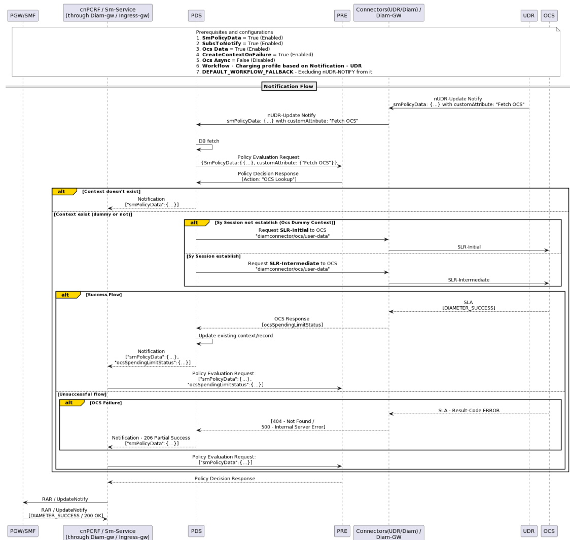
Figure 4-5 UDR PDS Notification Flow
