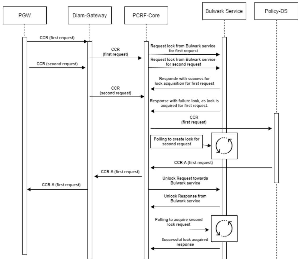
Figure 4-129 CCR-I, CCR-U and CCR-T messages Integration with Bulwark Service
