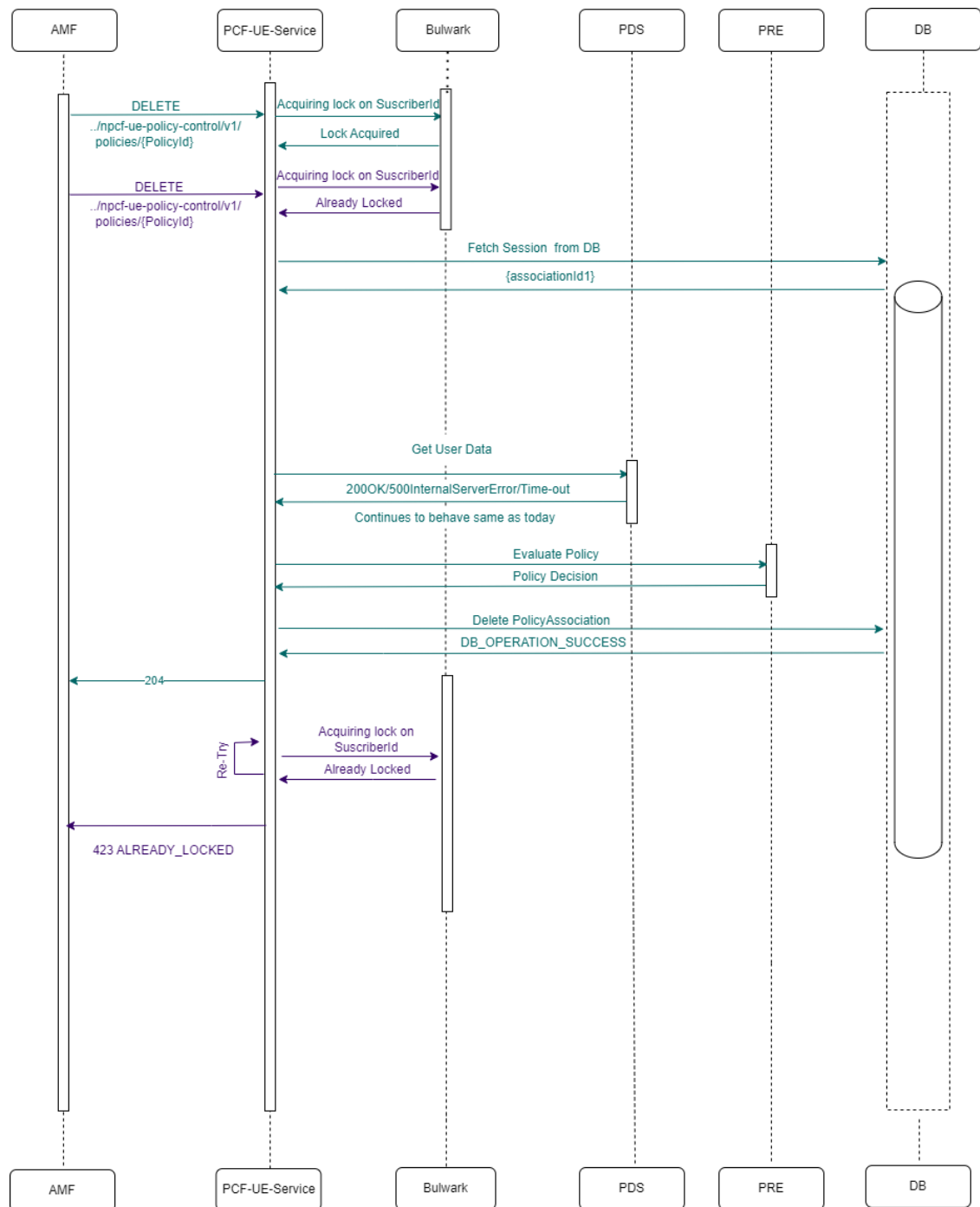
Figure 4-126 Two UE-Update requests for same Subscriber but different Sessions and retry failure (retry =1)
