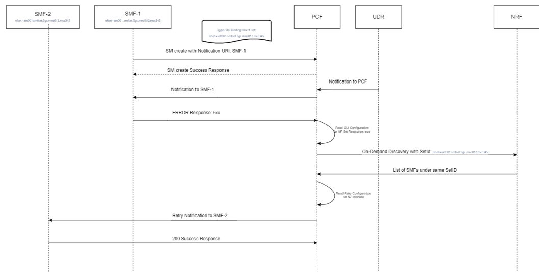
Figure 4-71 On demand NF Discovery is enabled (NF Set Resolution is set to NRF Discovery)
