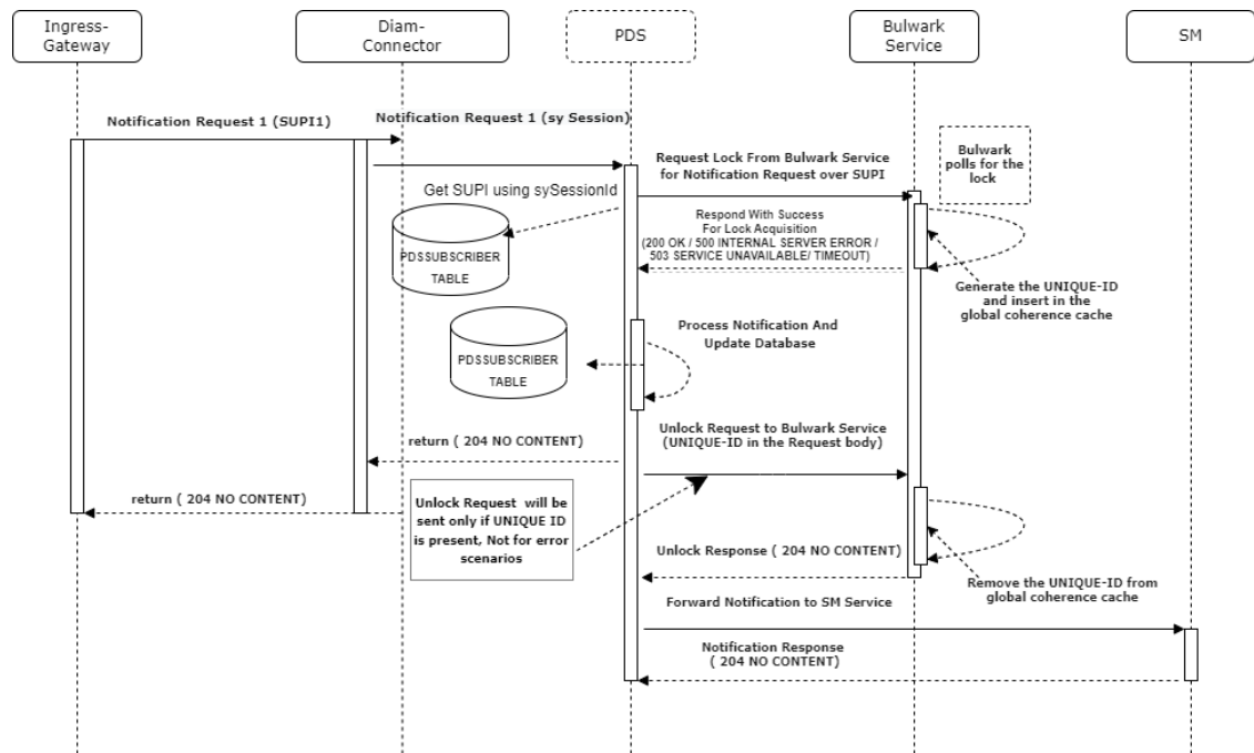
Figure 4-133 Call Flow - Bulwark Lock Request For OCS Notification
