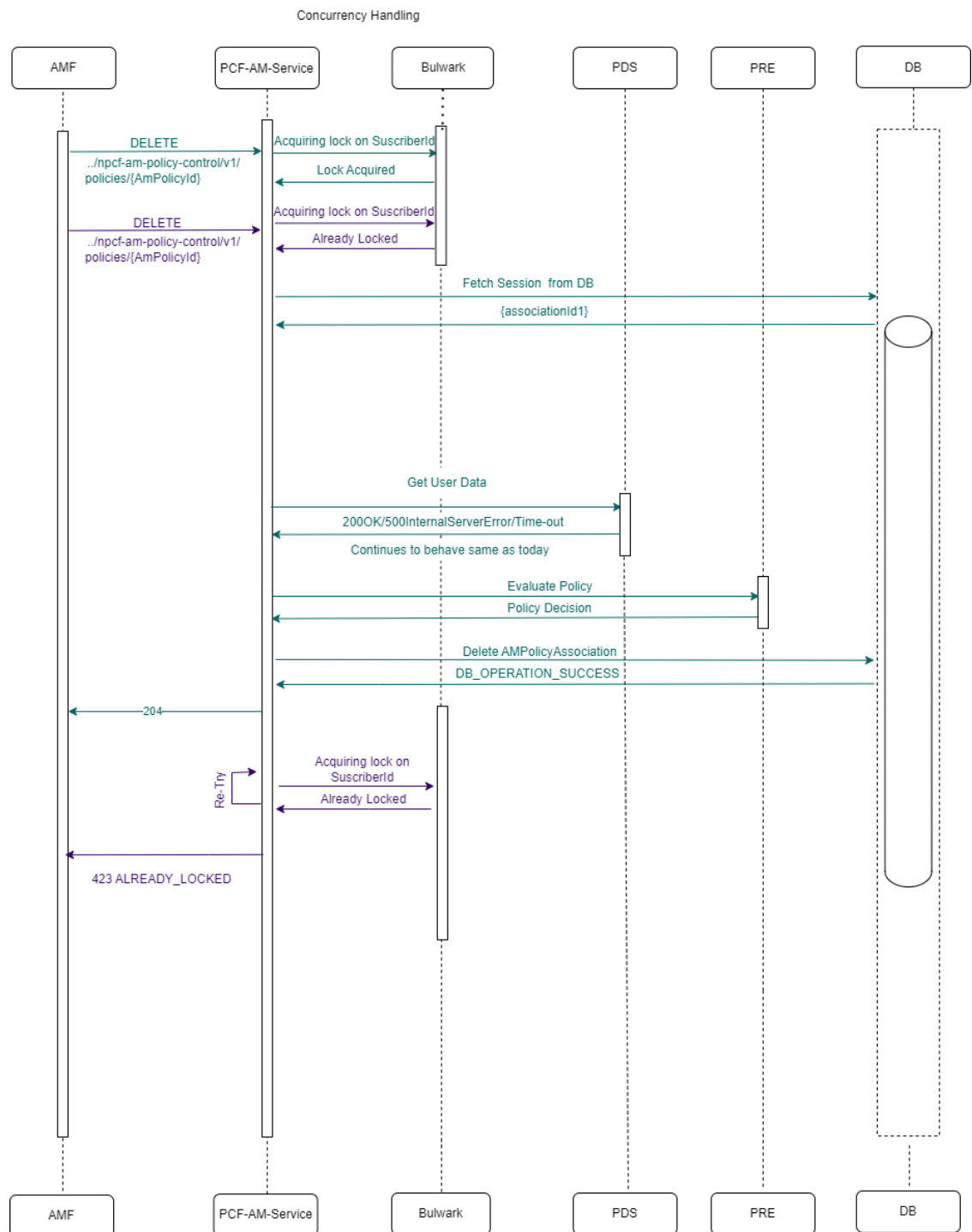
Figure 4-116 Two AM-Delete requests for same Subscriber and retry failure (retry =1)
