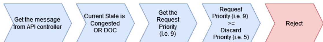
Figure 4-30 Process Flow for Triggering Congestion Control
