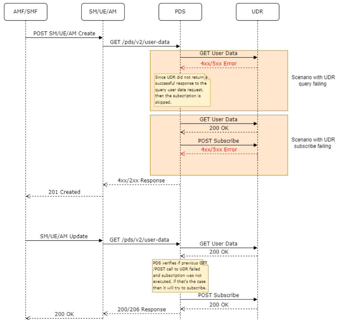
Figure 4-45 Retrieving user data from UDR upon a GET or Update request to a Policy Service
