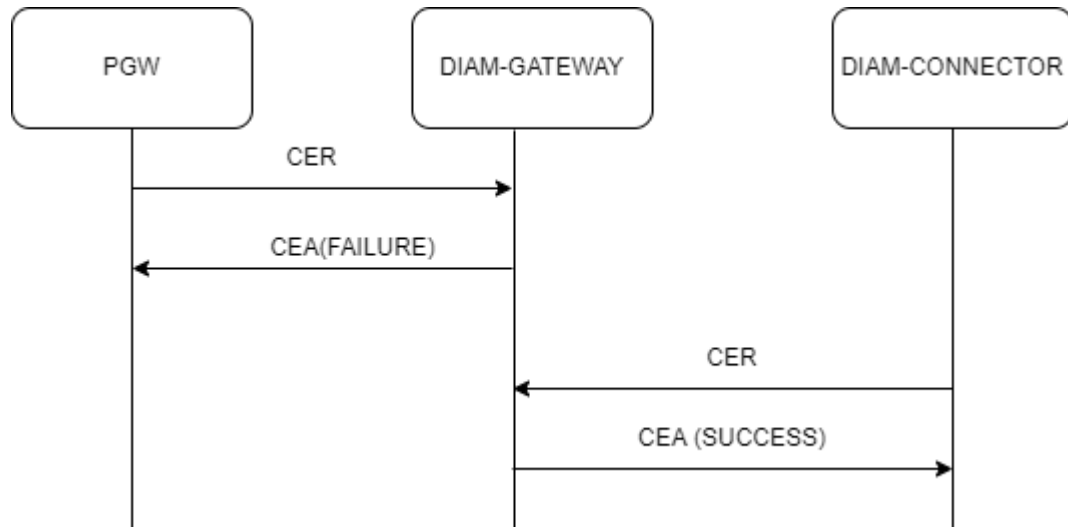
Figure 4-143 Call Flow for Diameter Gateway COMPLETE SHUTDOWN
