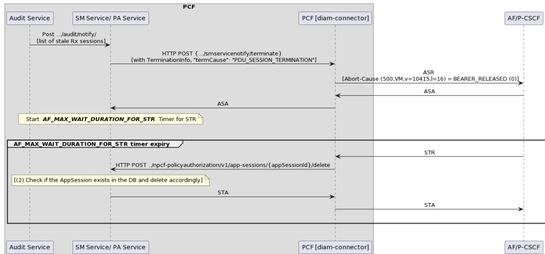
Figure 4-41 Rx session cleanup when Audit service detects a stale session
