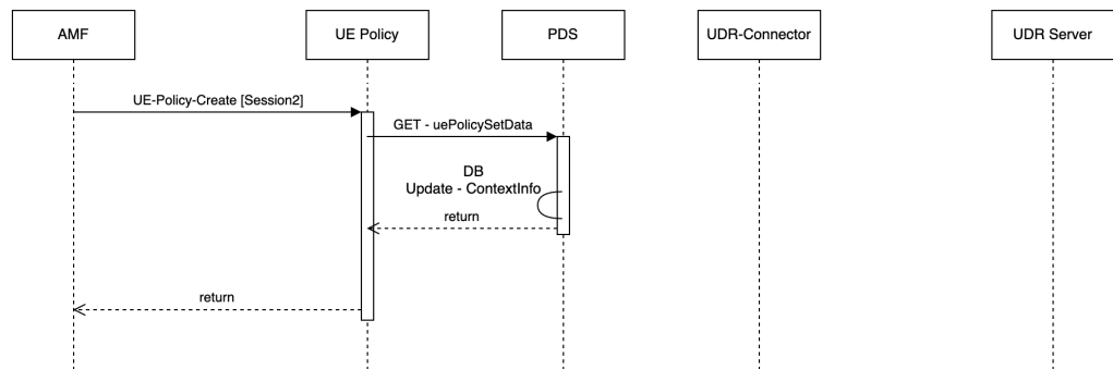
Figure 4-151 resetContextUePolicySetData set to false when there are existing sessions for UE Policy service
