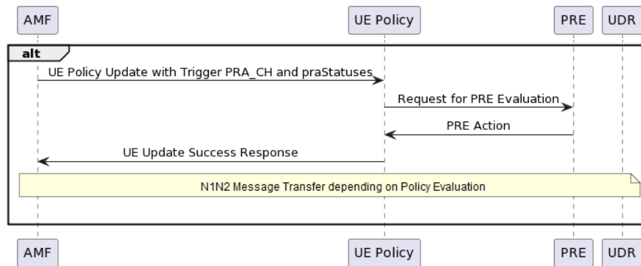
Figure 4-48 UE Policy Association update scenario
