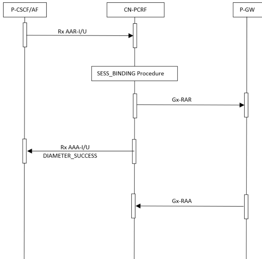
Figure 4-63 Subscription to notification of the AF Signaling Transmission in 4G
