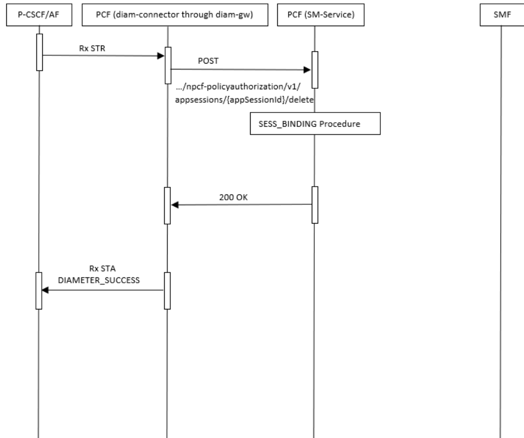
Figure 4-64 Cancellation of subscription to notification of the AF Signaling Transmission in 5G
