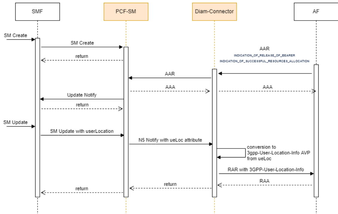
Figure 4-66 3GPP-User-Location-Info Call Flow
