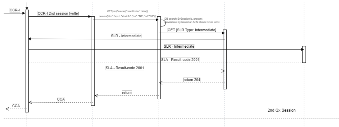
Figure 4-18 Second Gx Session
