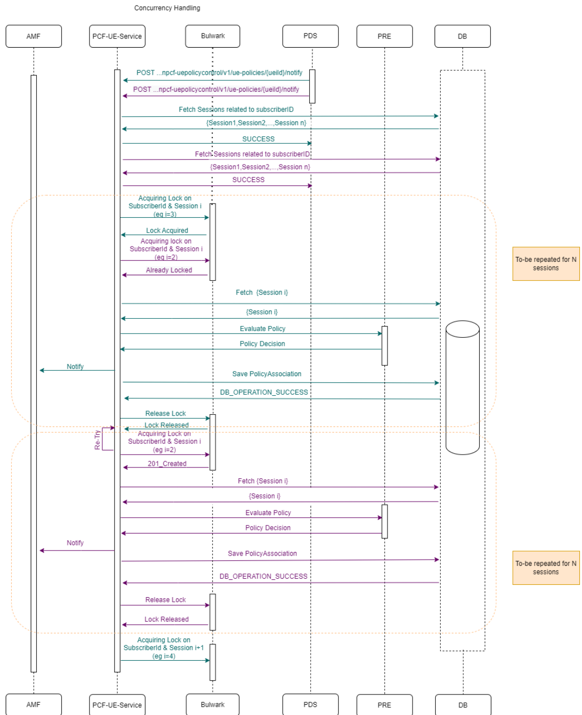
Figure 4-128 Two UENotify request for same Subscriber each having n sessions
