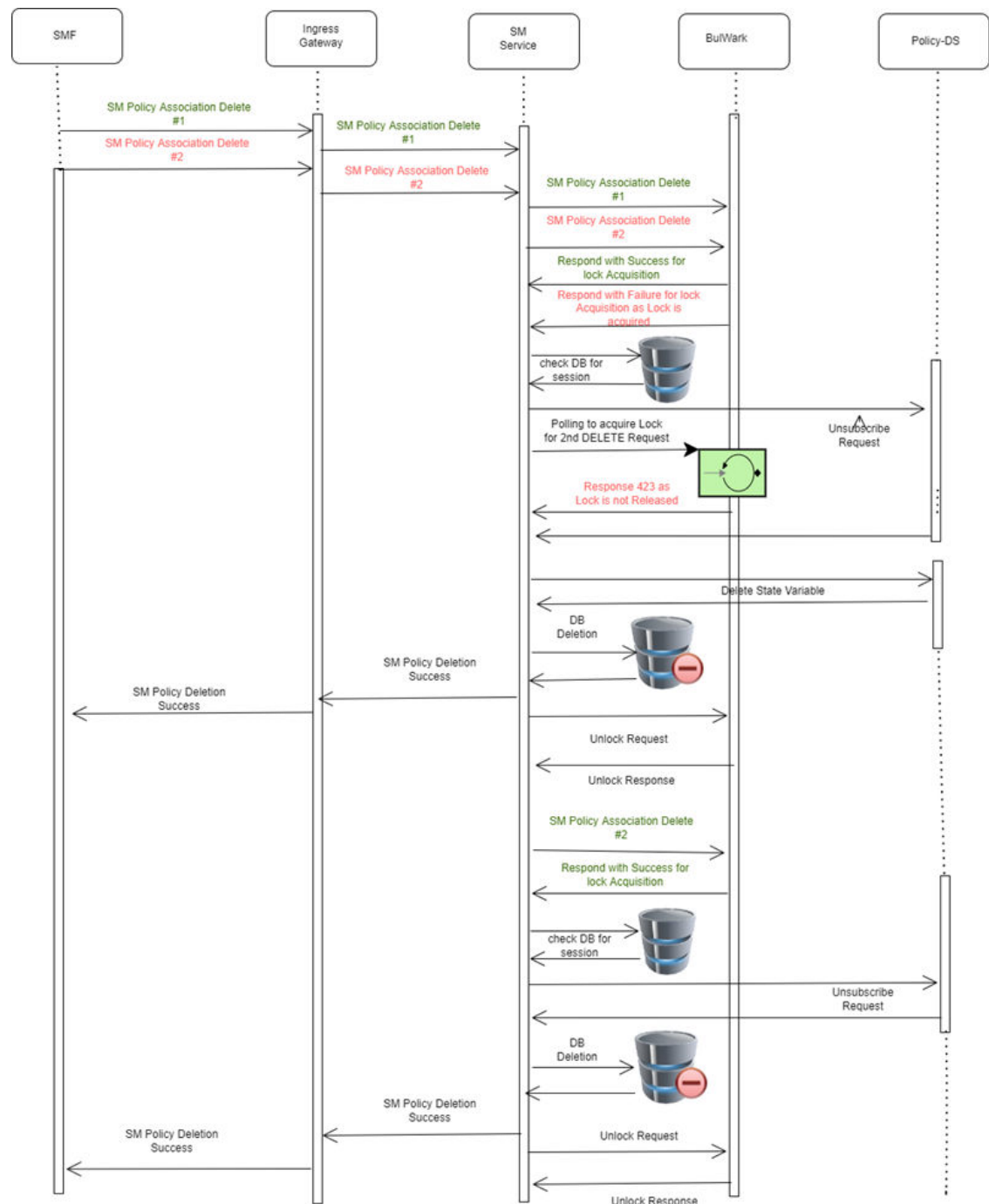
Figure 4-109 Call Flow - Bulwark Lock Request SM Delete Procedure
