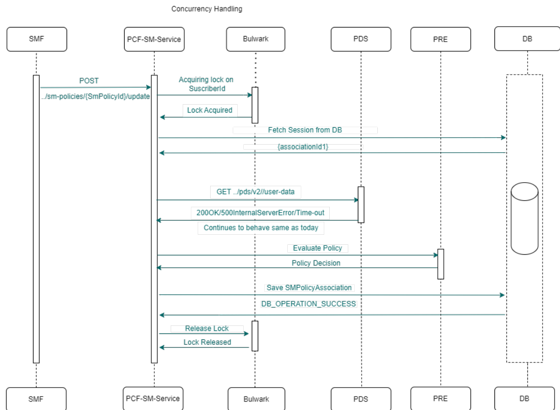
Figure 4-102 Concurrency enabled for SM Update for a single session
