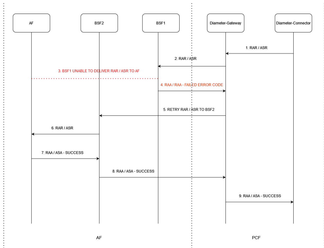
Figure 4-51 Call Flow Rx RAR or Rx ASR one time message retry - Success Case:
