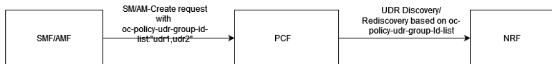
Figure 4-32 UDR Discovery with oc-policy-udr-group-id-list Header to NRF
