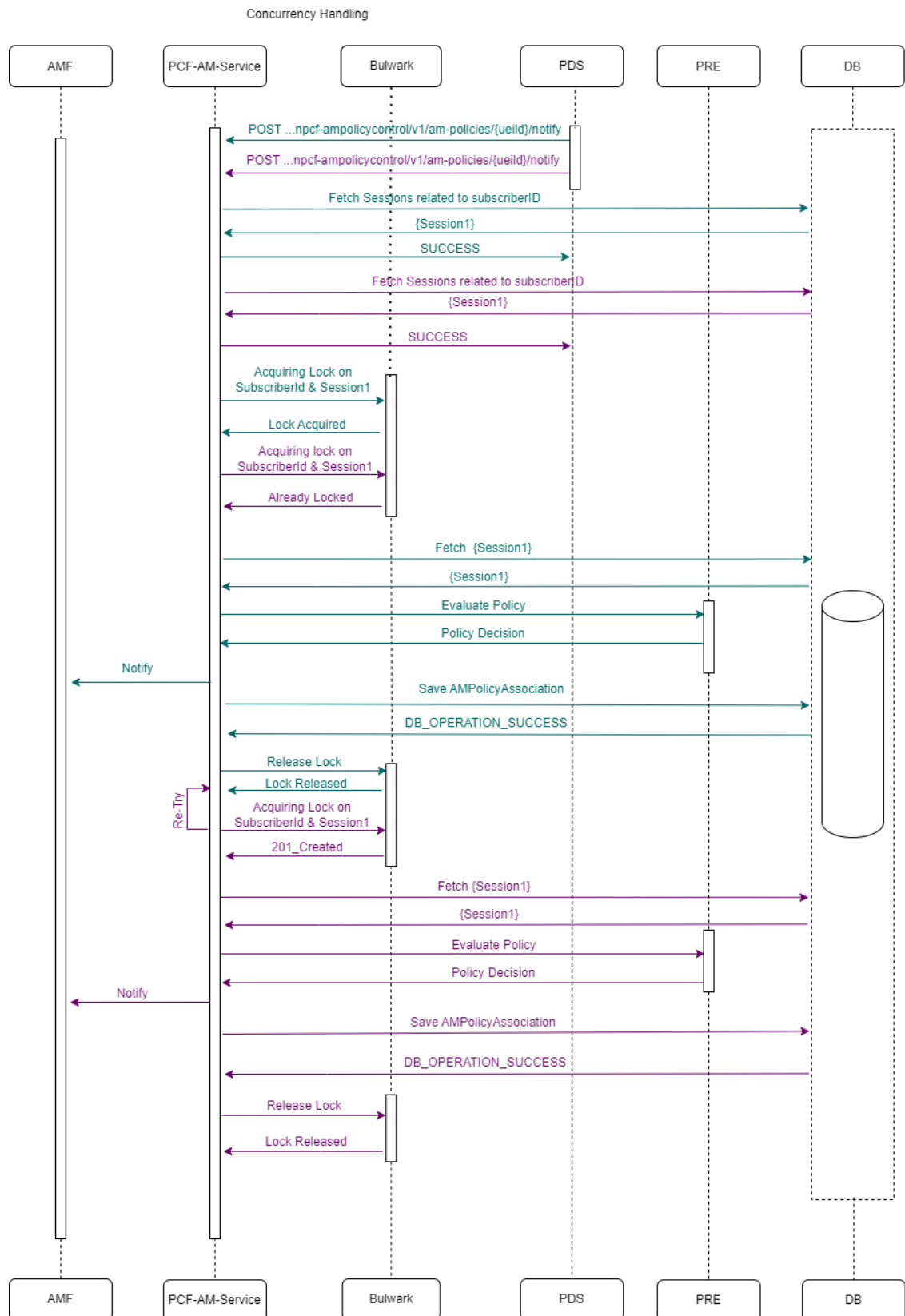
Figure 4-119 Two AM-Notify requests for same Subscriber each having 1 Session
