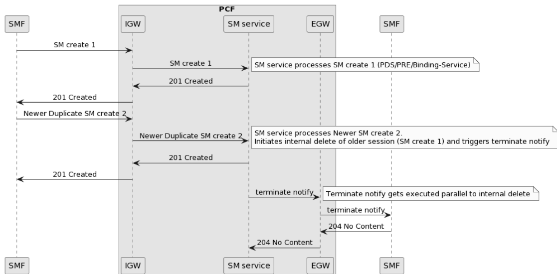
Figure 4-67 Sample call flow for sending Terminate Notify when duplicate session is found (collision detection) and SM service cleans up the older session from database
