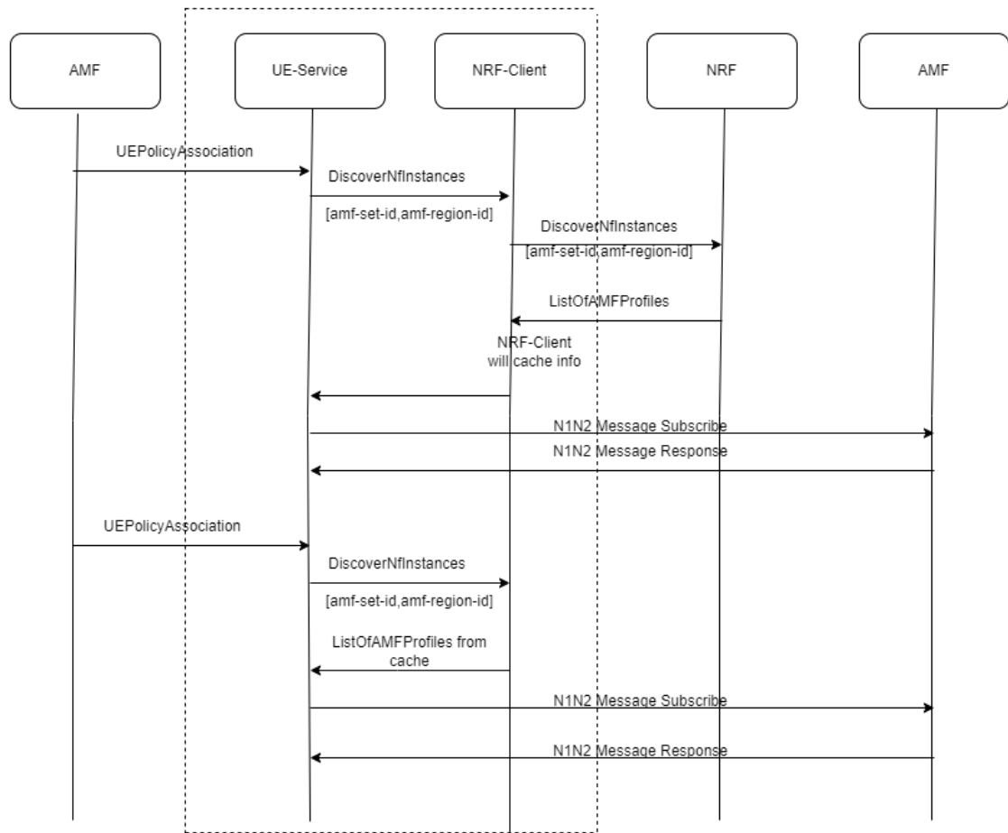
Figure 4-13 AMF Discovery/ Re-Discovery
