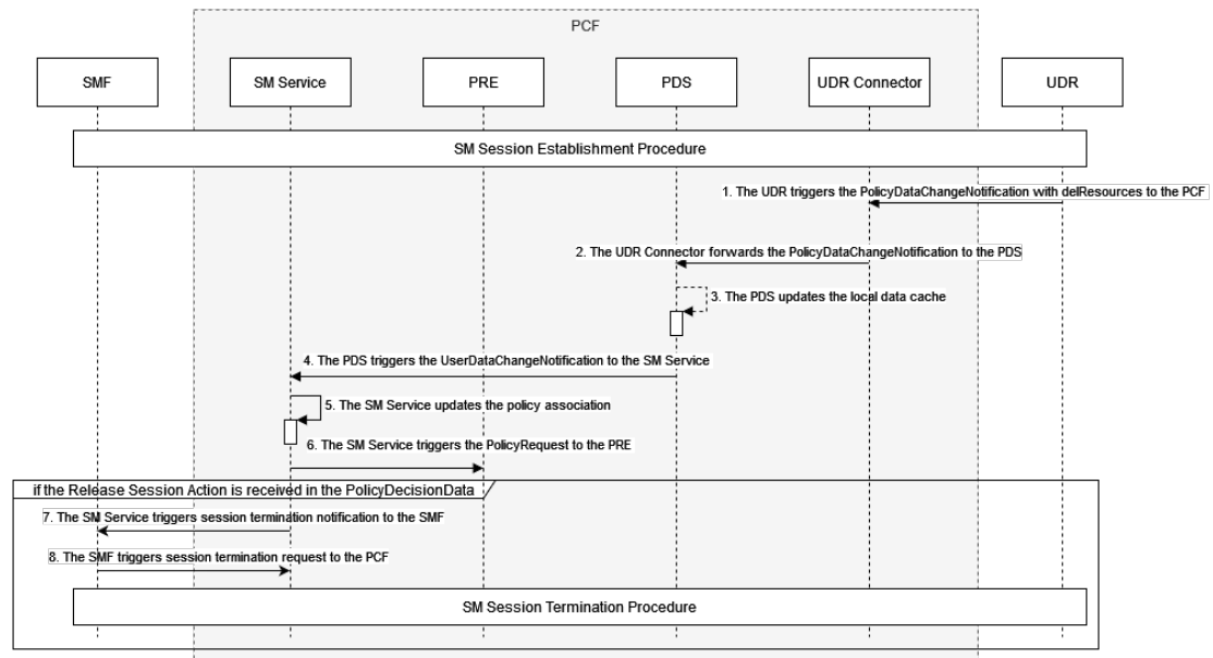
Figure 4-26 Call Flow for SM Terminate for UDR updateNotify with delResources
