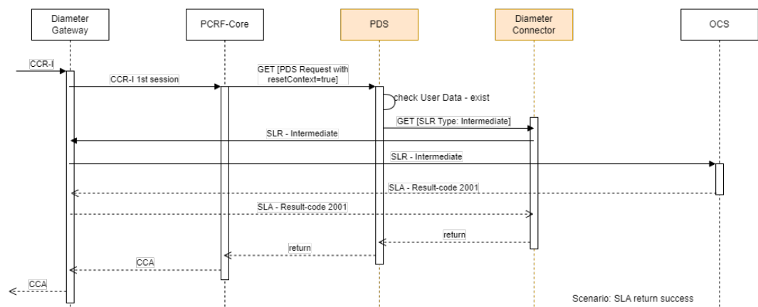
Figure 4-15 SLA Returns Success
