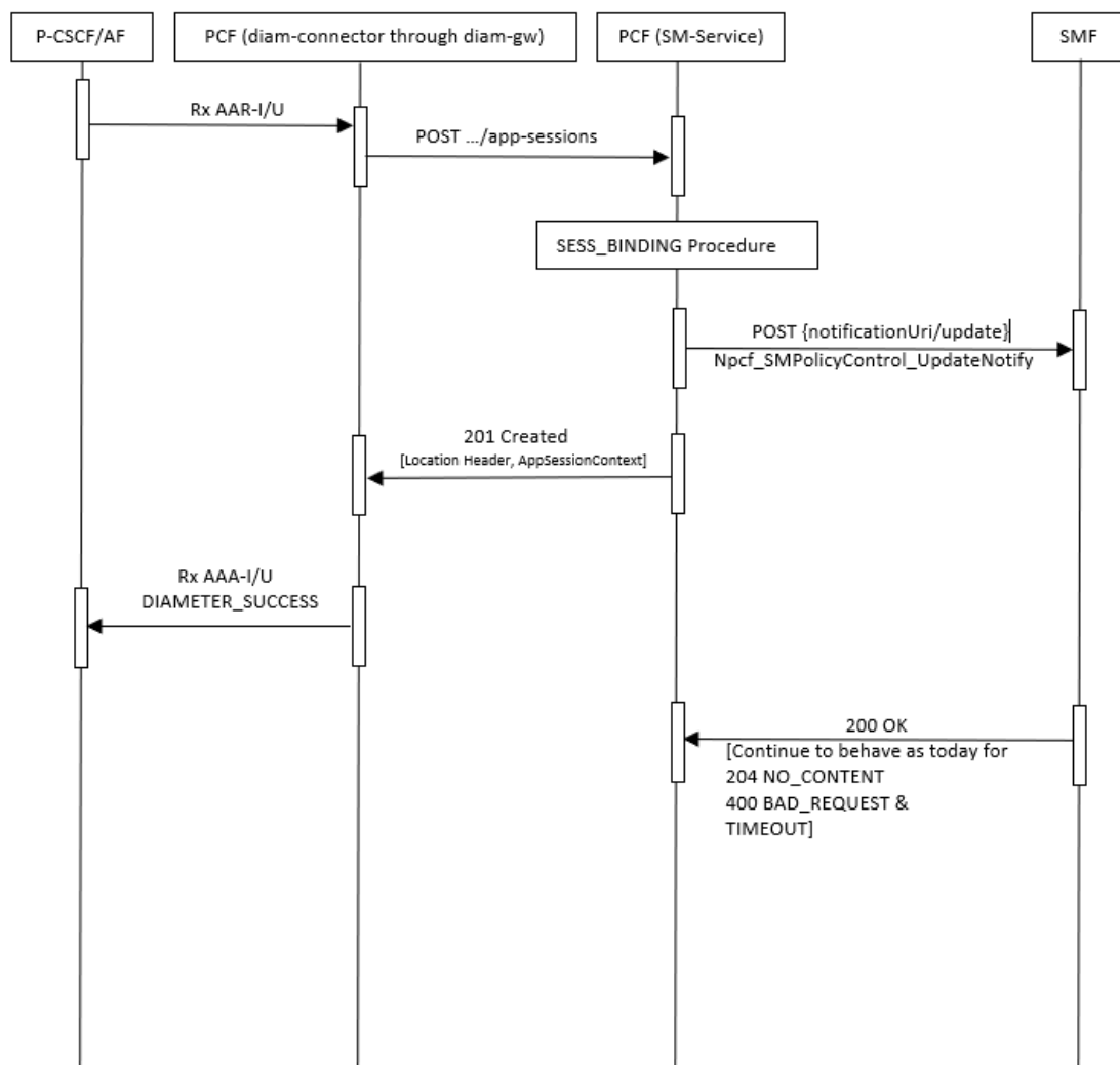
Figure 4-62 Subscription to notification of the AF Signaling Transmission in 5G
