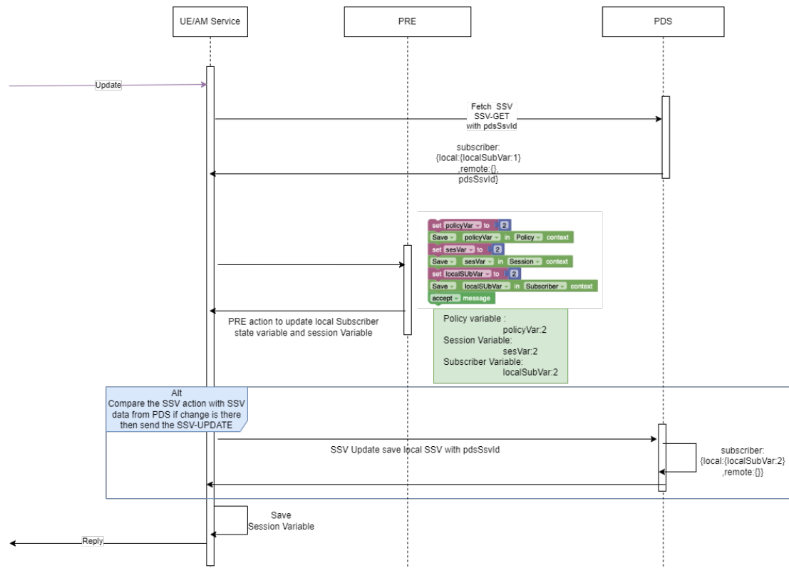
Figure 4-161 State variables in update session call flow
