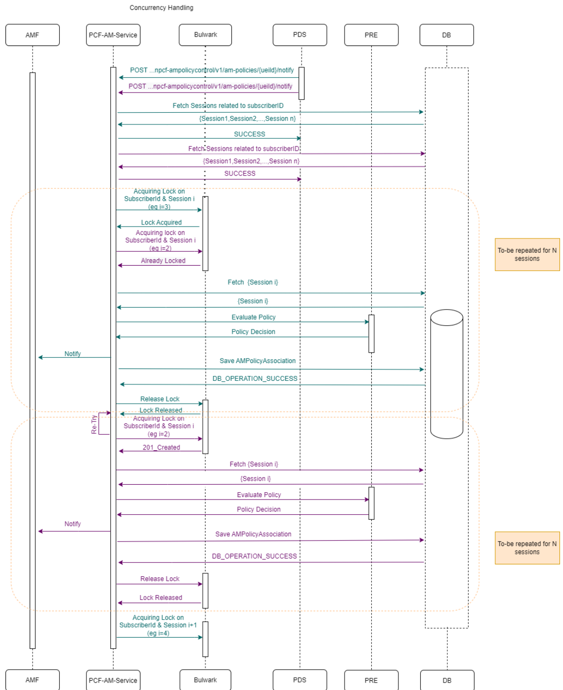
Figure 4-120 Two AM-Notify request for same Subscriber each having n Sessions
