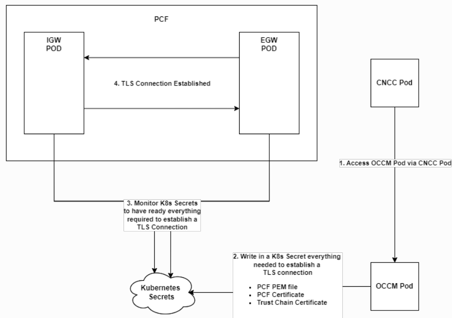
Figure 4-2 Policy Integration with OCCM
