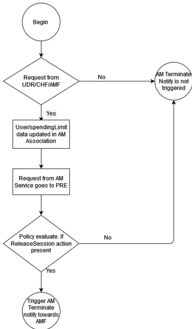
Figure 4-20 PCF Triggering AM UpdateNotify Terminate
