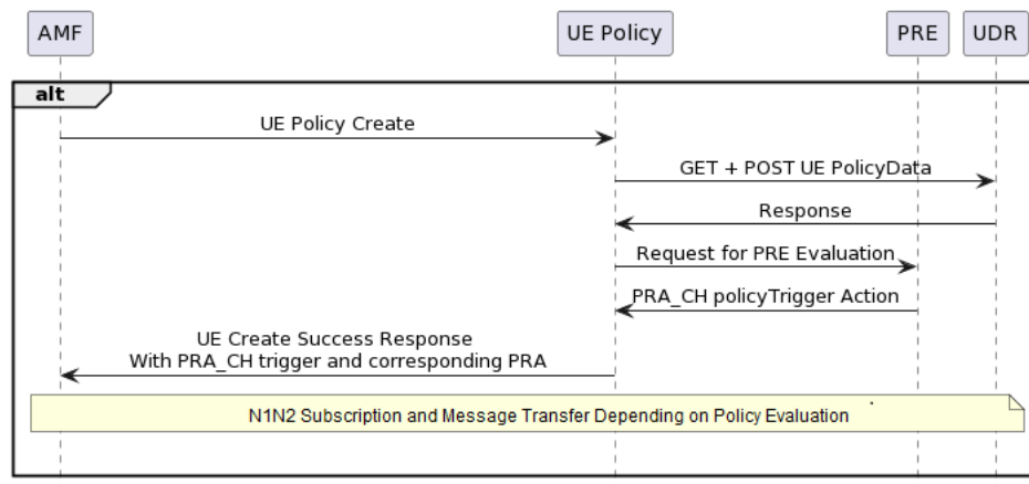
Figure 4-47 UE Policy Association create scenario:
