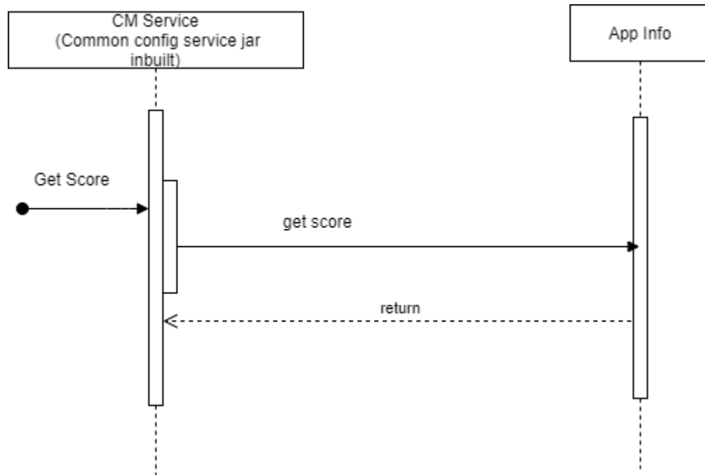
Figure 4-156 Call flow to Get the NF Score
