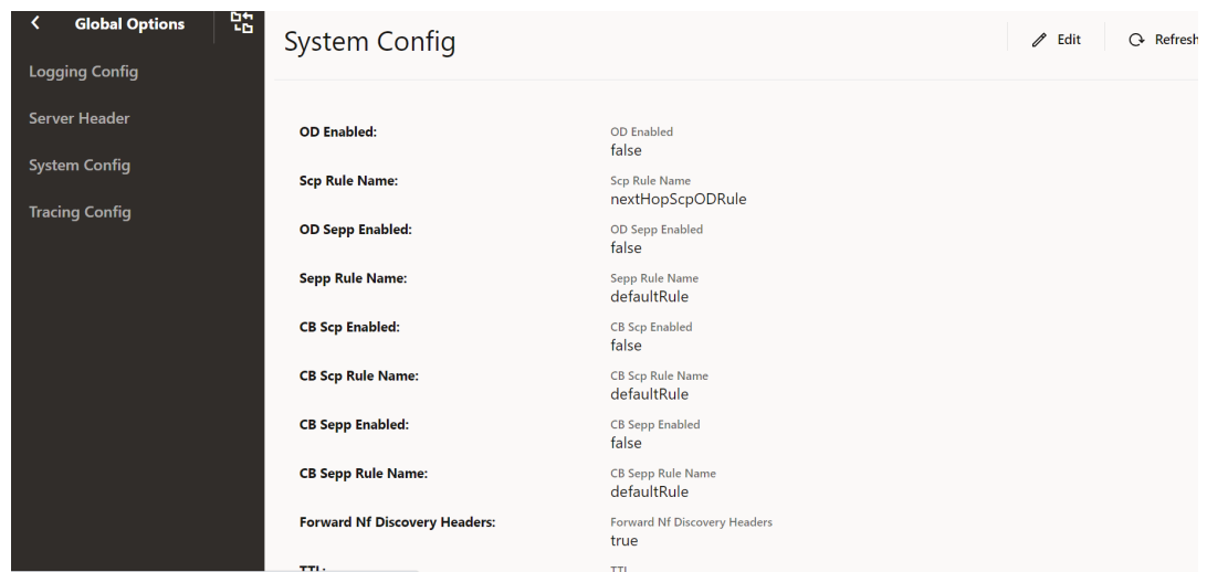
Figure 4-37 System Config
