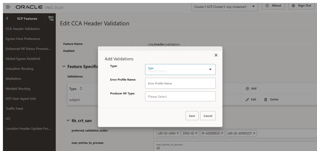
Figure 4-15 Add Validations
