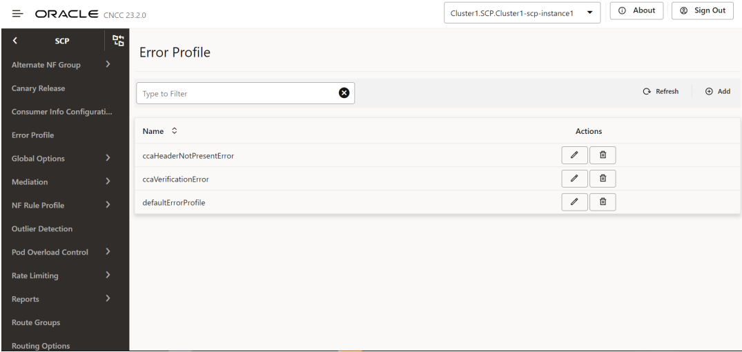
Figure 4-31 Error Profile
