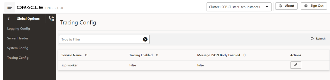
Figure 4-38 Tracing Config
