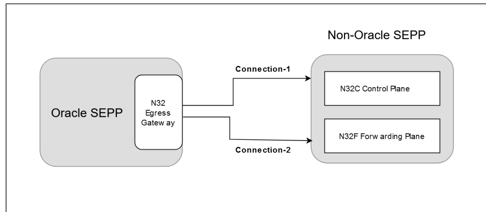
Figure 3-3 Separate Port Configurations Design Diagram
