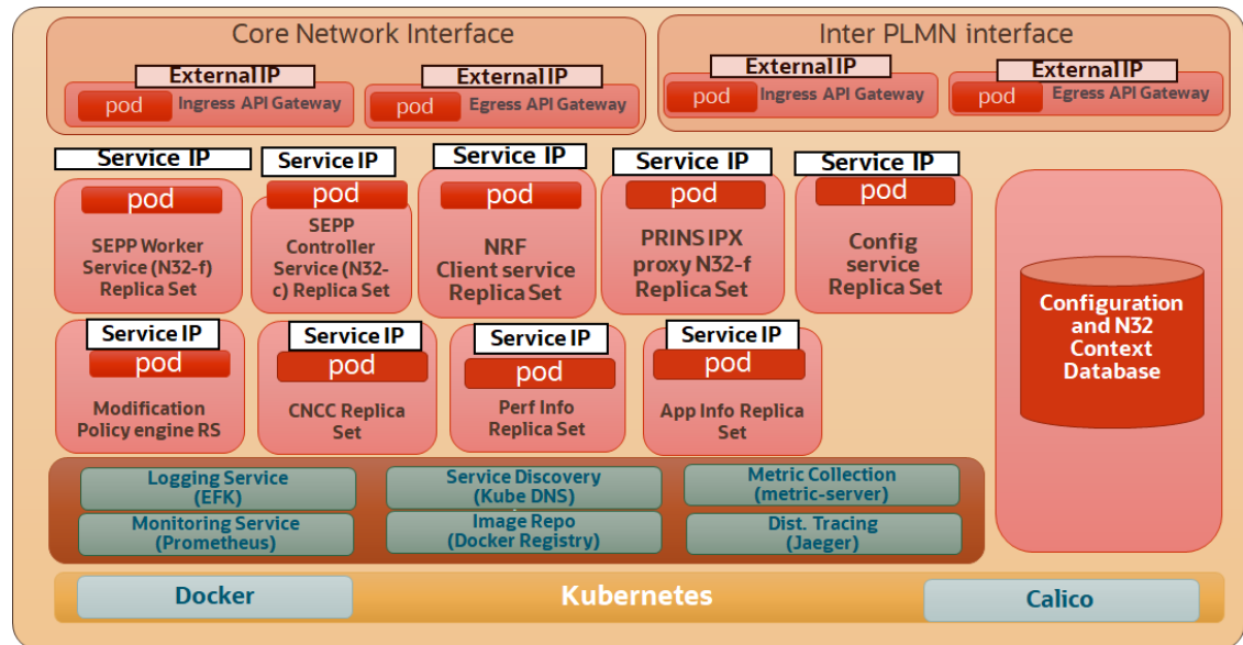
Figure 3-21 Dedicated gateways for IntraPLMN InterPLMN traffic
