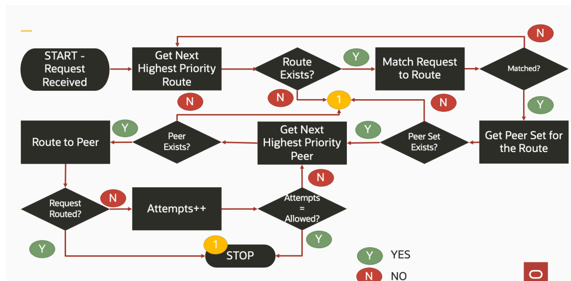
Figure 3-19 Alternate Routing Flow Chart Representation
