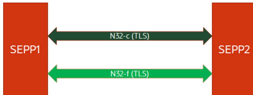
Figure 3-20 Topology for SEPP MNO functionality
