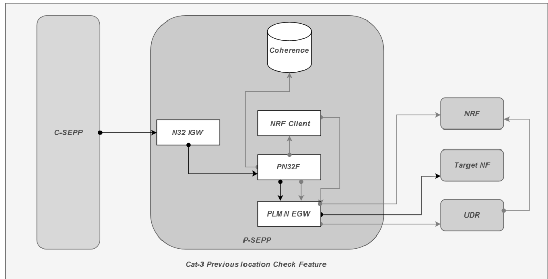
Figure 3-38 Design and Architecture
