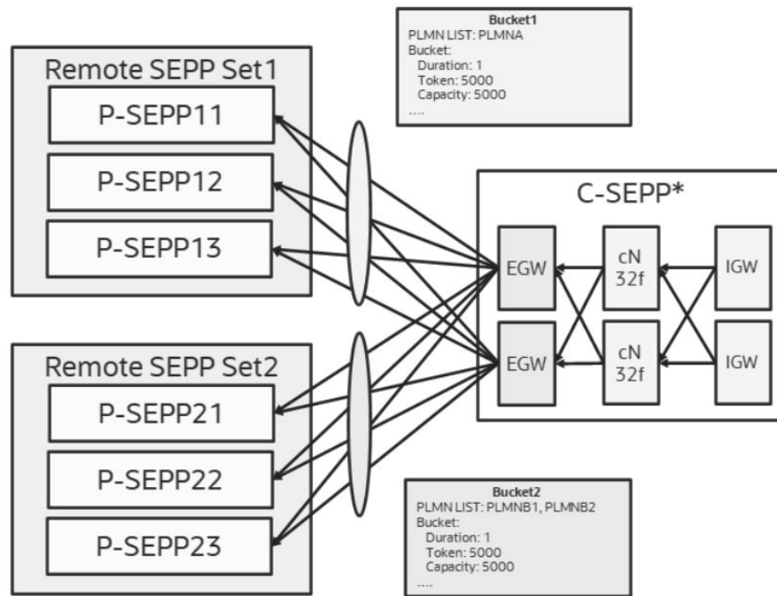
Figure 3-50 Implementation at C-SEPP
