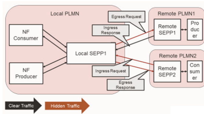
Figure 3-6 Topology Hiding Architecture
