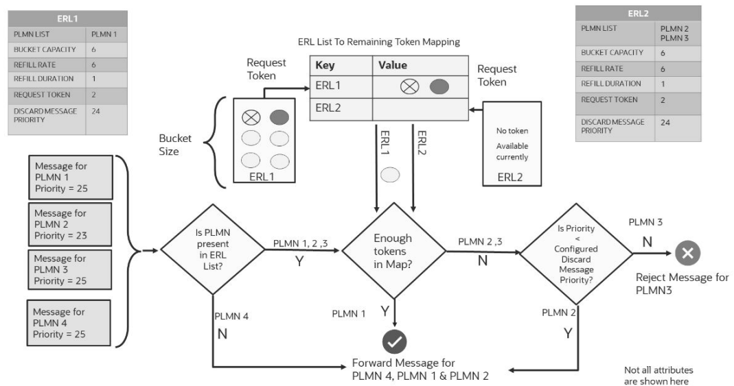
Figure 3-49 Token Bucket Algorithm
