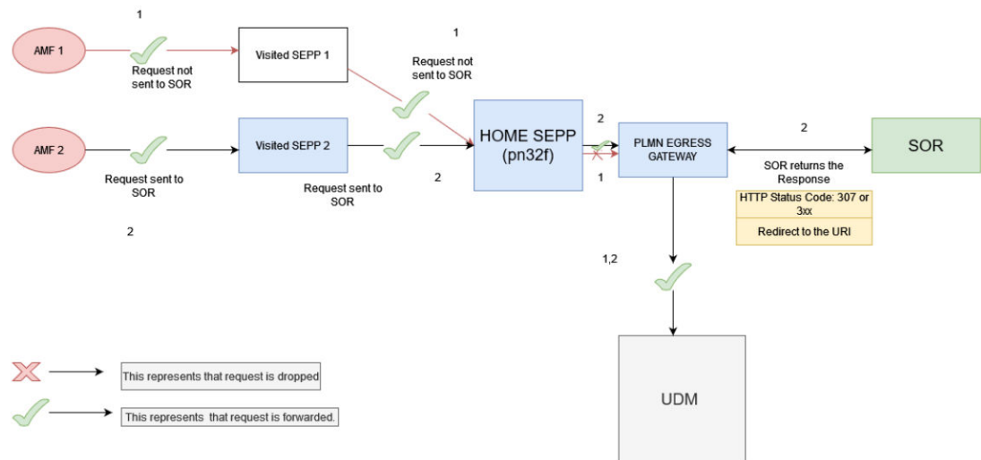
Figure 3-40 Redirection Enabled Mode
