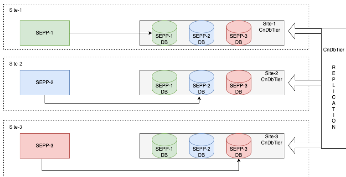
Figure 3-43 Three-Site Georedundancy Deployment
