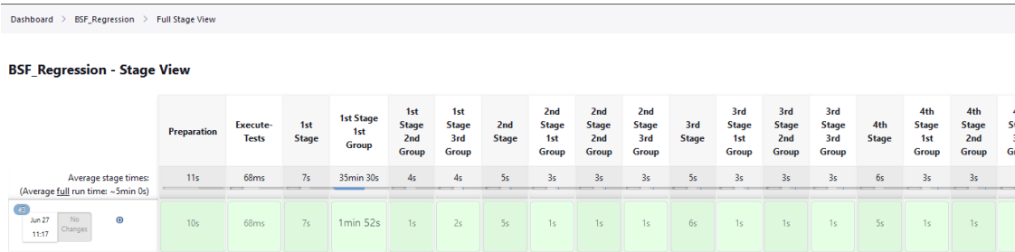
Figure 4-11 BSF_Regression Pipeline
