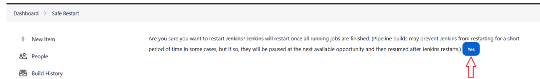
Figure 2-26 Restart Jenkins
