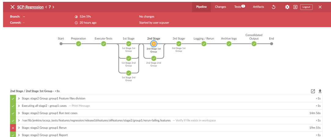
Figure 2-58 Stage Execution
