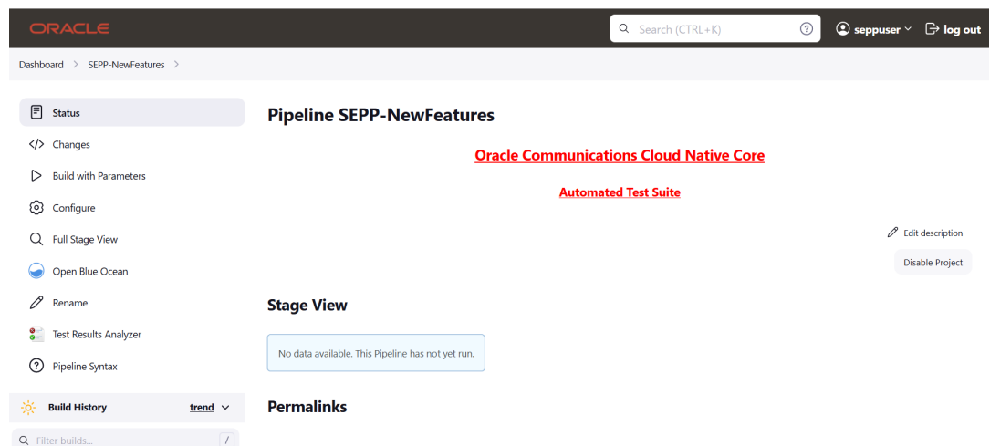
Figure 4-75 SEPP-NewFeatures Pipeline
