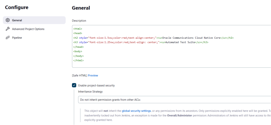
Figure 4-18 Pipeline Tab
