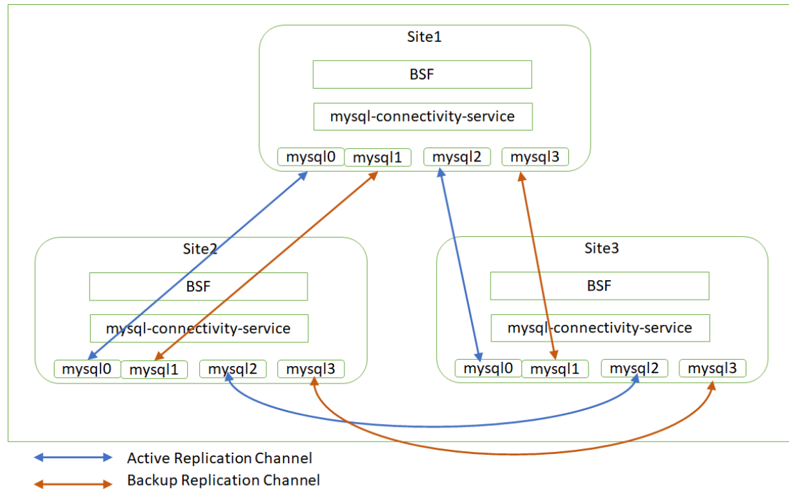
Figure 3-19 Three-Site Georedundancy
