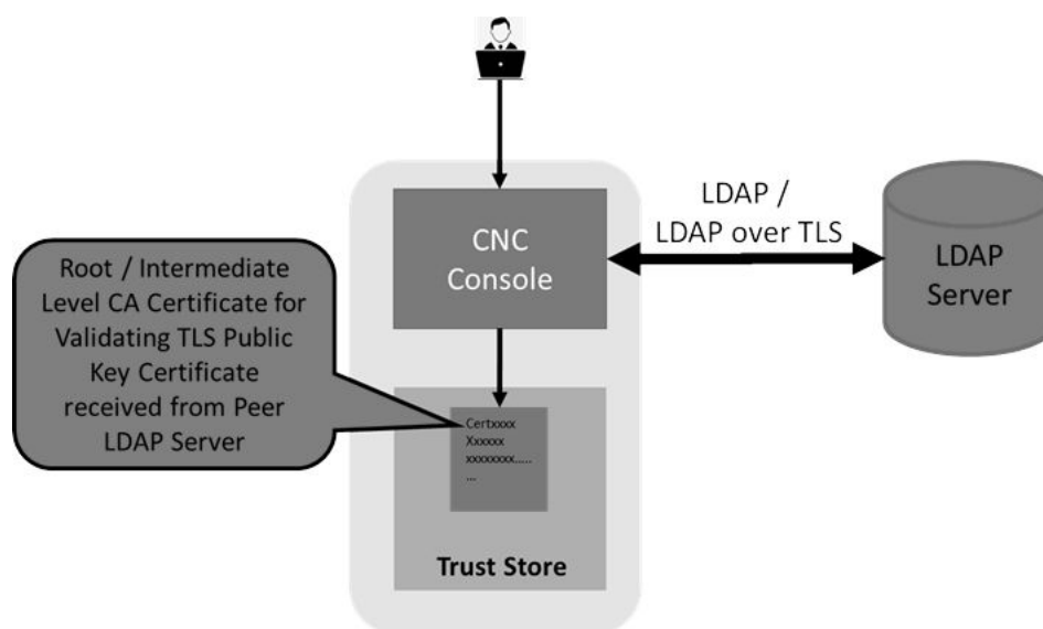
Figure 2-1 LDAP
