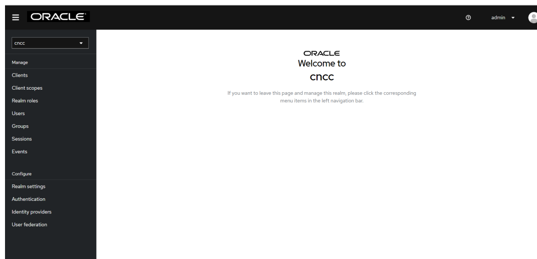
Figure 4-2 Realm Settings
