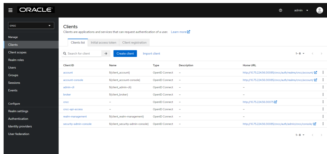
Figure 4-12 Clients Screen
