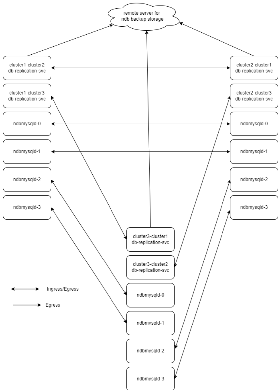
Figure 2-6 Three_Cluster_Ingress_Egress_Routes
