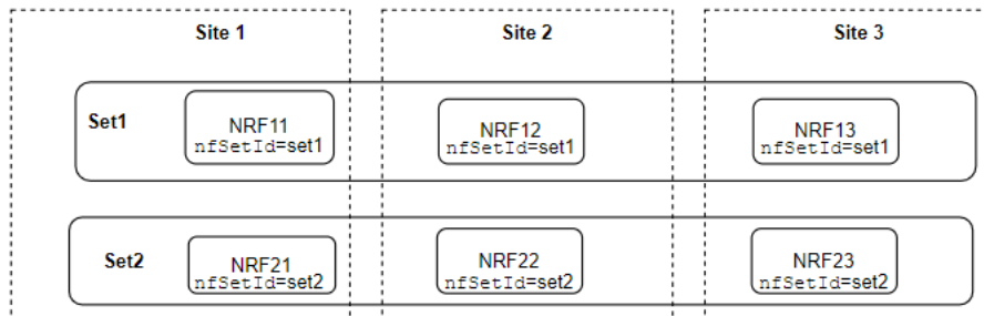
Figure 4-6 NRF Growth nfSetId Configuration
