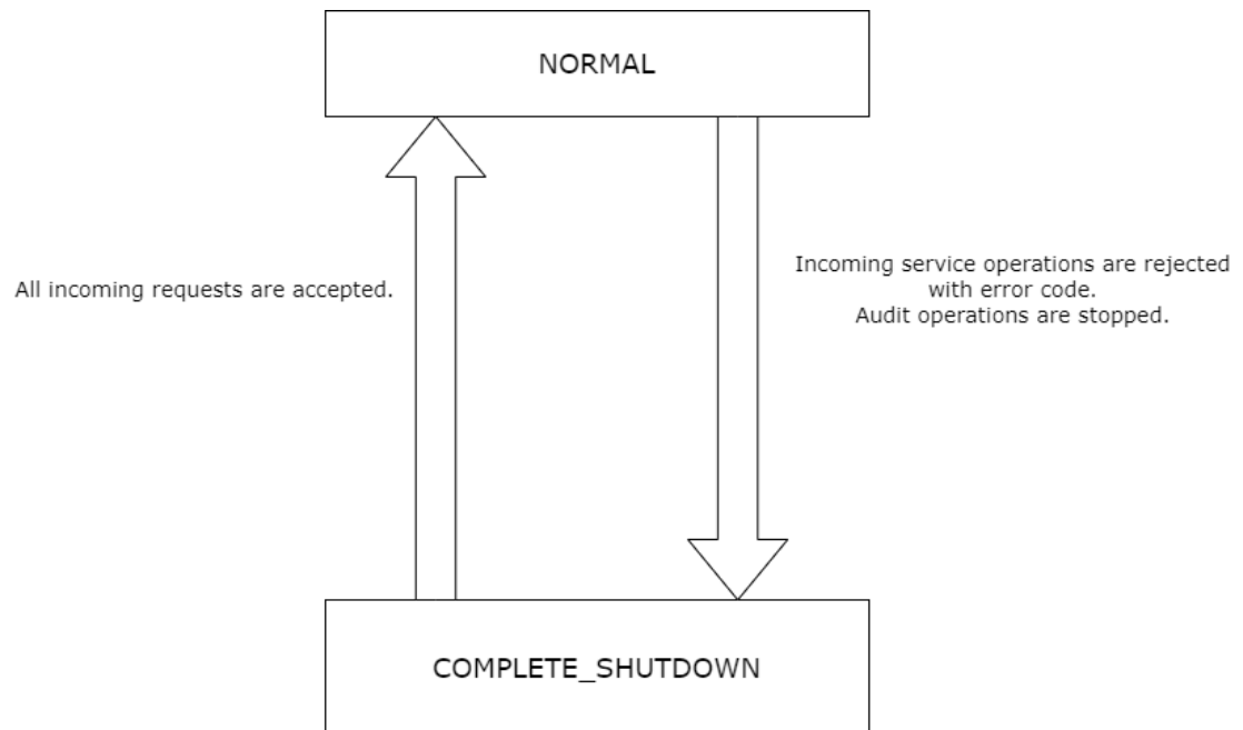
Figure 4-14 Operational State changes
