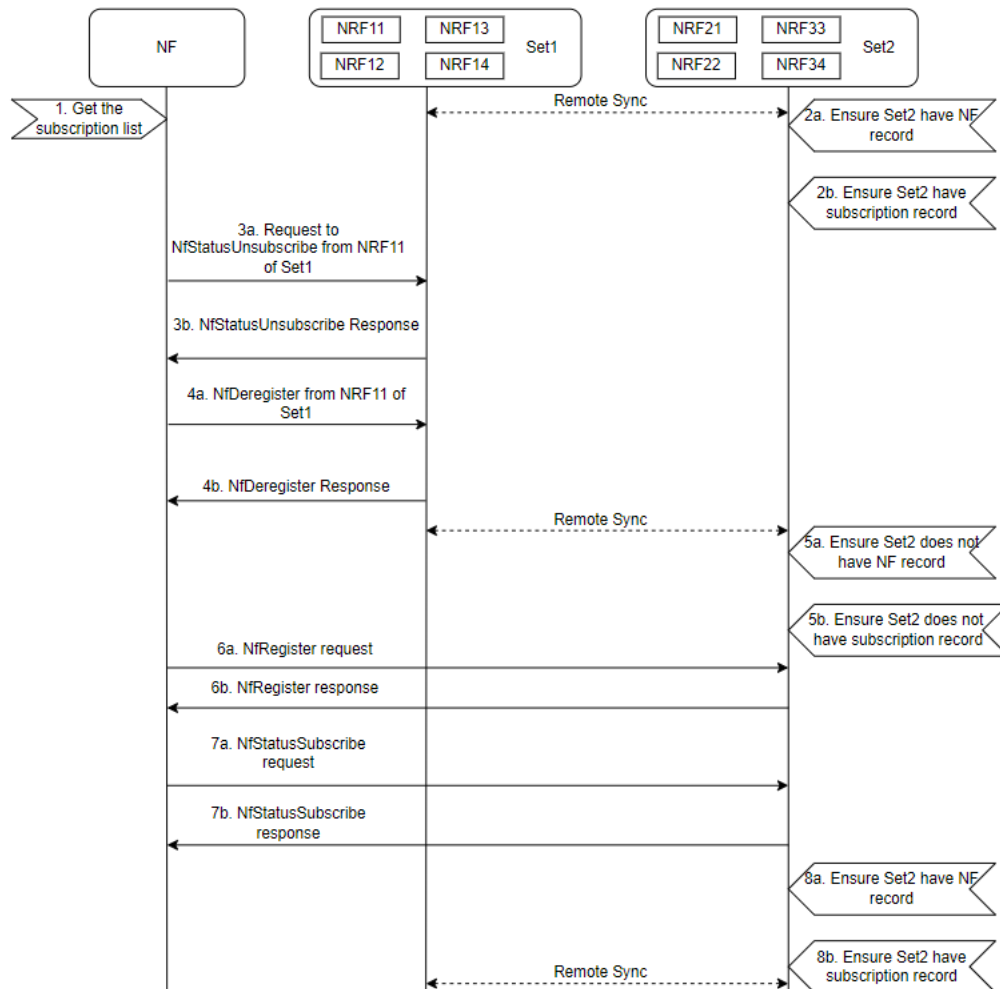
Figure 4-7 Migration of NF from one set to another
