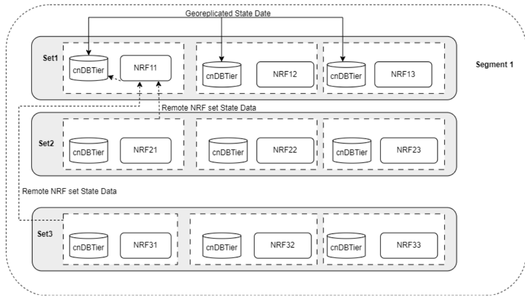
Figure 4-4 State Data in NRF
