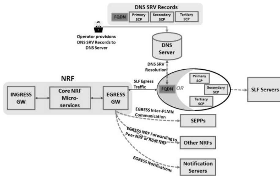
Figure 4-9 Routing Egress Messages through SCP
