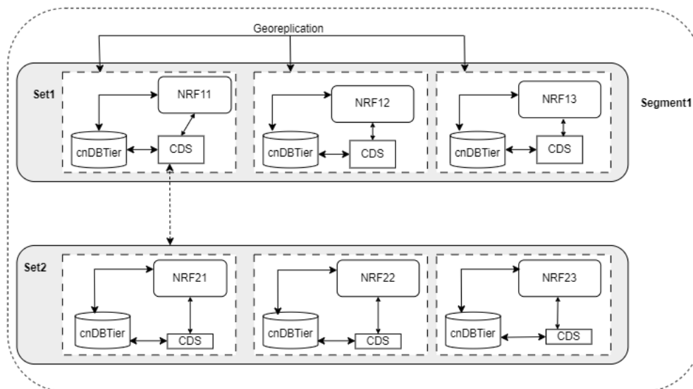
Figure 4-5 Cache Data Service
