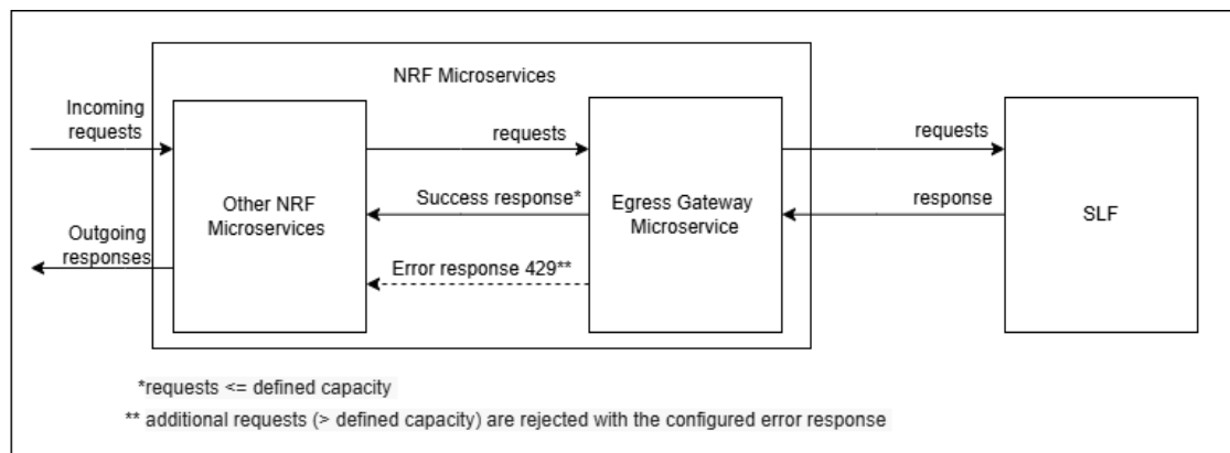
Figure 4-1 Egress Gateway Pod Throttling Mechanism
