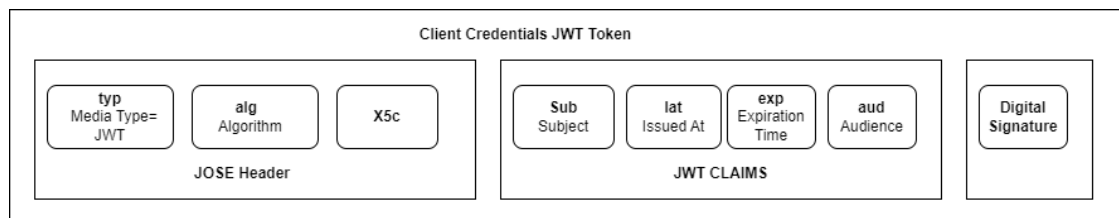
Figure 4-12 Client Credentials JWT Token
