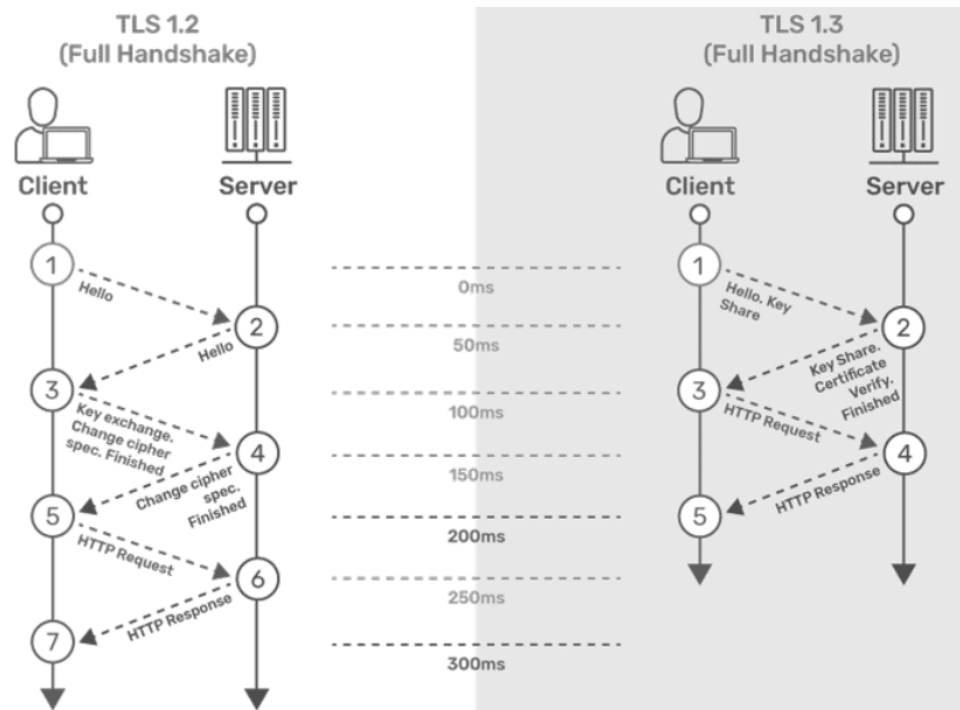
Figure 4-2 TLS Handshake
