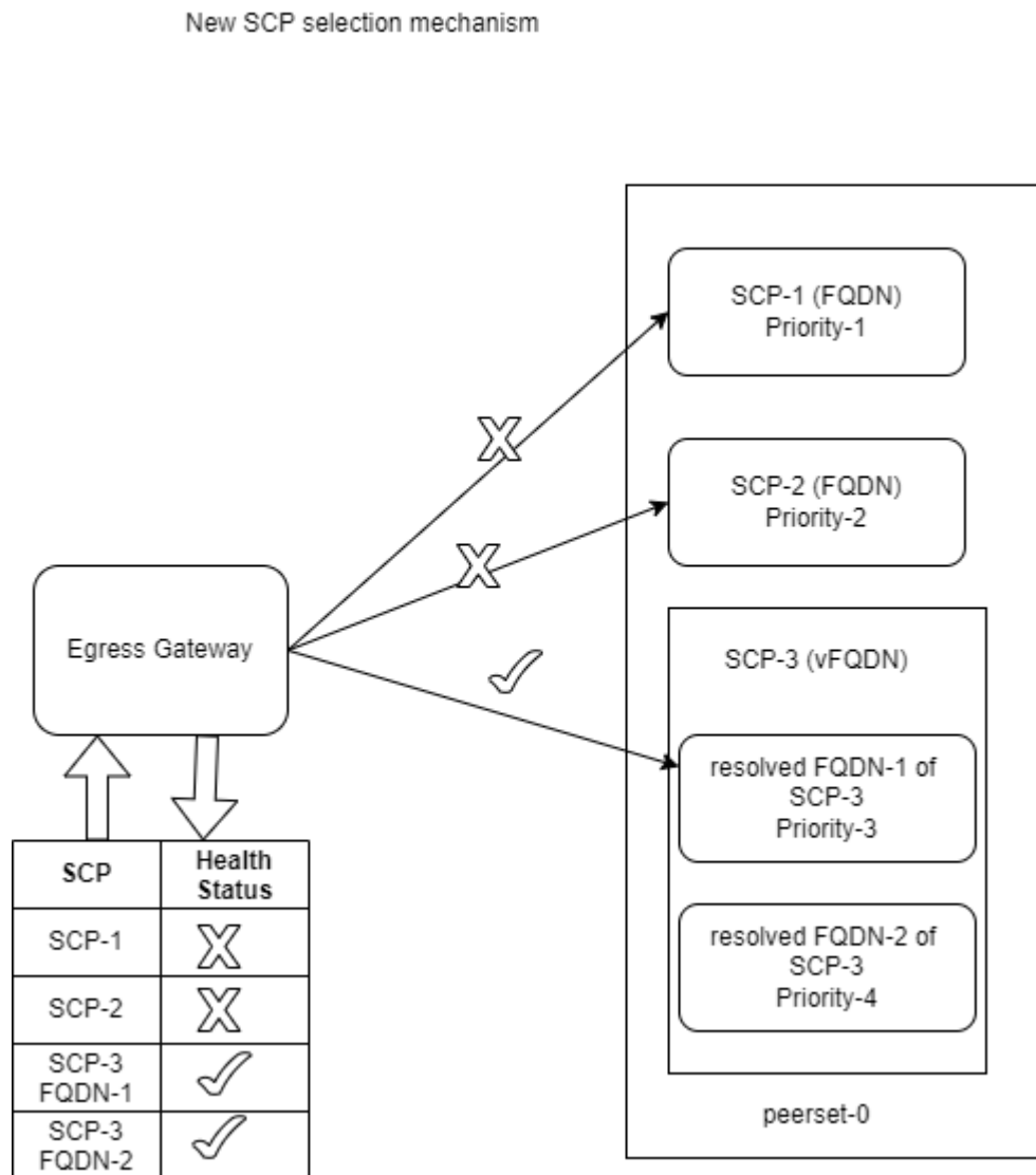
Figure 4-13 SCP Selection Mechanism
