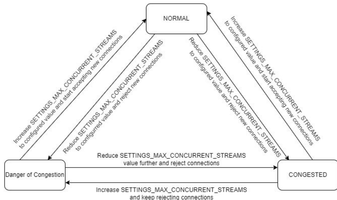
Figure 4-11 Pod Protection State Transition
