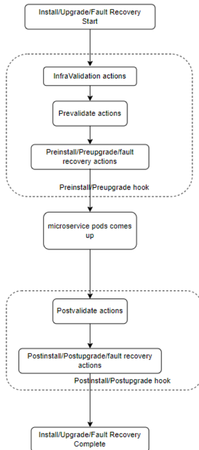
Figure 4-17 Pre and Post Install/Upgrade Validations
