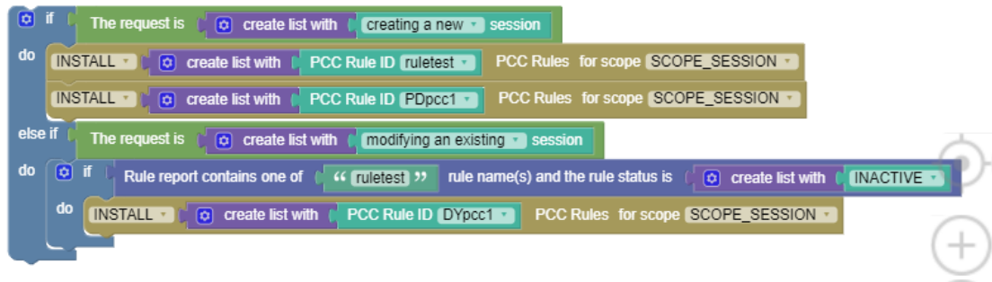
Figure 4-18 Use case for Rule Report Conditions
