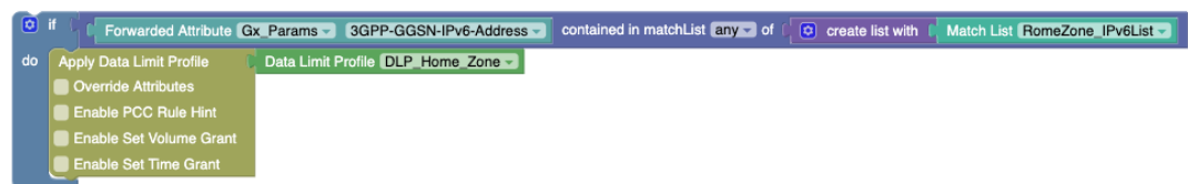
Figure 4-57 Example for IPV6 Data Type in Match List
