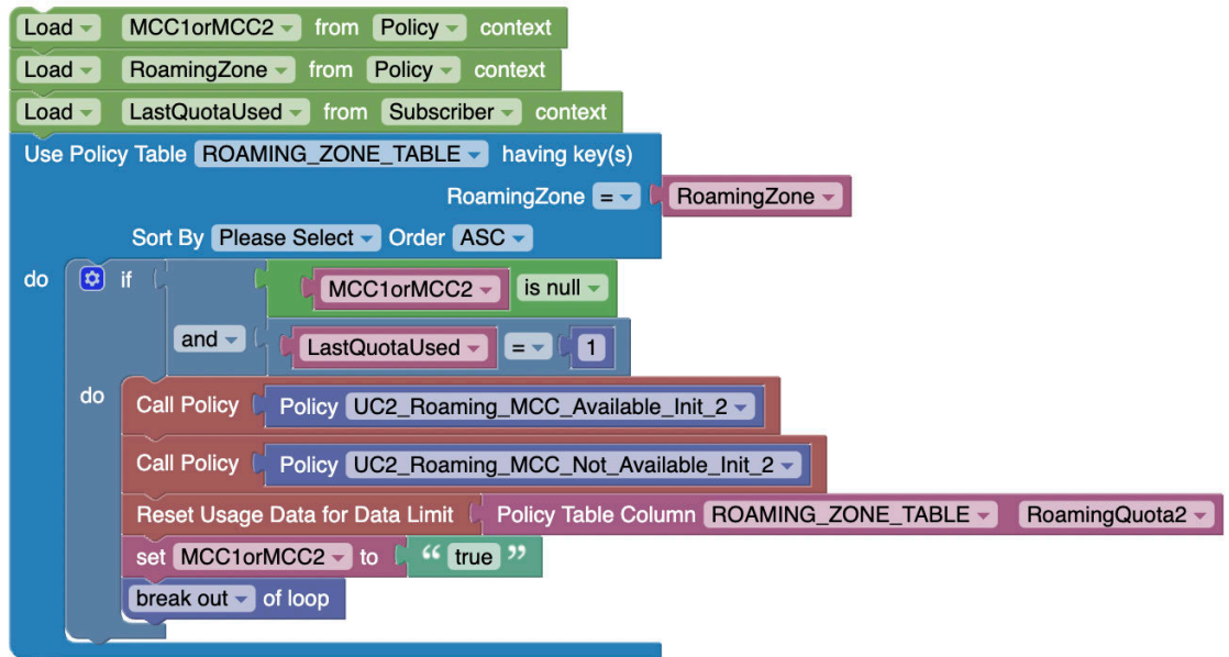
Figure A-17 Policy Project for Roaming Variable Init Override
