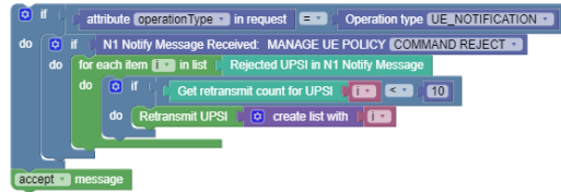
Figure 4-16 Use case scenario 4:
