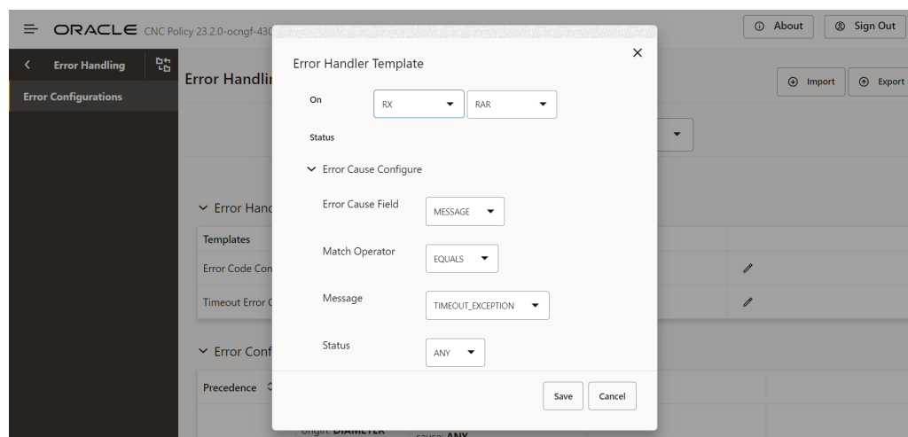
Figure 7-11 Diameter Timeout Error Configuration:
