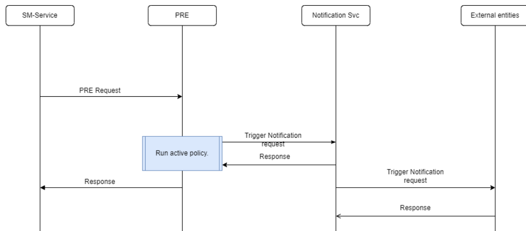
Figure 3-5 Notifier Call Flow for SM Service
