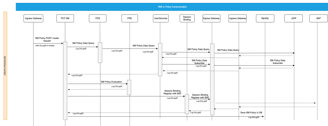
Figure 4-6 Example: Unique Identifier for SM Create Call Flow
