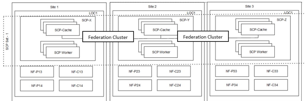
Figure 3-10 Role of SCP-Cache
