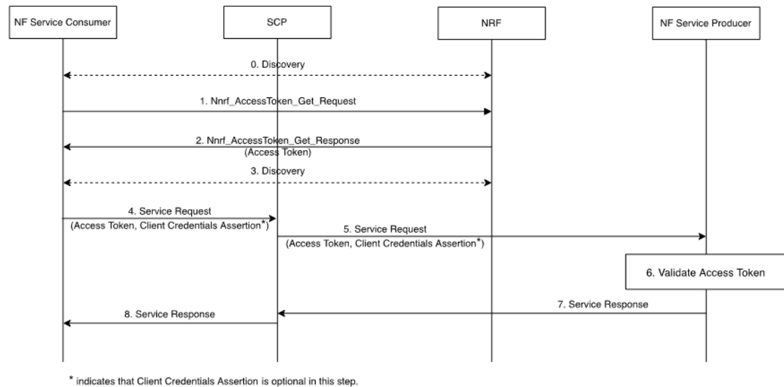
Figure 3-5 NF Consumer Obtains Access Tokens from NRF
