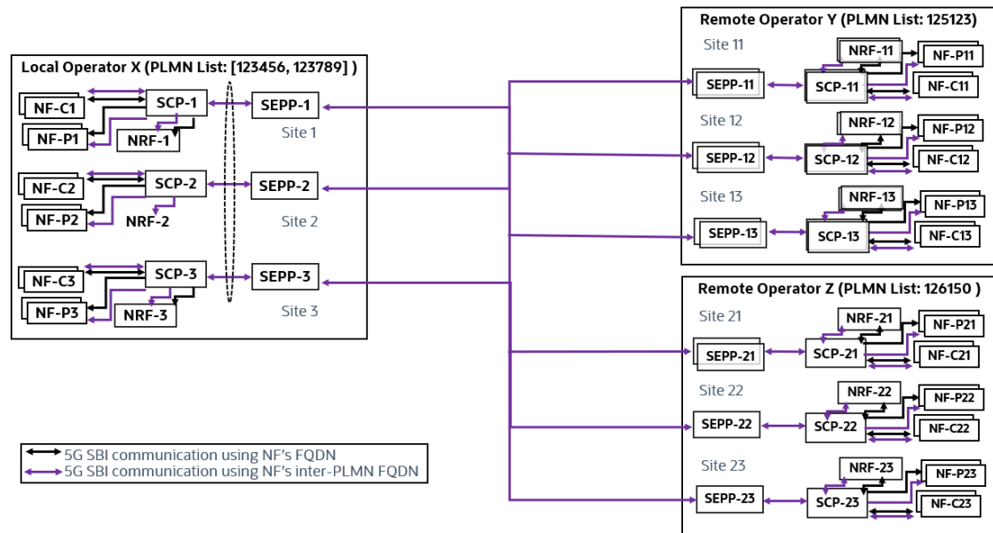
Figure 3-12 Local and Remote Routing
