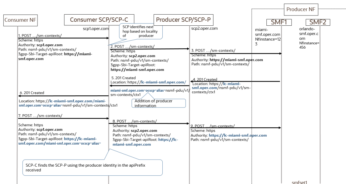
Figure 3-3 Initial and Subsequent Request Routing Supported at SCP
