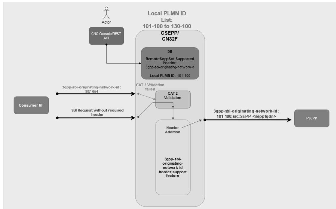
Figure 3-1 C SEPP side functionality
