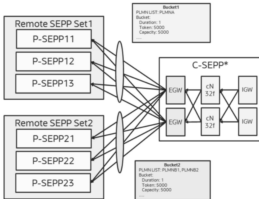
Figure 3-53 Implementation at C-SEPP
