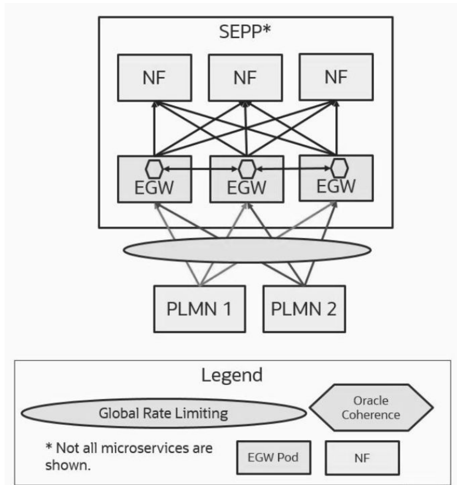
Figure 3-11 Architecture
