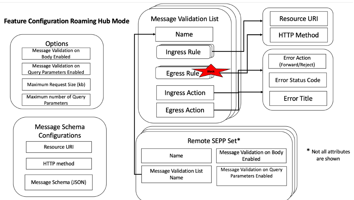
Figure 3-36 CNC Console options available for Cat - 0 SBI Message Schema Validation feature in Roaming Hub Mode
