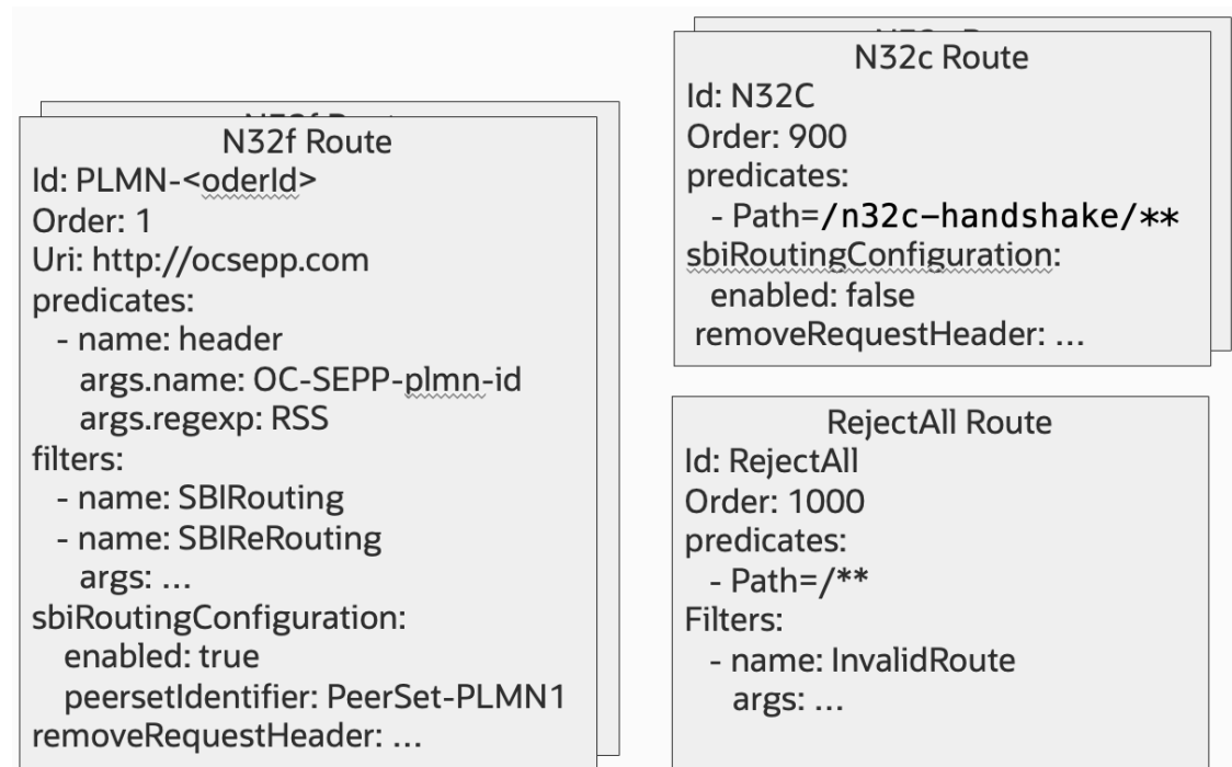
Figure 3-21 Default Routes
