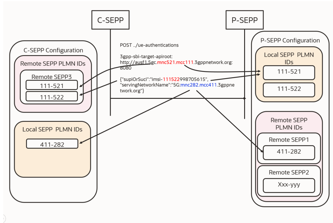
Figure 3-37 SEPP Mode
