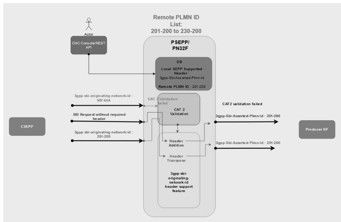
Figure 3-2 P SEPP side functionality
