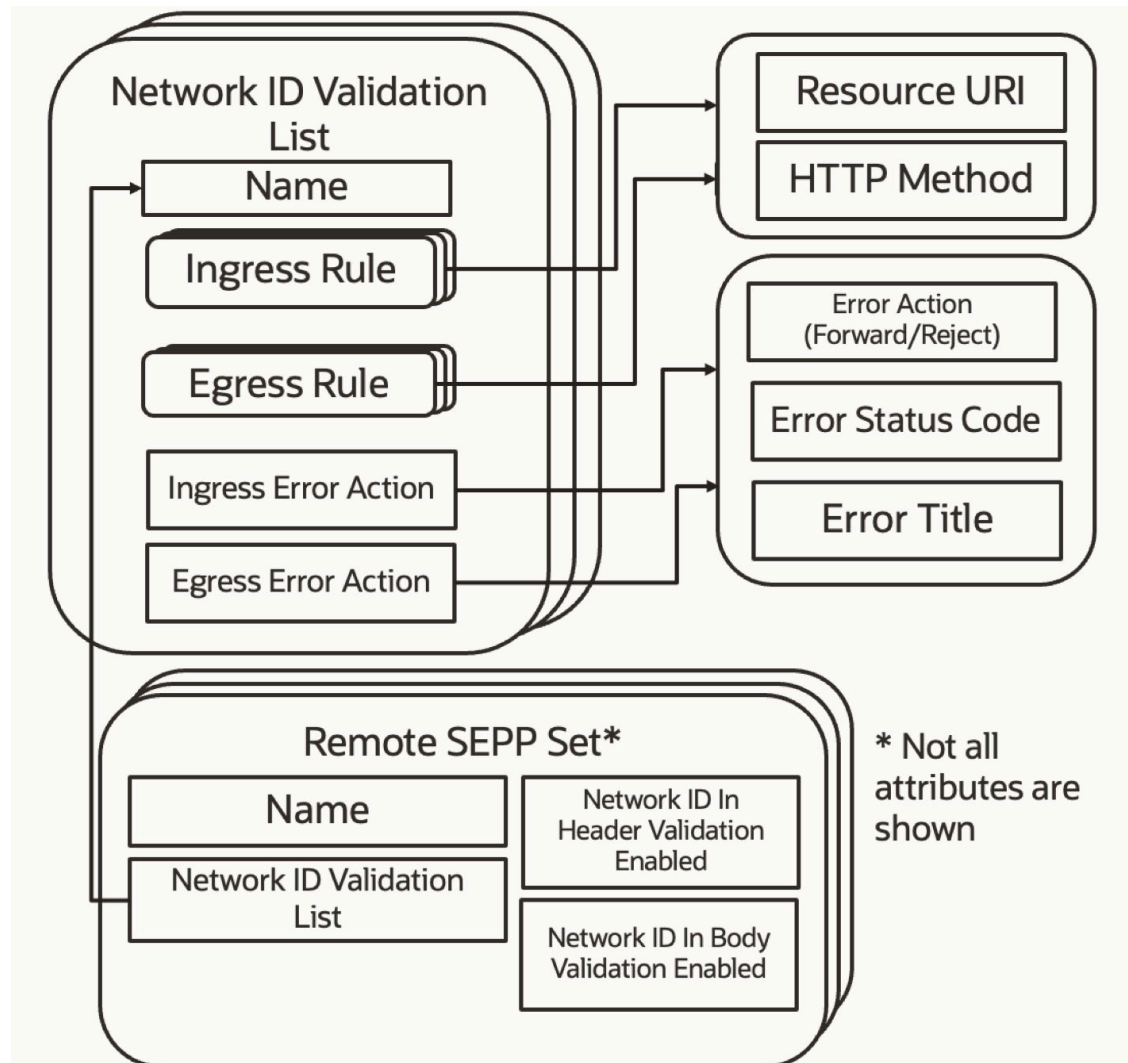
Figure 3-40 Feature Configuration – Network ID Validation List
