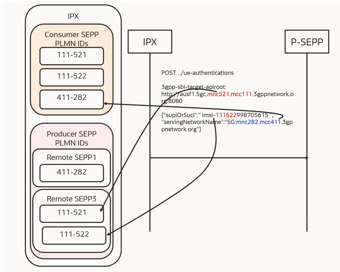
Figure 3-38 Roaming Hub mode
