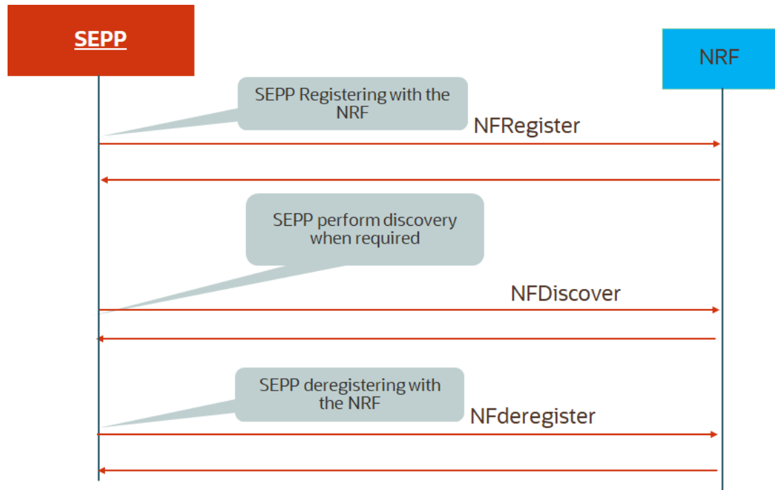
Figure 3-27 NRF Interface Registration & Reregistration.
