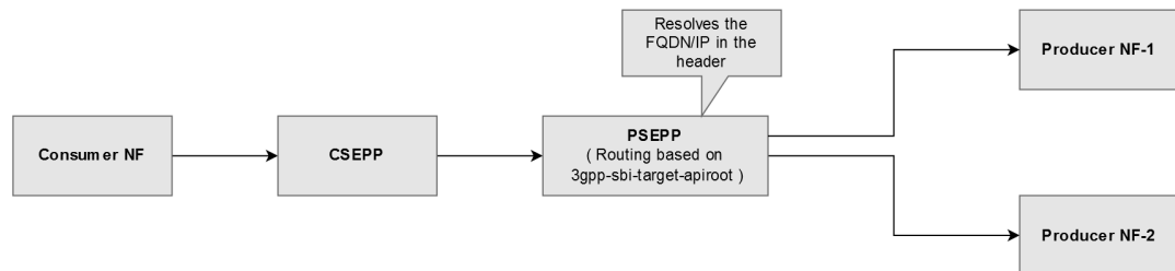
Figure 3-50 Direct Communication
