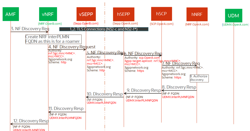
Figure 3-25 SEPP sets the 3GPP-SBI-Target-APIroot header
