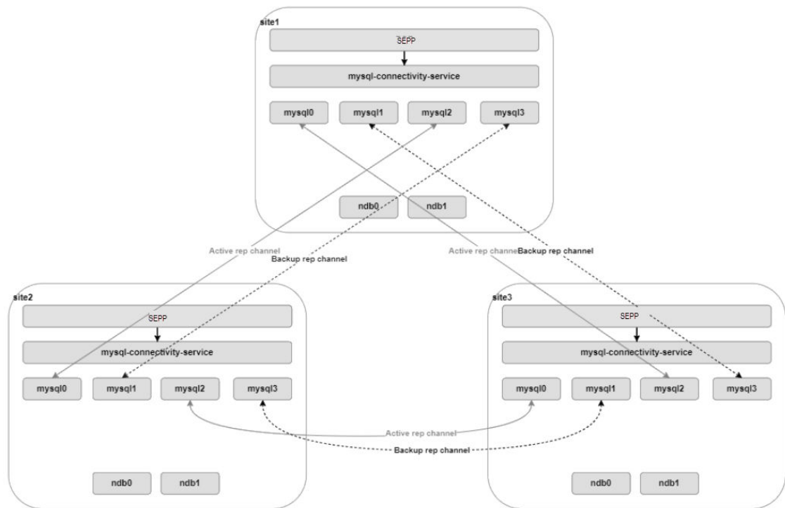
Figure 3-48 Three-Site Georedundancy
