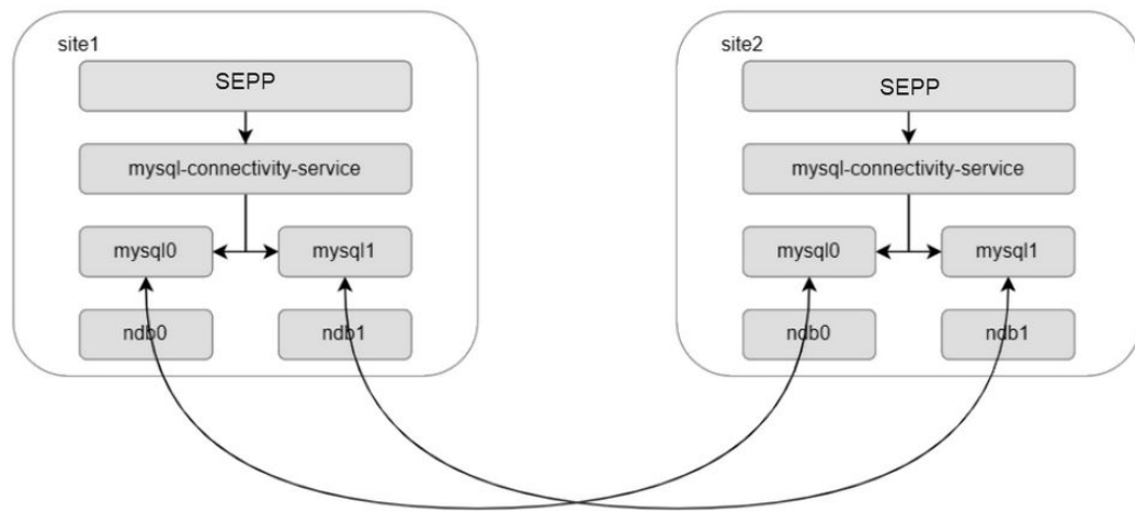
Figure 3-47 Two-Site Georedundancy
