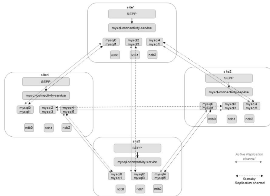
Figure 3-49 Four-site Georedundancy
