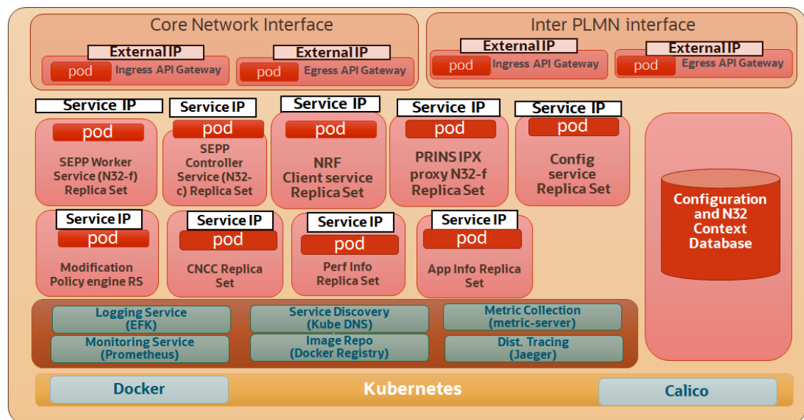
Figure 3-24 Dedicated gateways for IntraPLMN InterPLMN traffic
