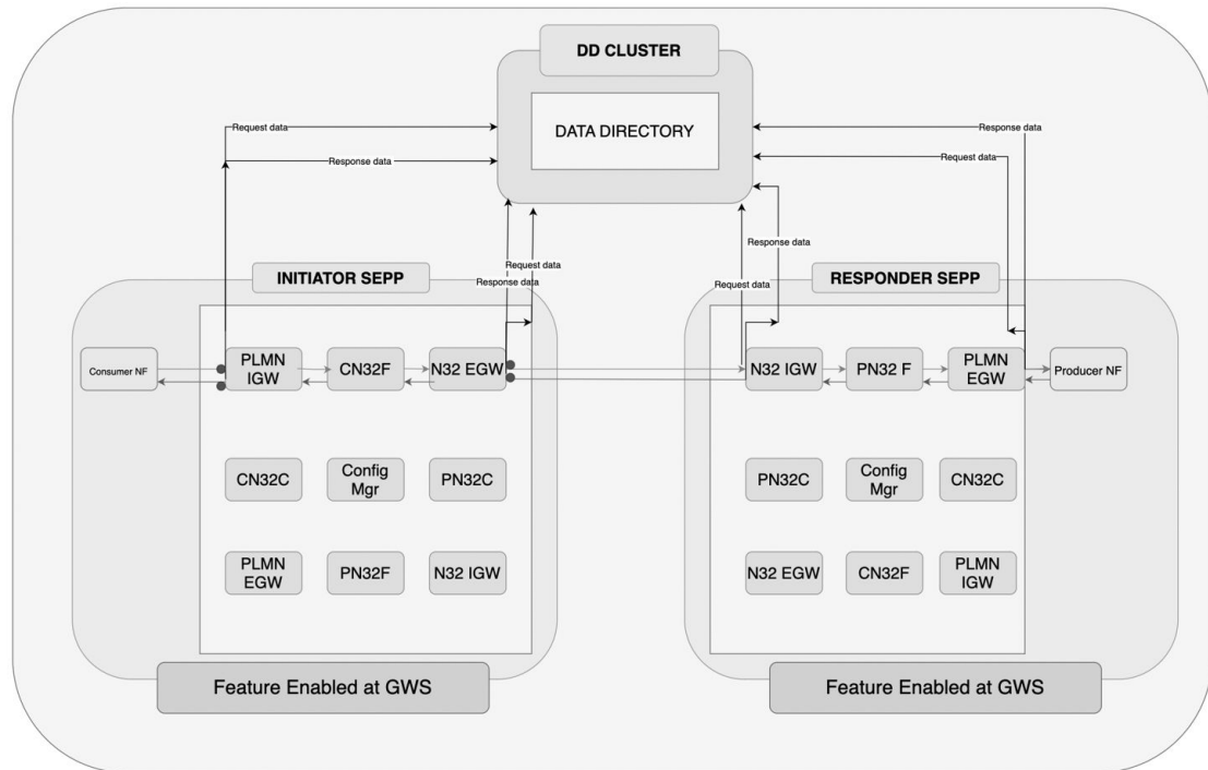
Figure 3-30 Detailed view of message feed feature in SEPP
