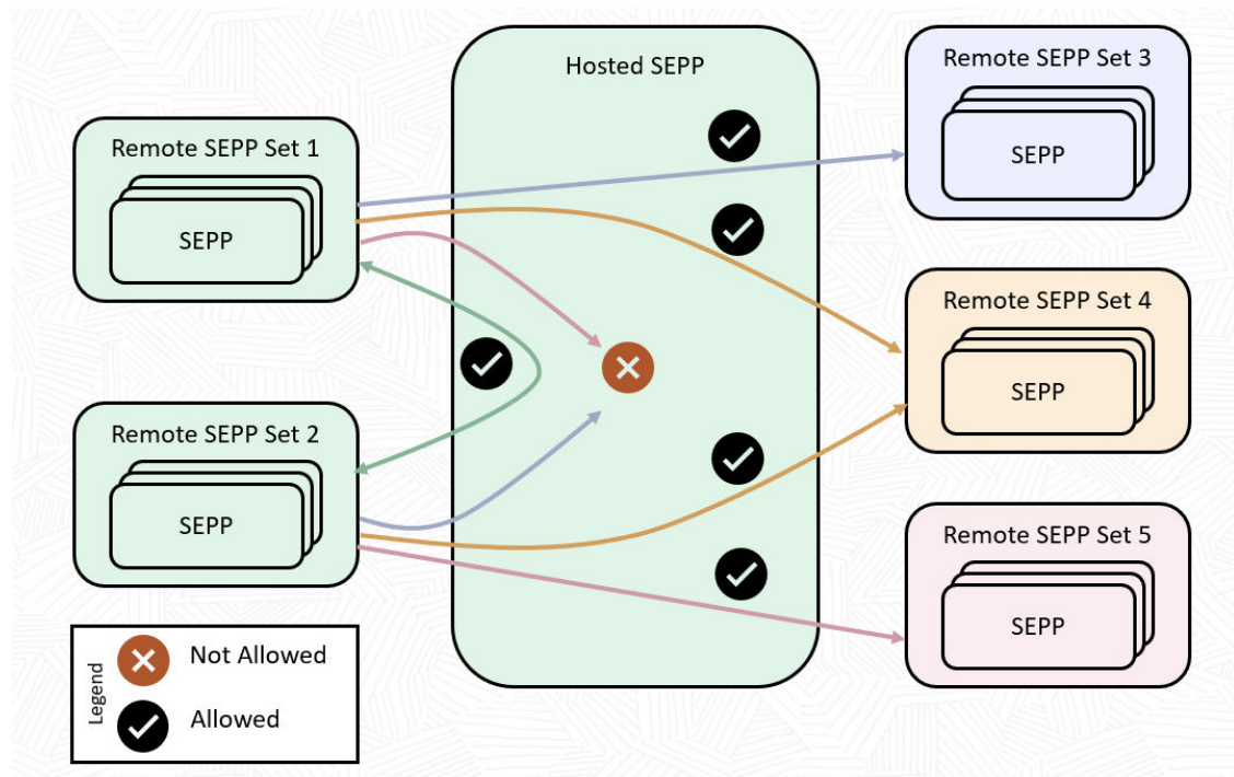
Figure 3-33 Hosted SEPP Overview
