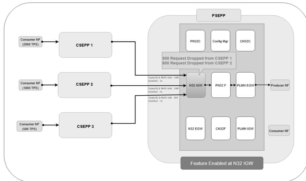
Figure 3-45 Rate limiting for Ingress Roaming Signaling per Remote SEPP Set Architecture
