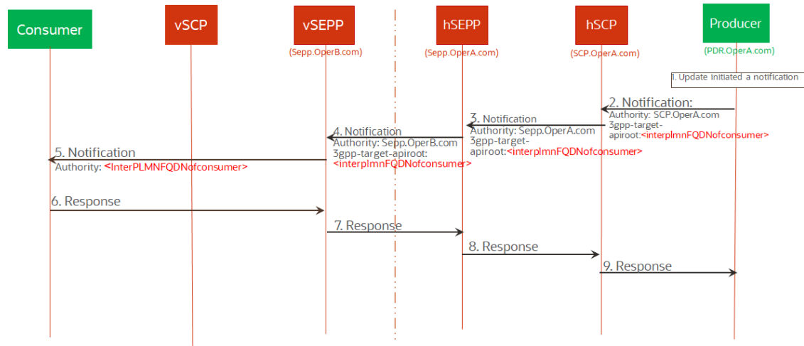
Figure 3-26 SEPP removes the 3GPP-SBI-Target-APIroot header
