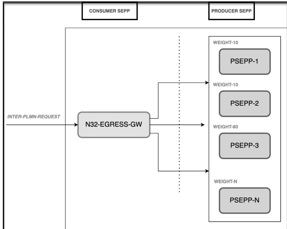
Figure 3-4 Architecture
