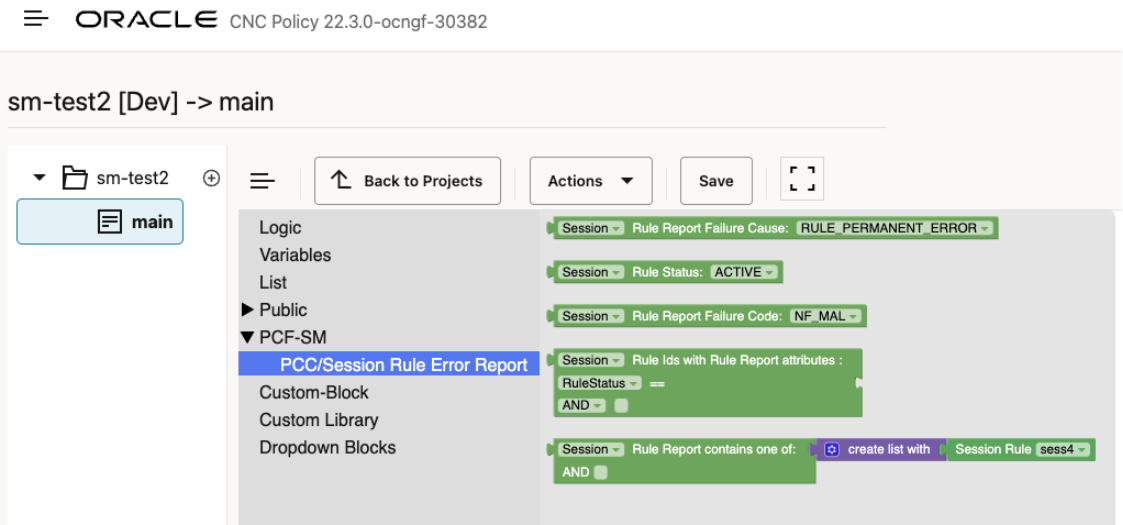
Figure 3-31 Sample block for PCC/Session Rule Error Report
