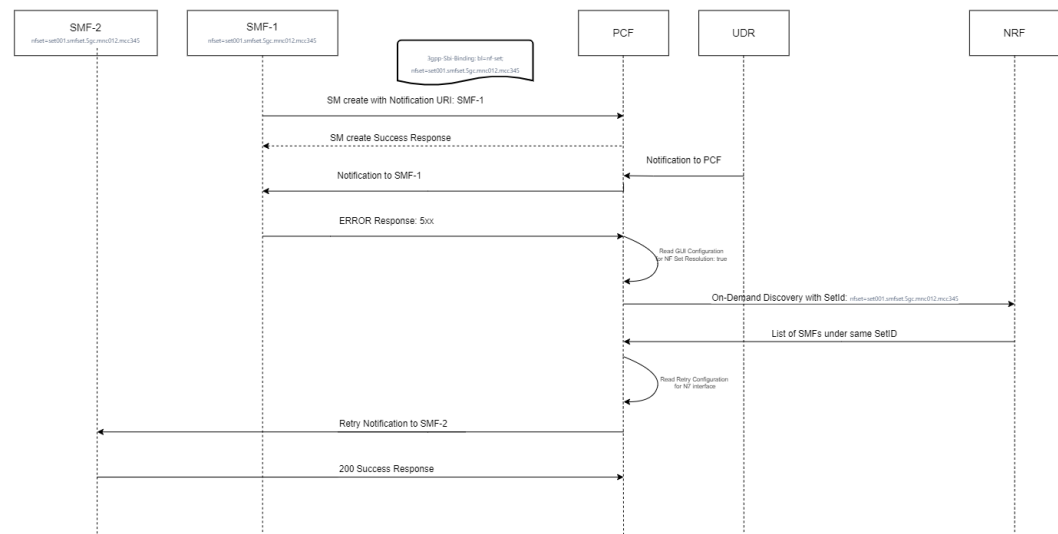
Figure 4-87 On demand NF Discovery is enabled (NF Set Resolution is set to NRF Discovery)
