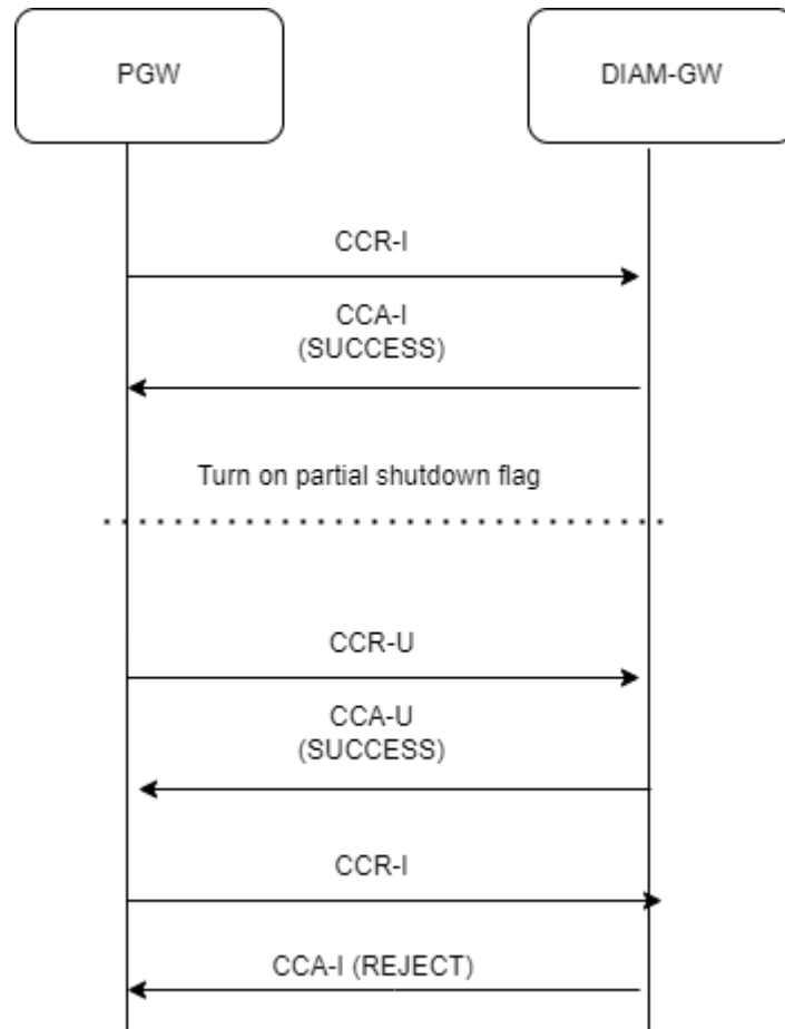
Figure 4-158 Call Flow for Diameter Gateway PARTIAL SHUTDOWN
