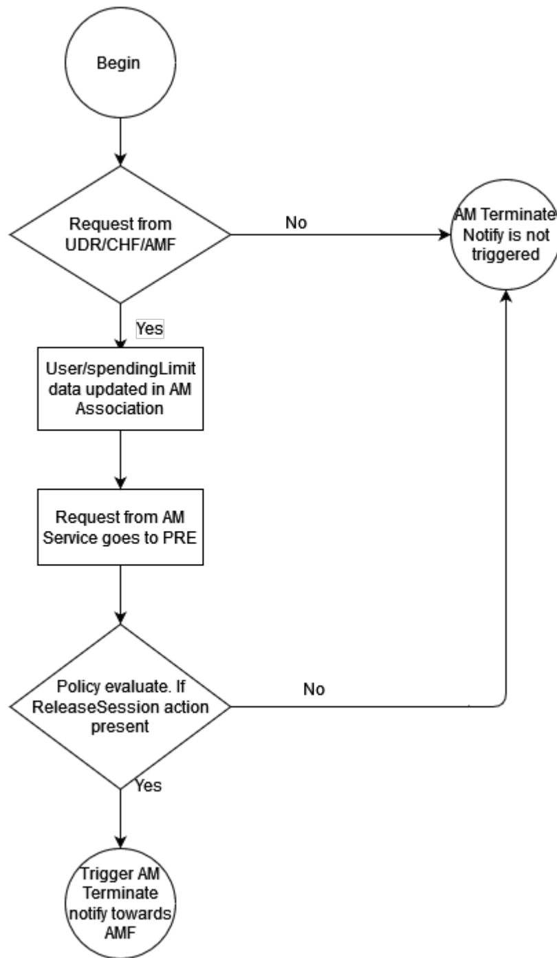
Figure 4-32 PCF Triggering AM UpdateNotify Terminate
