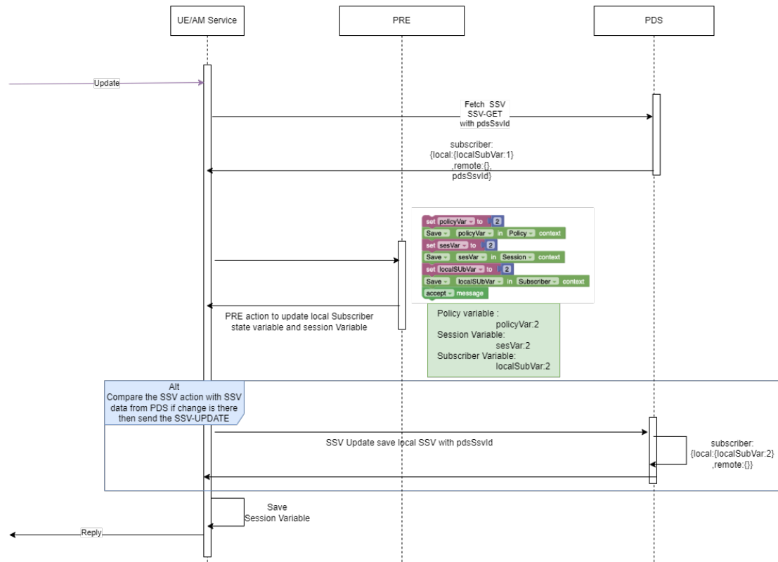
Figure 4-177 State variables in update session call flow
