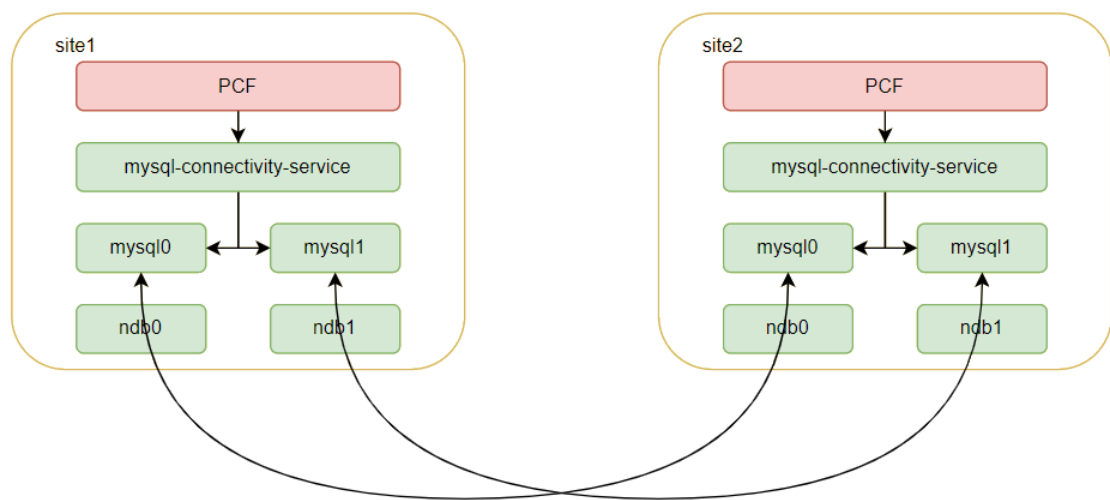
Figure 4-100 Two-Site Georedundancy Deployment
