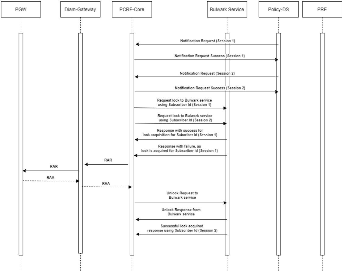
Figure 4-146 Call Flow- PDS notification (RAR) Integration with Bulwark Service
