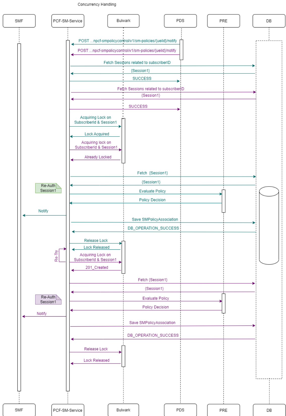
Figure 4-116 Call Flow for SM Update-Notify Request (Two Notifications and 1 Session)
