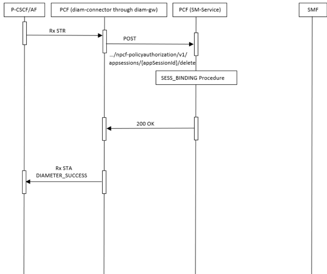
Figure 4-80 Cancellation of subscription to notification of the AF Signaling Transmission in 5G
