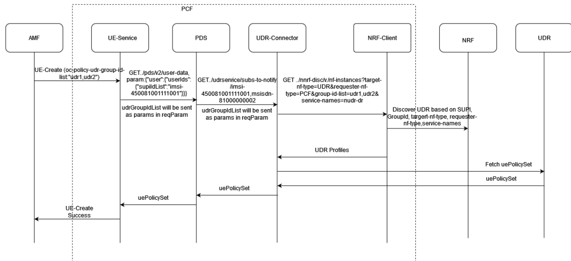
Figure 4-51 AMF sends UE Policy Association Request with oc-policy-udr-group-id
