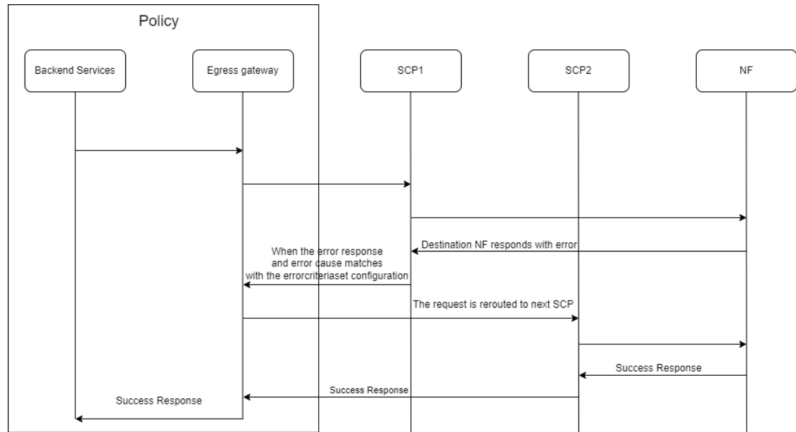
Figure 4-86 Session Retry at Egress Gateway
