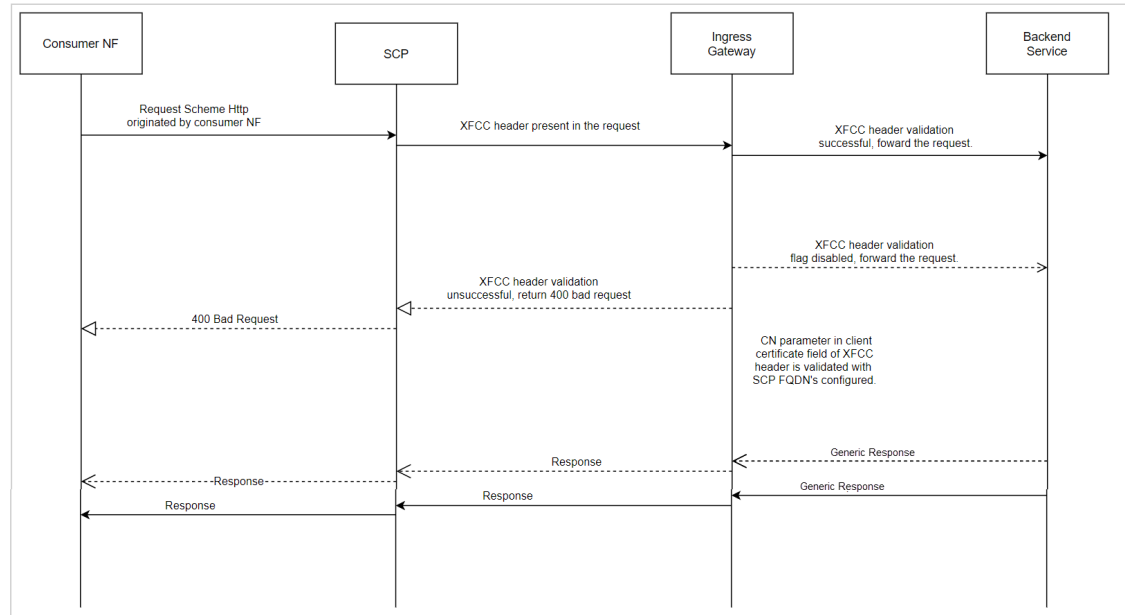
Figure 4-108 Call Flow Validating single XFCC Header
