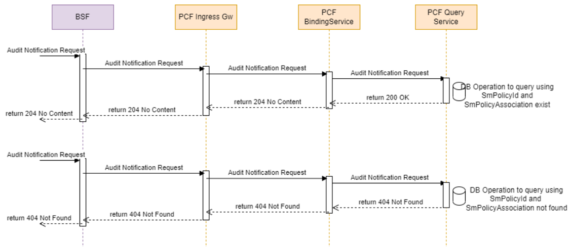
Figure 4-112 BSF and PCF Interaction for Stale Binding Detection
