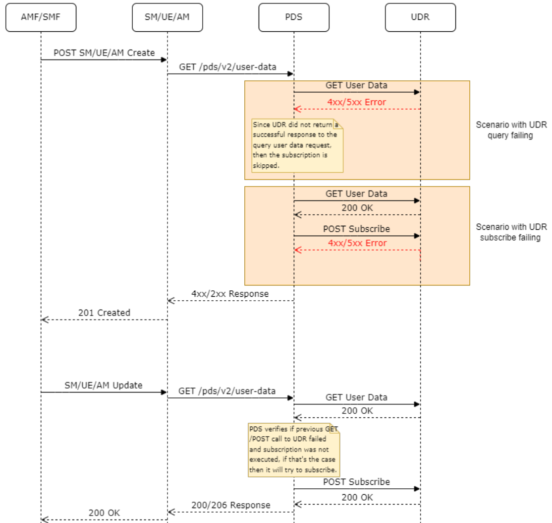
Figure 4-61 Retrieving user data from UDR upon a GET or Update request to a Policy Service
