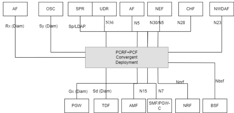
Figure 4-185 Converged Policy Architecture to Support EPC and 5GC
