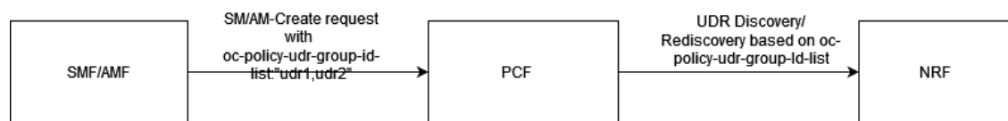
Figure 4-48 UDR Discovery with oc-policy-udr-group-id-list Header to NRF
