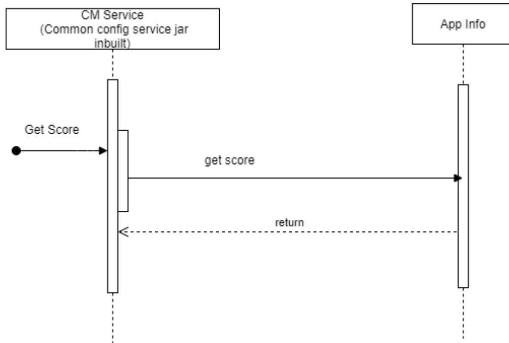
Figure 4-172 Call flow to Get the NF Score
