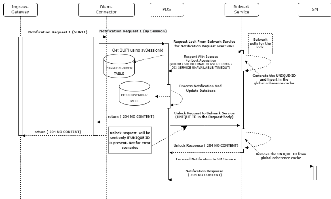
Figure 4-149 Call Flow - Bulwark Lock Request For OCS Notification
