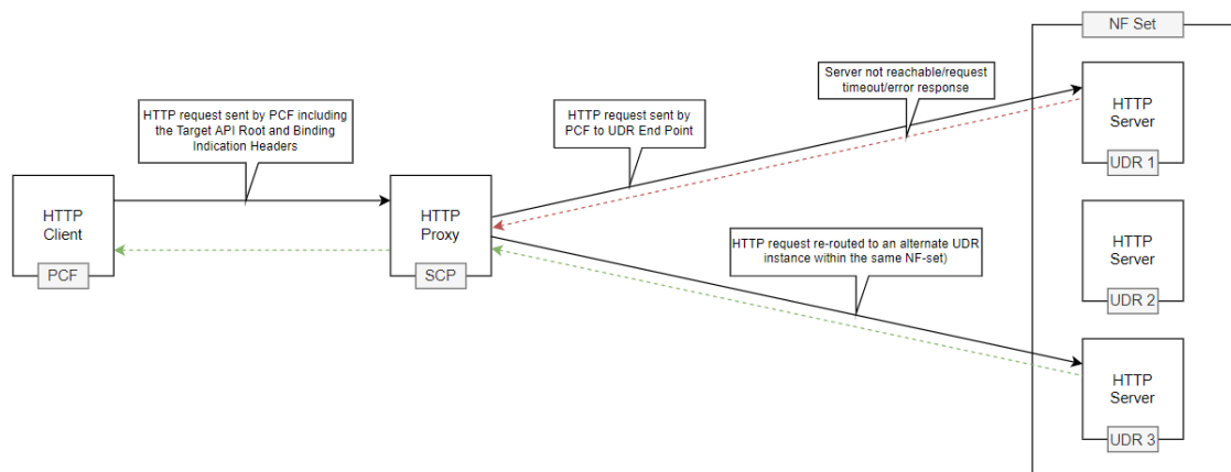
Figure 4-99 Example of NF Set and Binding Header based Indirect Communication
