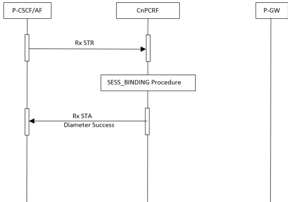
Figure 4-81 Cancellation of subscription to notification of the AF Signaling Transmission in 4G
