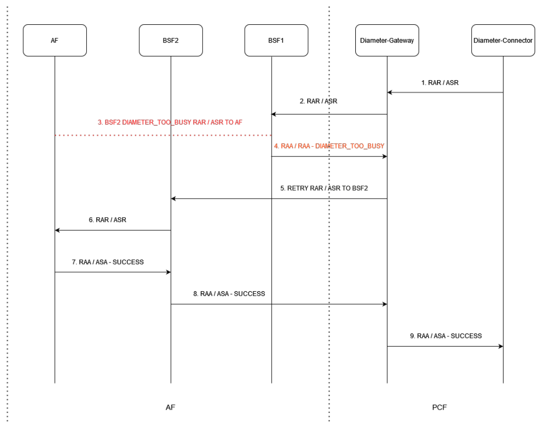
Figure 4-70 RX RAR/RX ASR Retry - Error Originated by Intermediate Peer
