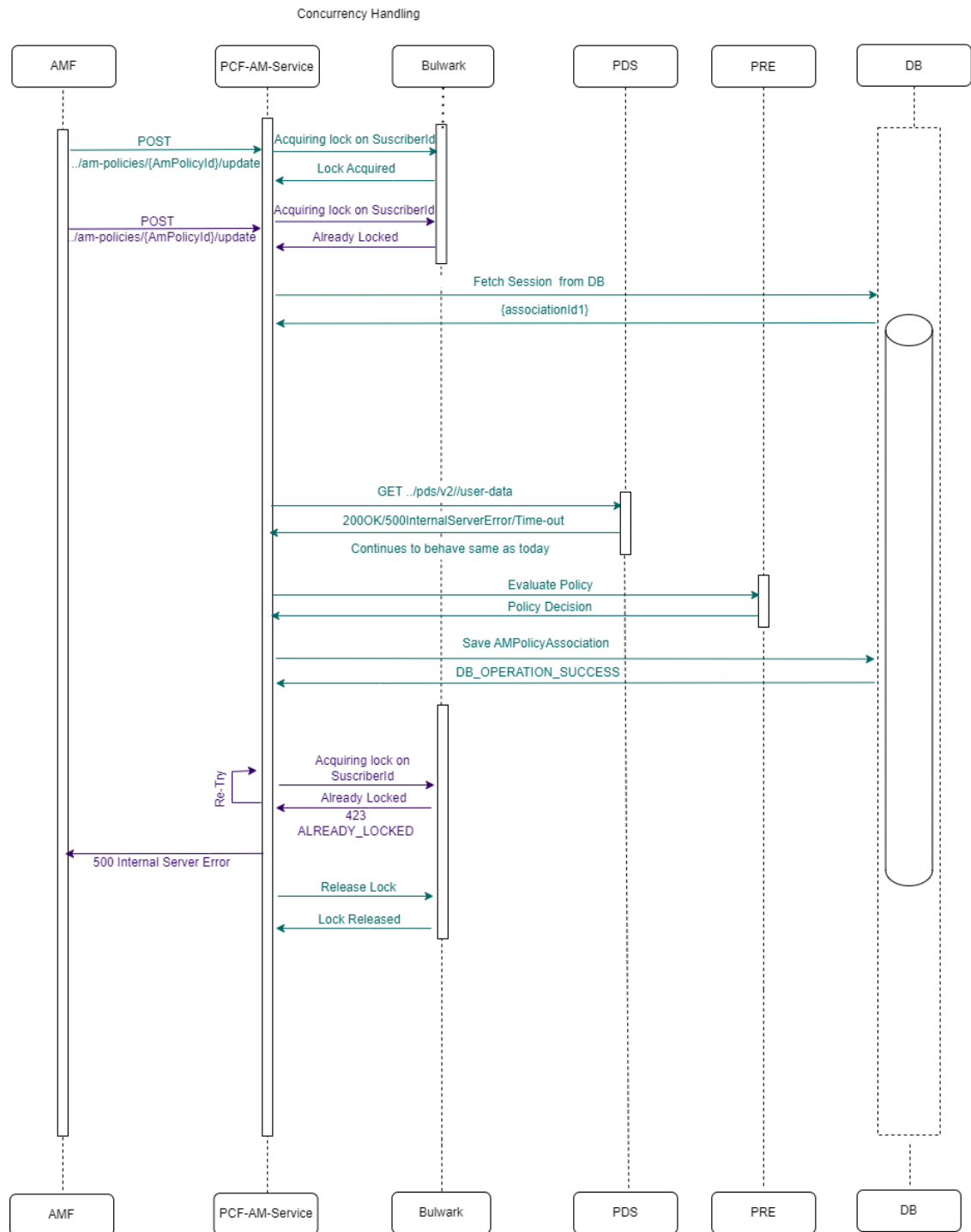
Figure 4-134 Two AM-Update requests for same Subscriber but different Sessions and retry failure (retry =1)
