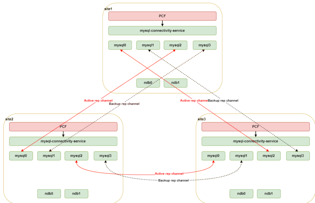
Figure 4-101 Three-Site Georedundancy Deployment
