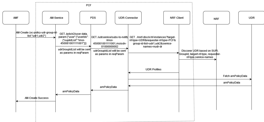
Figure 4-50 AMF sends AM Policy Association Request with oc-policy-udr-group-id
