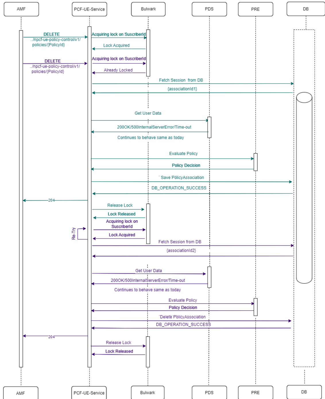
Figure 4-139 Two UE-Delete requests for same Subscriber and retry success.
