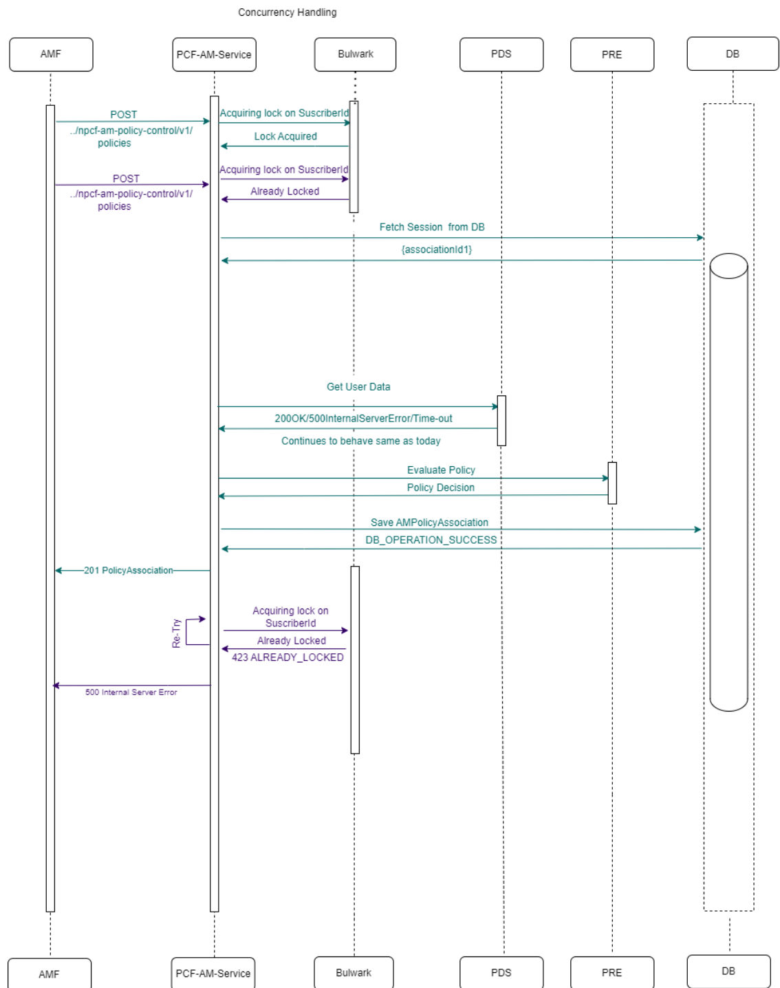
Figure 4-130 Two AM-Create requests for same Subscriber and retry failure (retry =1)
