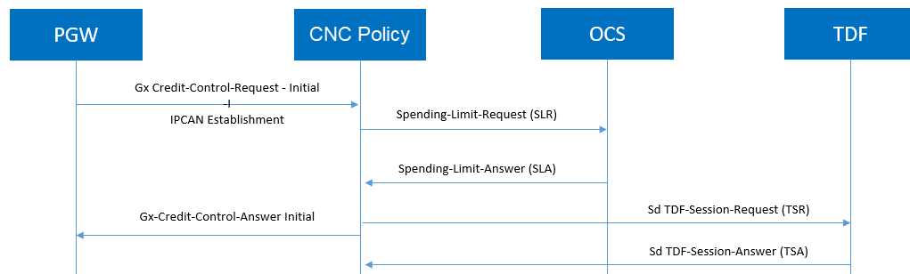
Figure 4-151 Call Flow for TDF Session
