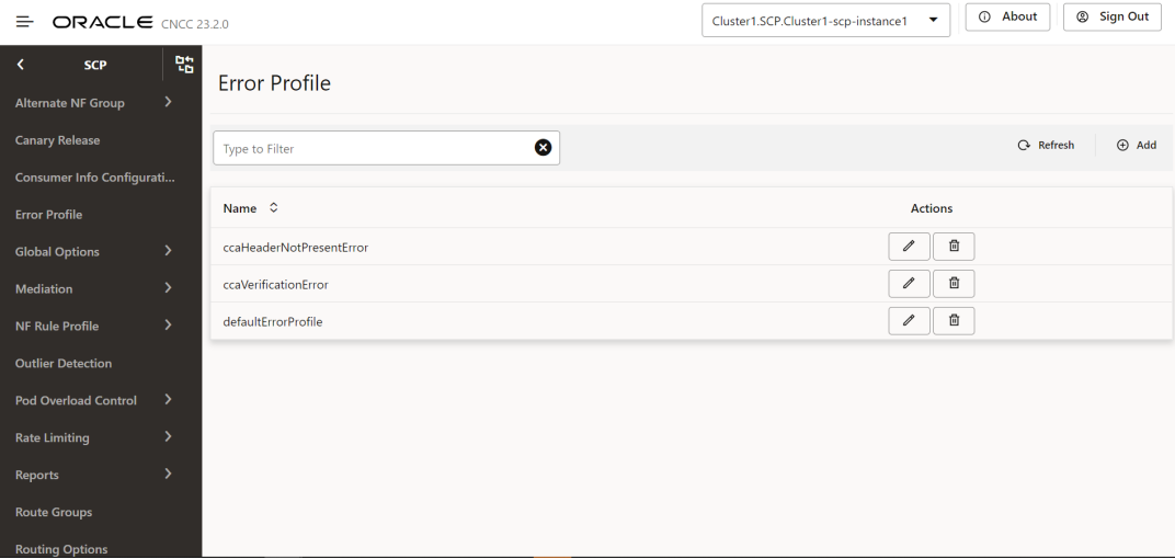
Figure 4-33 Error Profile
