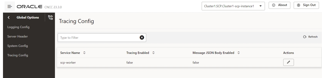
Figure 4-41 Tracing Config
