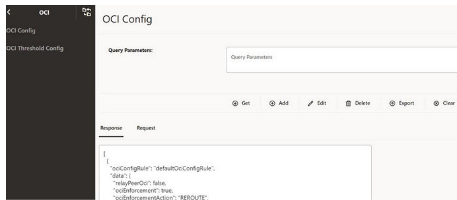
Figure 4-25 OCI Config
