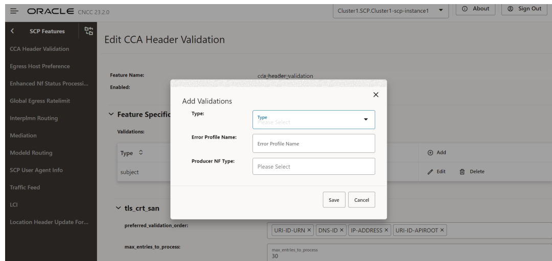
Figure 4-17 Add Validations
