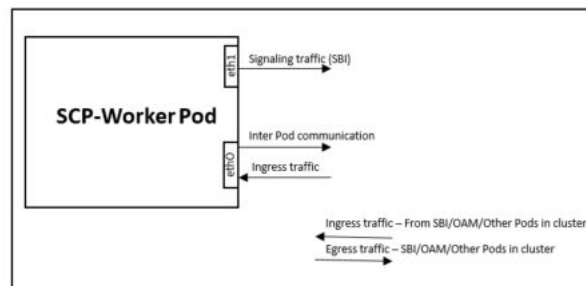
Figure 3-12 Networking-Multus Support
