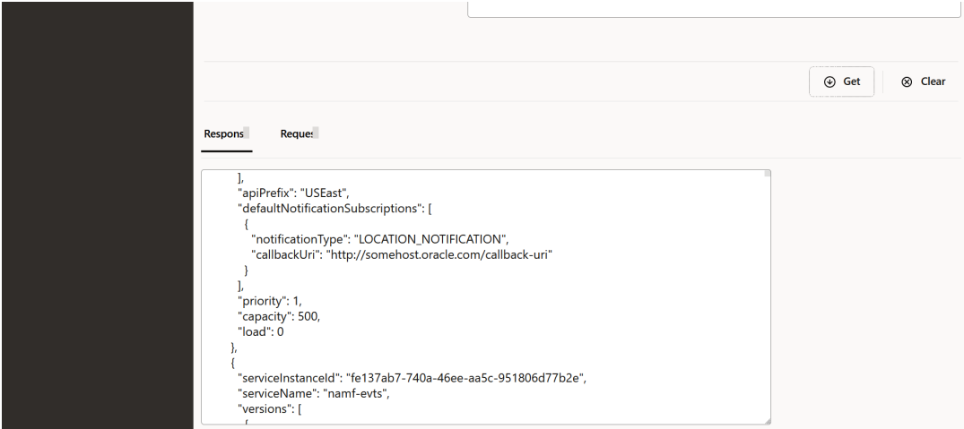
Figure 4-54 Response data
