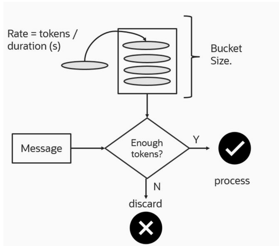
Figure 3-17 Algorithm Overview
