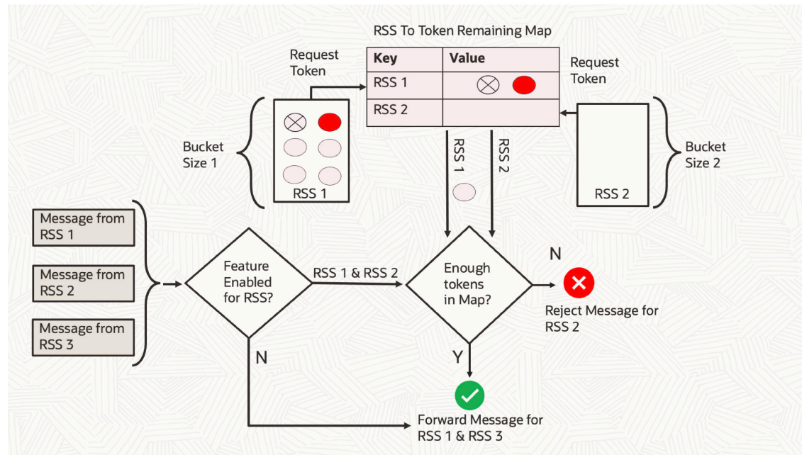
Figure 3-40 Token Bucket Algorithm
