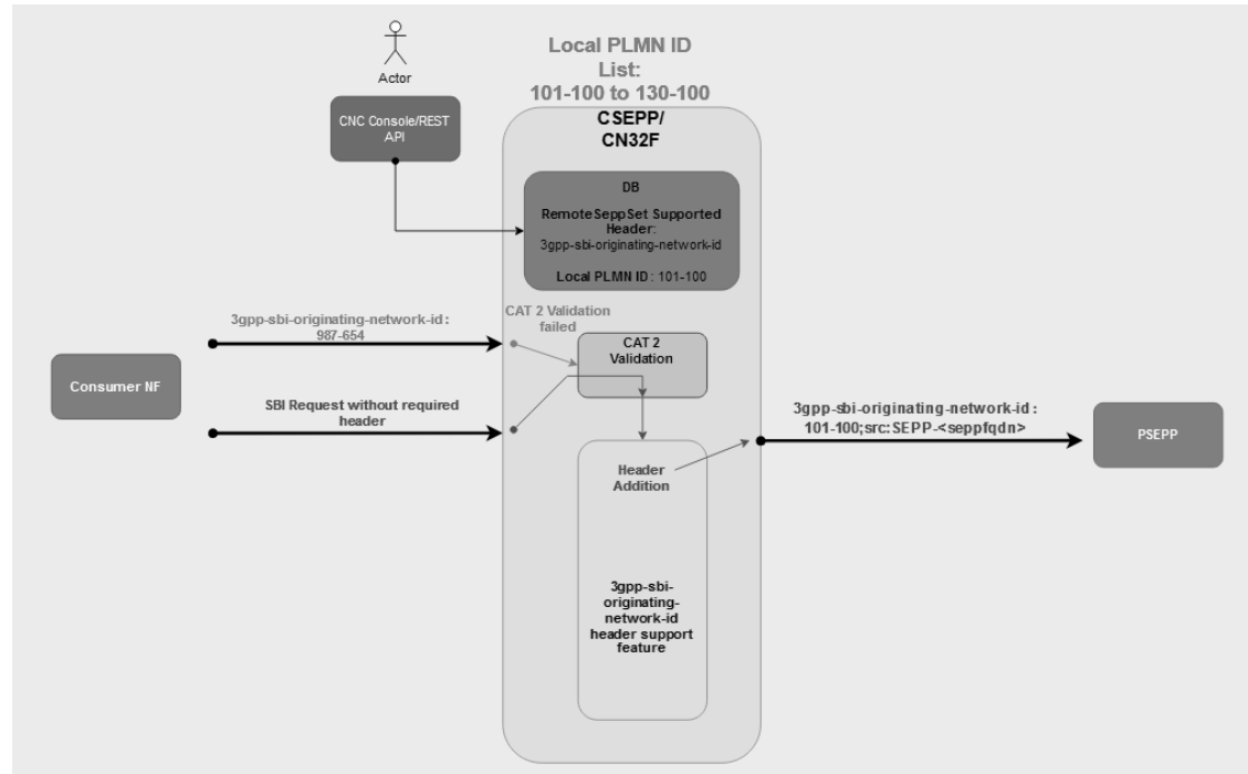
Figure 3-5 C SEPP side functionality
