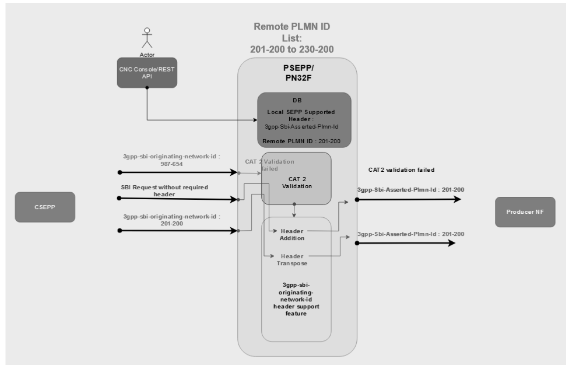
Figure 3-6 P SEPP side functionality
