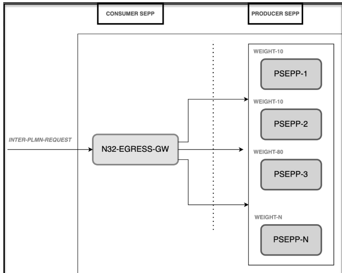
Figure 3-8 Architecture
