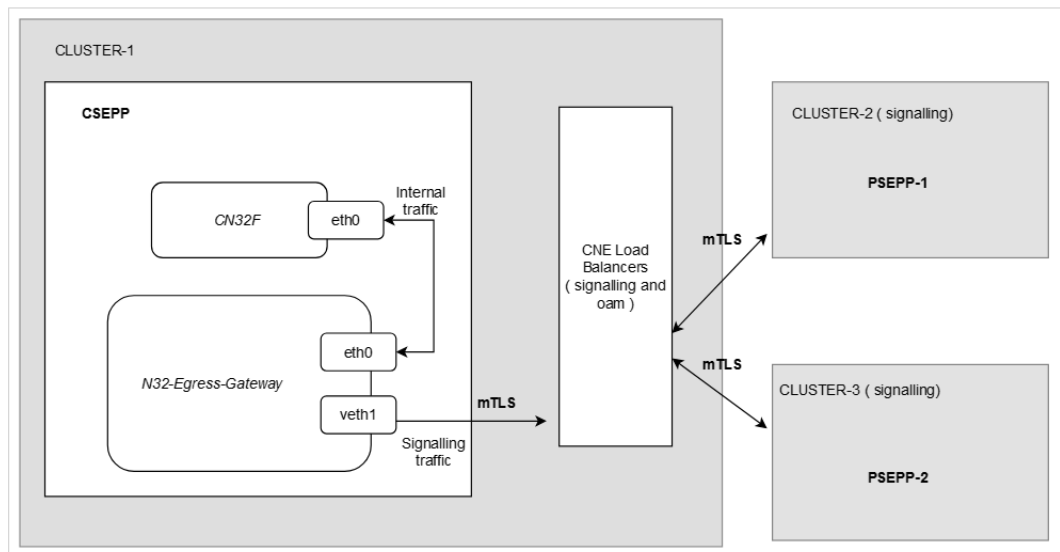
Figure 3-4 Egress Traffic Segregation
