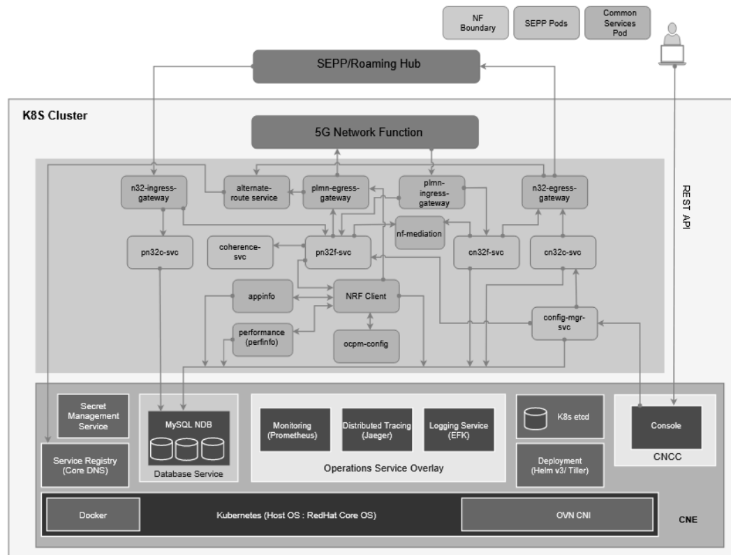
Figure 2-2 Security Edge Protection Proxy Architecture
