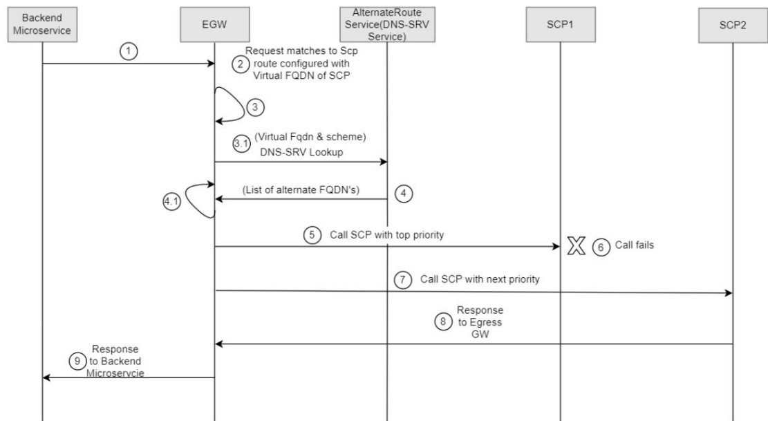
Figure 3-48 Priority Based Routing
