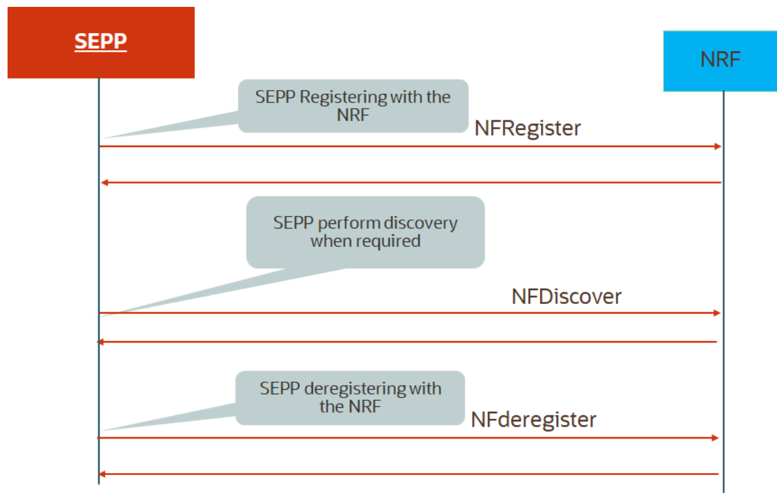
Figure 3-31 NRF Interface Registration & Reregistration.
