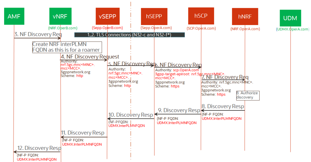
Figure 3-29 SEPP sets the 3GPP-SBI-Target-APIroot header
