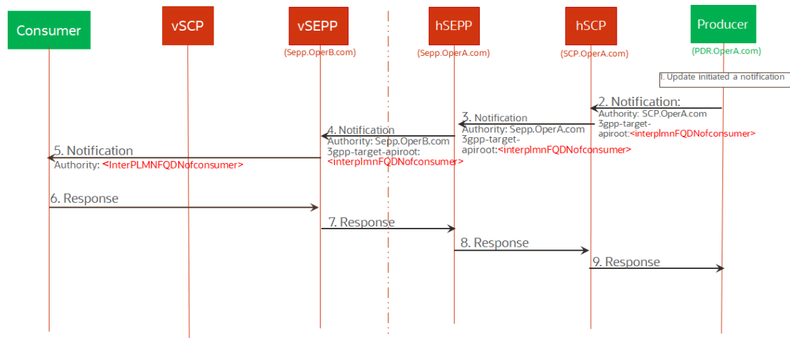
Figure 3-30 SEPP removes the 3GPP-SBI-Target-APIroot header
