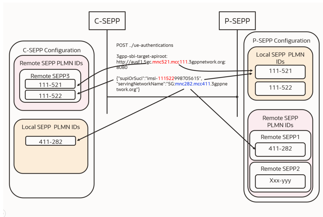
Figure 3-56 SEPP Mode
