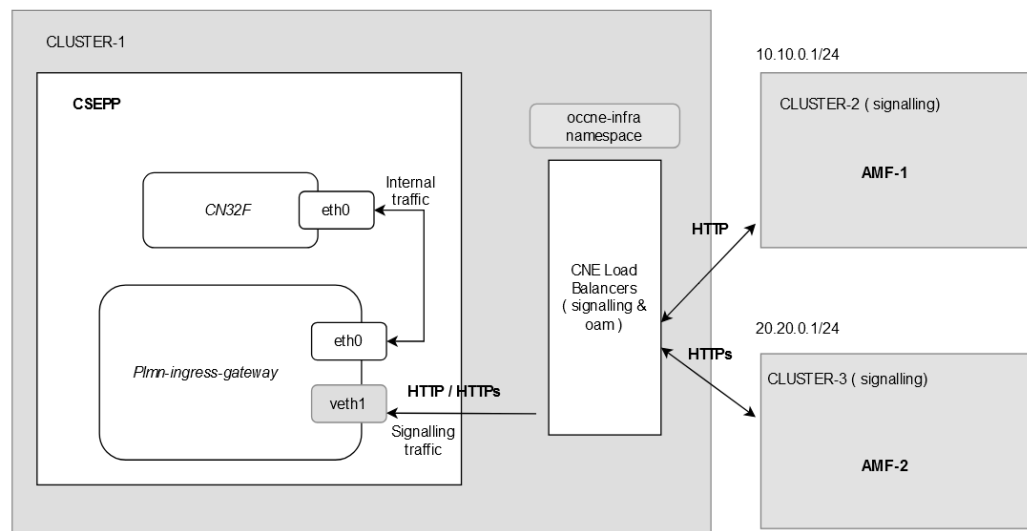
Figure 3-3 Ingress Traffic Segregation
