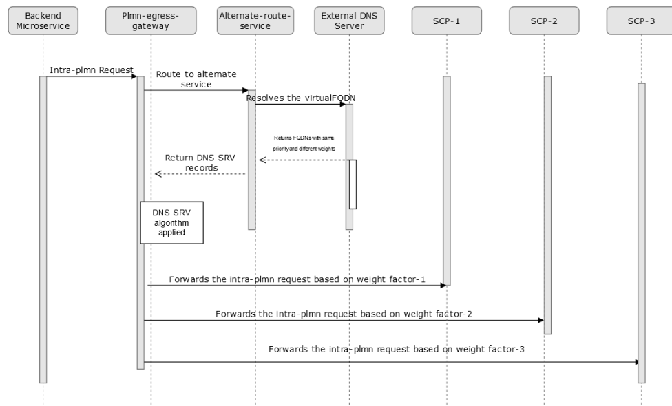
Figure 3-49 Weight Based Routing or Load Sharing
