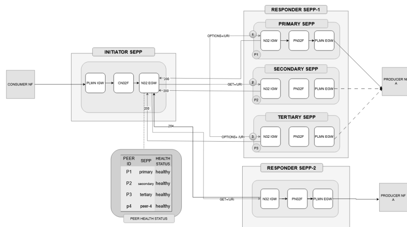
Figure 3-2 Proactive Status Updates on SEPP Architecture
