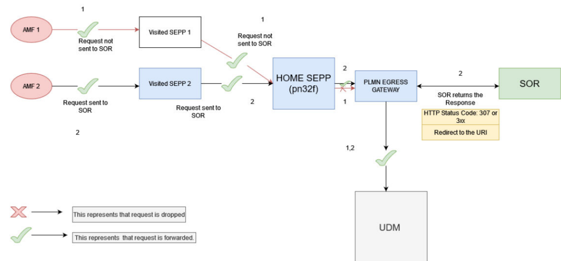
Figure 3-39 Redirection Enabled Mode
