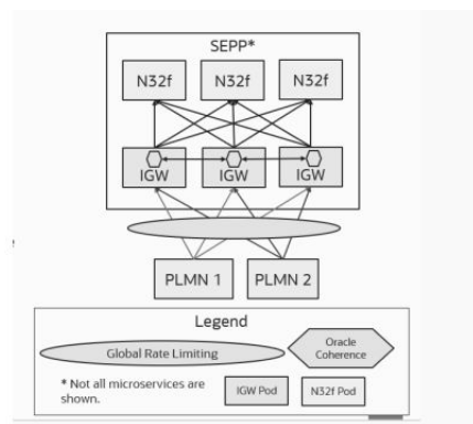
Figure 3-18 Architecture
