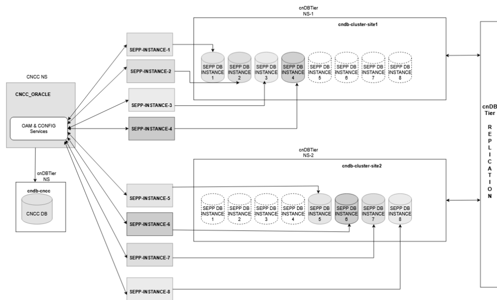
Figure 3-1 Multiple SEPP instances on shared cnDBTier cluster architecture
