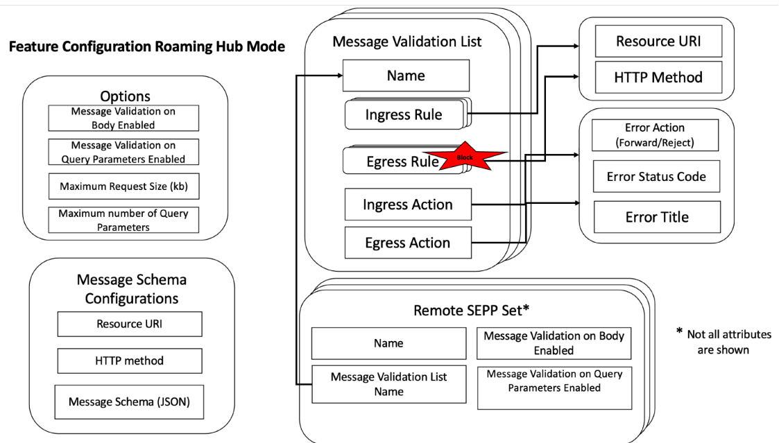
Figure 3-54 CNC Console options available for Cat - 0 SBI Message Schema Validation feature in Roaming Hub Mode
