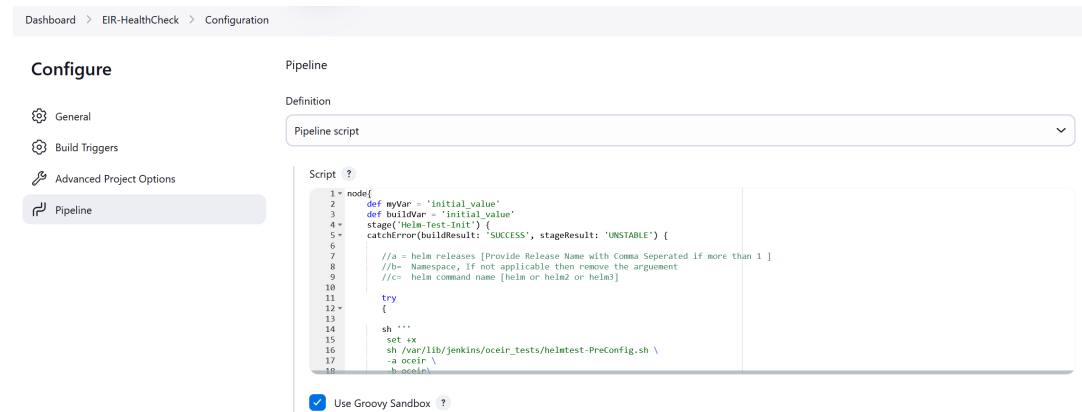
Figure 4-109 EIR-HealthCheck Pipeline configuration
