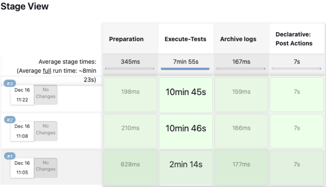
Figure 4-20 Sample Screen: NRF-ATS Full Execution
