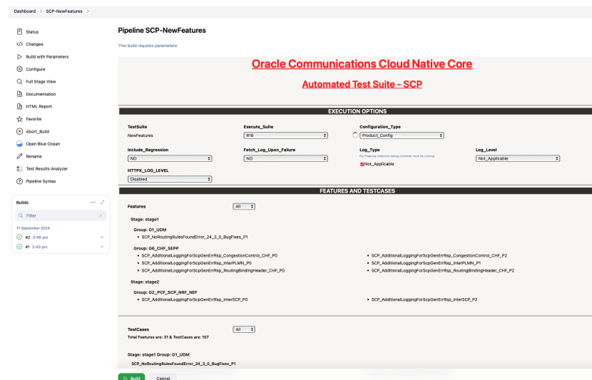
Figure 4-34 Build
