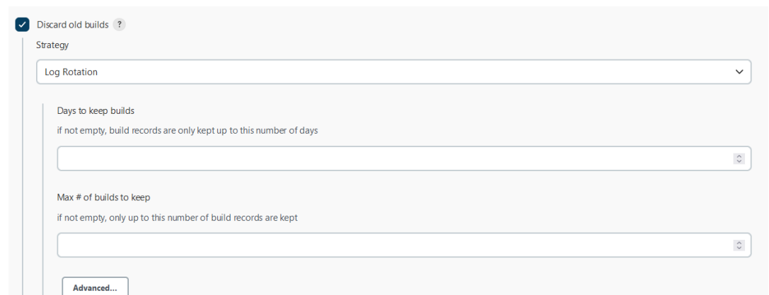
Figure 4-104 Discard Builds
