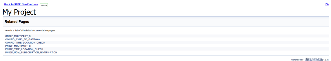
Figure 4-49 Documentation
