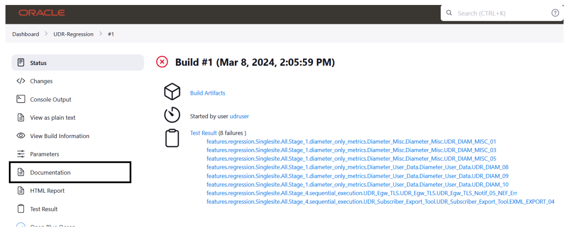
Figure 4-98 UDR-Regression Documentation
