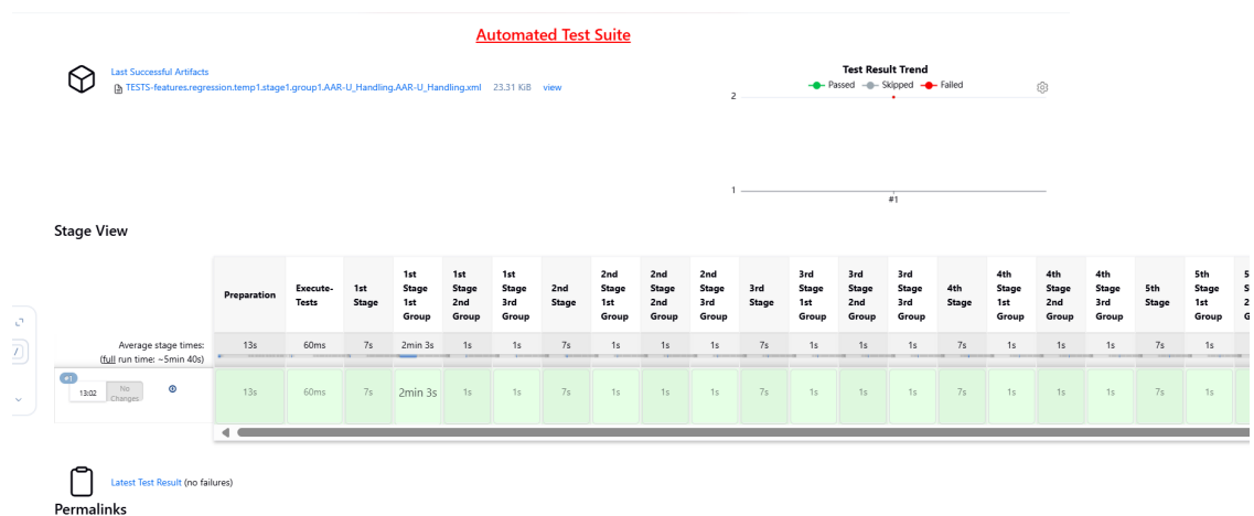
Figure 4-11 BSF_Regression Pipeline
