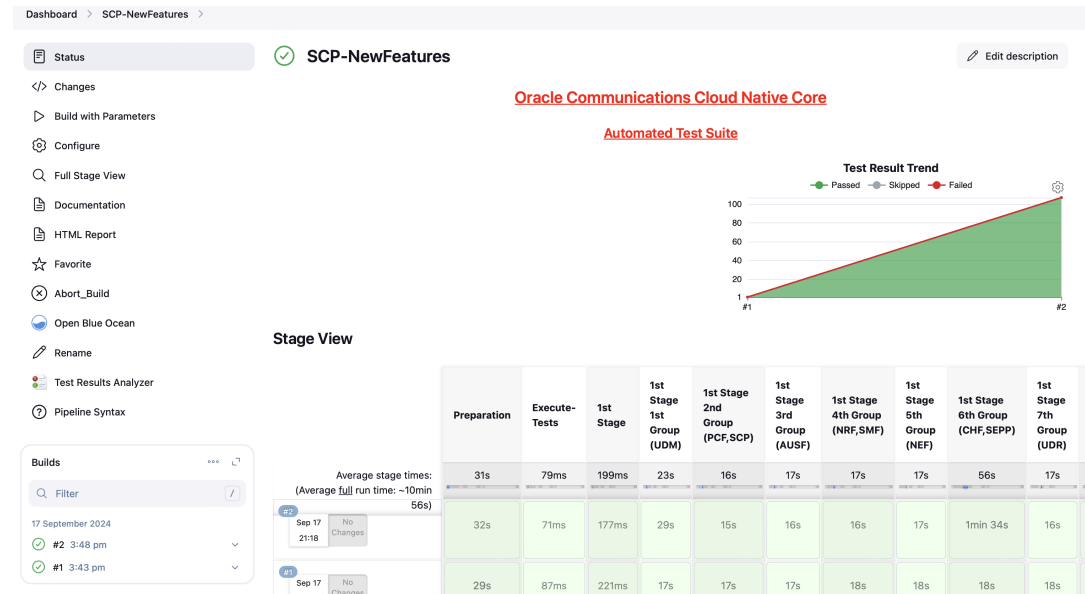
Figure 4-32 SCP-NewFeatures
