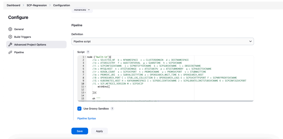
Figure 4-39 Regression - Pipeline Script
