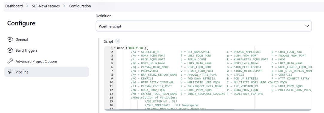
Figure 4-63 SLF Configuration page
