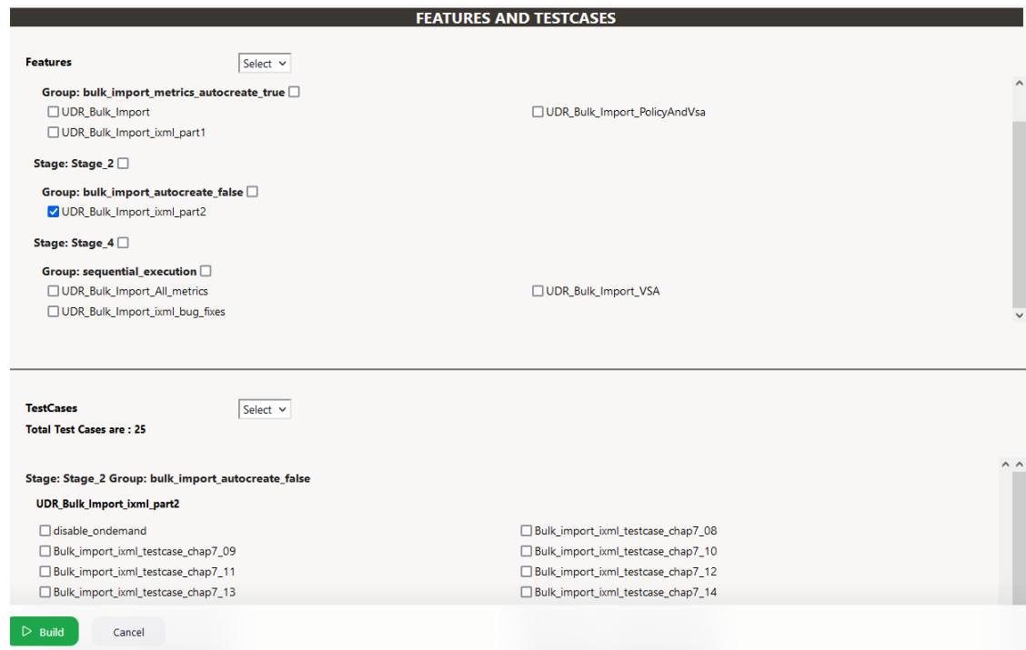
Figure 2-18 Multiselect Features and Scenarios
