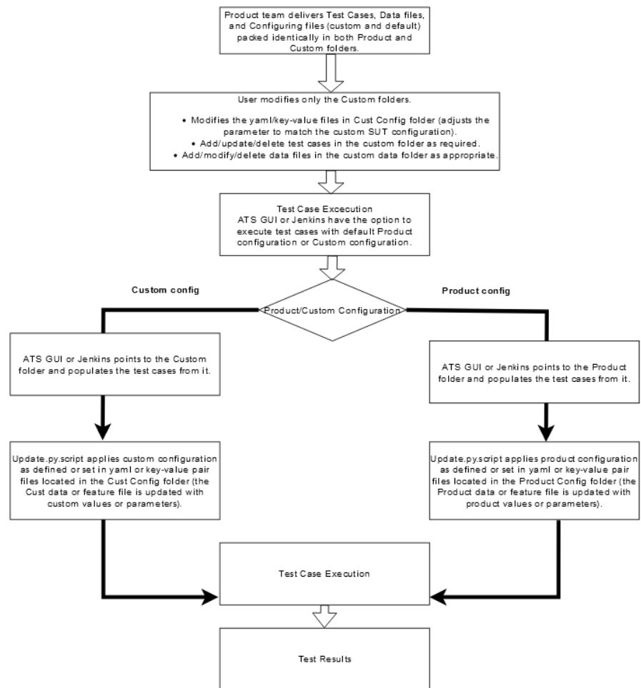
Figure 2-71 ATS Execution Flow
