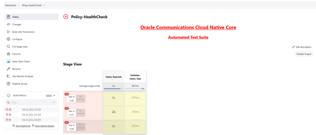
Figure 2-31 Configure Healthcheck
