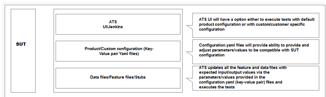
Figure 2-69 SUT Design Summary
