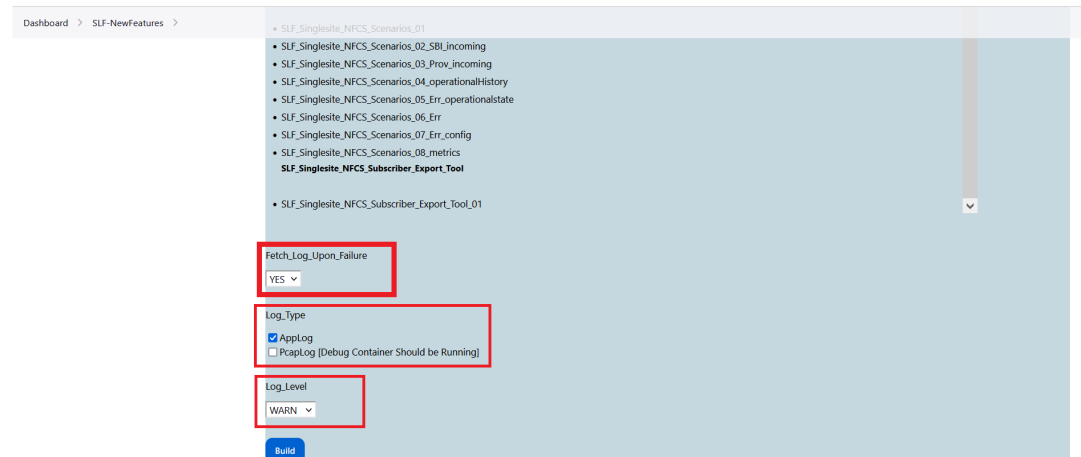
Figure 4-55 SLF-NewFeatures BuildWithParameters
