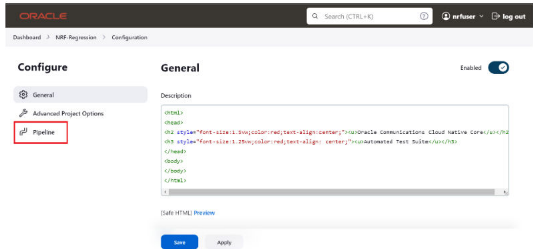
Figure 4-17 Pipeline Tab
