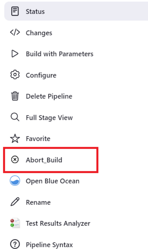
Figure 2-11 Abort Build
