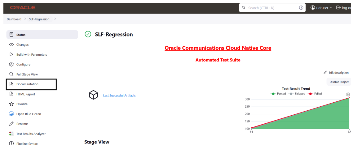
Figure 4-80 SLF-Regression Documentation
