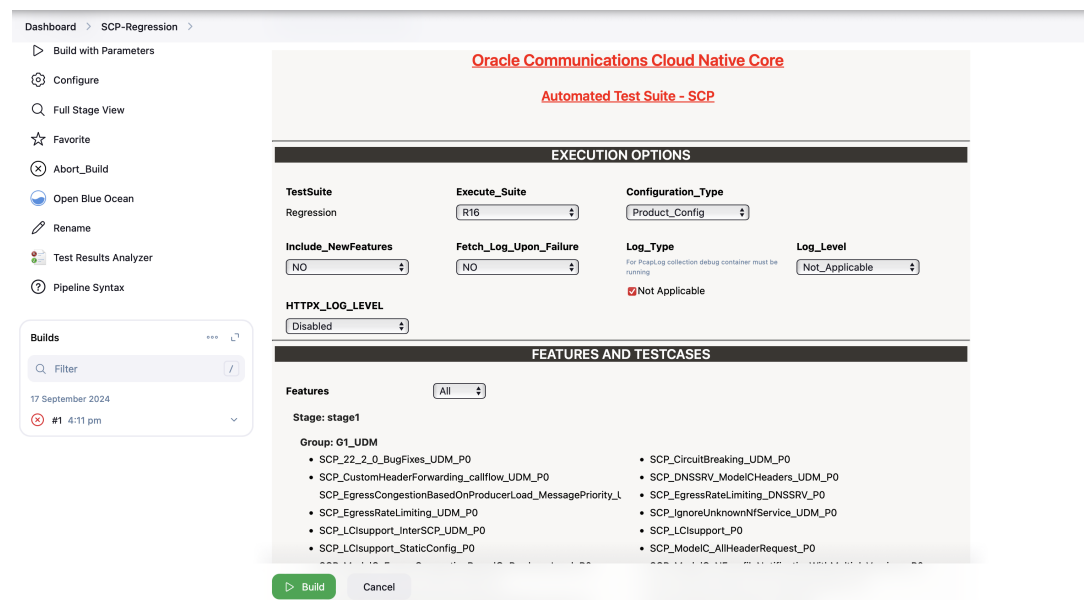
Figure 4-38 SCP-Regression Pipeline
