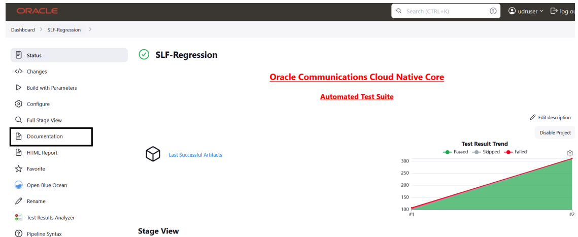
Figure 4-79 SLF-Regression Documentation
