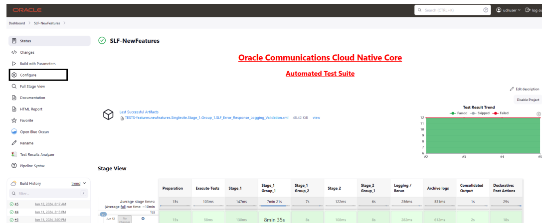
Figure 4-61 SLF-NewFeatures Configure
