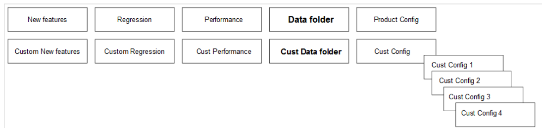
Figure 2-70 Folder Structure
