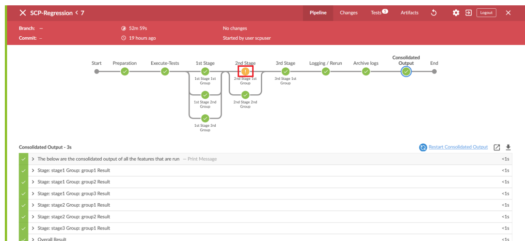
Figure 2-66 Executed Groups
