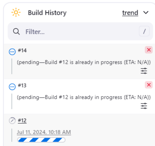
Figure 2-10 Stopping Builds
