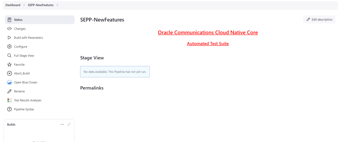
Figure 4-45 SEPP-NewFeatures Pipeline
